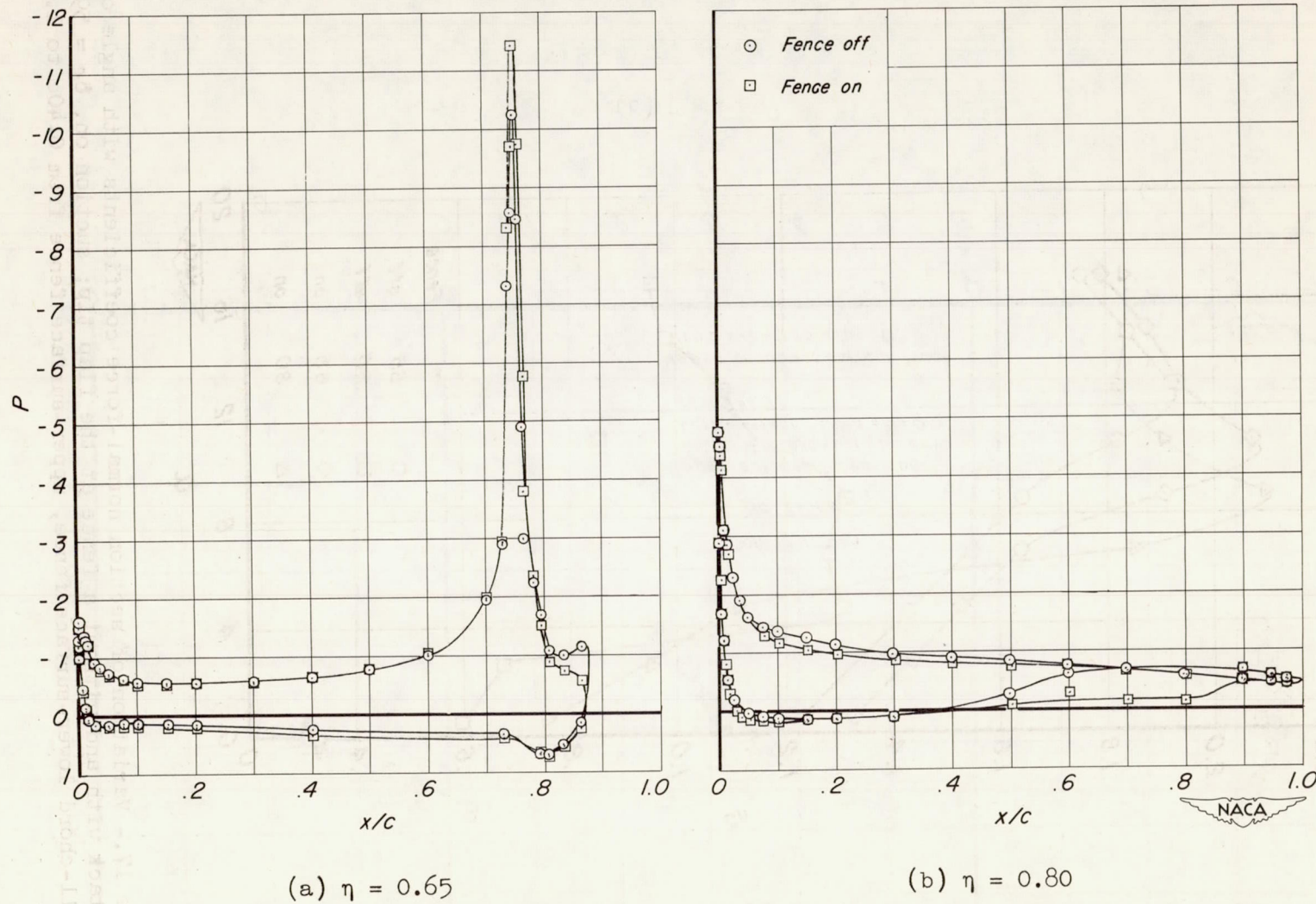
Figure 16.- Typical chordwise pressure distributions for the model with and without fence; suction on, \delta_f = 59^\circ , \alpha = 0.5^\circ .
