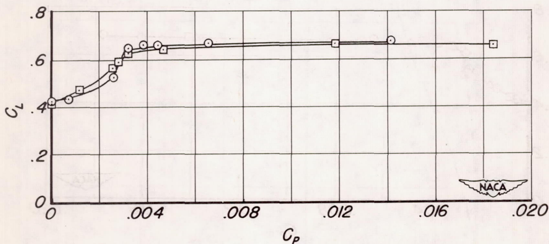
(a) Variation of lift coefficient with flow and power coefficient.
