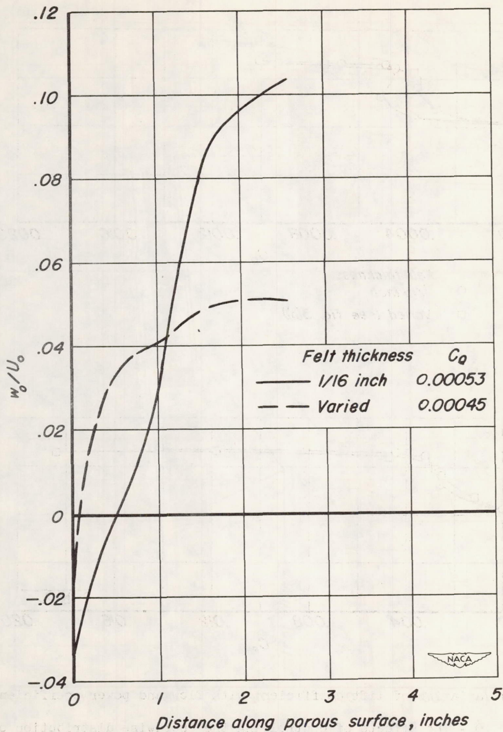
(b) Chordwise distribution of suction-air velocities.
