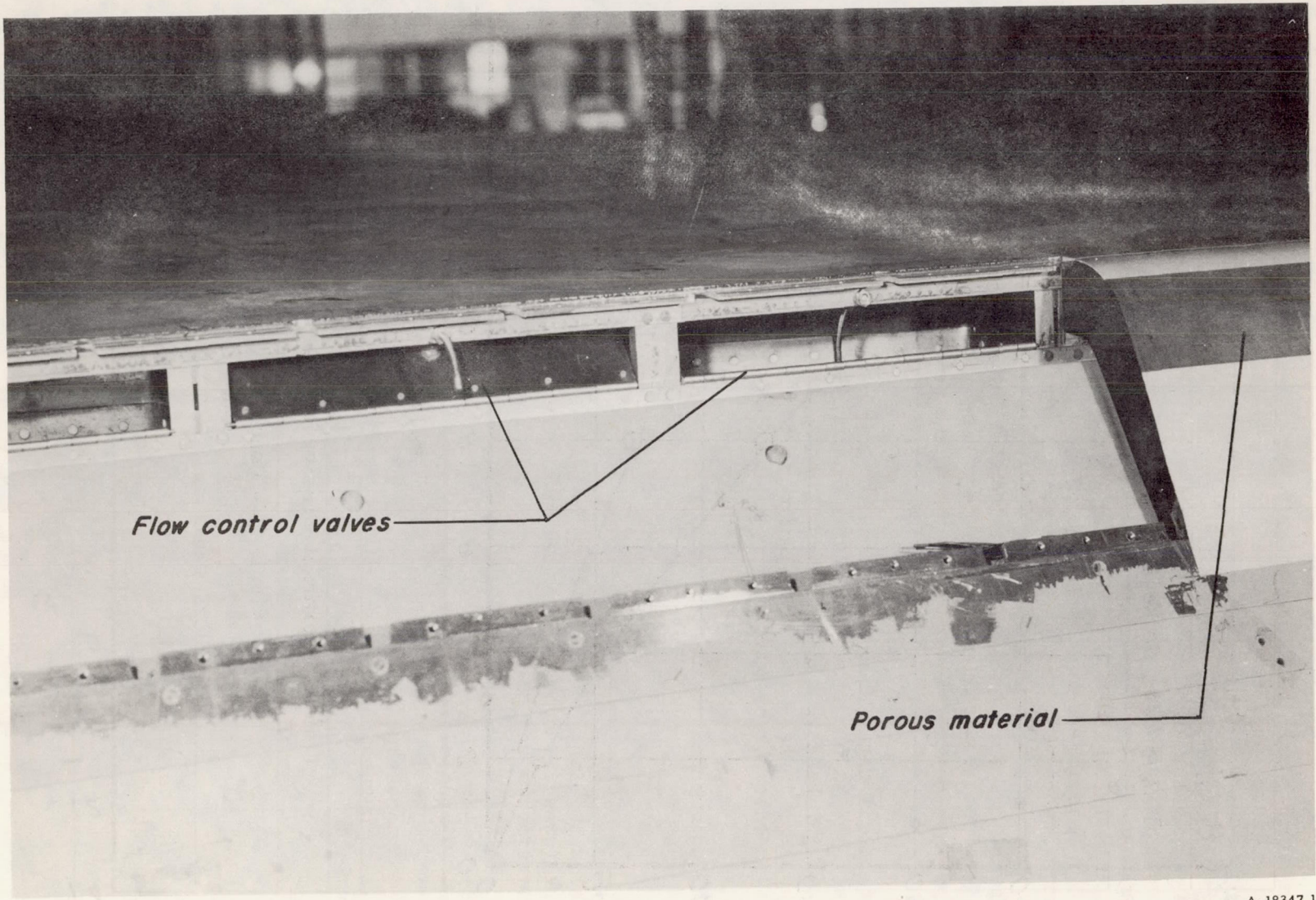
Figure 4.- Photograph of porous material insert and wing ducts.
