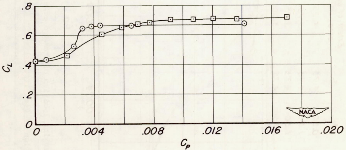
Figure 6.- Typical variation of flap lift increment with flow and power coefficient for two flap deflections; \alpha = 0.5^\circ .
