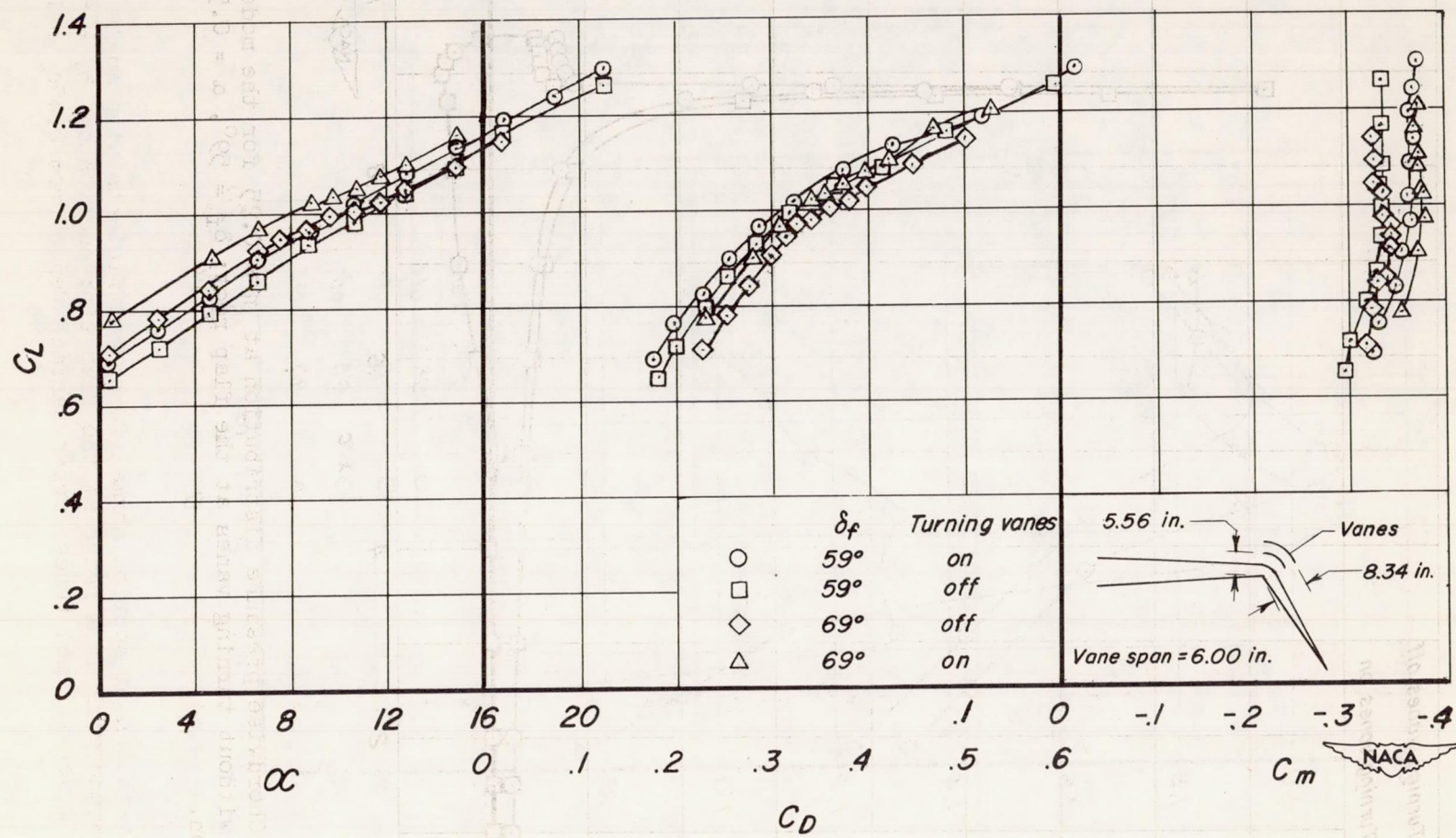
Figure 18.- Aerodynamic characteristics of the model with the flap deflected and with turning vanes at the flap root; suction on.
