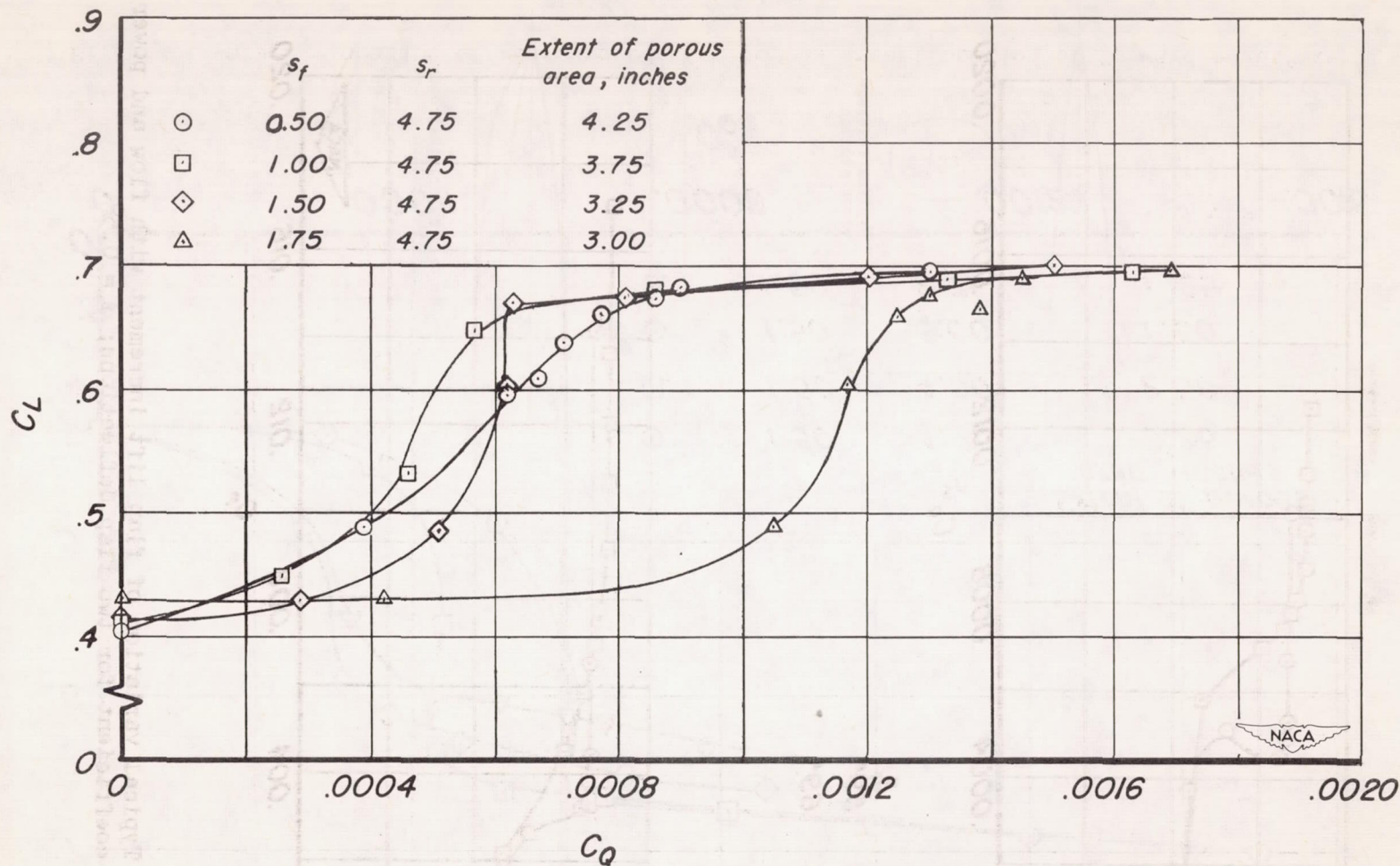
(a) Effect of varying location of forward edge of porous area (location of rearward edge fixed).
