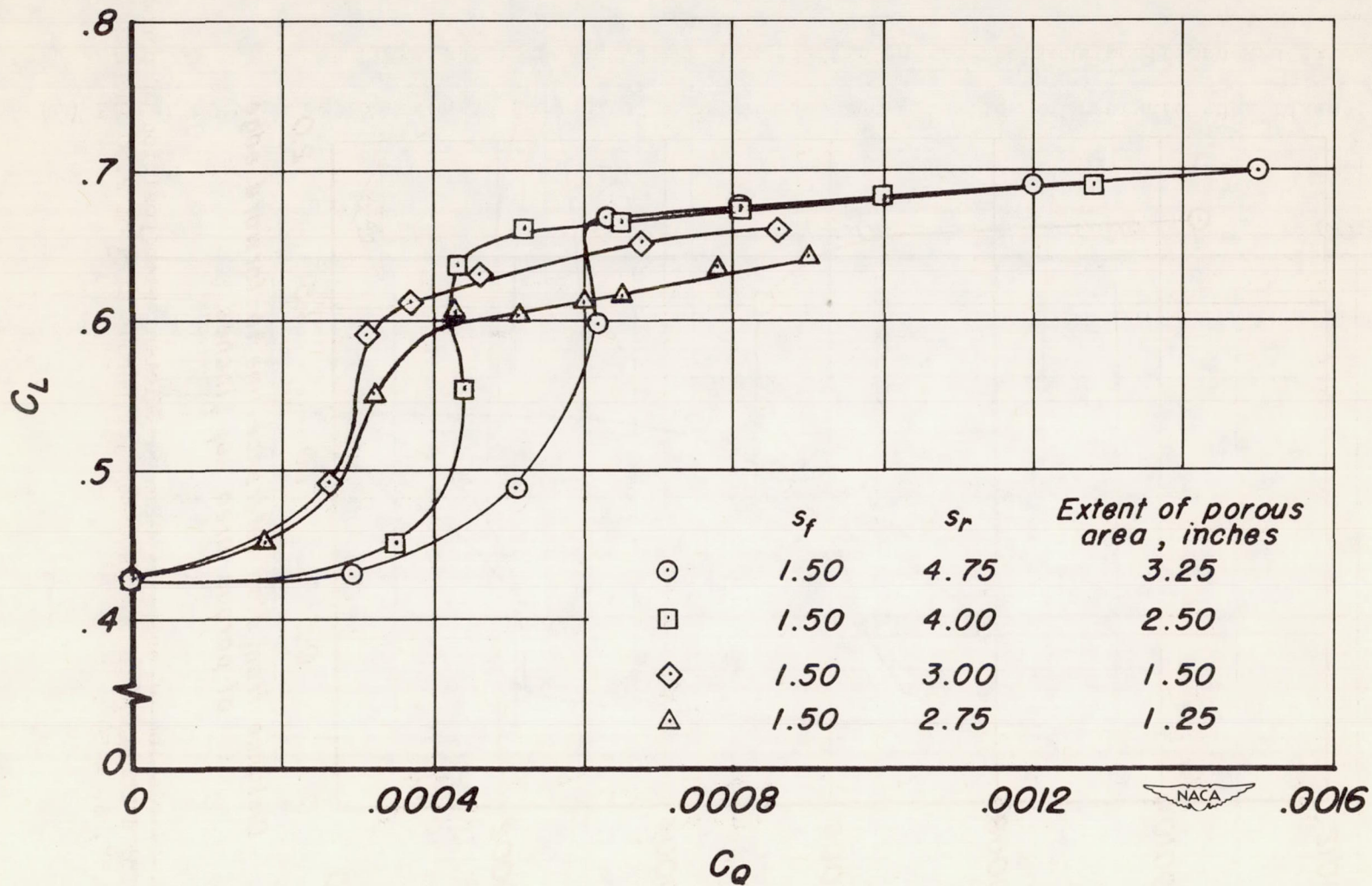
(b) Effect of varying location of rearward edge of porous area (location of forward edge fixed).
