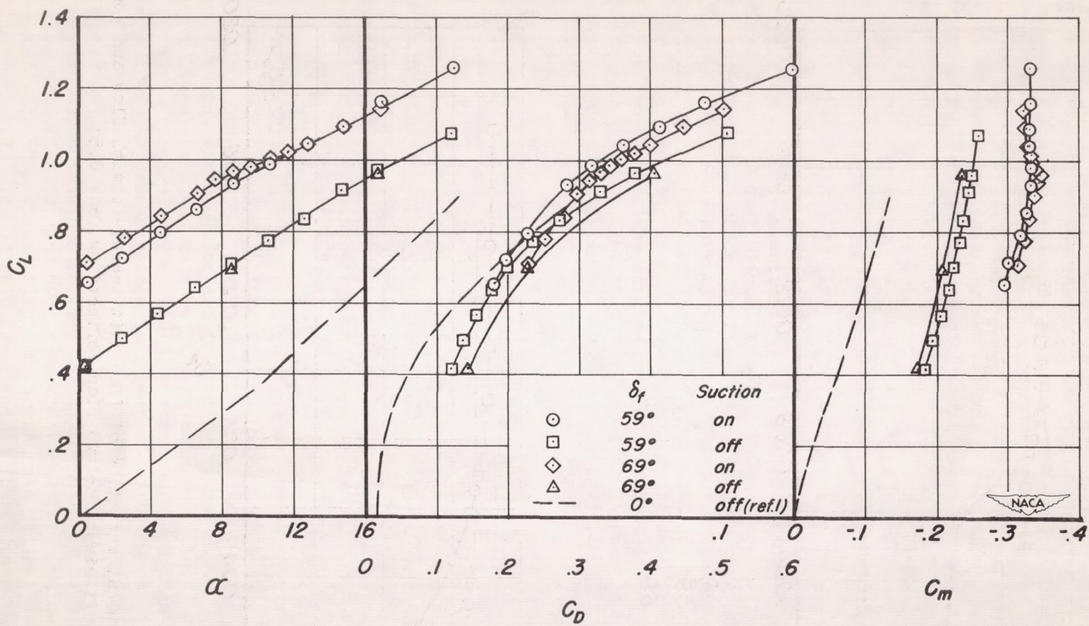
Figure 5.- Aerodynamic characteristics of the model with the suction flap deflected 59° and 69° with and without suction.
