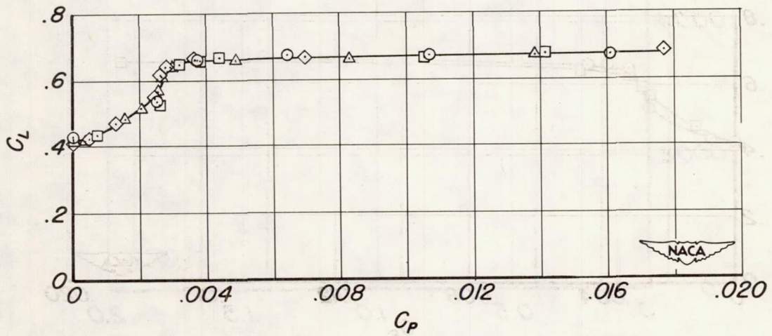
Figure 9.- Variation of lift coefficient with flow and power coefficient for various free-stream velocities; \alpha = 0.5^\circ , \delta_f = 59^\circ , S_f = 1.50 in., extent of porous area = 2.50 in.
