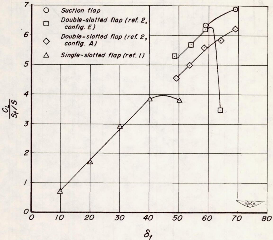
Figure 22.- Comparison of suction flap with single- and double-slotted flaps; \alpha = 0^\circ .
