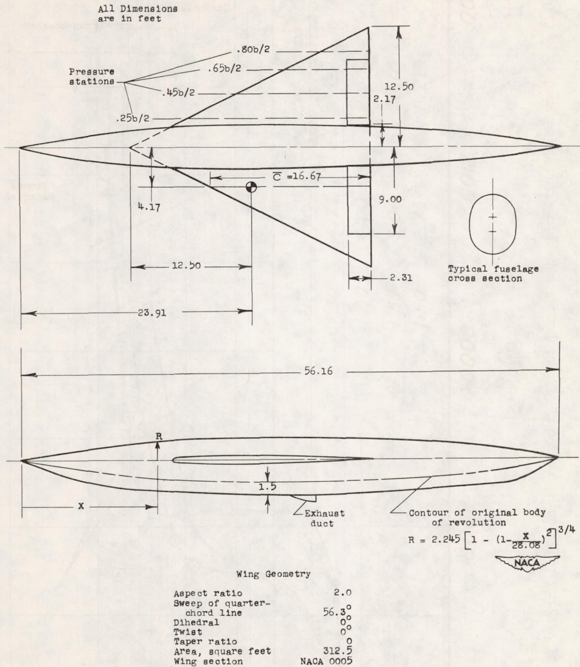
Figure 2.- Geometric characteristics of the model.
