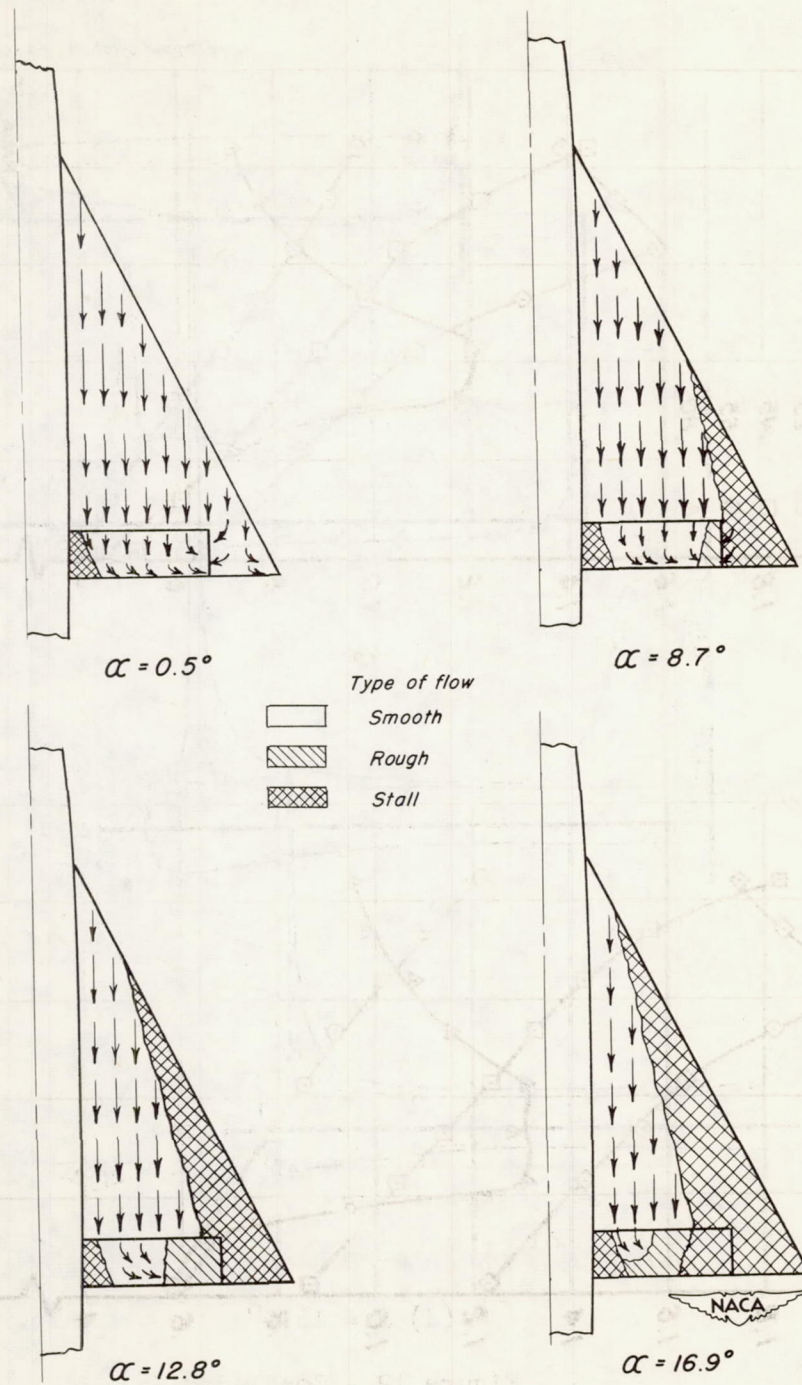
Figure 13.- Progression of flow separation with angle of attack for the model with suction; \delta_f = 59^\circ .
