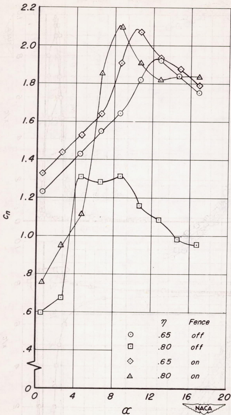
Figure 17.- Variation of section normal-force coefficients with angle of attack with and without a fence at the flap tip; suction on, \delta_f = 59^\circ , full-chord lower-surface fence, upper-surface fence from 0.40c to 1.00c.
