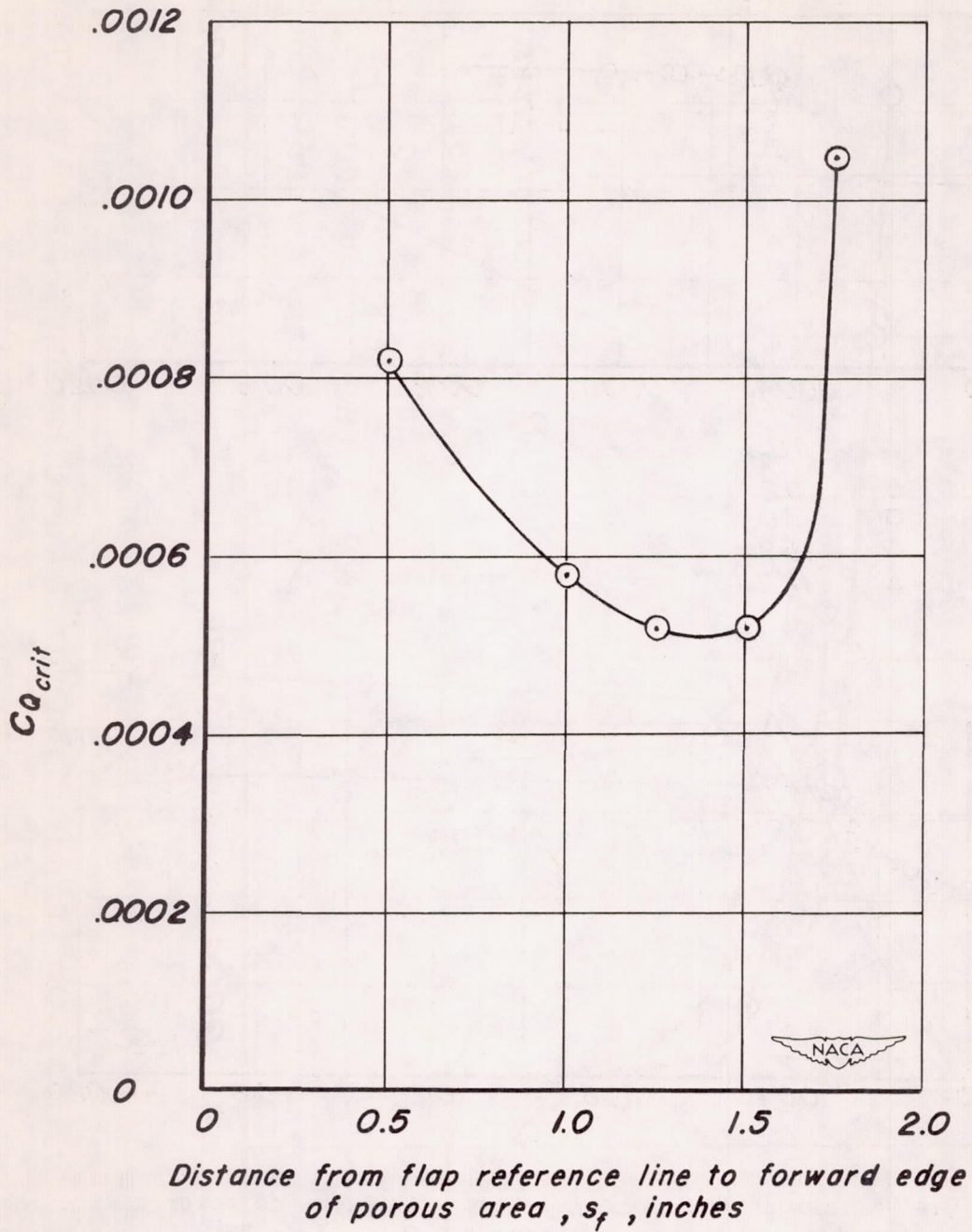
Figure 8.- Variation of critical flow coefficient with position of porous area for a constant chordwise extent of porous area of 2.50 inches; \alpha = 0.5^\circ , \delta_f = 59^\circ .
