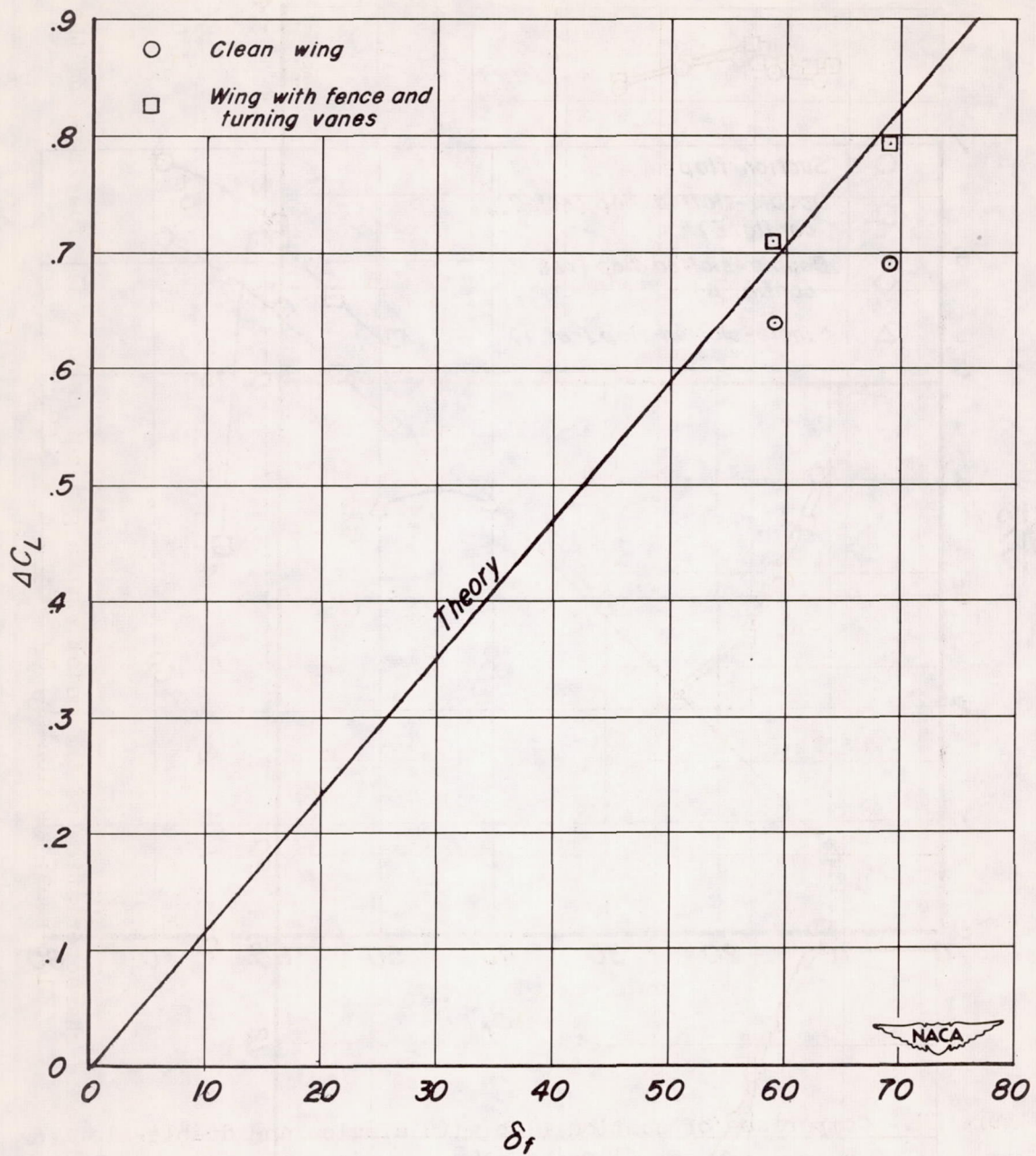
Figure 21.- Comparison of experimental flap lift increment with theory; \alpha = 0^\circ .
