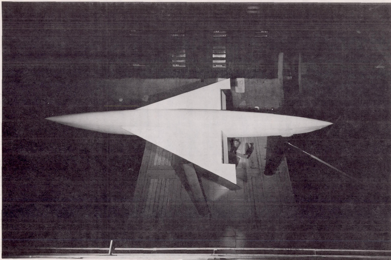
Figure 1.- View of triangular-wing model mounted in the 40- by 80-foot wind tunnel.
