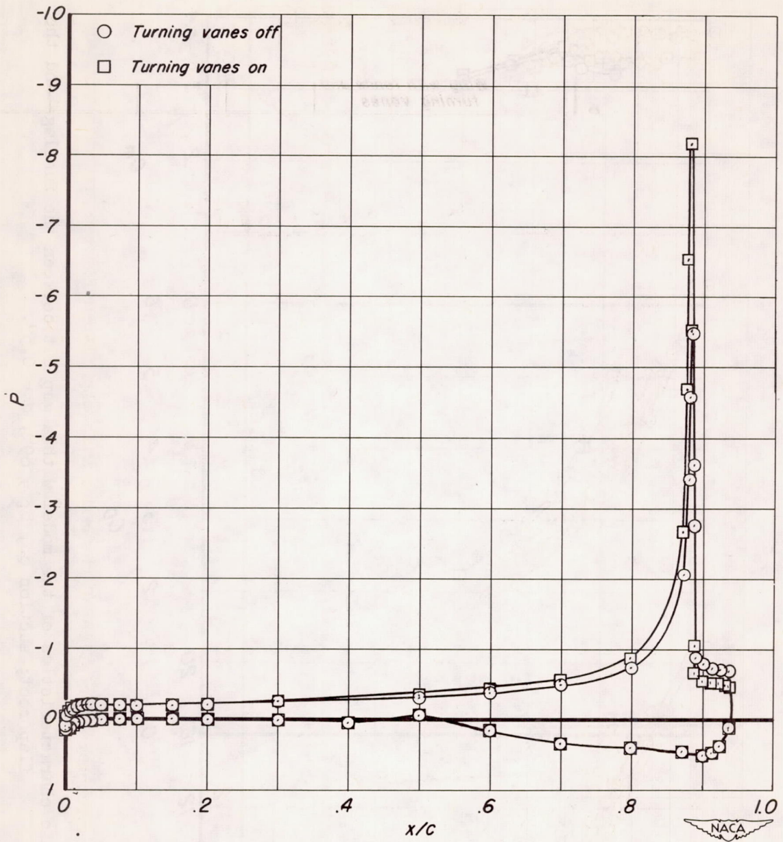
Figure 19.- Chordwise pressure distribution at \eta = 0.25 for the model with and without turning vanes at the flap root; \delta_f = 59^\circ , \alpha = 0.5^\circ , suction on.
