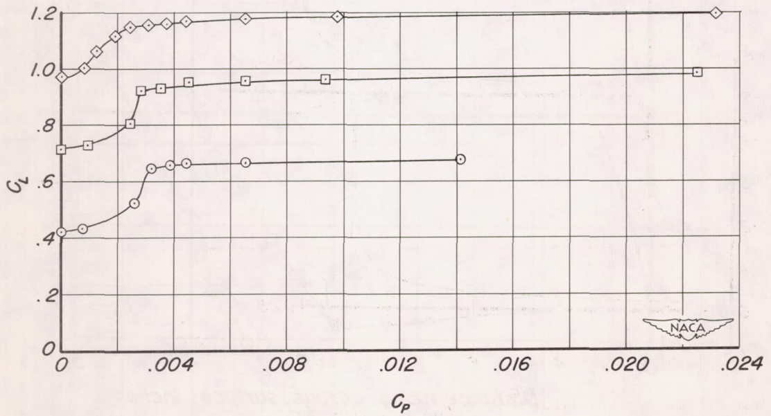
Figure 11.- Typical variation of lift coefficient with flow and power coefficients for various angles of attack; \delta_f = 59^\circ .
