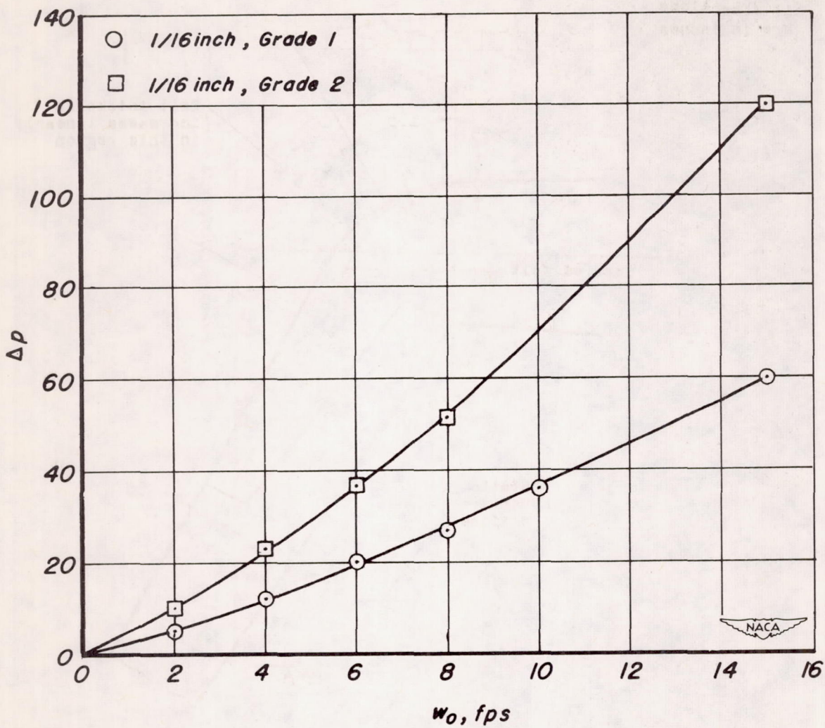
(c) Flow characteristics of felt backing.
