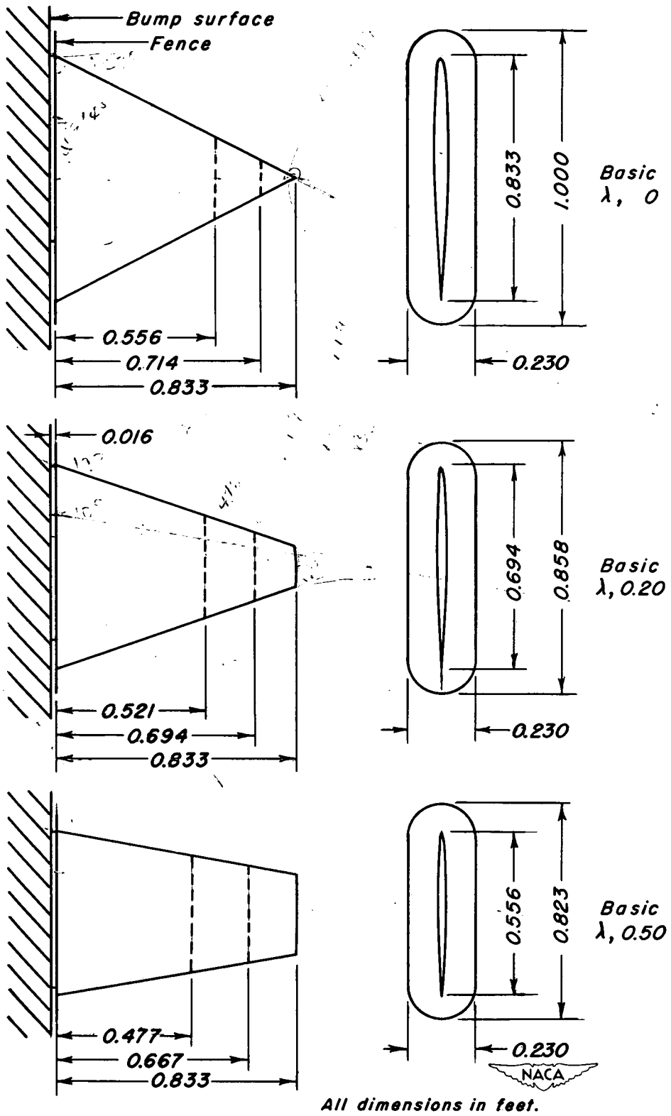
Figure 2.- Plan forms of the wings.
