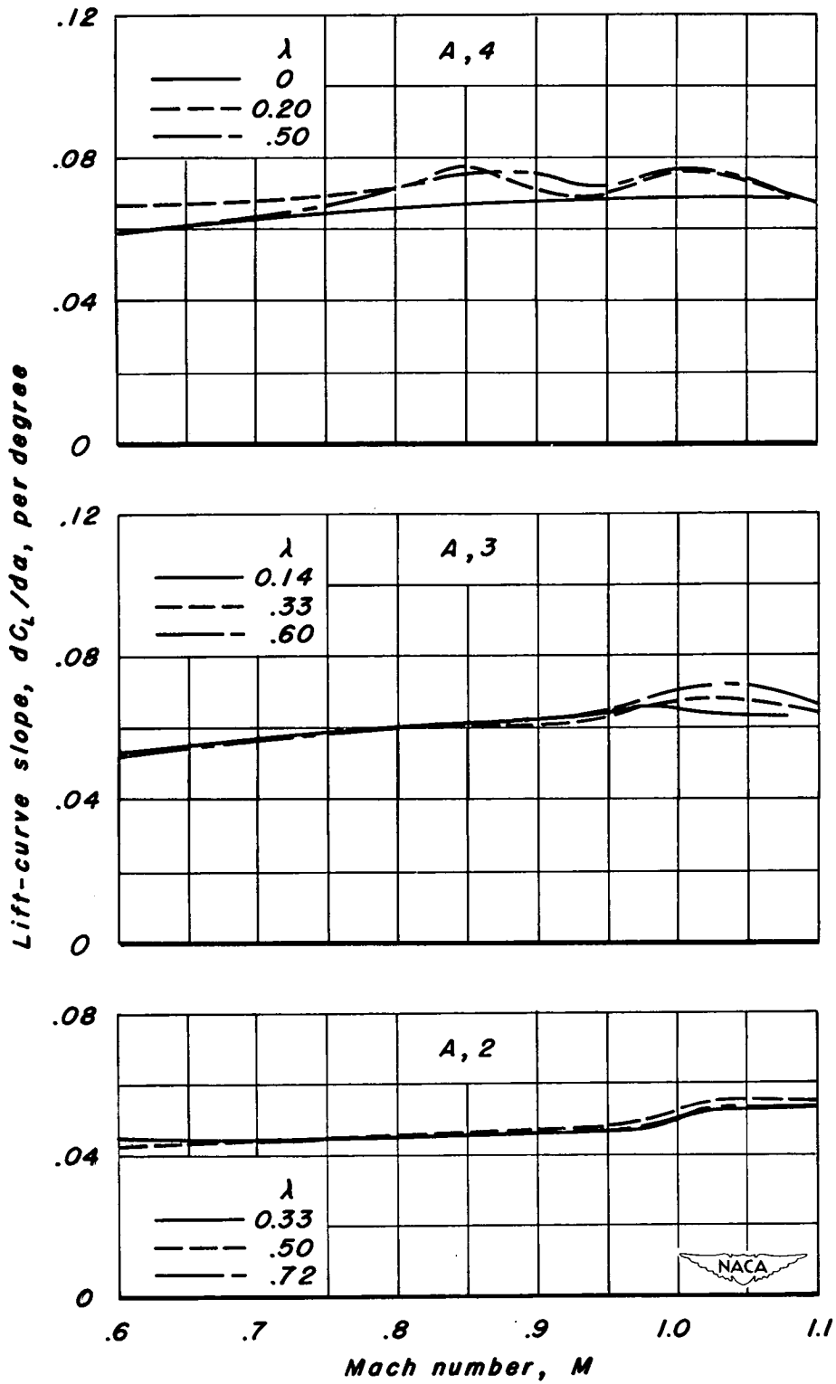
(a) NACA 63A008 sections.
