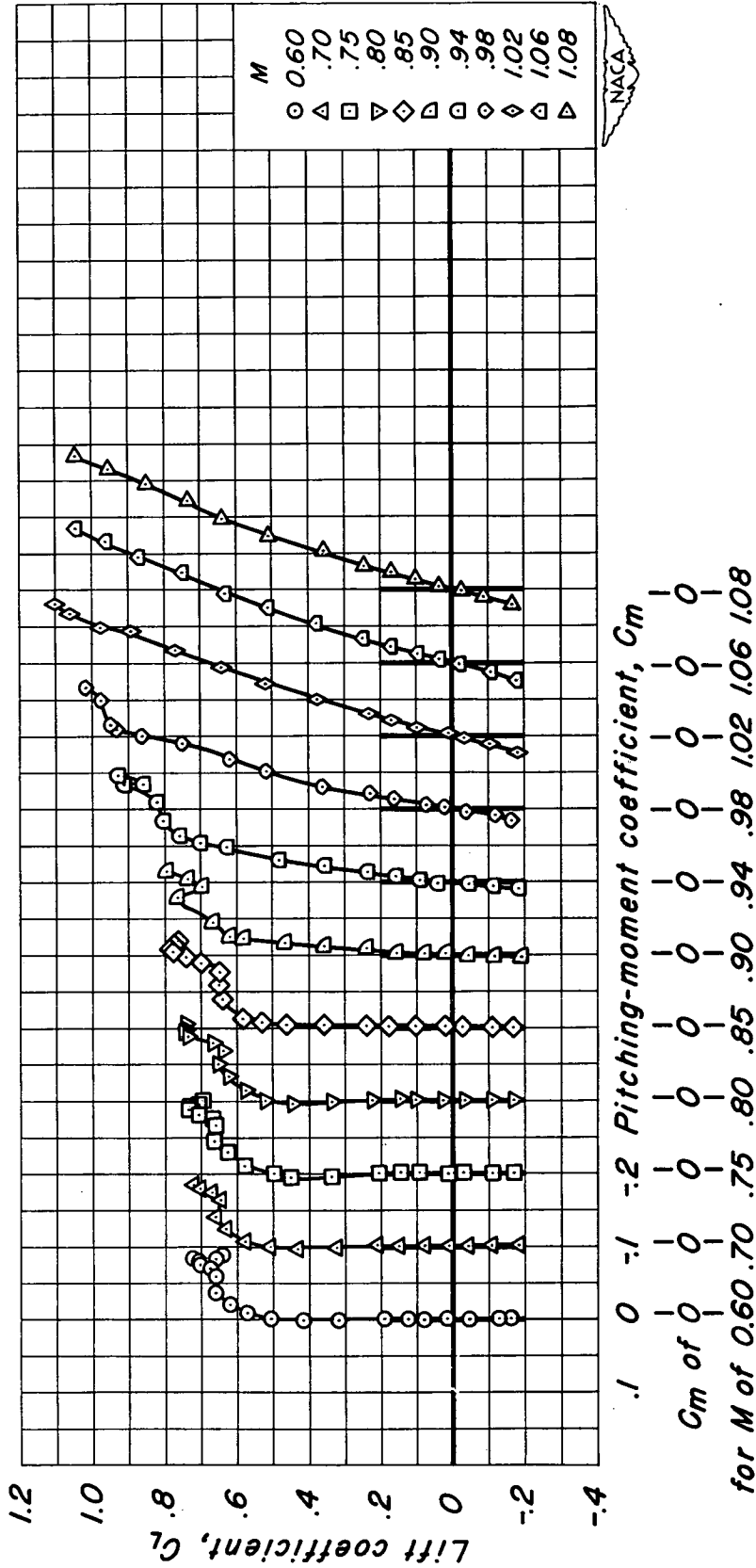
(a) t/c = 0.08 ; \lambda = 0
