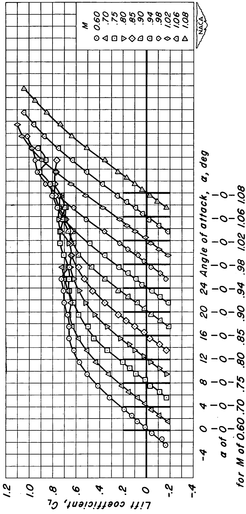
(a) t/c = 0.08 ; \lambda = 0
