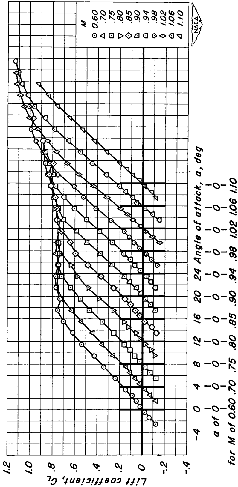
(f) t/c = 0.06 ; \lambda = 0.72
