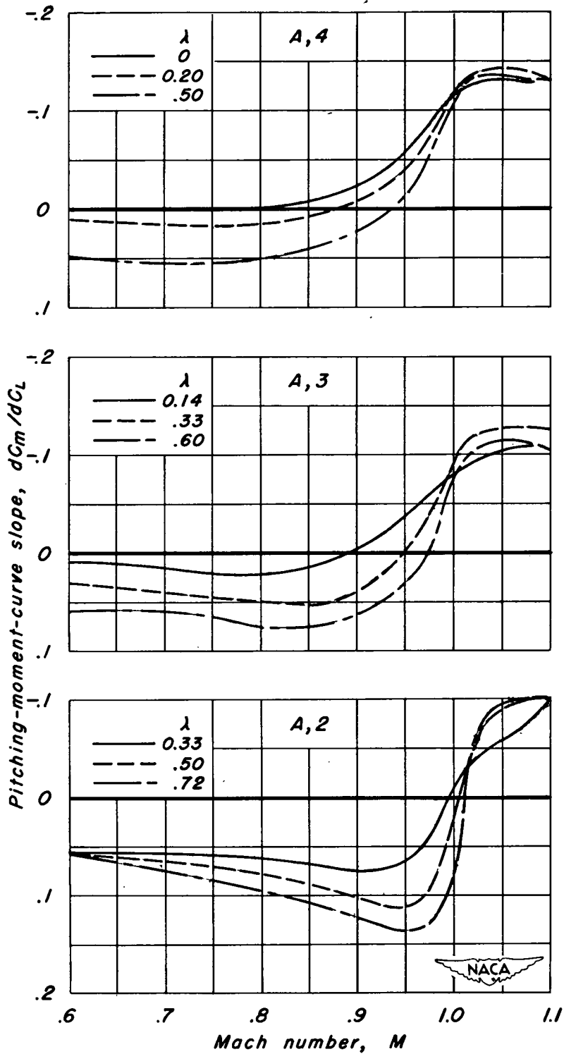
(a) NACA 63A008 sections.
