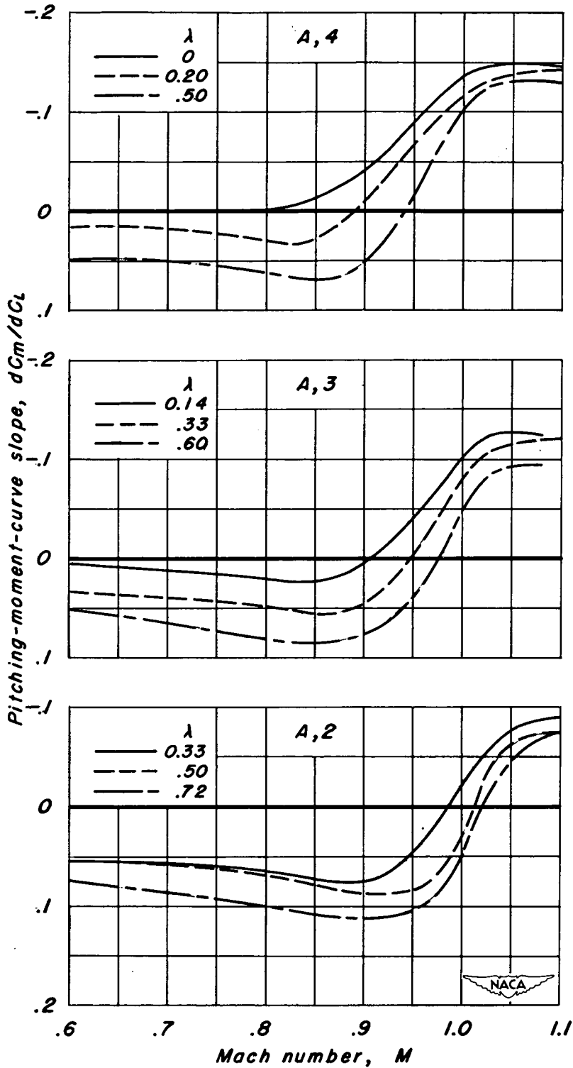
(b) NACA 63A006 sections.
