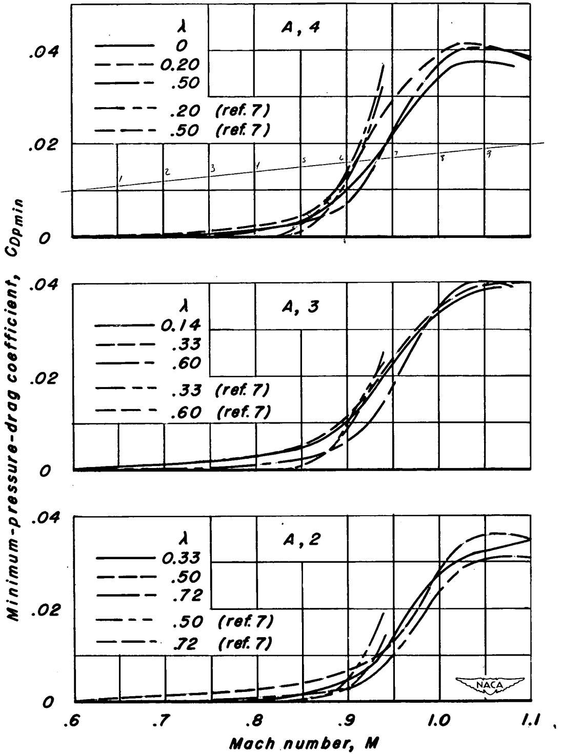
(a) NACA 63A008 sections.
