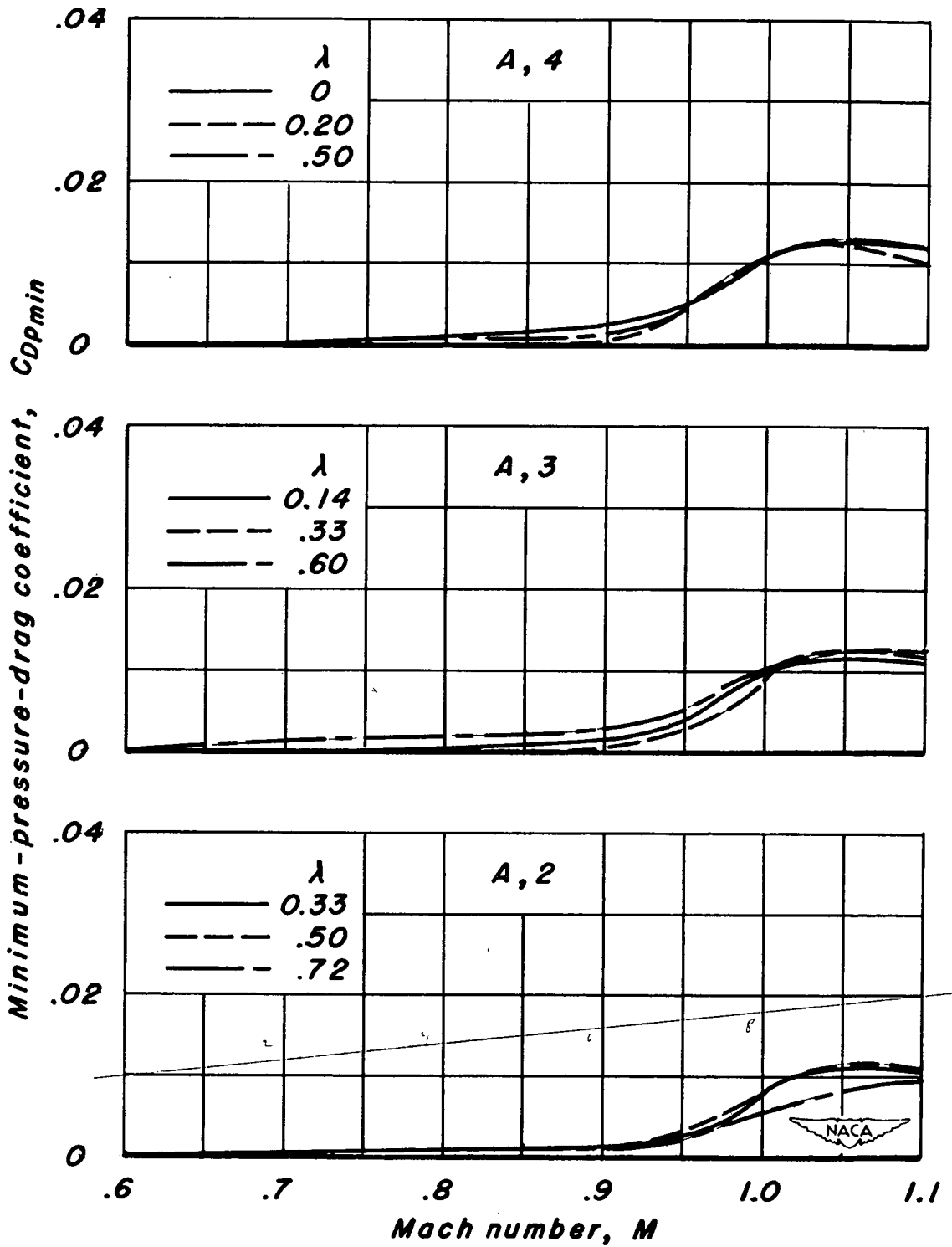
(c) NACA 63A004 sections.
