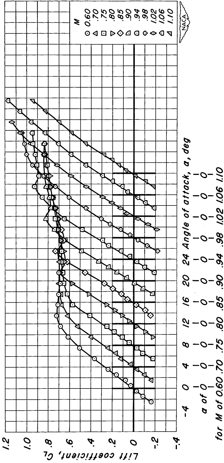
(f) t/c = 0.06 ; \lambda = 0.5
