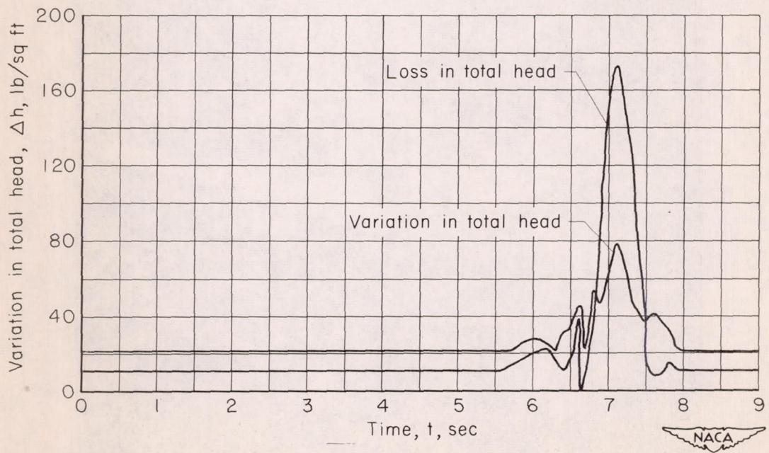
Figure 5.- Time history of normal acceleration and total head at tail during pitch-up; M = 0.92 .
