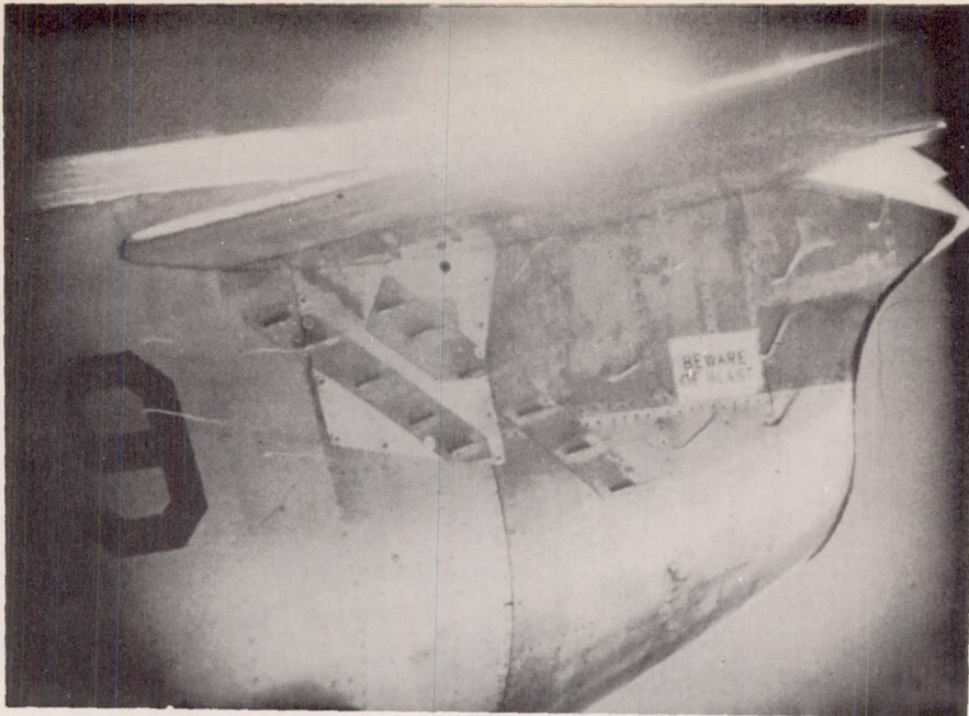
(a) High-tail configuration; M = 0.905 , 1 g flight.
