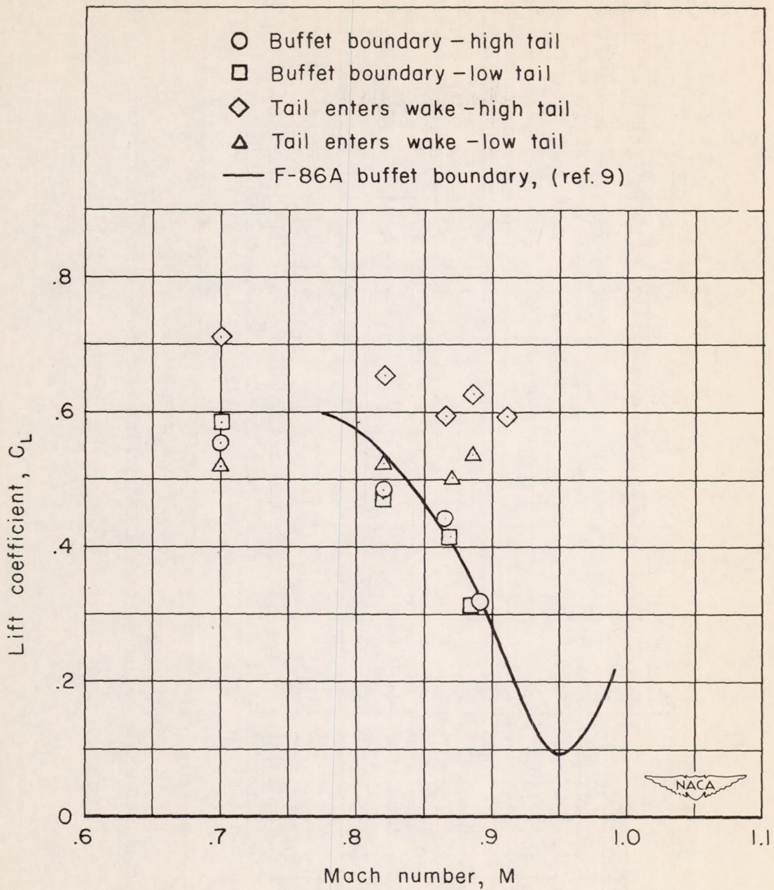
Figure 4.- Buffet boundary of test airplane.
