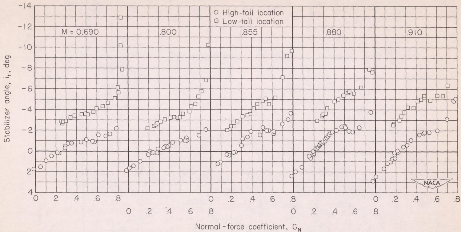
Figure 3.- Stabilizer angle required to balance airplane for both high- and low-tail installations.
