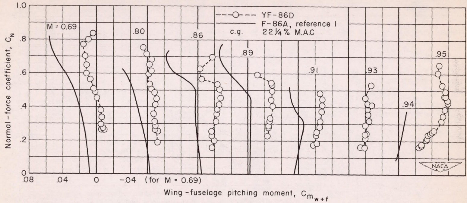
Figure 7.- Wing-fuselage pitching moments.
