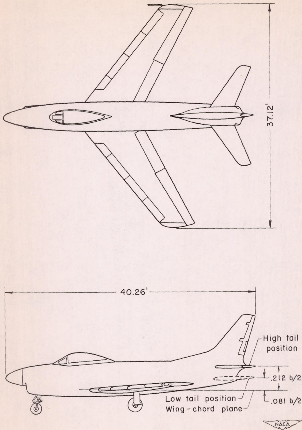
(a) Two-view drawing.
