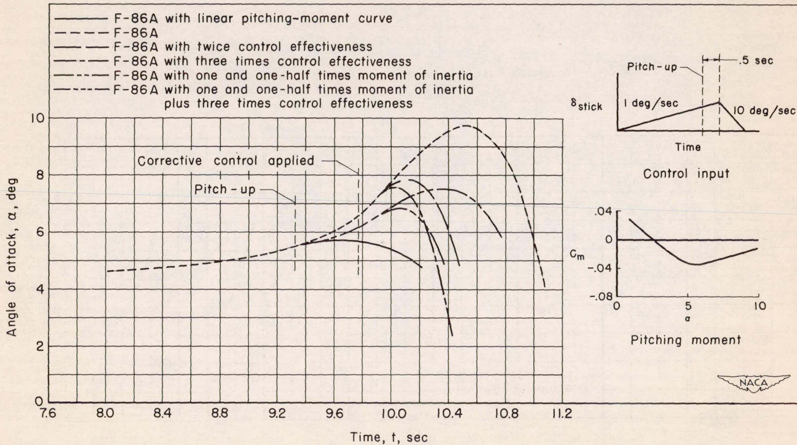
Figure 8.- Calculated time histories of the pitch-up.
