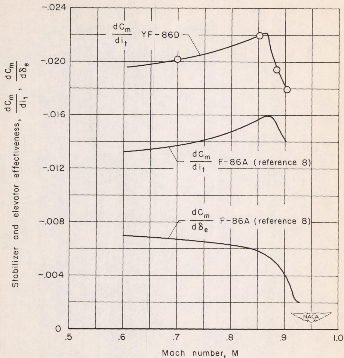
Figure 2.- Stabilizer and elevator effectiveness.
