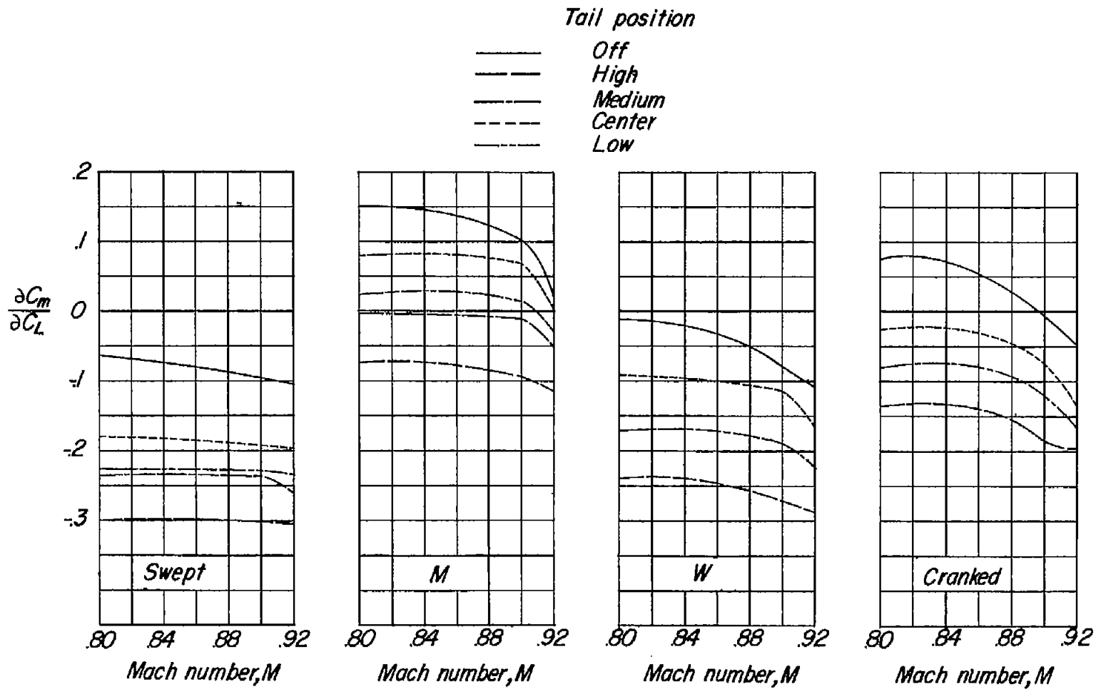
Figure 11.- Variation of \frac{\partial C_m}{\partial C_L} with Mach number for the composite-wing model with various horizontal-tail locations. C_L = 0 .
