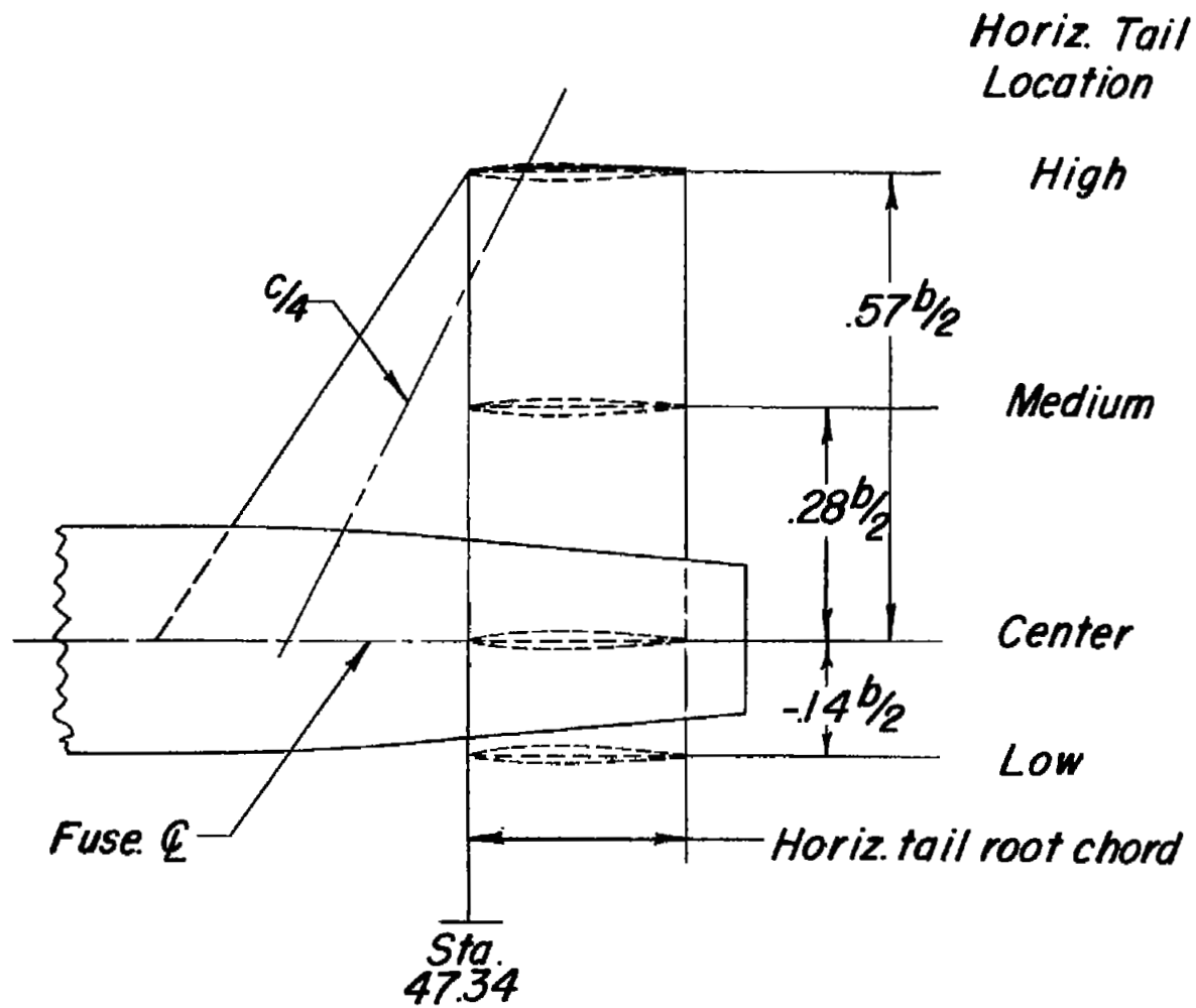
(c) Horizontal-tail locations.
