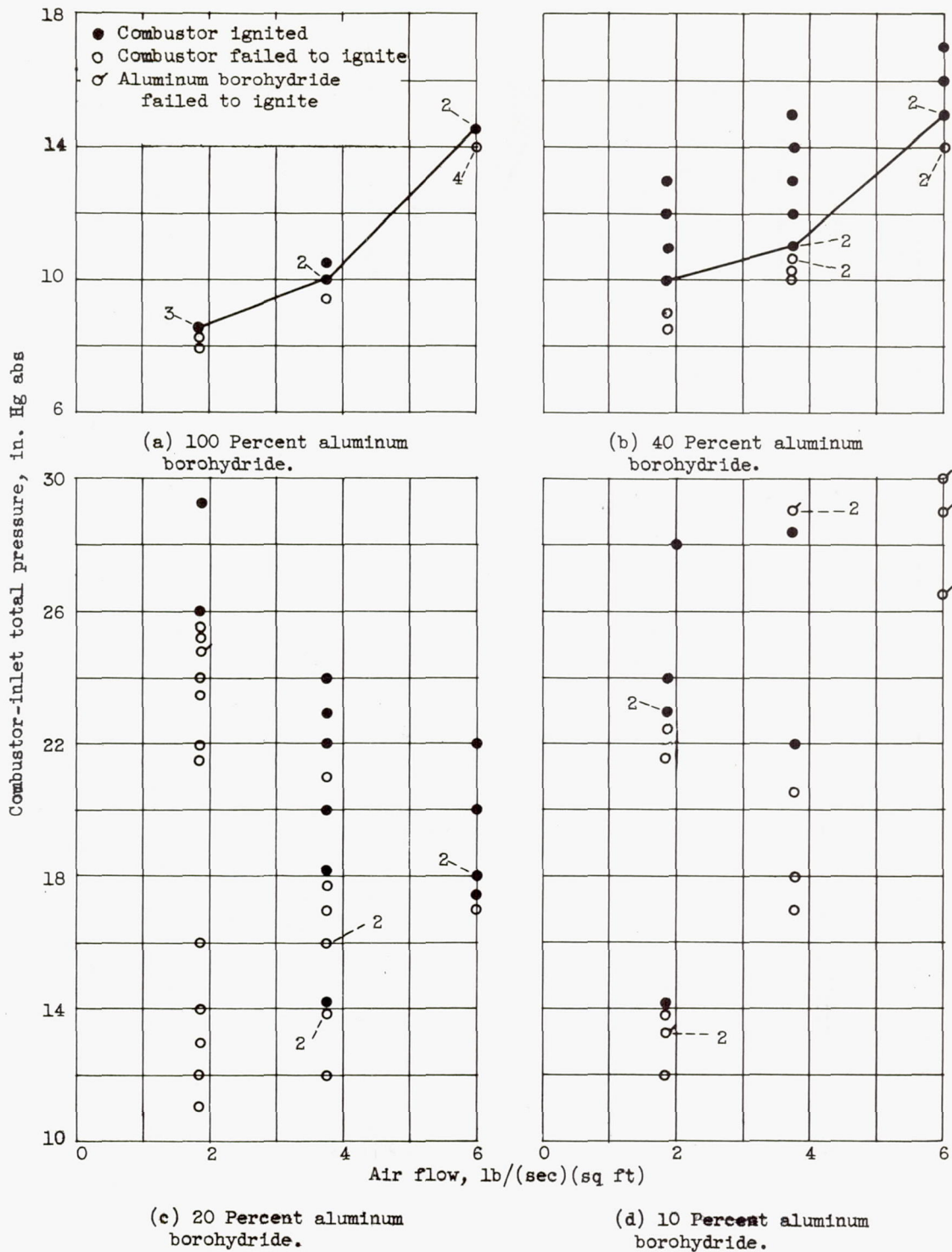
Figure 3. - Combustor ignition limits for various concentrations of aluminum borohydride. Diluent, JP-4 fuel; combustor-inlet air and fuel temperatures, 10° F.
