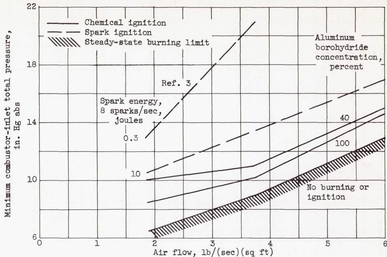
Figure 4. - Comparison of combustor burning limits with combustor ignition limits obtained with two concentrations of aluminum borohydride and with electric sparks as ignition sources. Diluent, JP-4 fuel; combustor-inlet air and fuel temperatures, 10^{\circ} F; capillary tube diameter, 0.025 inch.
