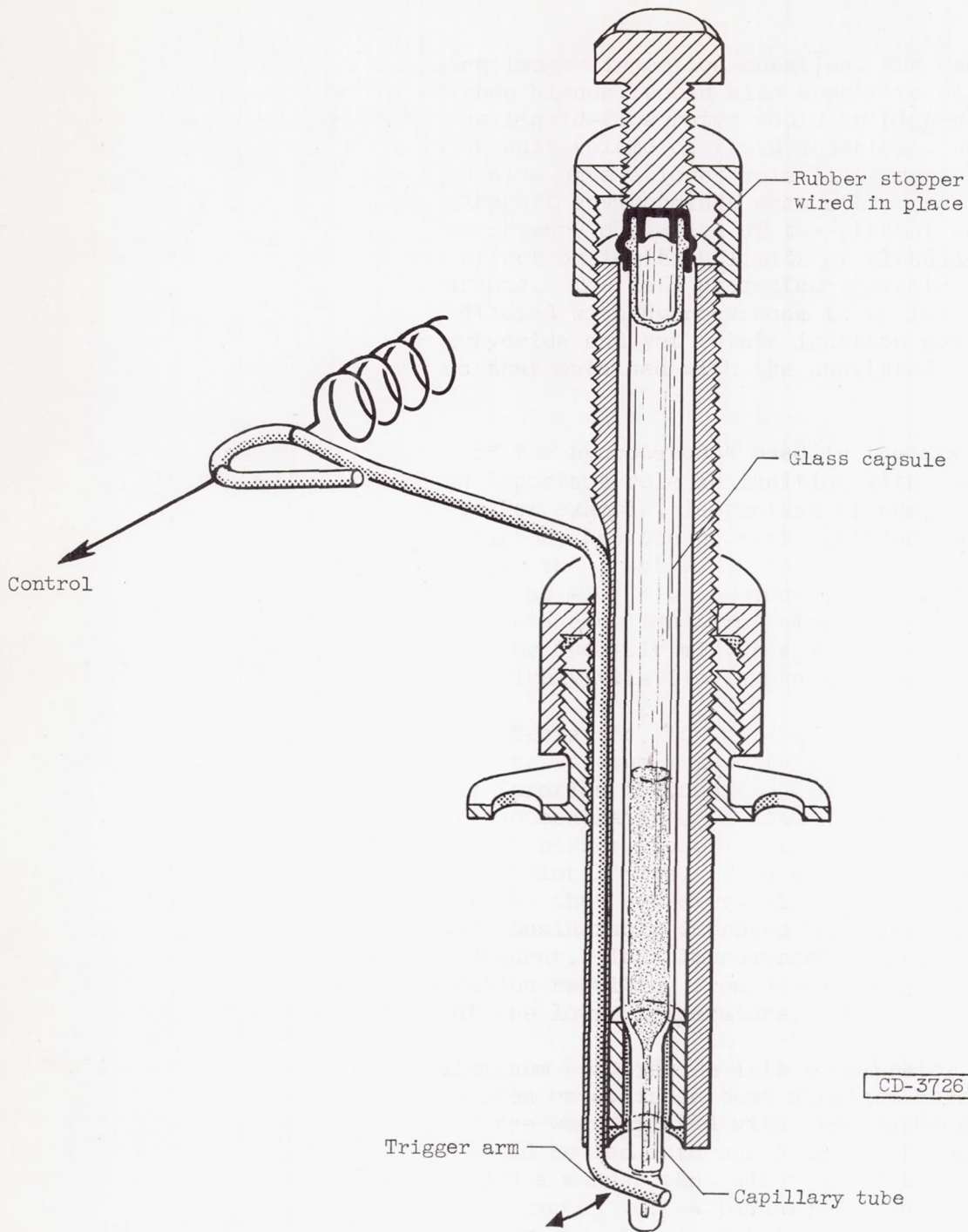
Figure 2. - Diagrammatic sketch of injector using pressurized glass capsules with capillary tube for single charges of chemical igniter.
