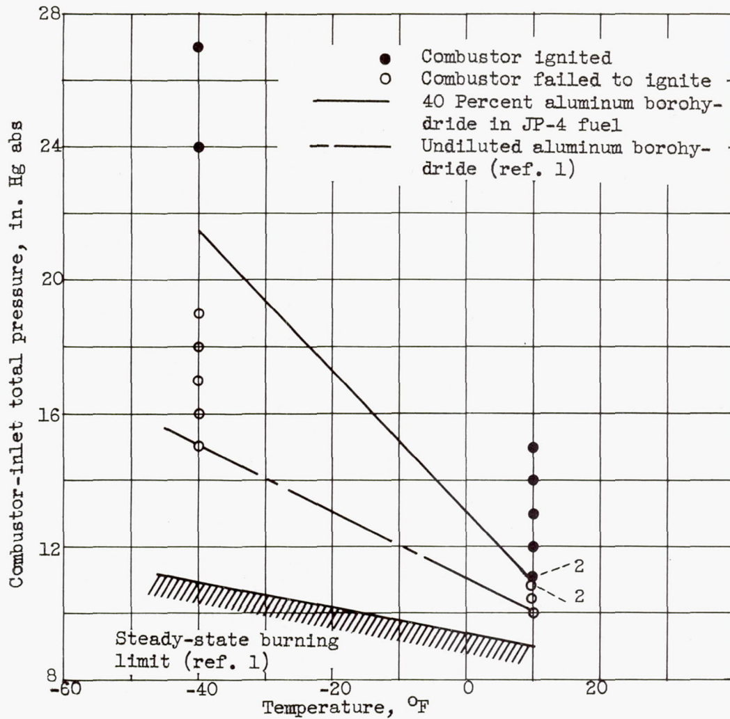
Figure 5. - Effect of inlet-air and -fuel temperatures on combustor ignition and burning limits. Aluminum borohydride concentration, 40 percent; air flow, 3.75 pounds per second per square foot; capillary tube diameter, 0.025 inch.
