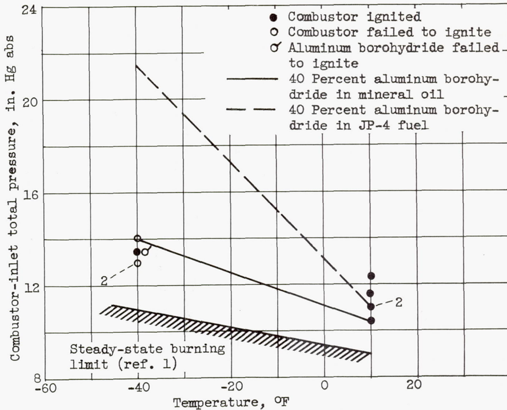
Figure 7. - Effect of diluent and inlet-air temperature on combustor ignition limits. Aluminum borohydride concentration, 40 percent; diluents, JP-4 fuel and mineral oil; air flow, 3.75 pounds per second per square foot; capillary tube diameter, 0.025 inch.
