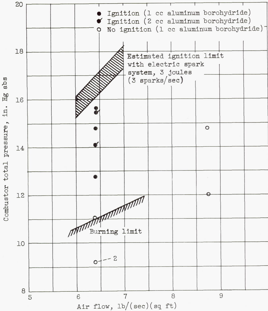
Figure 9. - Ignition data obtained in 48-inch ram-jet engine with aluminum borohydride as ignition source. Inlet-air temperature, 525° F (approx); fuel, JP-5.
