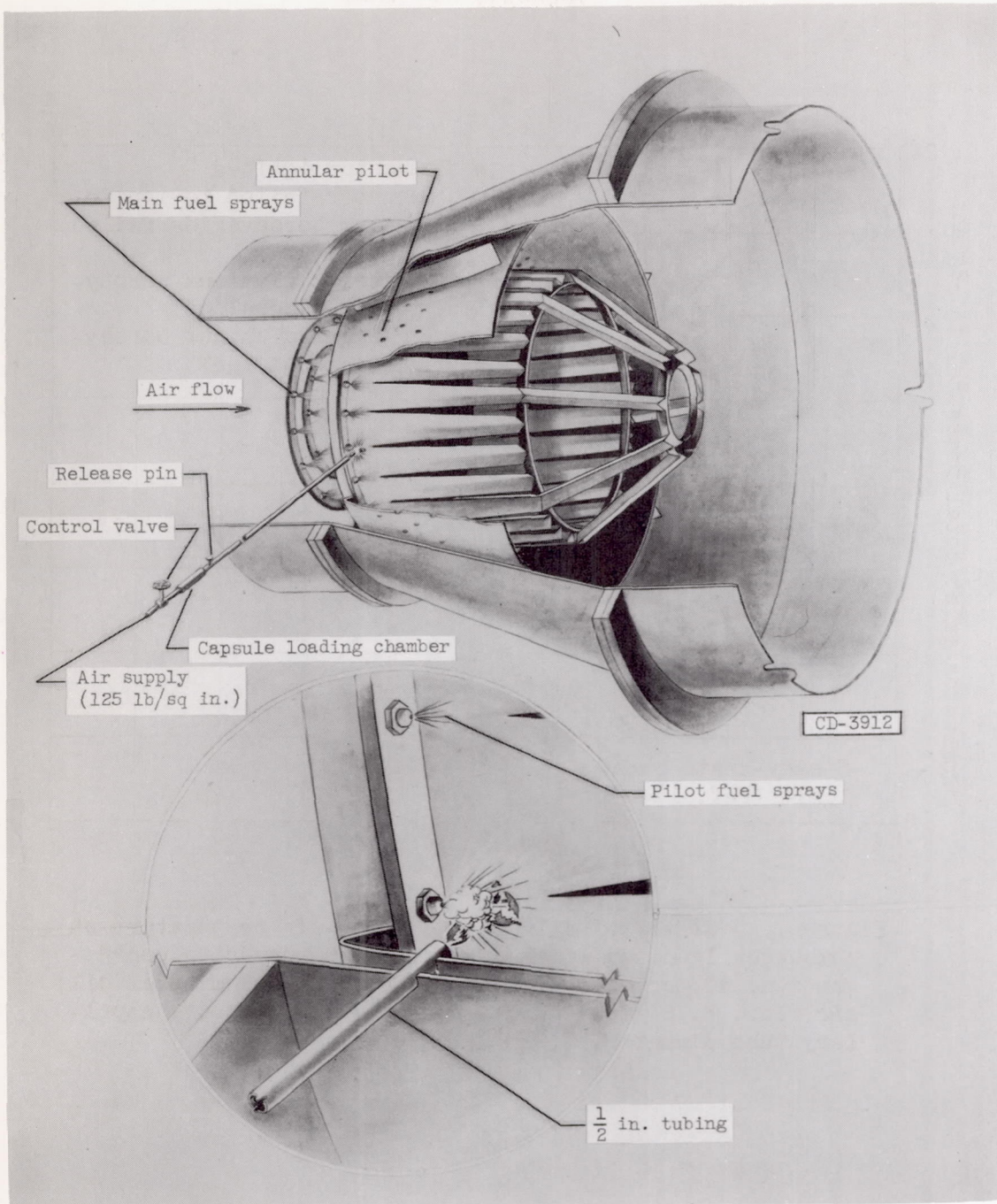
Figure 8. - Aluminum borohydride injection system for ignition in 48-inch ram-jet engine.
