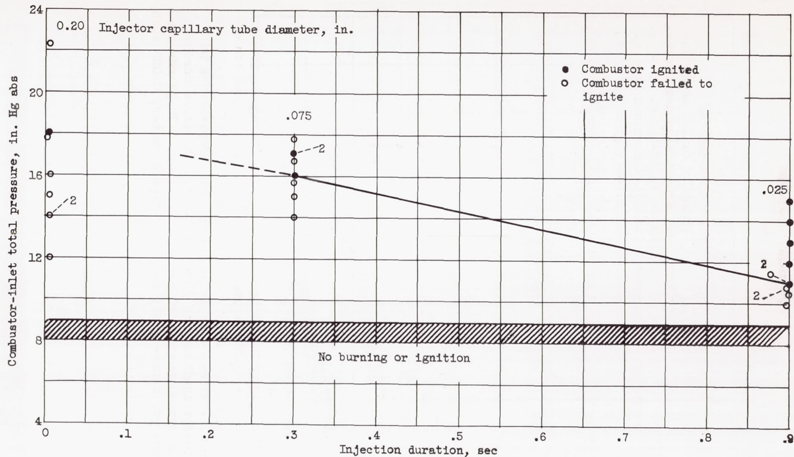
Figure 6. - Effect of injection duration on combustor ignition limits. Aluminum borohydride concentration, 40 percent; diluent, JP-4 fuel; inlet-air and -fuel temperatures, 10° F; air flow, 3.75 pounds per second per square foot; capillary length, 0.75 inch.
