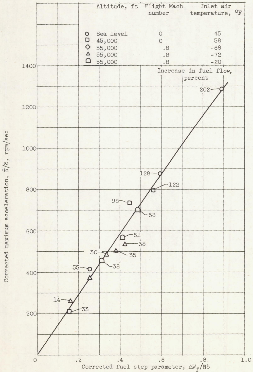
Figure 13. - Variation of acceleration with fuel step parameter for a range of fuel step sizes up to surge fuel flow. Inlet guide vanes, open.
