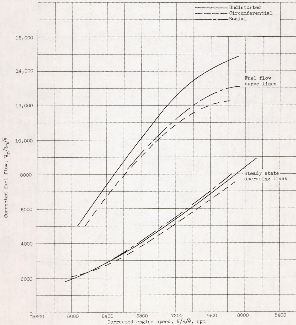
Figure 16. - Effect of inlet distortion on steady state and surge fuel flow lines. Inlet guide vanes, open. Altitude, 35,000 ft; flight Mach number 0.8.
