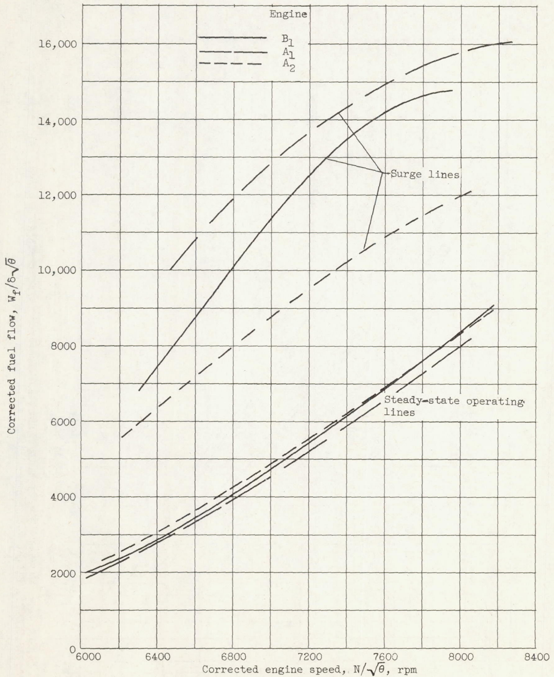
Figure 9. - Variation of surge and steady-state fuel flow, with corrected engine speed for three production engines. Altitude, 35,000 ft; flight Mach number, 0.8. Inlet guide vanes, open.
