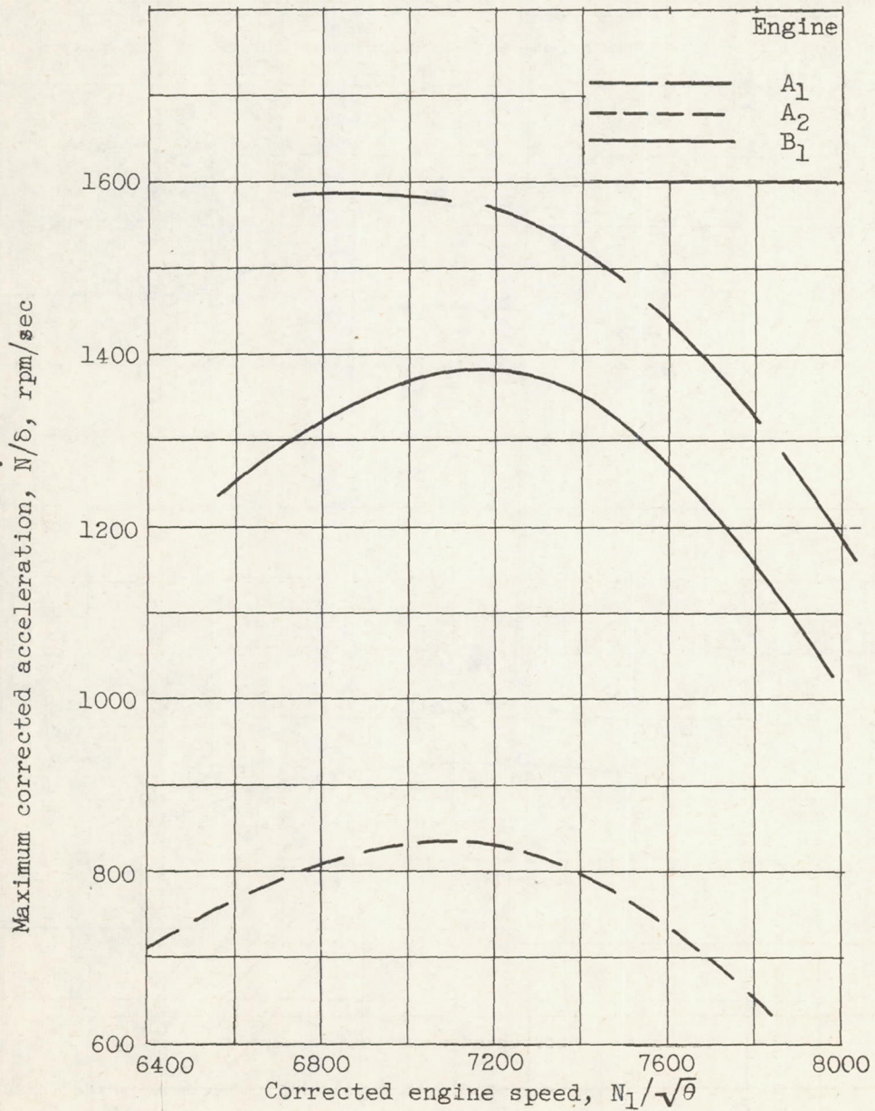
Figure 7. - Maximum acceleration obtained with three turbojet engines. Inlet guide vanes open. Altitude, 35,000 ft; flight Mach number, 0.8.
