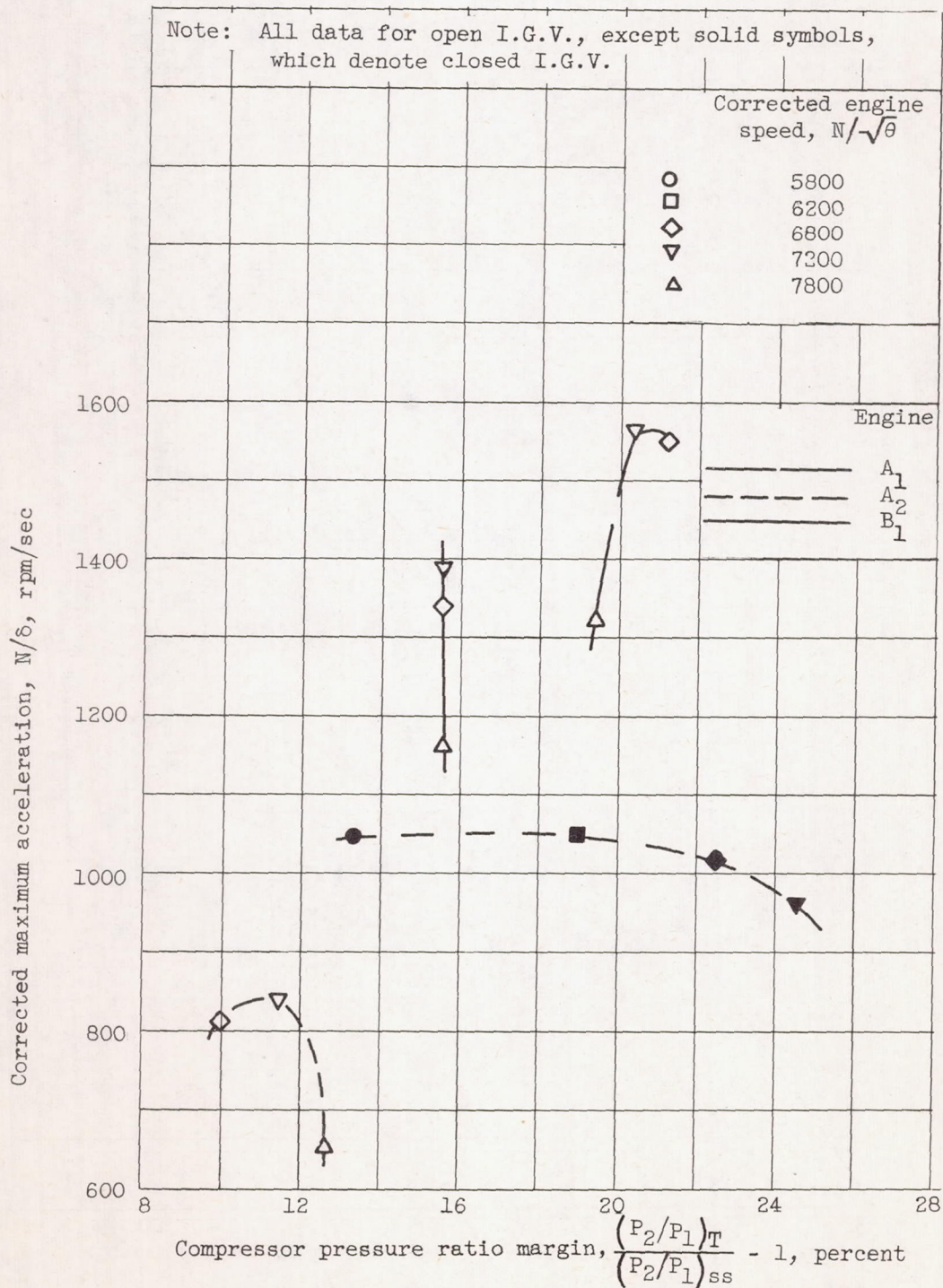
Figure 10. - Variation of maximum acceleration with pressure ratio margin for three turbojet engines. (Surge-limited fuel steps.) Altitude, 35,000 ft; flight Mach number, 0.8.
