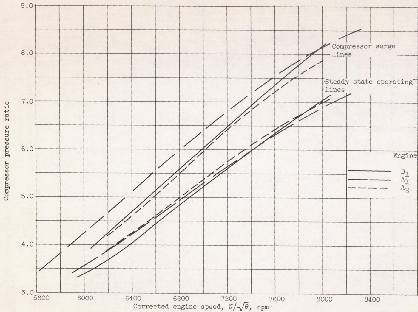
Figure 8. - Surge and steady-state operating lines for three turbojet engines. Altitude, 35,000 ft; flight Mach number, 0.8. Inlet guide vanes, open.
