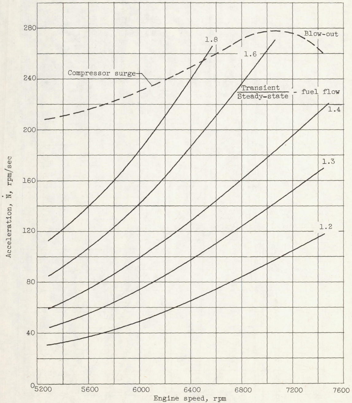
(a) Inlet guide vanes open.
