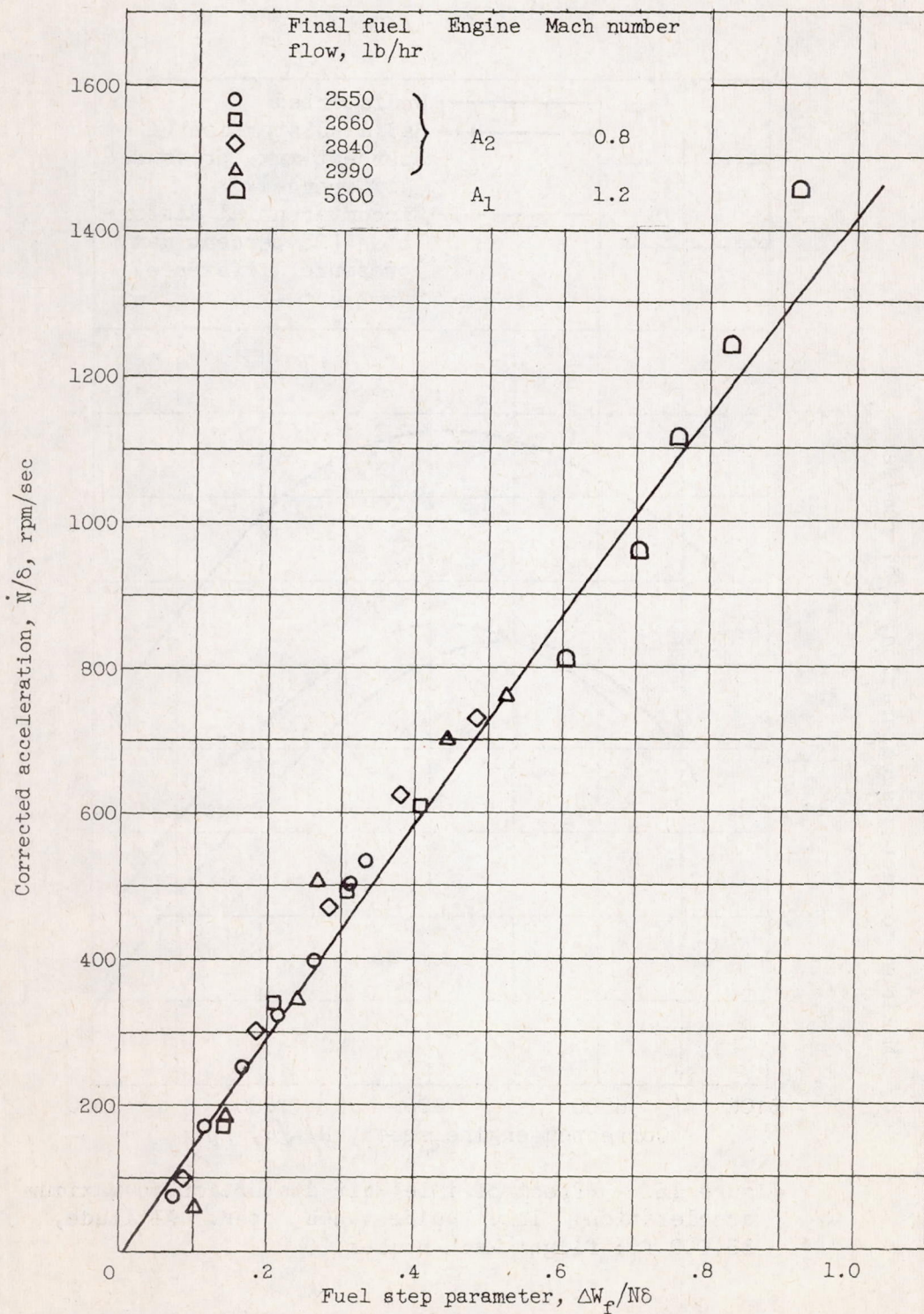
Figure 14. - Acceleration values from time history of step change in engine fuel flow. Inlet guide vanes, open. Altitude, 35,000 feet.
