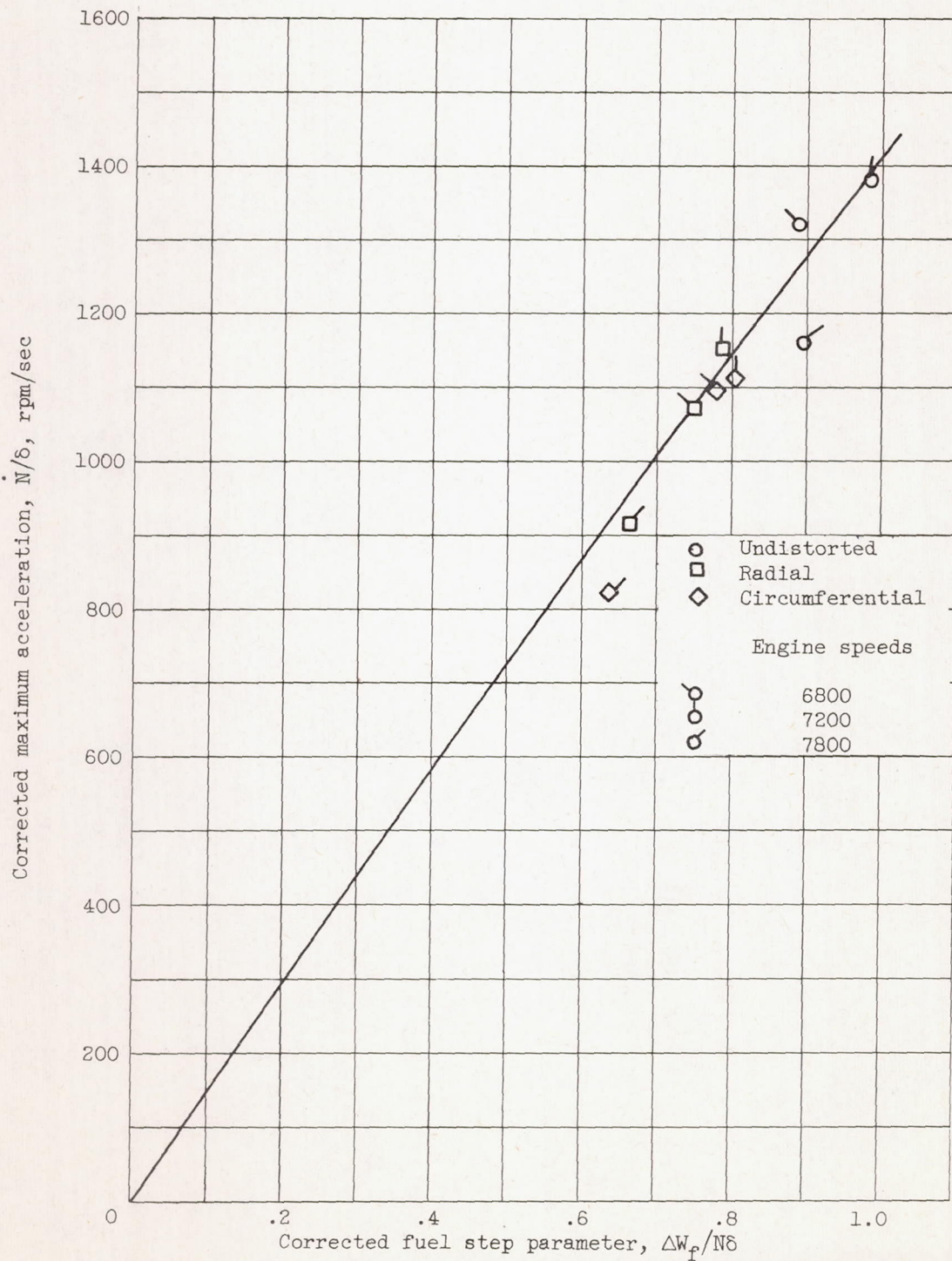
Figure 18. - Variation of maximum acceleration with fuel step parameter for inlet air distortion. Altitude, 35,000 ft; flight Mach number, 0.8. Inlet guide vanes, open.
