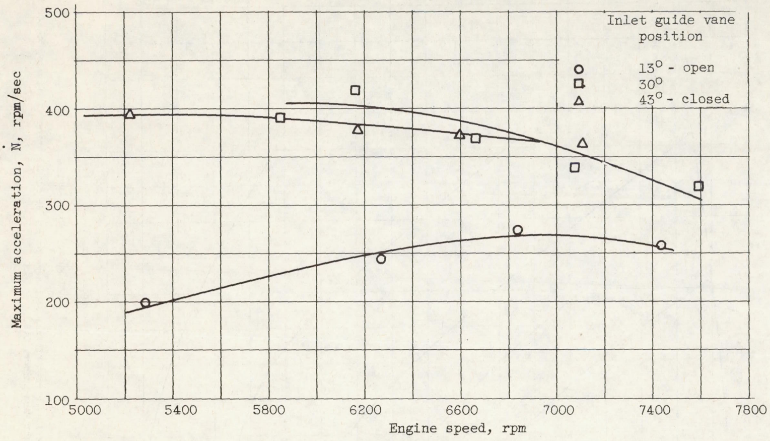
Figure 5. - Effect of inlet guide vane position on maximum acceleration. (Surge limited fuel steps.) Altitude, 35,000 ft; flight Mach number, 0.8.
