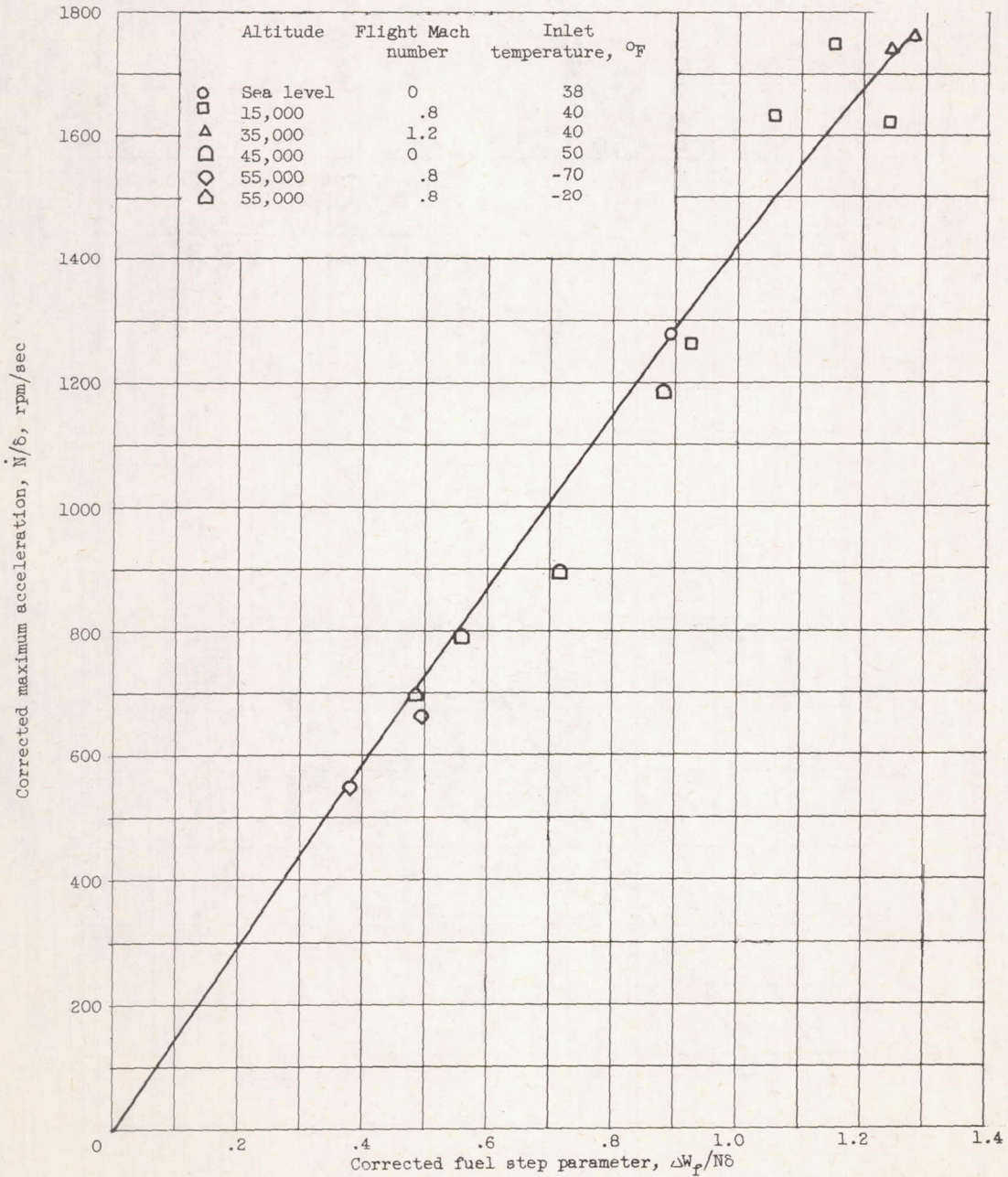
Figure 12. - Variation of maximum acceleration with fuel step parameter for range of inlet conditions. Inlet guide vanes, open. (Surge limited fuel steps.)
