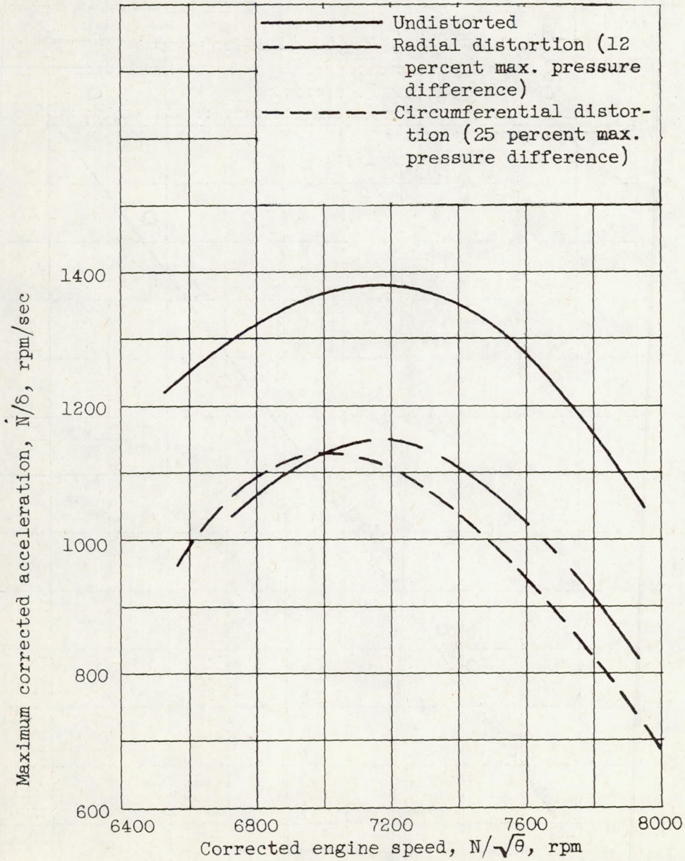
Figure 15. - Effect of inlet air distortion on maximum acceleration. Inlet guide vanes, open. Altitude, 35,000 ft; flight Mach number, 0.8.
