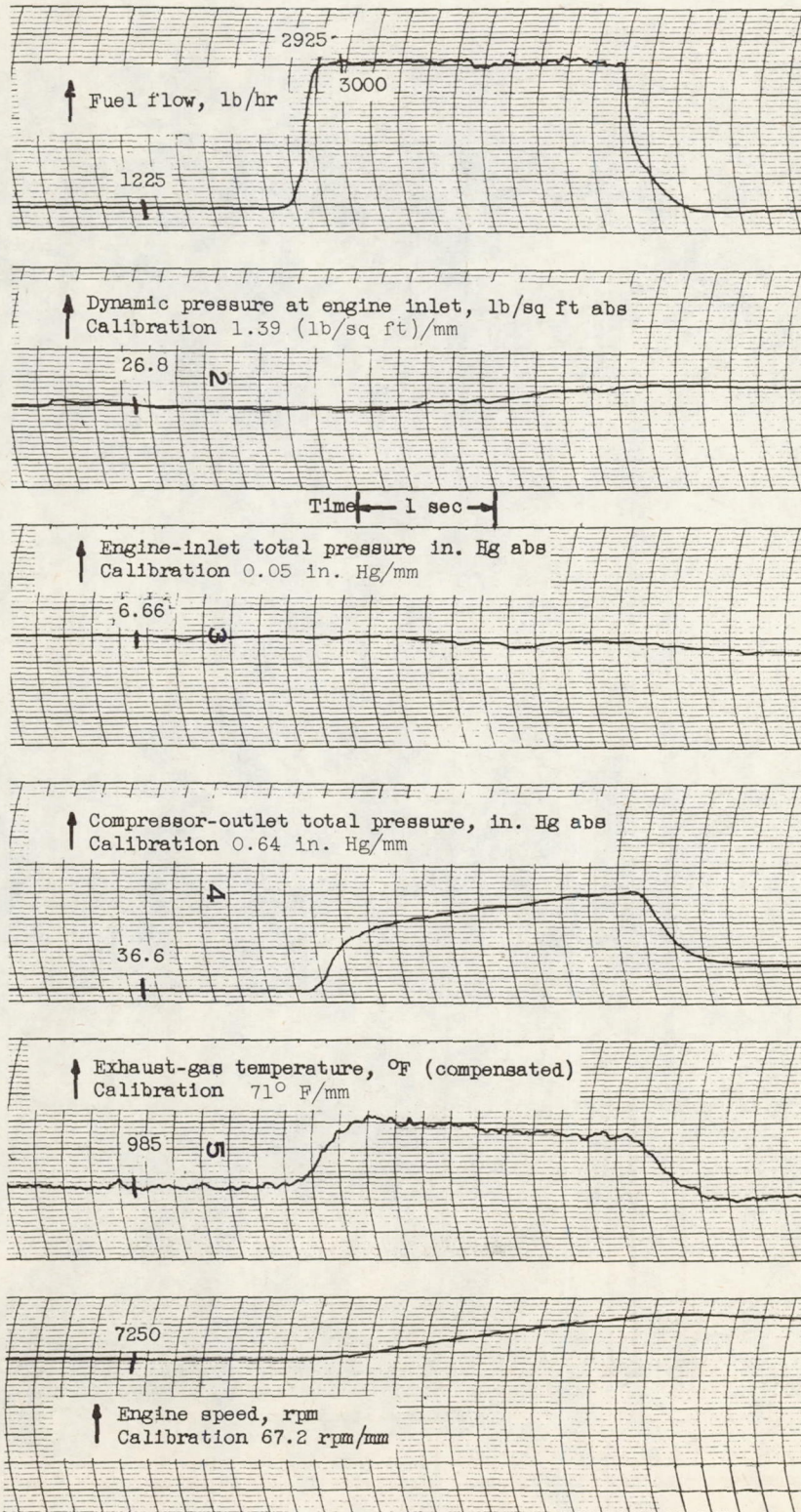
Figure 2. - Typical oscillograph trace showing measured parameters.
