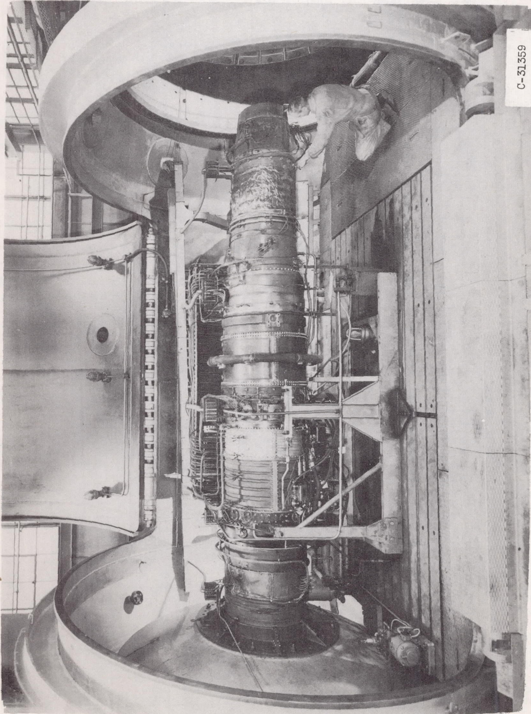
Figure 1. - Turbojet installation in altitude chamber.
