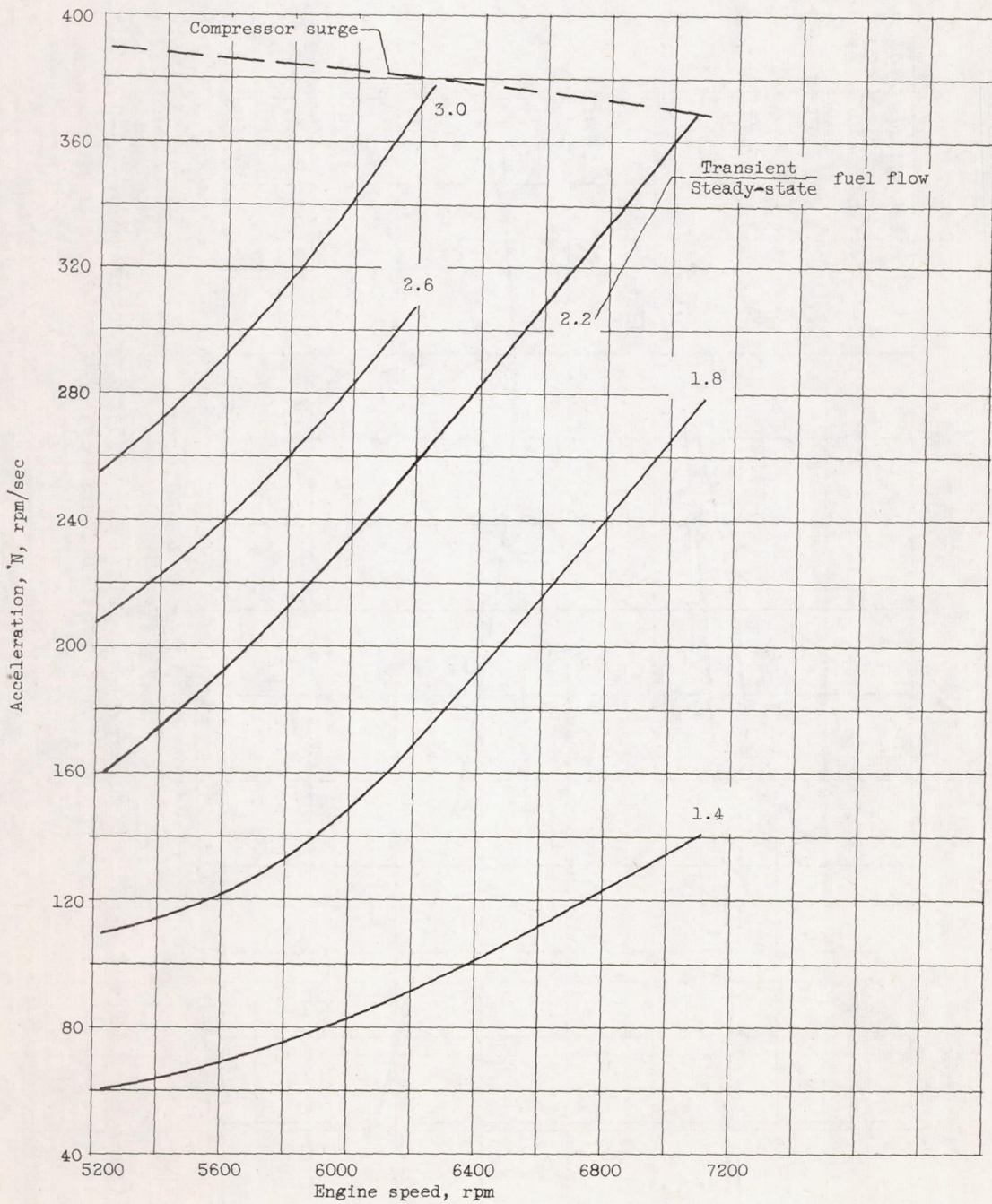
(b) Inlet guide vanes closed.
