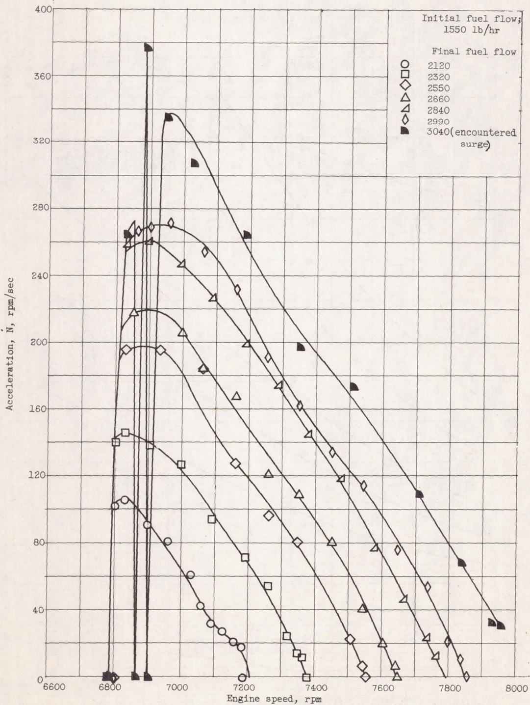
Figure 3. - Acceleration histories from same initial speed with increasing fuel steps to compressor surge. I.G.V. open. Altitude, 35,000 ft; Flight Mach number, 0.8.
