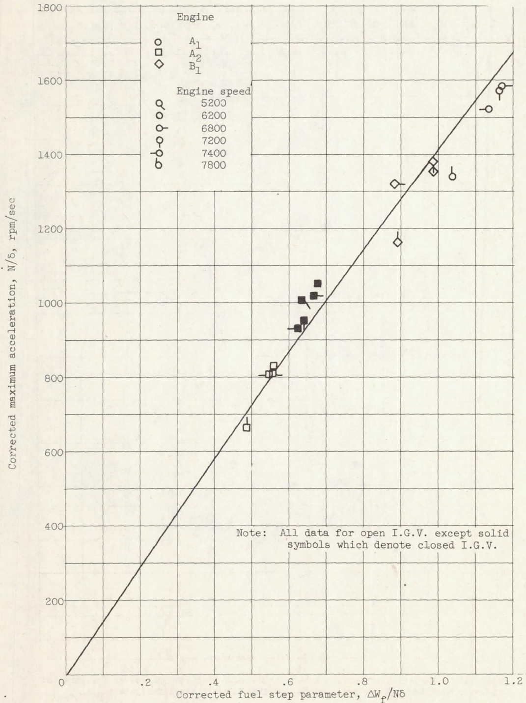
Figure 11. - Variation of maximum acceleration with fuel step parameter for three production engines at various speeds and inlet guide vane settings. Altitude, 35,000 ft; flight Mach number, 0.8. (Surge-limited fuel steps.)
