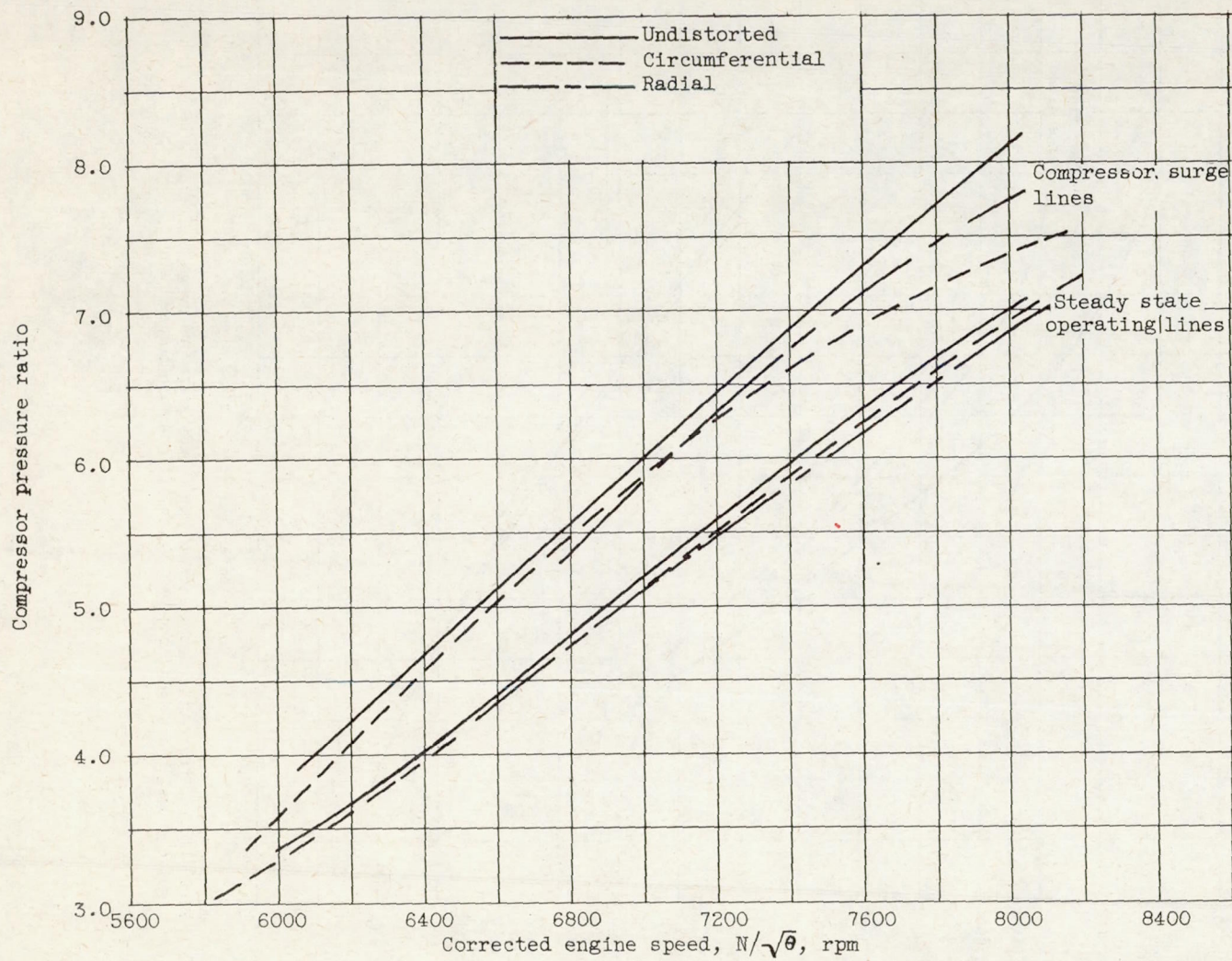
Figure 17. - Effect of inlet air distortion on compressor surge and steady state operating lines. Altitude, 35,000 ft; flight Mach number, 0.8. Inlet guide vanes, open.
