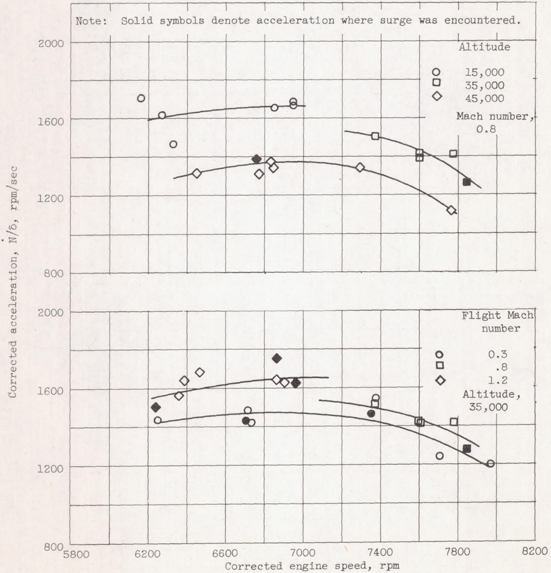
Figure 6. - Effect of changes in flight condition on maximum corrected acceleration. (Surge limited fuel steps.)
