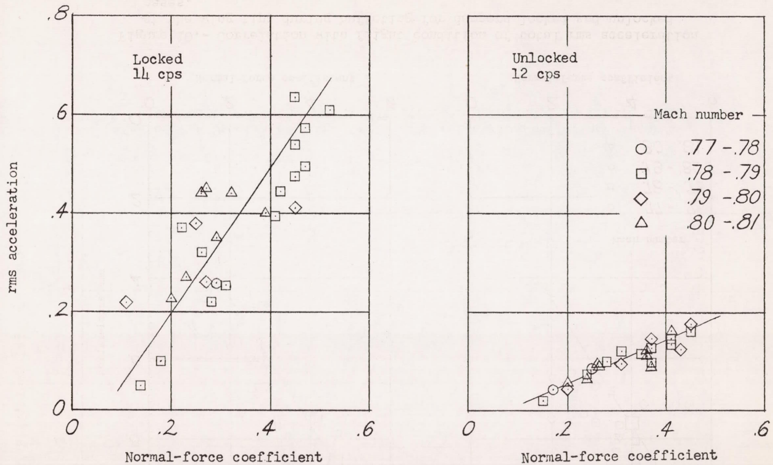
Figure 11.- Correlation with flight condition of rms acceleration passed by filter of 3 cps band width centered on frequency of second bending mode.
