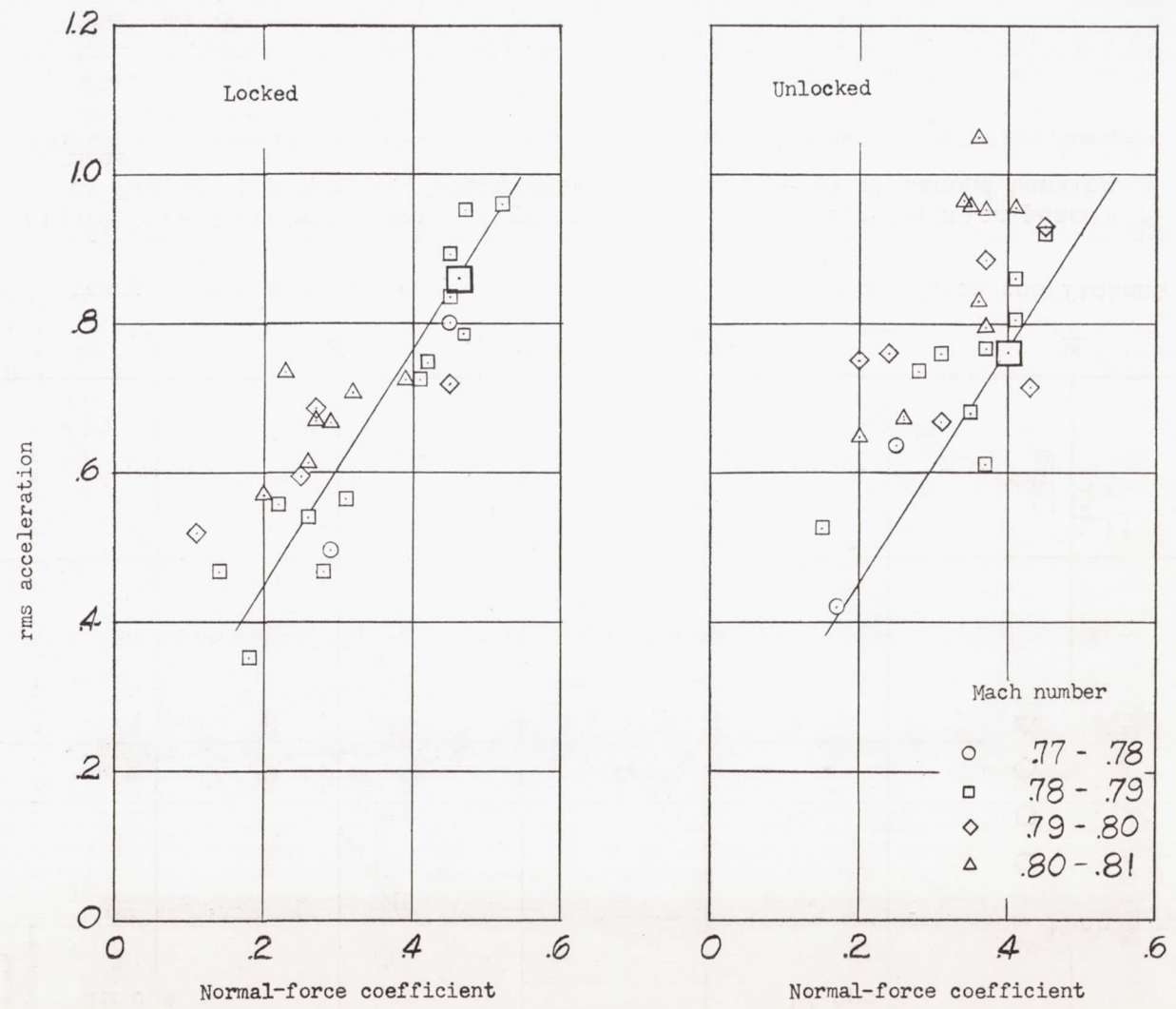
Figure 10.- Correlation with flight condition of total rms acceleration at the wing tips during buffeting for dampers locked and unlocked cases.
