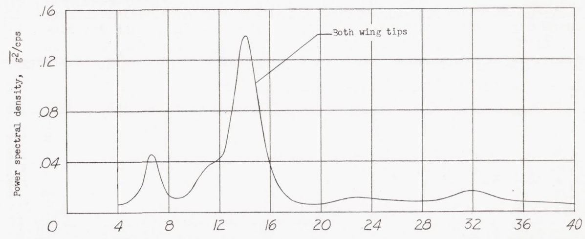
(a) Dampers locked. Average Mach number 0.79; average normal force coefficient 0.46.
