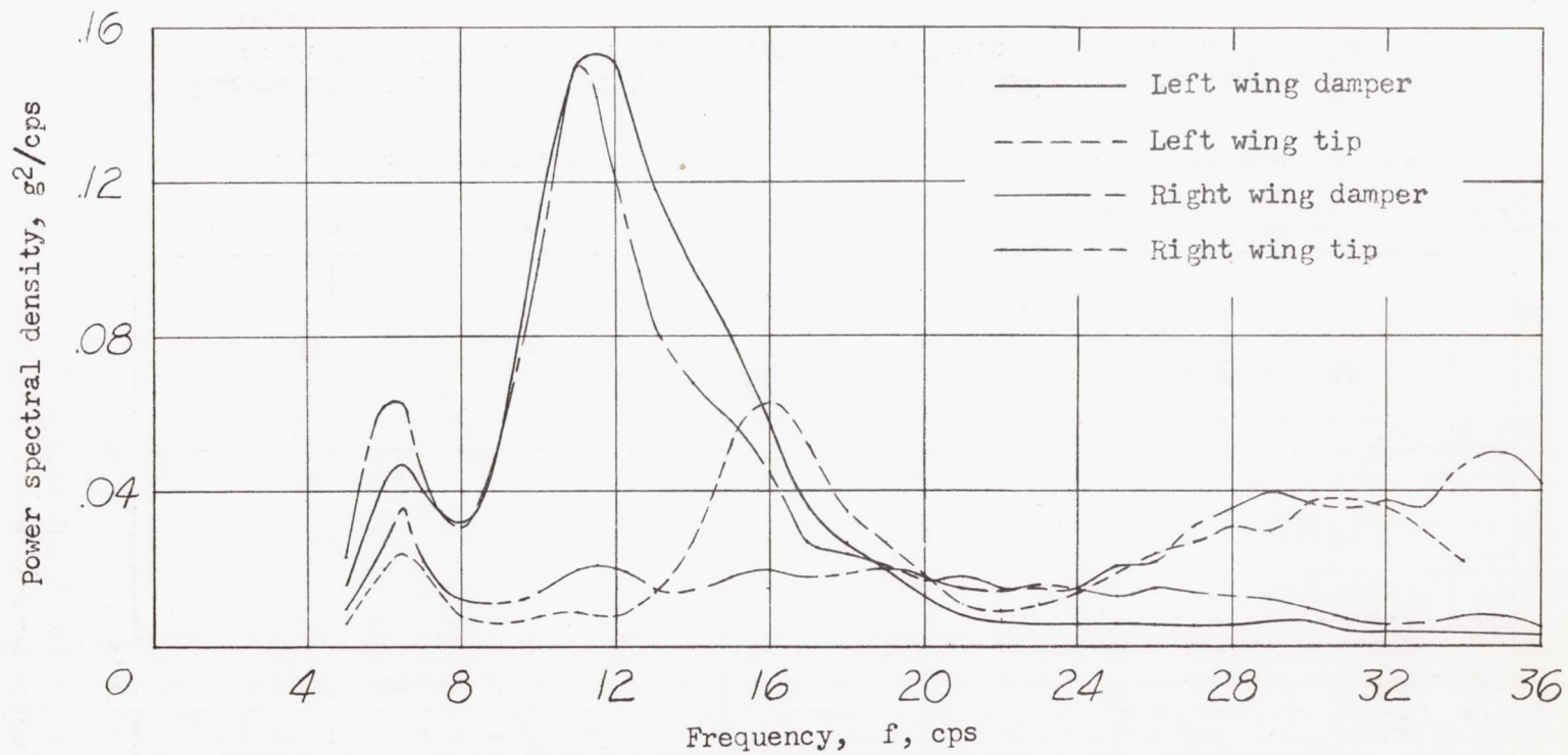
Figure 12.- Spectra of damper accelerations during buffeting compared with spectra of wing tip accelerations reproduced from figure 8(b).
