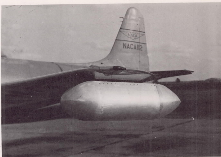
Figure 2.- Photograph of test airplane showing damper fairing mounted on the left wing tip. L-82814
