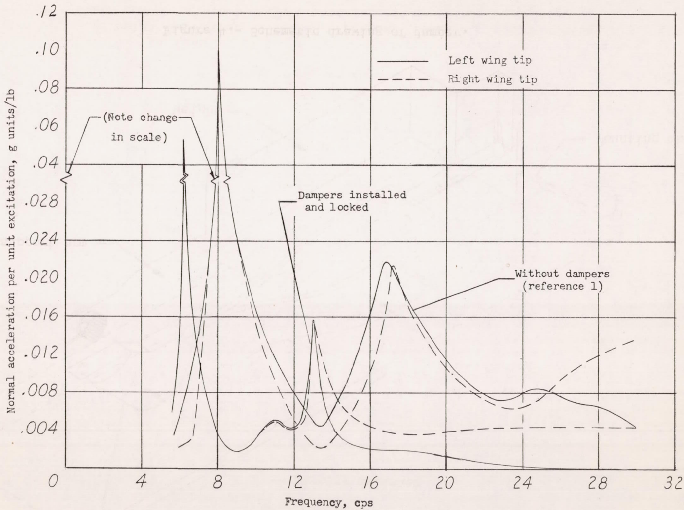
Figure 5.- Response of airplane structure to sinusoidal excitation applied at the right wing tip with and without dampers installed.
