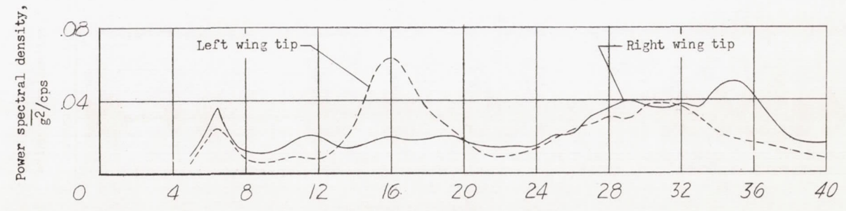
(b) Dampers unlocked. Average Mach number 0.79; average normal force coefficient 0.40.
