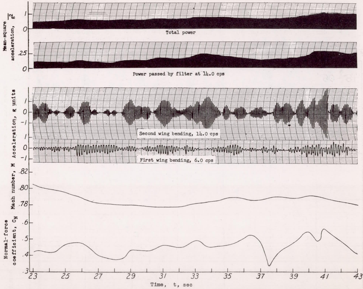
Figure 9.- Time histories of flight conditions, component accelerations, and total and component average square accelerations for the left wing tip during typical buffeting run with dampers locked. The power time histories have been shifted to account for the apparent lag of the thermocouple.
