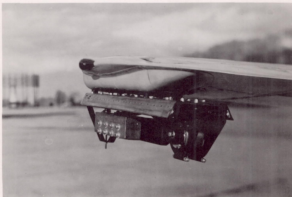
Figure 3.- Photograph showing damper mounted on left wing tip of test airplane with fairing removed. L-82812
