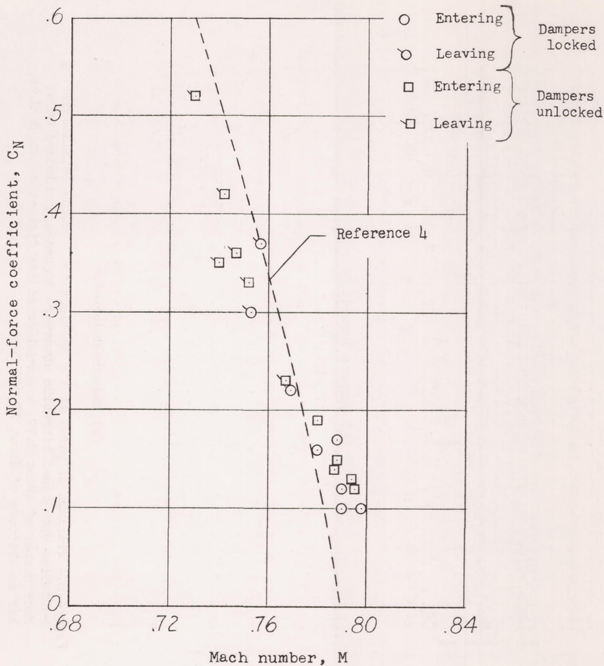
Figure 7.- Buffet boundary data for the test airplane with tuned vibration absorbers installed.
