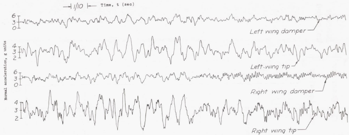
(a) Dampers locked.
