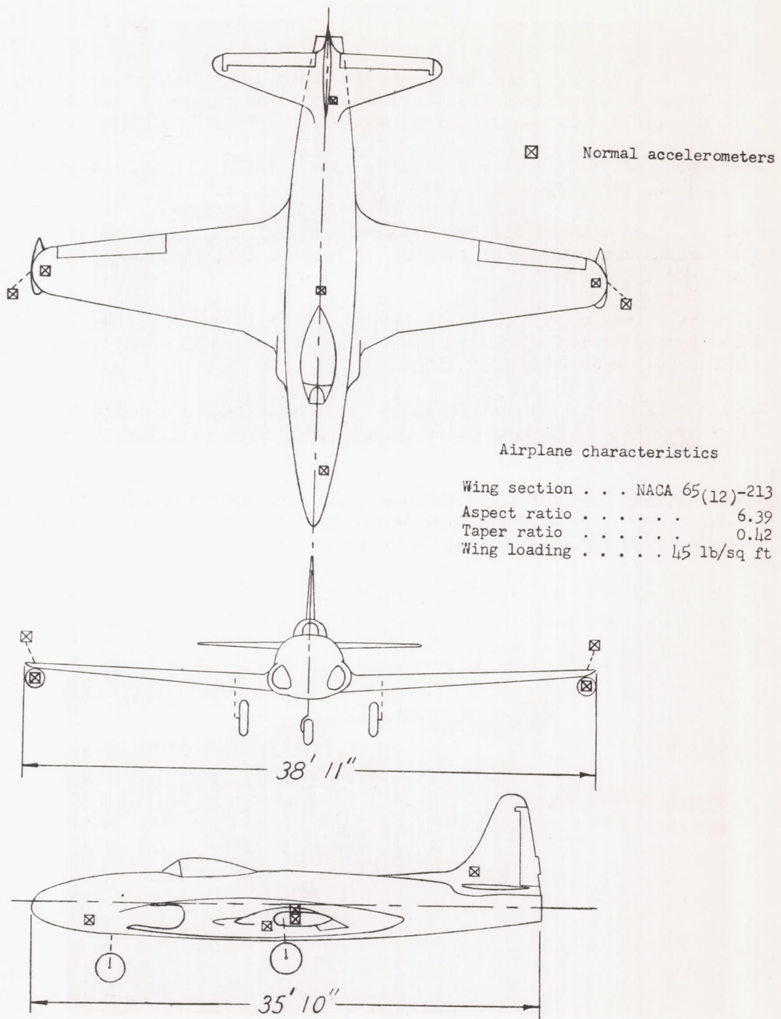
Figure 1.- Three-view drawing of test airplane (Lockheed F-80A) showing location of accelerometers and damper fairings.
