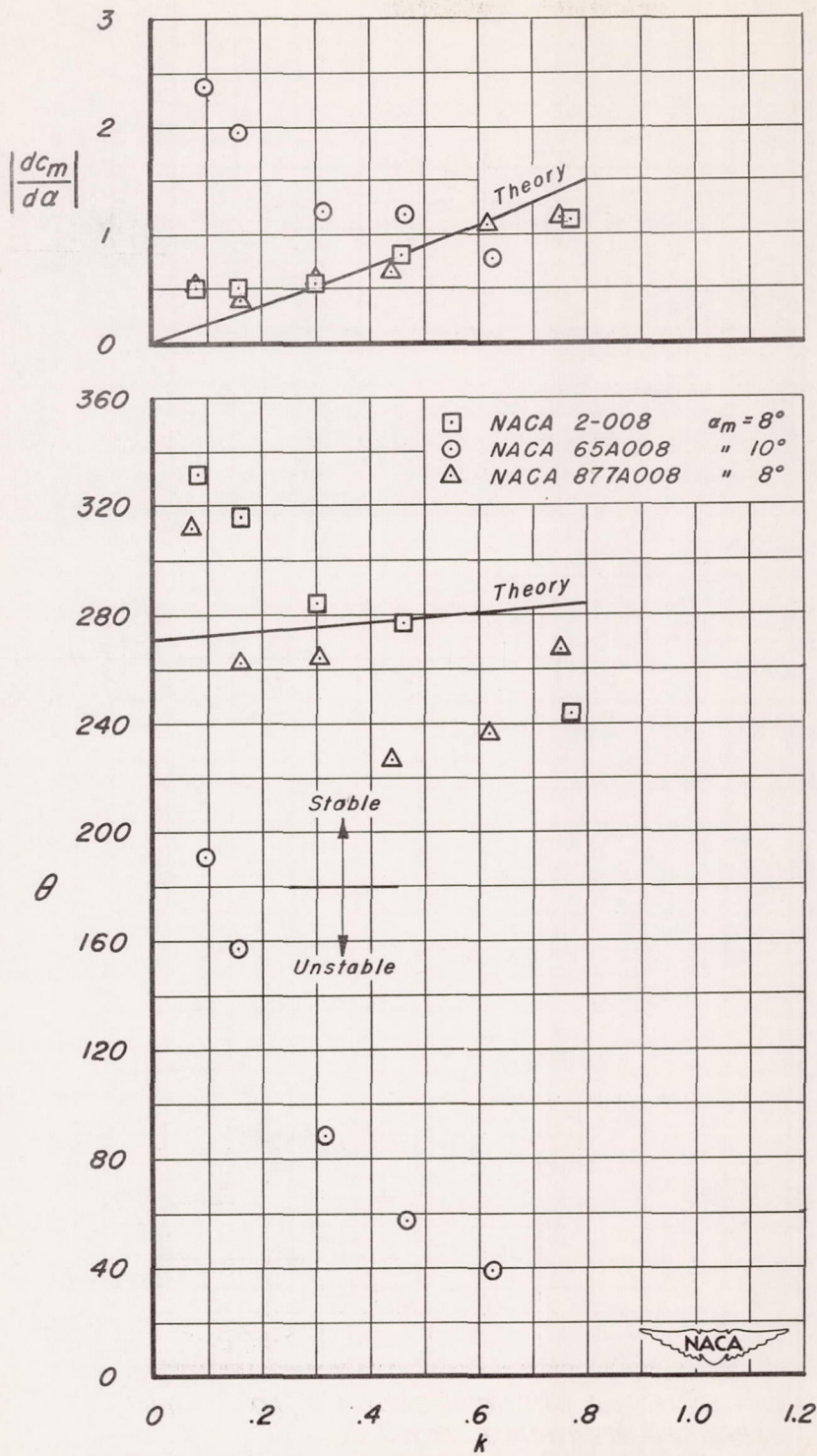
(b) Moment derivative and phase angle as a function of reduced frequency. M = 0.30 .
