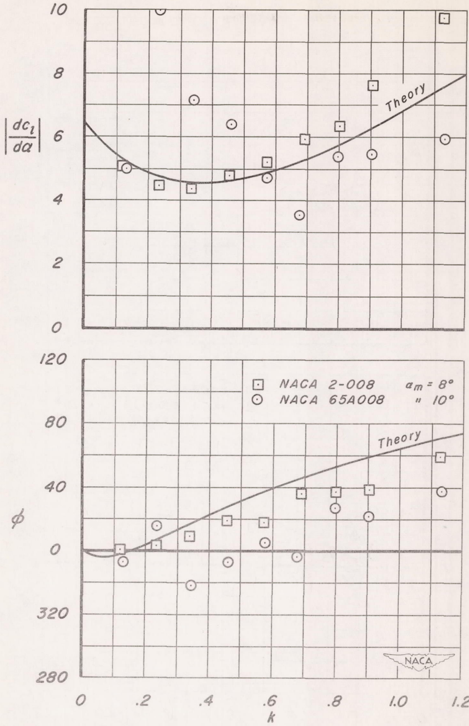
(a) Lift derivative and phase angle as a function of reduced frequency. M = 0.20 . Figure 8.- Effects of airfoil thickness distribution on lift flutter derivative and phase angle.
