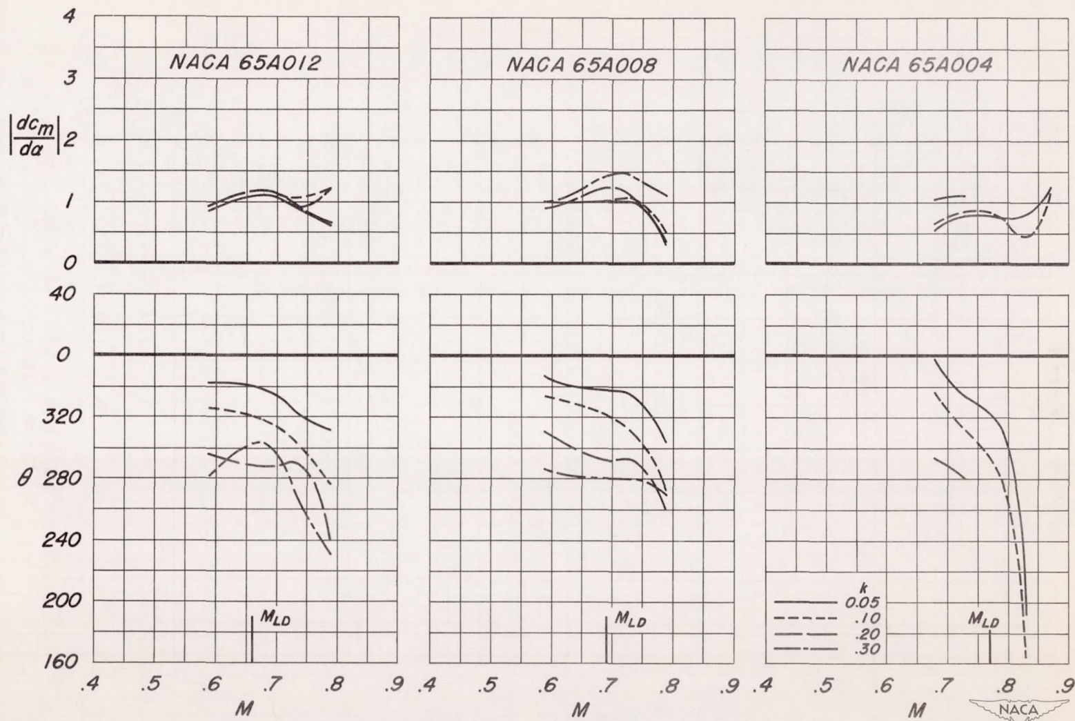
(b) Moment derivative and phase angle. Figure II.- Concluded.
