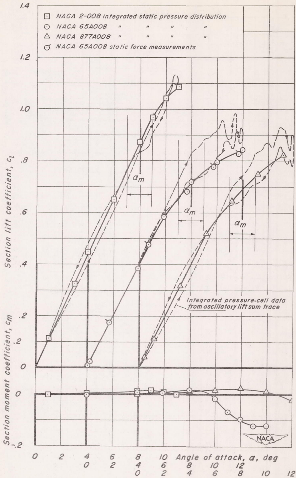
Figure 10.- Aerodynamic characteristics of the 8-percent-thick airfoils for 0.40 Mach number.
