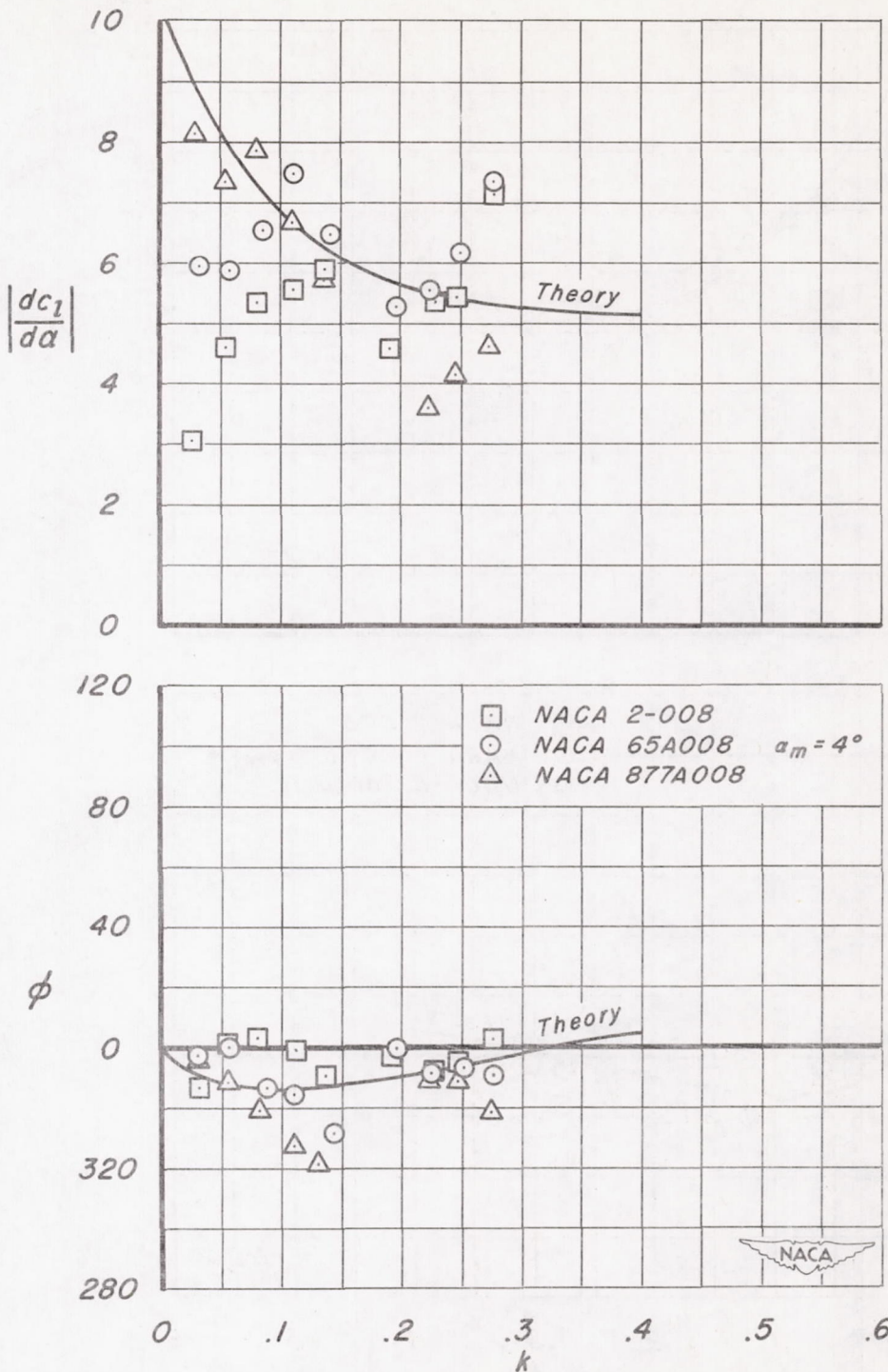
(f) Lift derivative and phase angle as a function of reduced frequency. M = 0.79 .
