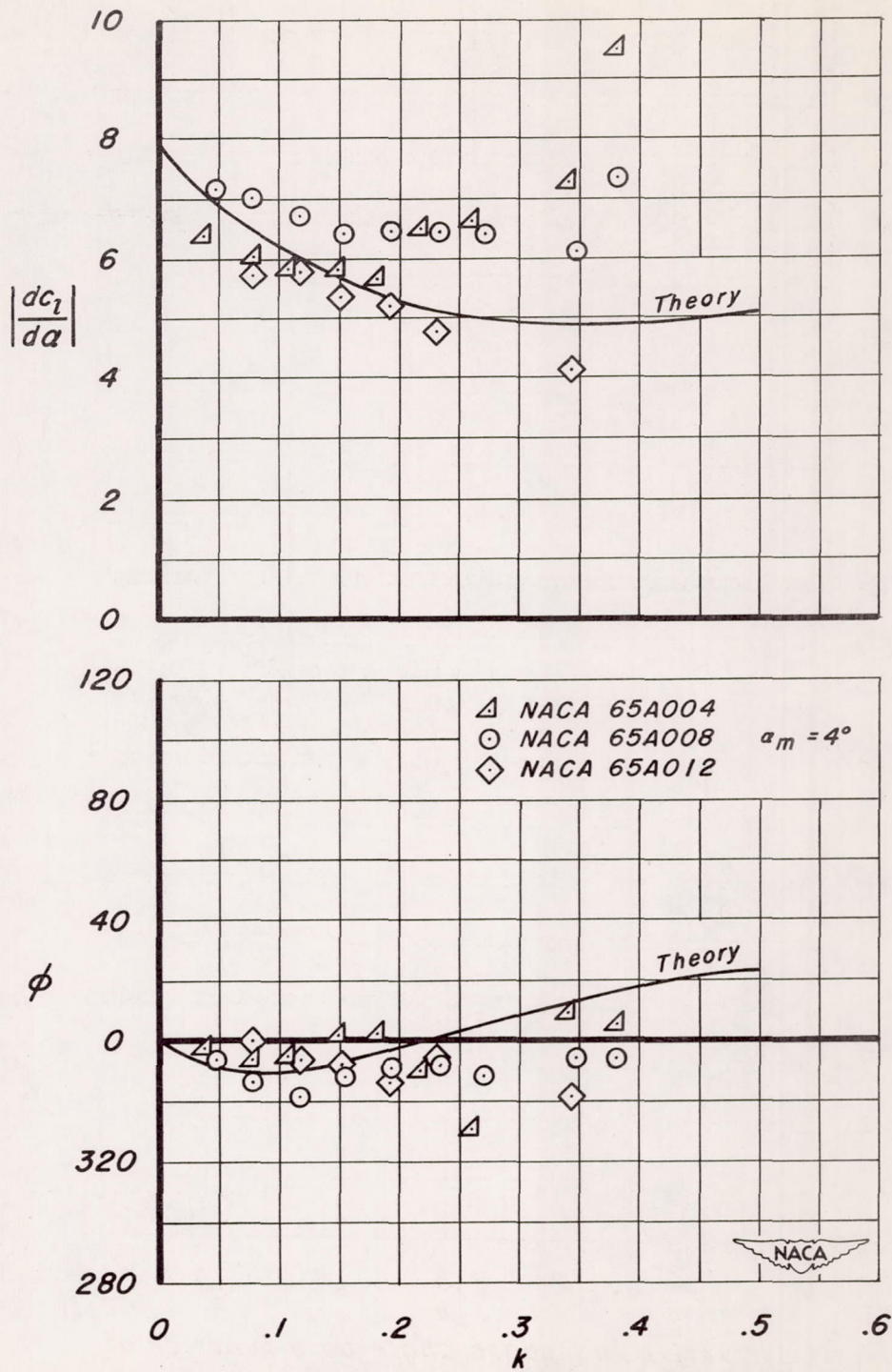
(b) Lift derivative and phase angle as a function of reduced frequency. M = 0.59 .
