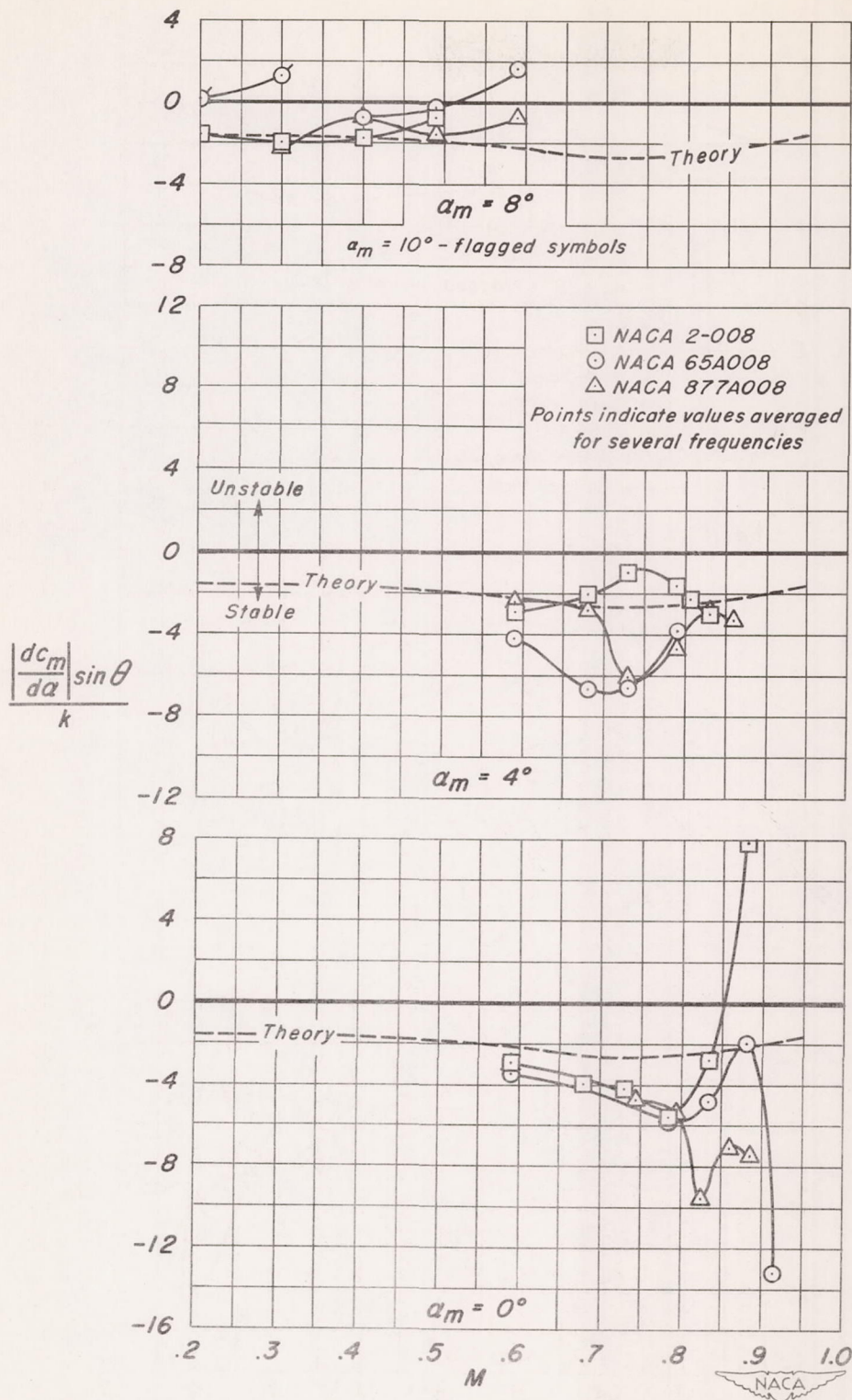
Figure 15.- The effect of airfoil thickness distribution on the torsional damping parameter. \alpha_m = 0^\circ, 4^\circ, and 8^\circ .
