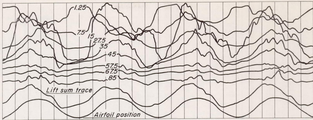
(a) Airfoil oscillating at 8° mean angle of attack, f=16.26 cps, M=0.59 .
