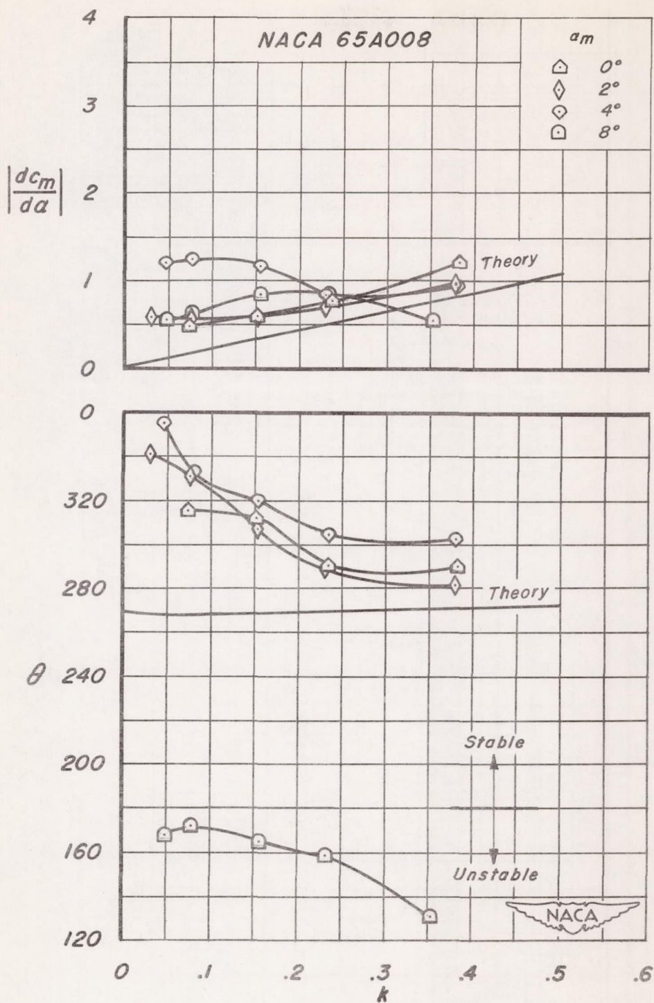
(b) Moment derivative and phase angle as a function of reduced frequency. M=0.59 .
