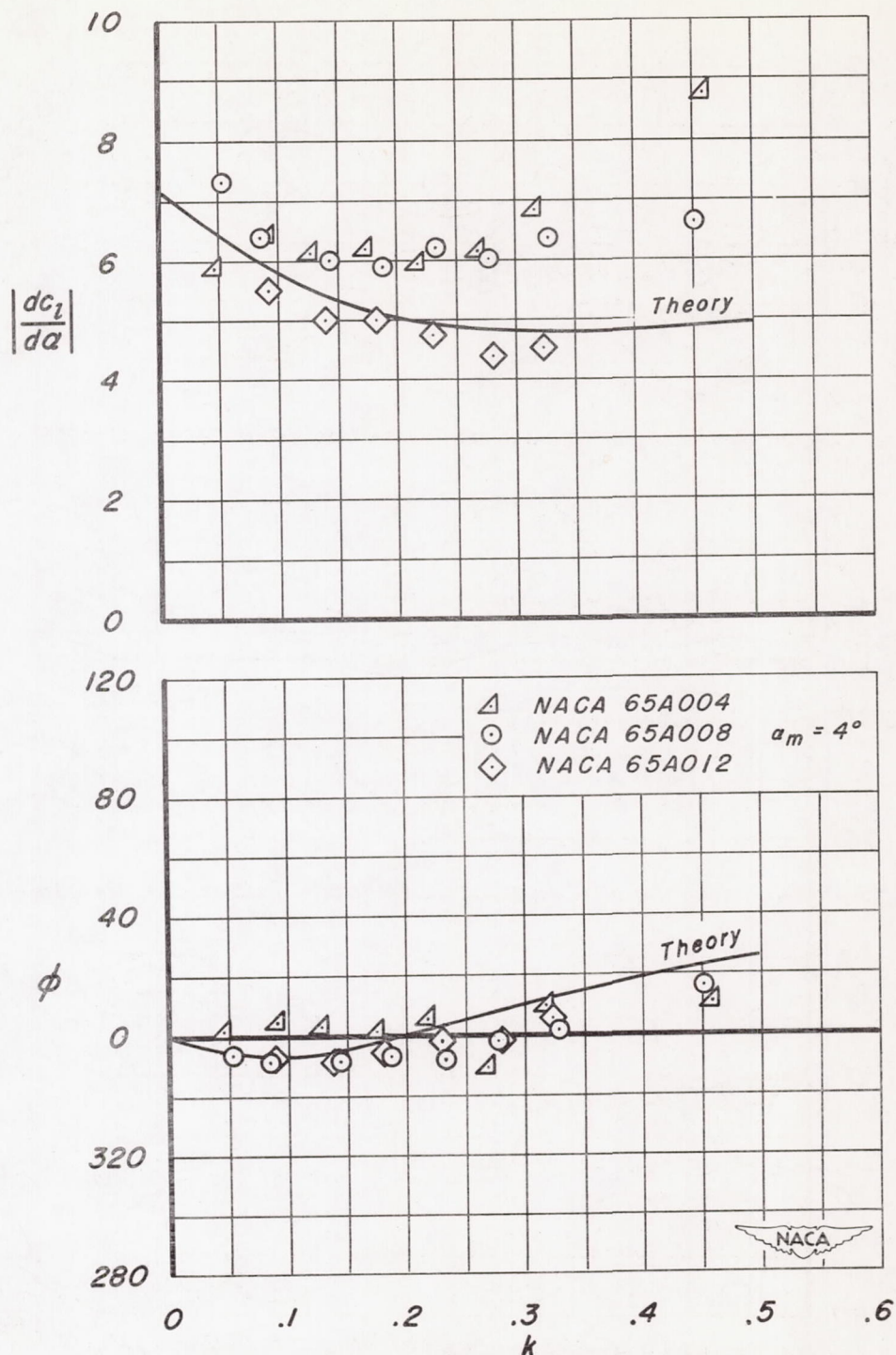
(a) Lift derivative and phase angle as a function of reduced frequency. M = 0.49 . Figure 4.- Effects of airfoil thickness on lift flutter derivative and phase angle.
