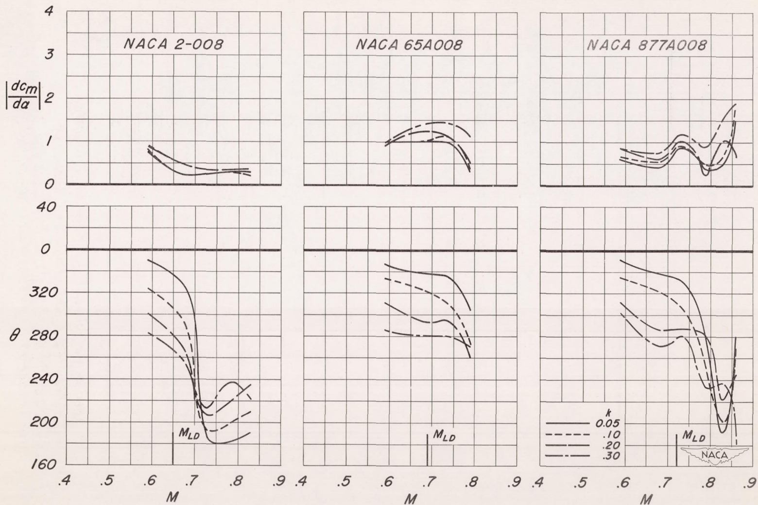
(b) Moment derivative and phase angle. Figure 12.- Concluded.
