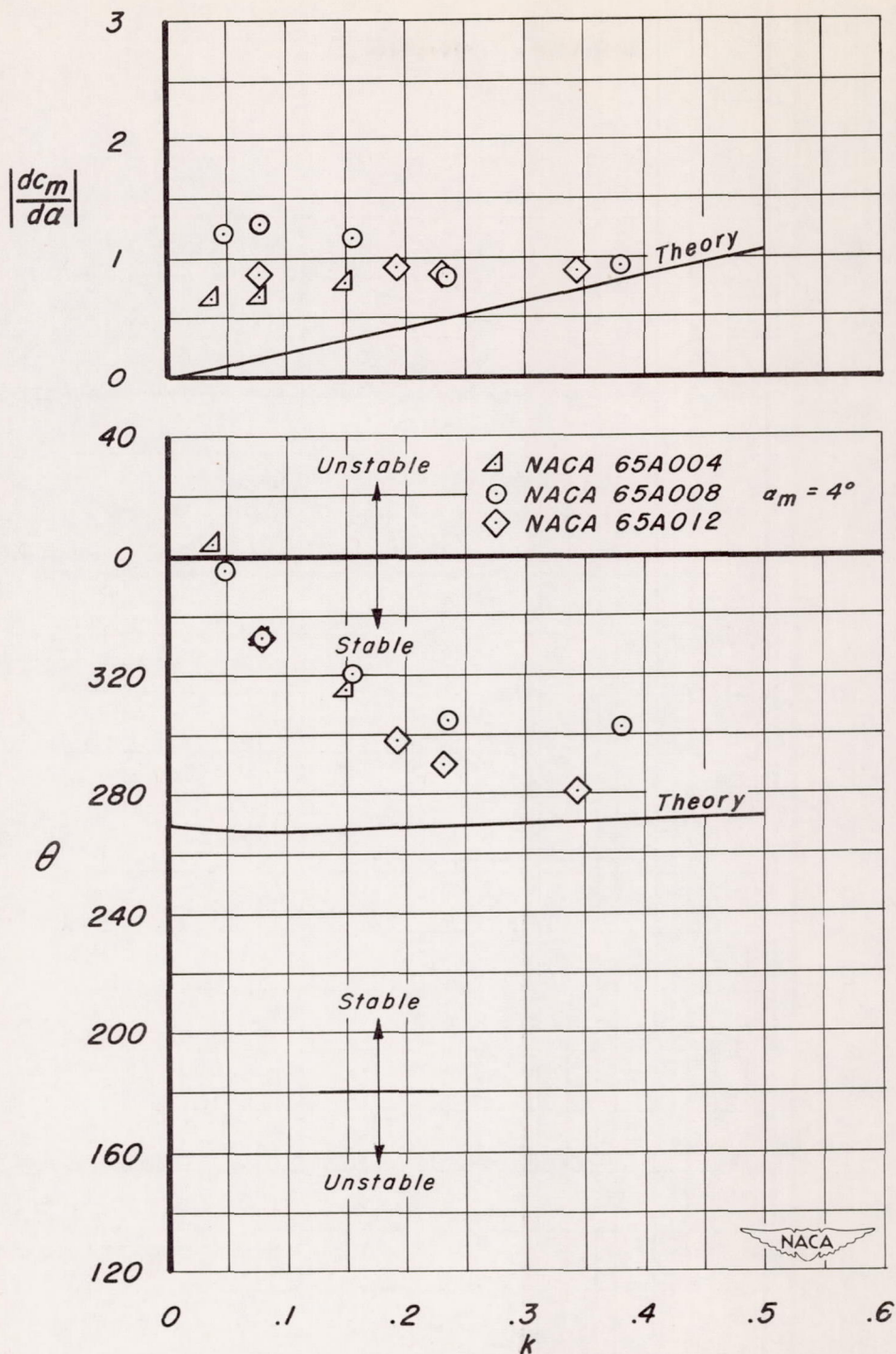
(a) Moment derivative and phase angle as a function of reduced frequency. M = 0.59 .
