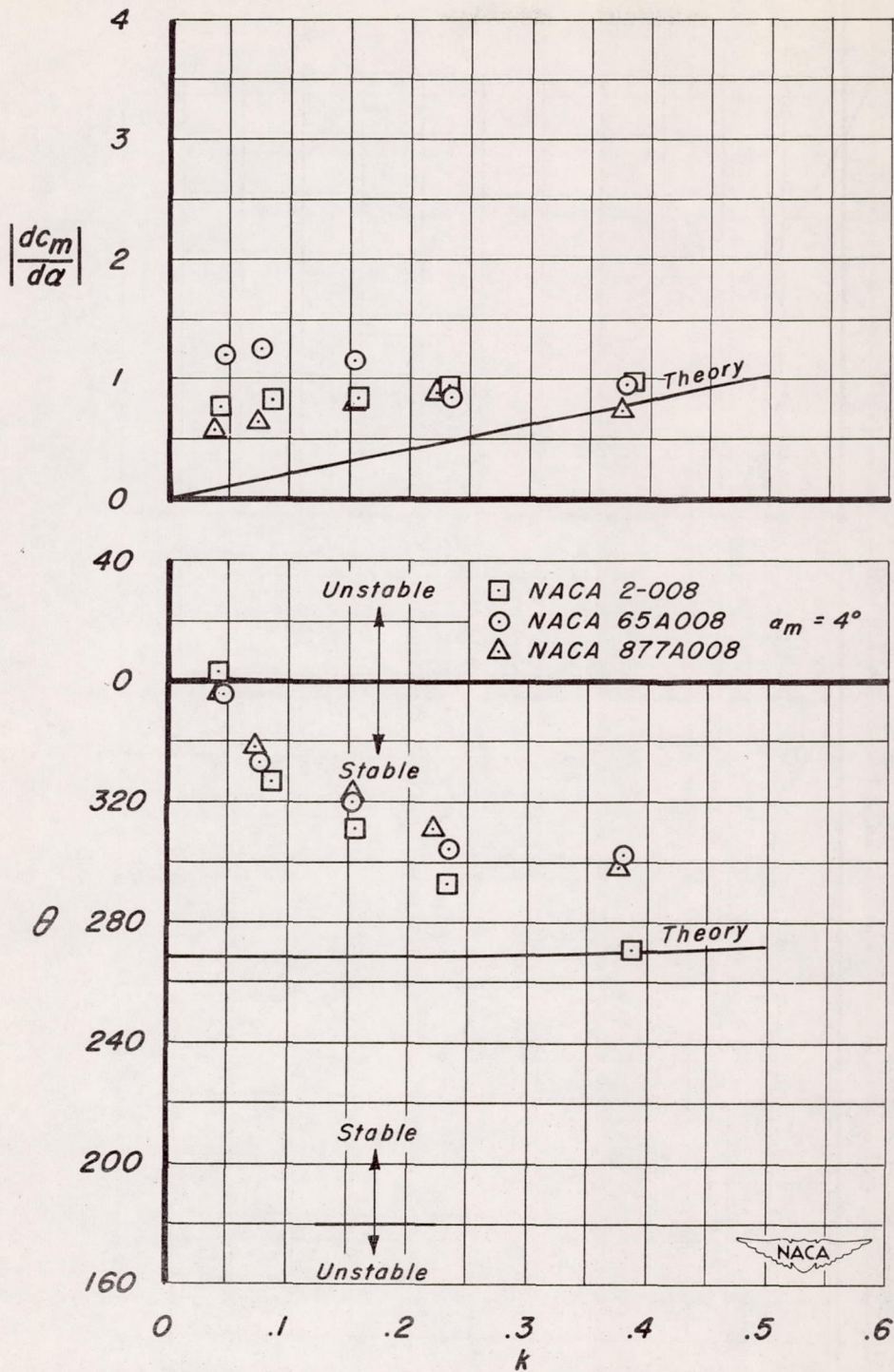
(a) Moment derivative and phase angle as a function of reduced frequency. M = 0.59 . Figure 7.- Effects of airfoil thickness distribution on moment flutter derivative and phase angle.
