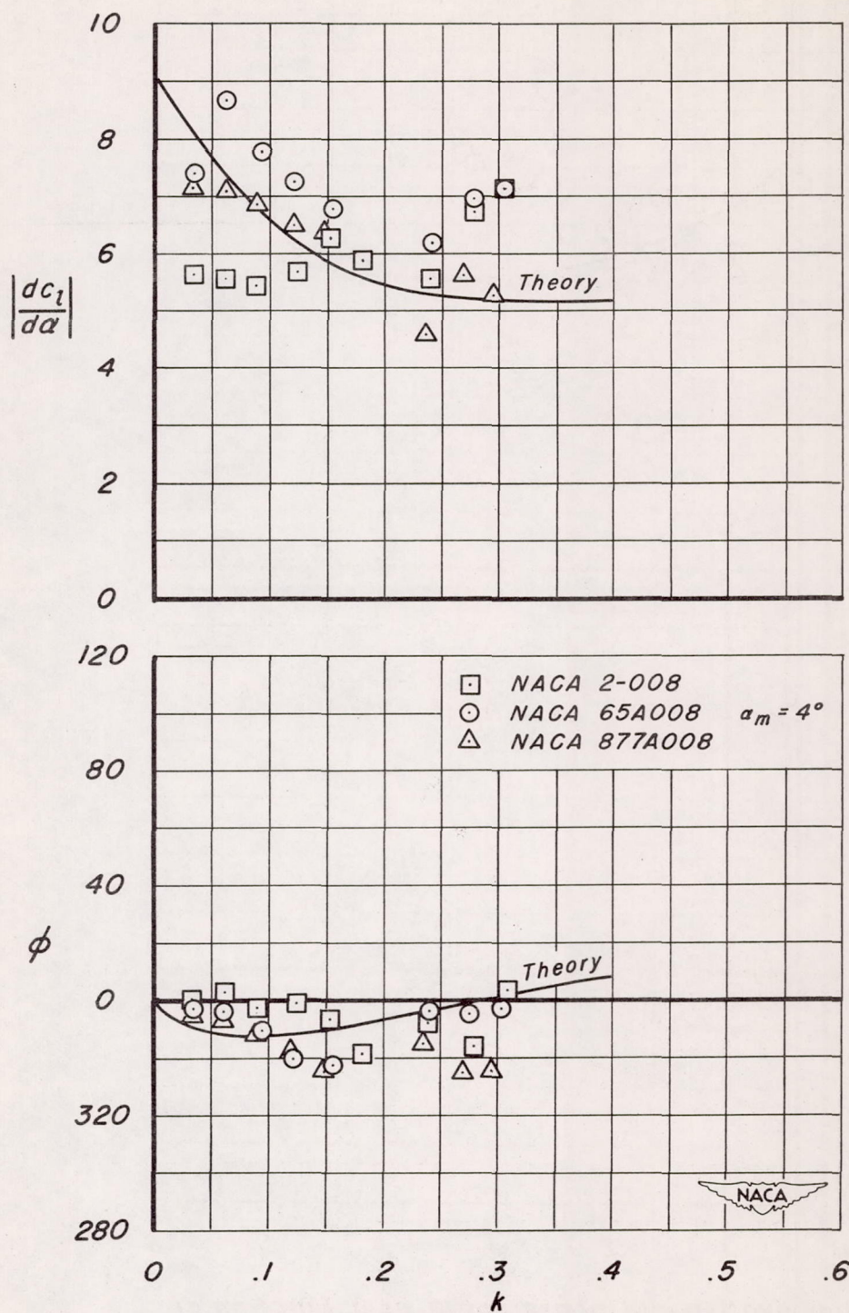
(e) Lift derivative and phase angle as a function of reduced frequency. M = 0.73 .
