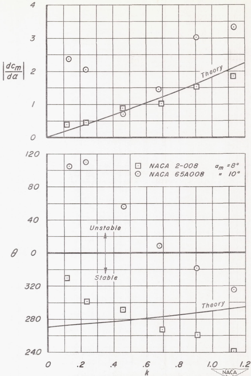
(a) Moment derivative and phase angle as a function of reduced frequency. M = 0.20 .
