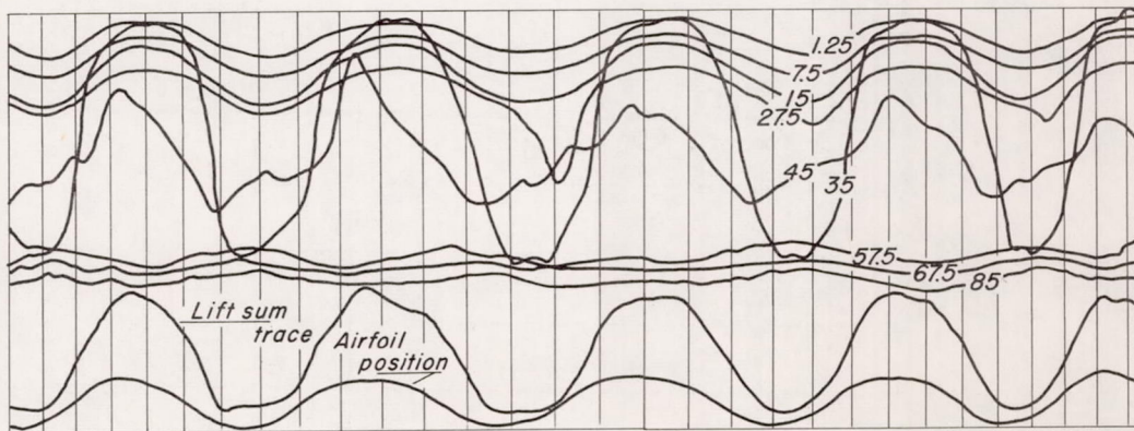
(c) Airfoil oscillating at 4° mean angle of attack, f=16.13 cps, M=0.79 .
