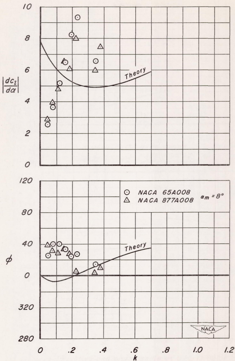
(e) Lift derivative and phase angle as a function of reduced frequency. M = 0.59 . Figure 8.- Concluded.
