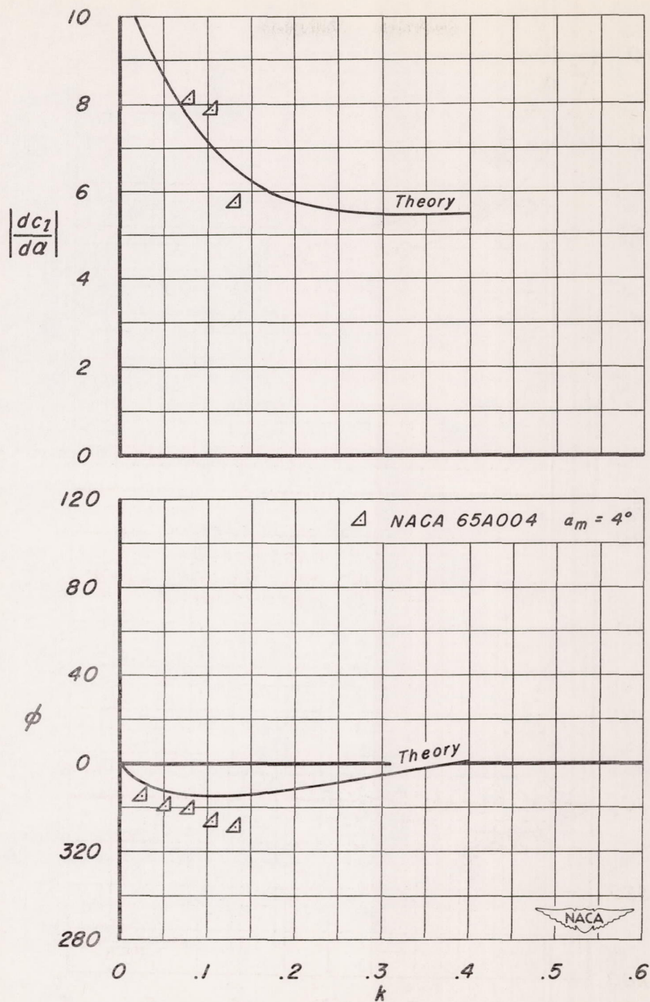
(f) Lift derivative and phase angle as a function of reduced frequency. M = 0.83 . Figure 4.- Continued.
