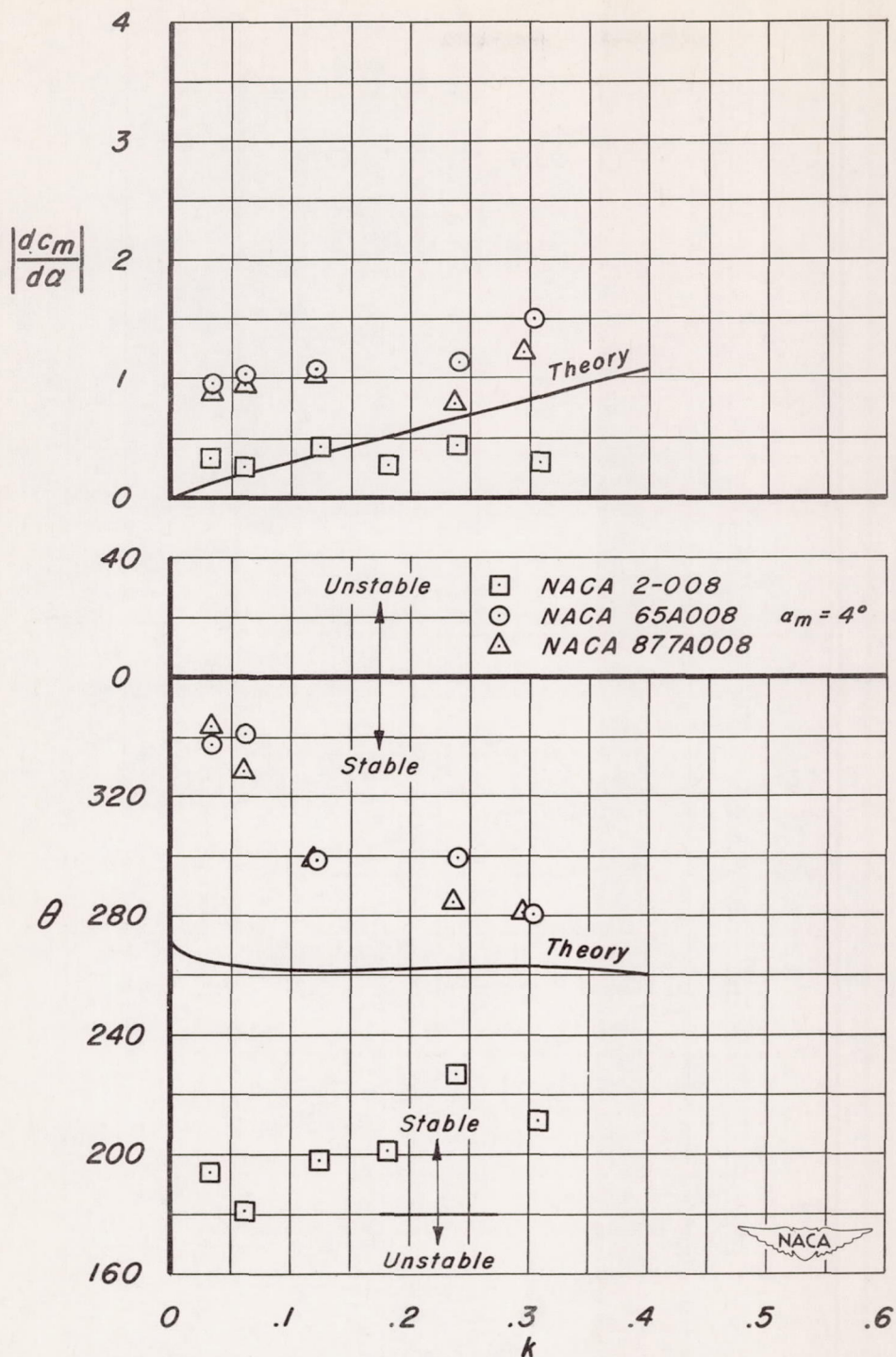
(c) Moment derivative and phase angle as a function of reduced frequency. M = 0.73 Figure 7.- Continued.
