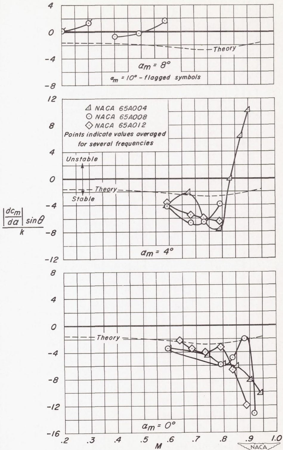
Figure 14.- The effect of airfoil thickness on the torsional damping parameter. \alpha_m = 0^\circ, 4^\circ, and 8^\circ .
