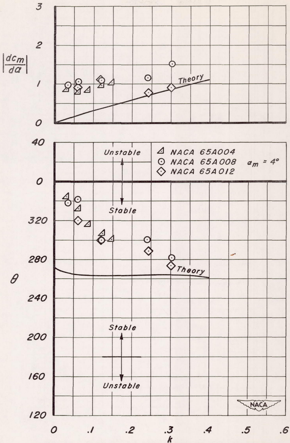
(c) Moment derivative and phase angle as a function of reduced frequency. M=0.73 .
