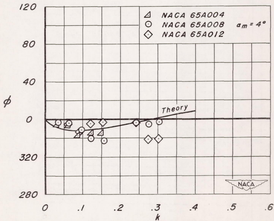
(d) Lift derivative and phase angle as a function of reduced frequency. M = 0.73 .
