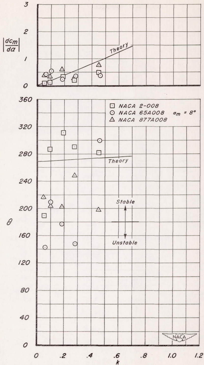
(d) Moment derivative and phase angle as a function of reduced frequency. M = 0.50 .
