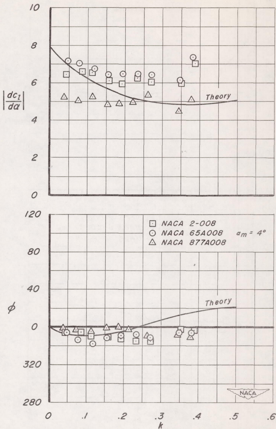
(c) Lift derivative and phase angle as a function of reduced frequency. M = 0.59 .
