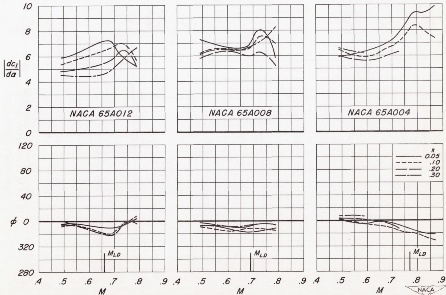
(a) Lift derivative and phase angle.
