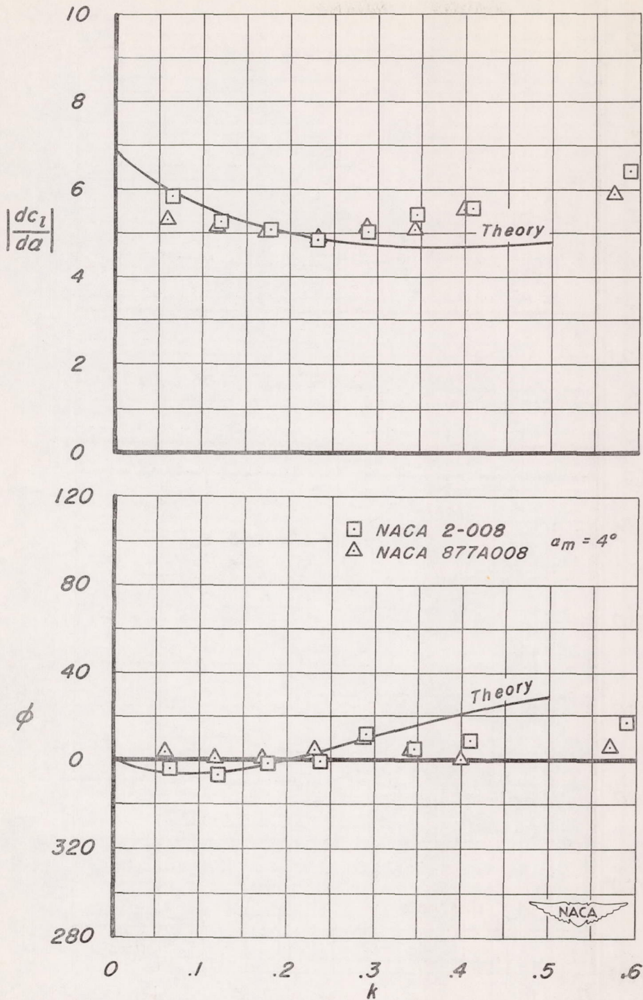
(a) Lift derivative and phase angle as a function of reduced frequency. M = 0.40 . Figure 6.- Effects of airfoil thickness distribution on lift flutter derivative and phase angle.
