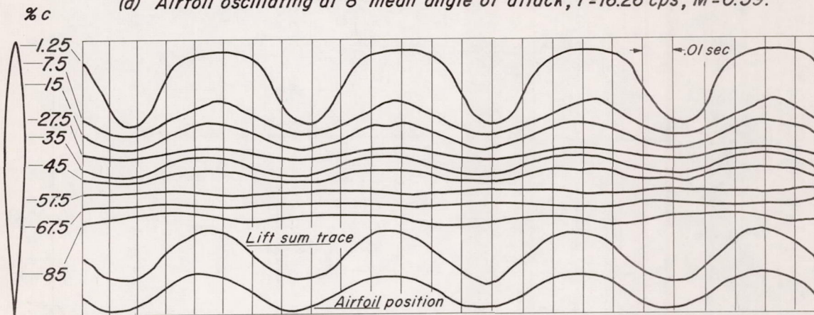
(b) Airfoil oscillating at 4° mean angle of attack, f=16.26 cps, M=0.59 .
