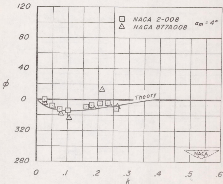
(g) Lift derivative and phase angle as a function of reduced frequency. M = 0.83 .
