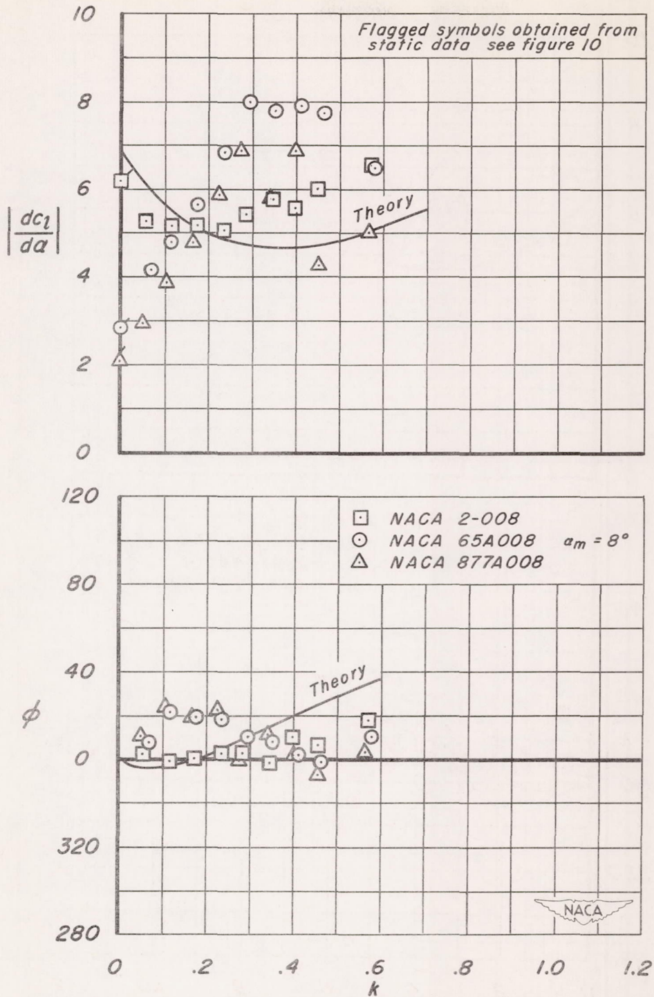
(c) Lift derivative and phase angle as a function of reduced frequency. M = 0.40 .
