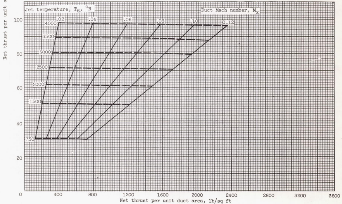
(b) Variable-area tip-jet nozzle; pressure ratio, 3.0; tip speed, 500 feet per second; \Delta P_f = 2.5q_x ; burner area/duct area, 1.5.
