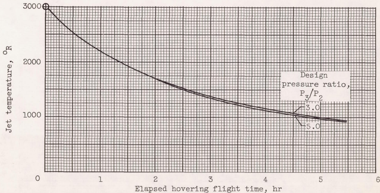
Figure 12. - Jet temperature as function of elapsed hovering time. Design jet temperature, 3000° R; tip speed, 700 feet per second; duct area/section area, 0.3; burner area/section area, 0.45.
