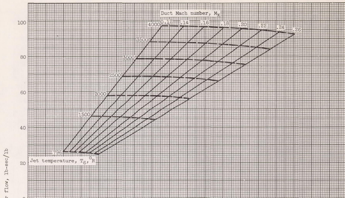
(o) Variable-area tip-jet nozzle; pressure ratio, 4.0; tip speed, 900 feet per second; \Delta P_f = 2.5q_x ; burner area/duct area, 1.5.
