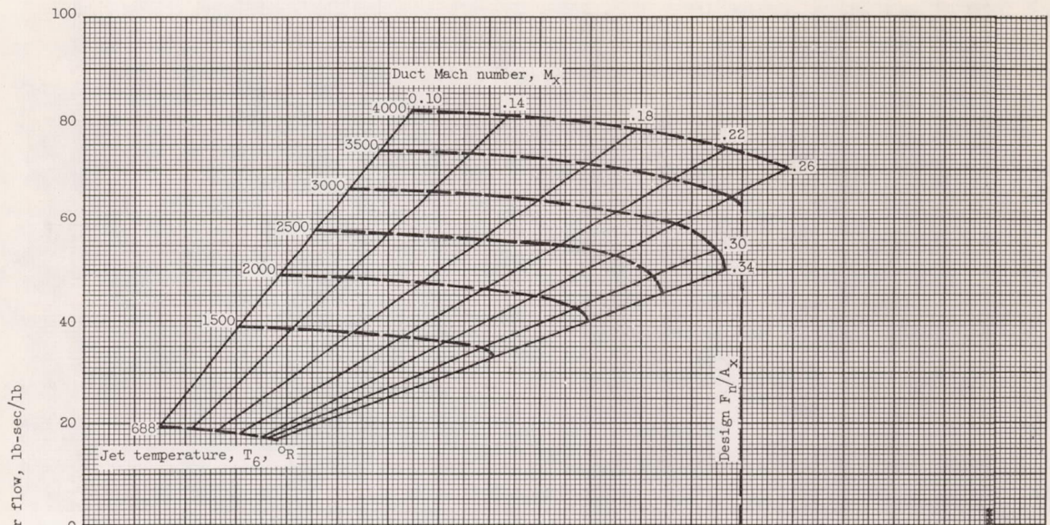
(g) Variable-area tip-jet nozzle; pressure ratio, 2.25; tip speed, 700 feet per second; \Delta P_f = 2.5q_x ; burner area/duct area, 1.5.
