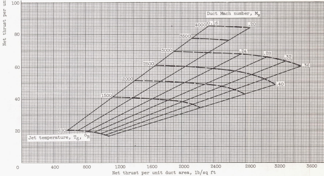
(j) Variable-area tip-jet nozzle; pressure ratio, 2.5; tip speed, 700 feet per second; \Delta P_f = 2.5q_x ; burner area/duct area, 2.5.
