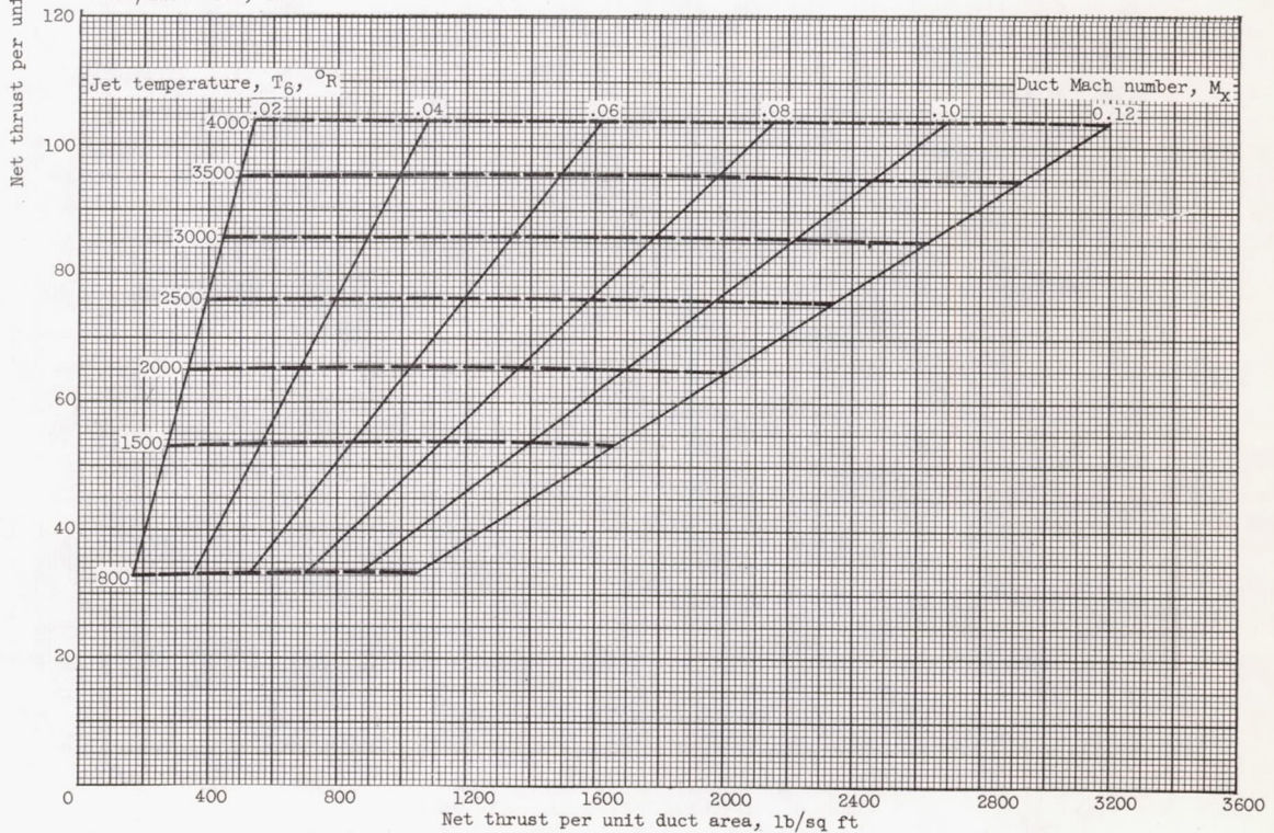
(f) Variable-area tip-jet nozzle; pressure ratio, 4.0; tip speed, 600 feet per second; \Delta P_f = 2.5q_x ; burner area/duct area, 1.5.
