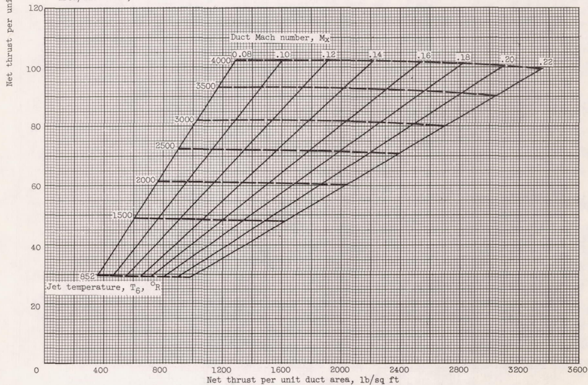
(p) Variable-area tip-jet nozzle; pressure ratio, 5.0; tip speed, 900 feet per second; \Delta P_f = 2.5q_x ; burner area/duct area, 1.5.
