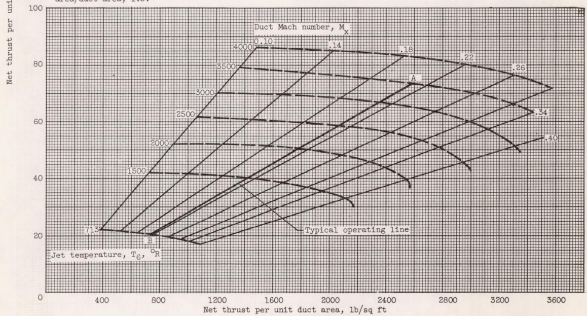
(h) Variable-area tip-jet nozzle; pressure ratio, 2.5; tip speed, 700 feet per second; \Delta P_f = 2.5q_x ; burner area/duct area, 1.5.
