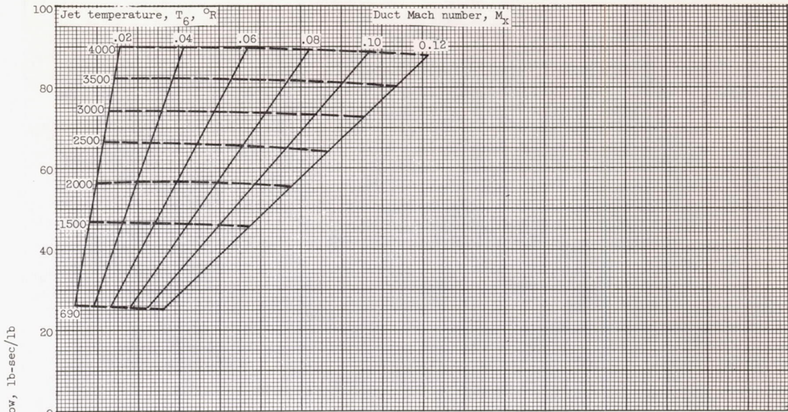
(a) Variable-area tip-jet nozzle; pressure ratio, 2.5; tip speed, 500 feet per second; \Delta P_f = 2.5q_x ; burner area/duct area, 1.5.
