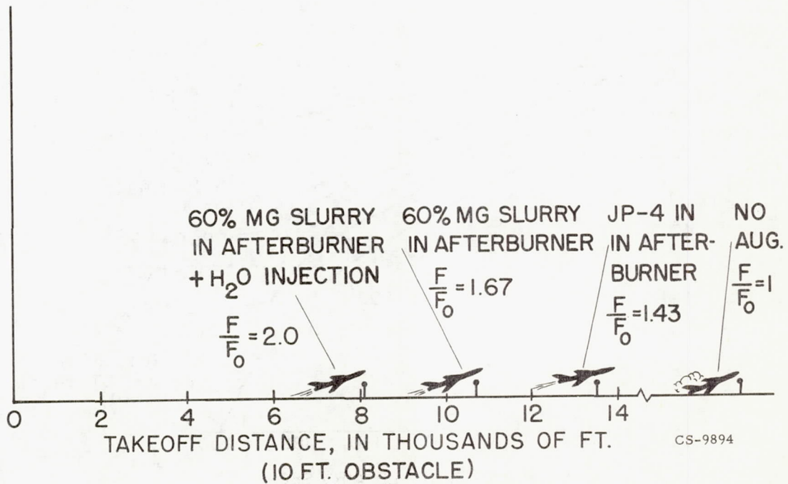
Figure 4. - Take-off characteristics of a turbojet bomber. F , augmented thrust; F_0 , unaugmented thrust.
