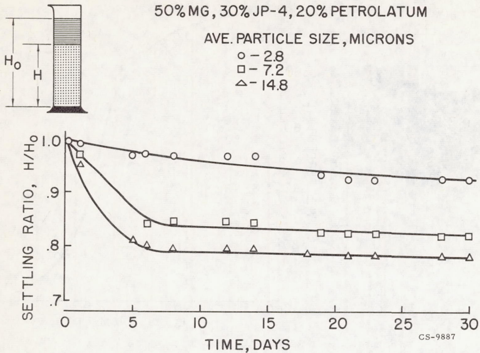
Figure 5. - Settling characteristics of magnesium particles. H, height of column of settled particles; H_0 , height of liquid column.
