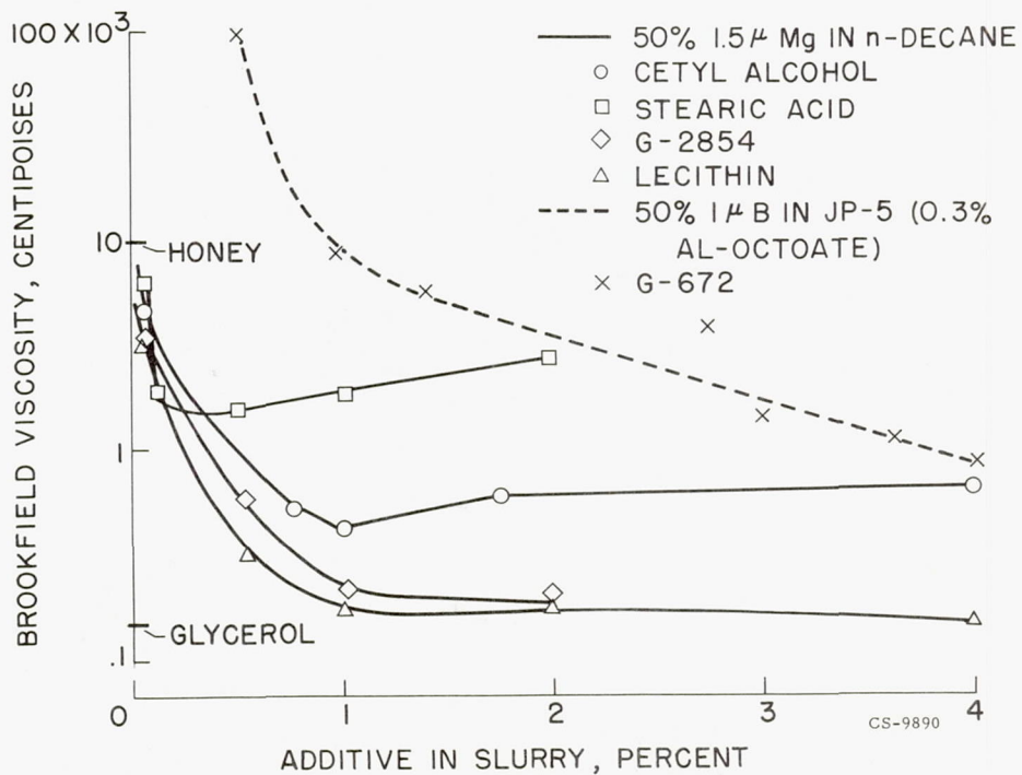
Figure 8. - Dispersing effect of surface-active agents.
