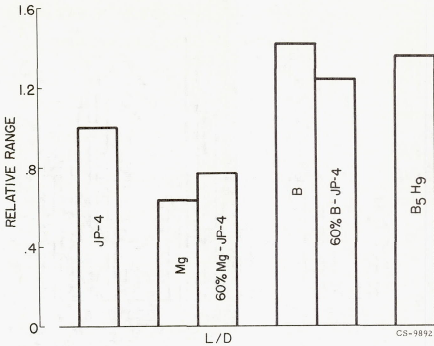
Figure 3. - Relative range of ram-jet missile. Initial altitude, 60,000 ft; free-stream Mach number, 3.2.
