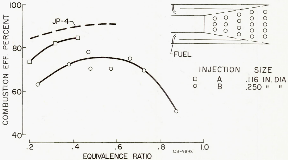
Figure 20. - Performance of 50-percent boron slurry in 16-inch ram-jet combustor. Pressure, 1 atmosphere; velocity, 260 feet per second; temperature, 560° F.
