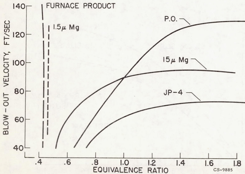
Figure 22. - Flame stability of 50-percent magnesium slurries.
