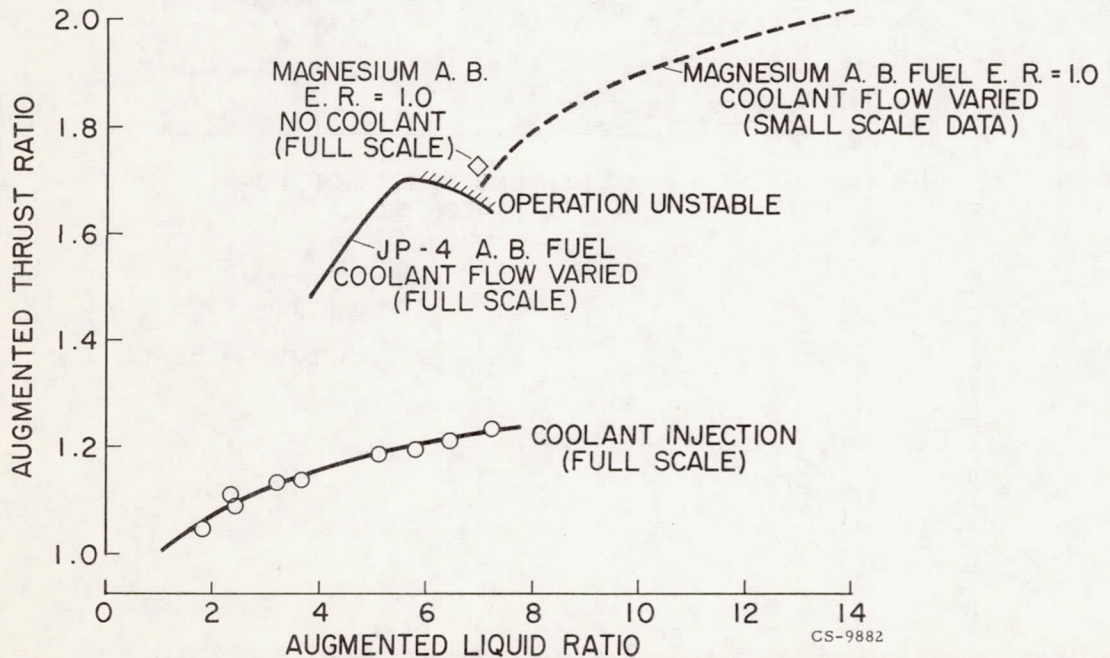
Figure 26. - Turbojet engine thrust augmentation with magnesium slurries (sea level static).
