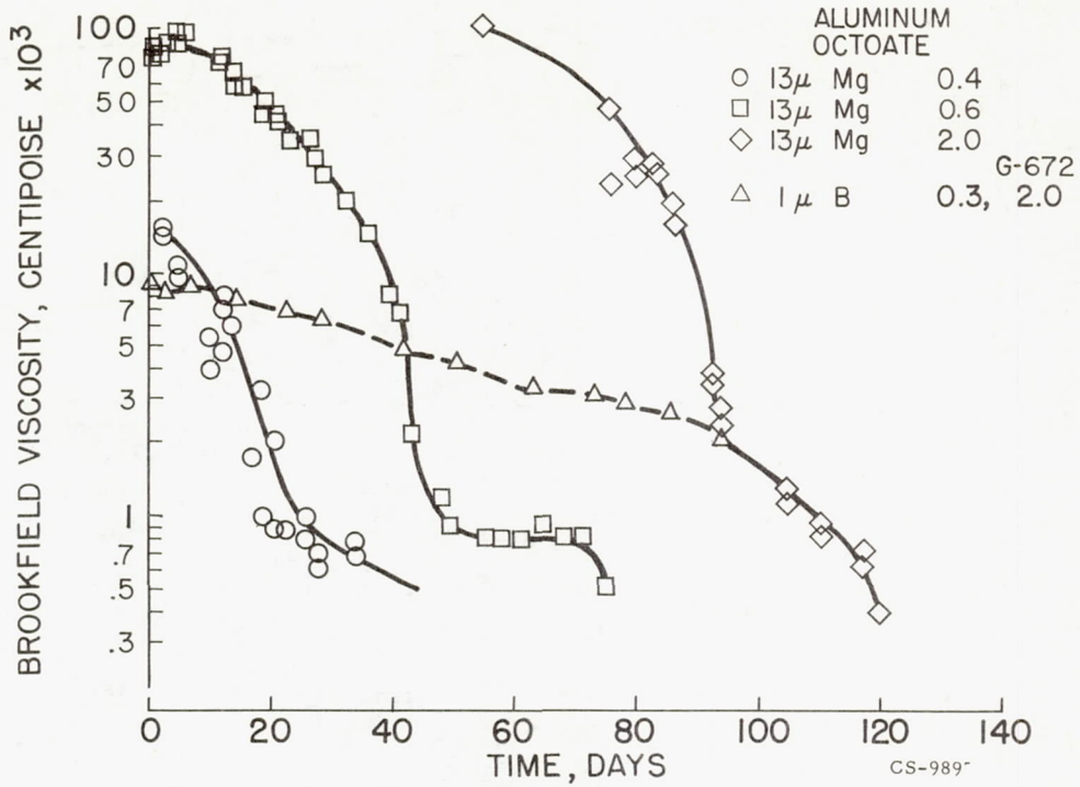
Figure 11. - Aging of 50-percent slurries containing gelling agent.
