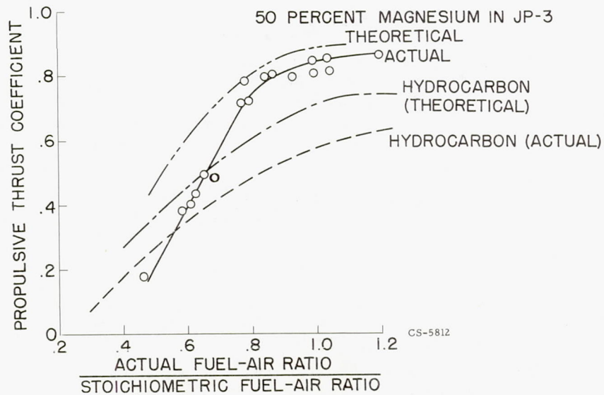
Figure 28. - Magnesium slurry performance.
