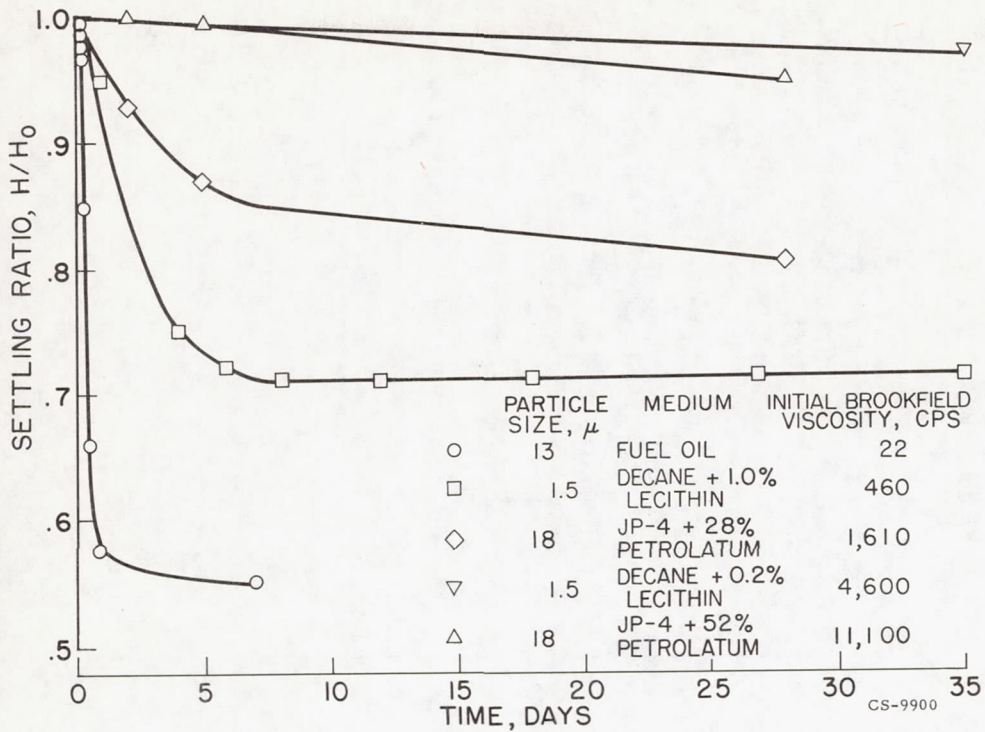
Figure 9. - Settling characteristics of 50-percent magnesium in various media. H, height of column of settled particles; H_0 , height of liquid column.
