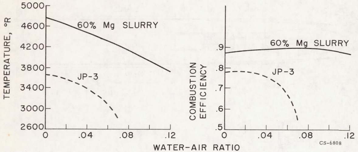
Figure 25. - Temperature and combustion efficiency in small-scale afterburner.
