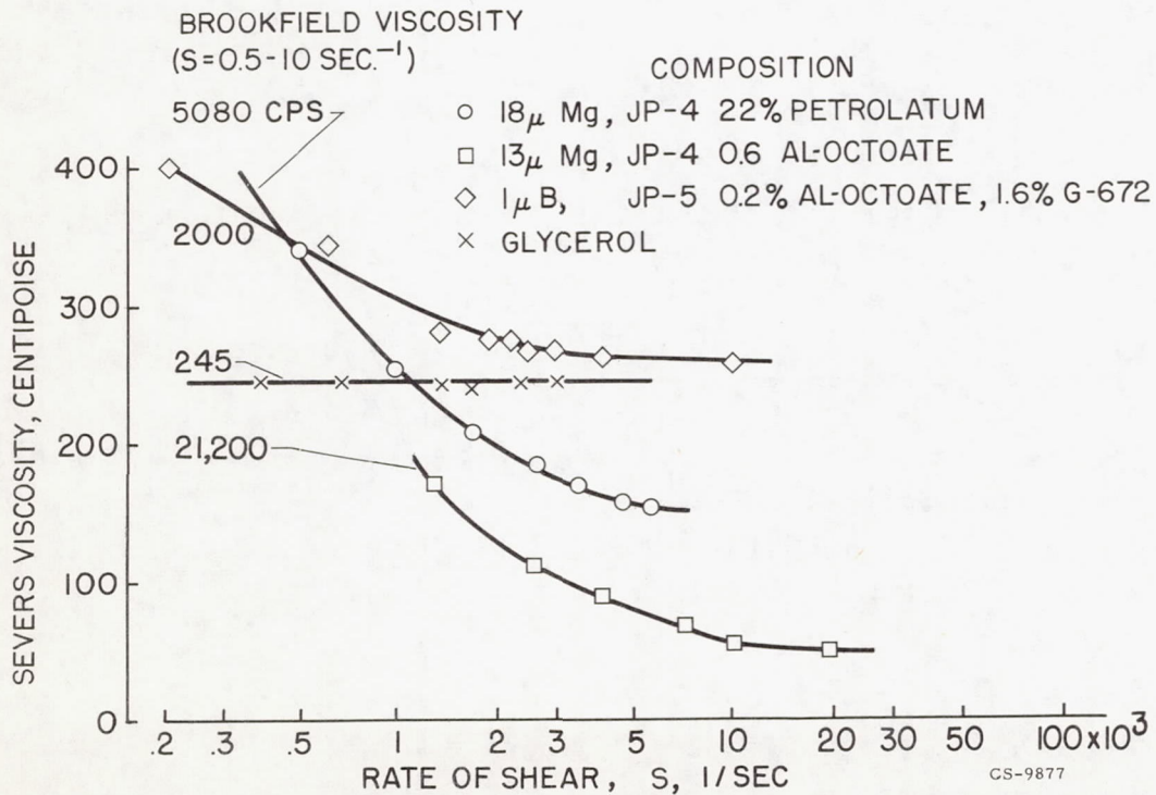
Figure 10. - Effect of rate of shear on viscosity of 50-percent slurries
