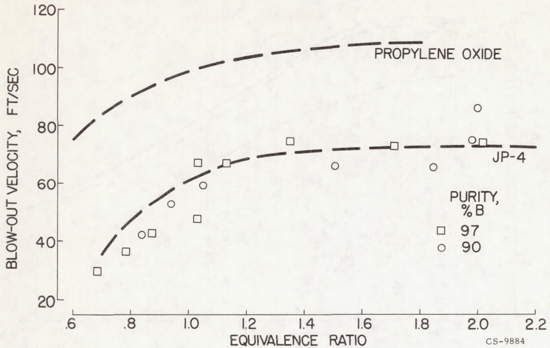
Figure 13. - Blow-out velocity of two 50-percent boron slurries. Burner diameter, 2 inches.
