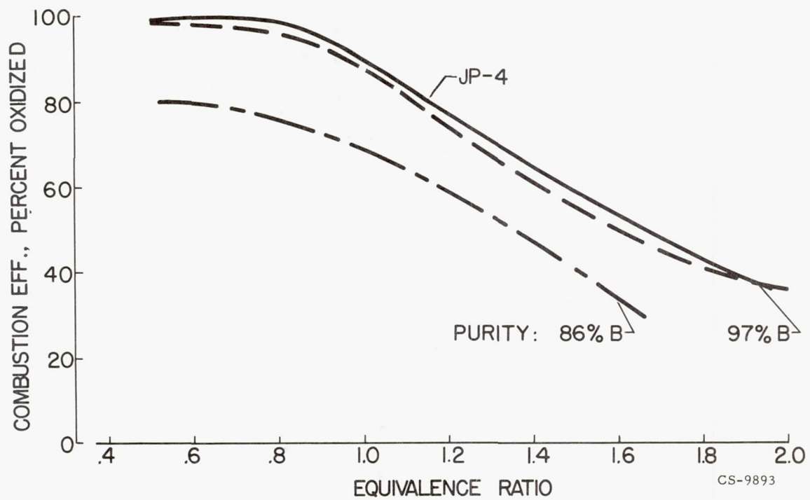
Figure 15. - Combustion efficiency of 30-percent boron slurries.
