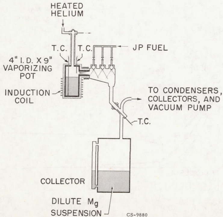
Figure 6. - Preparation of small particles from magnesium vapor.
