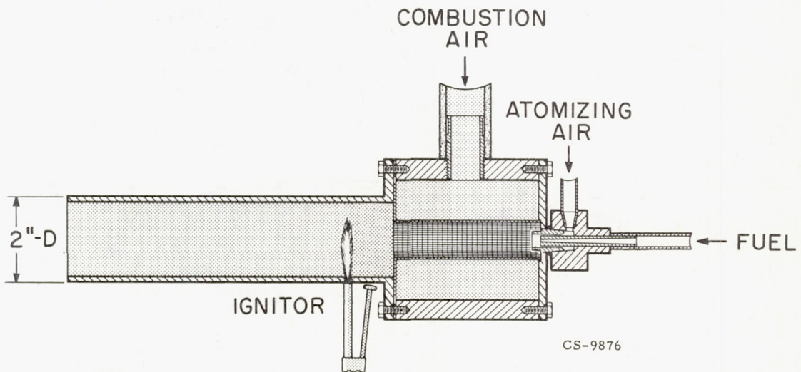
Figure 12. - Blow-out velocity apparatus.
