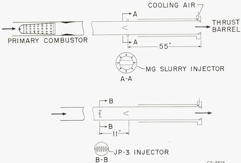
Figure 23. - Simulated afterburner of 6-inch diameter.
