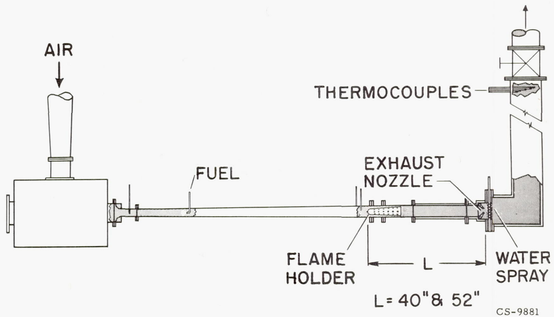
Figure 16. - 5-Inch-diameter ram-jet burner used for boron fuels.
