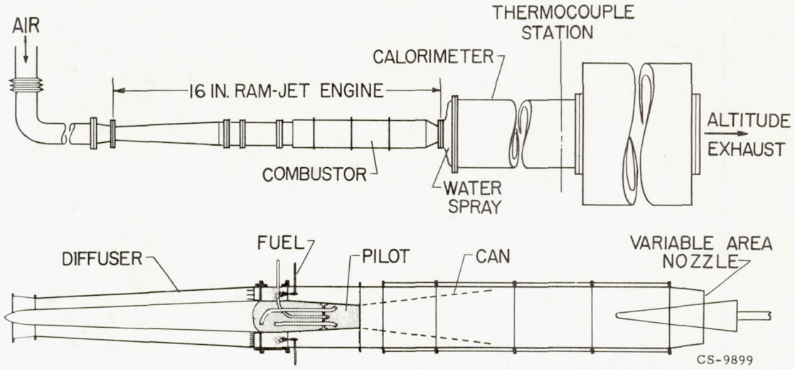
Figure 19. - 16-Inch-diameter ram-jet engine used for boron fuels.
