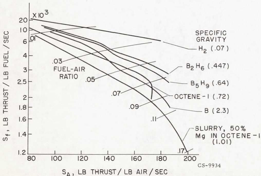
Figure 2. - Impulse characteristics of jet engine fuels.
