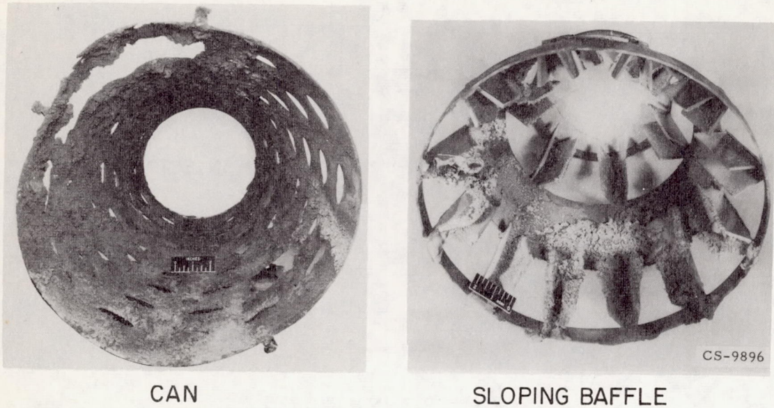
Figure 21. - Combustors after use of boron fuel.
