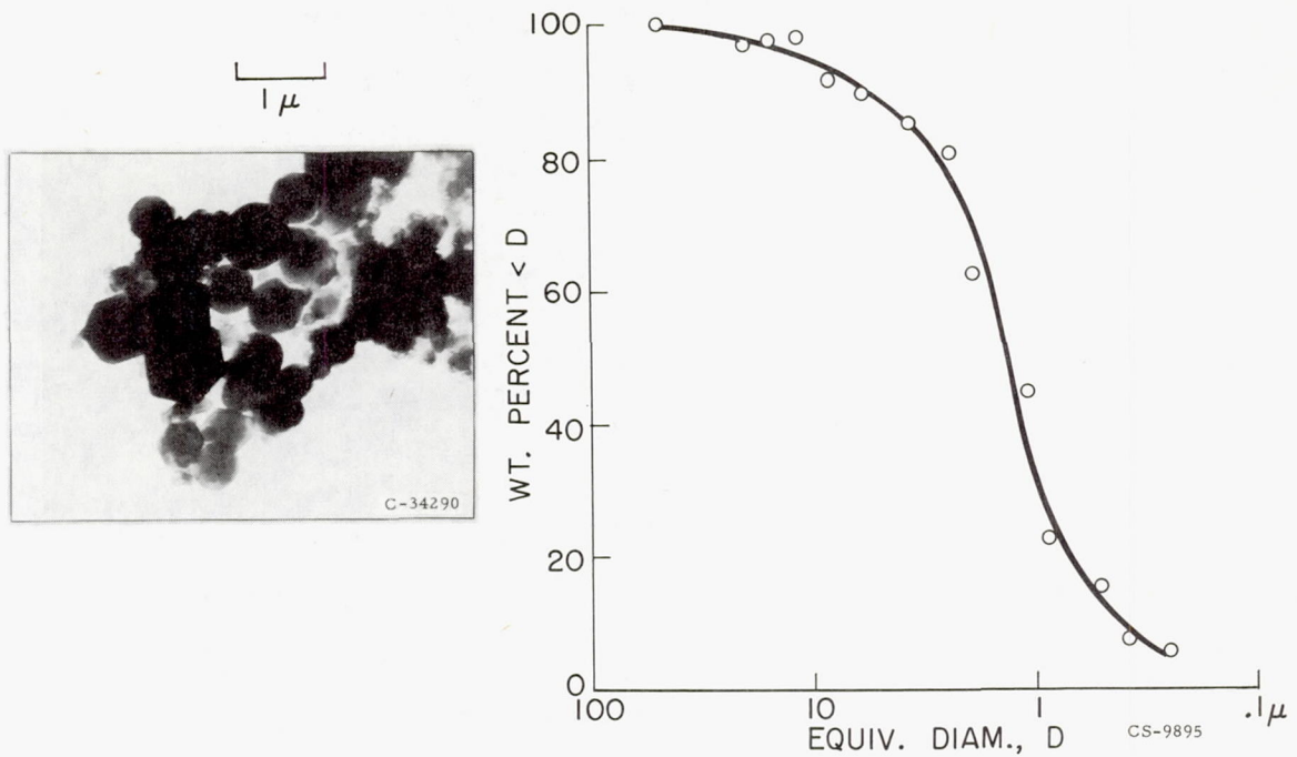
Figure 7. - Particles from magnesium vapor.
