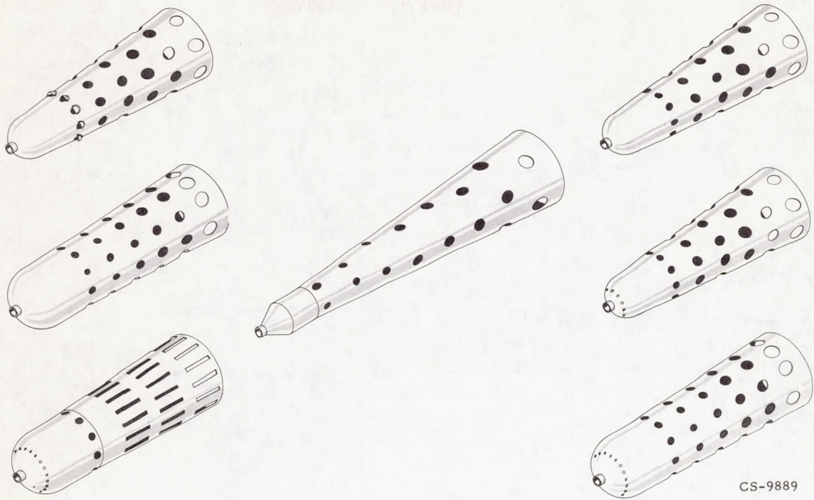
Figure 17. - Boron-slurry flame holders.
