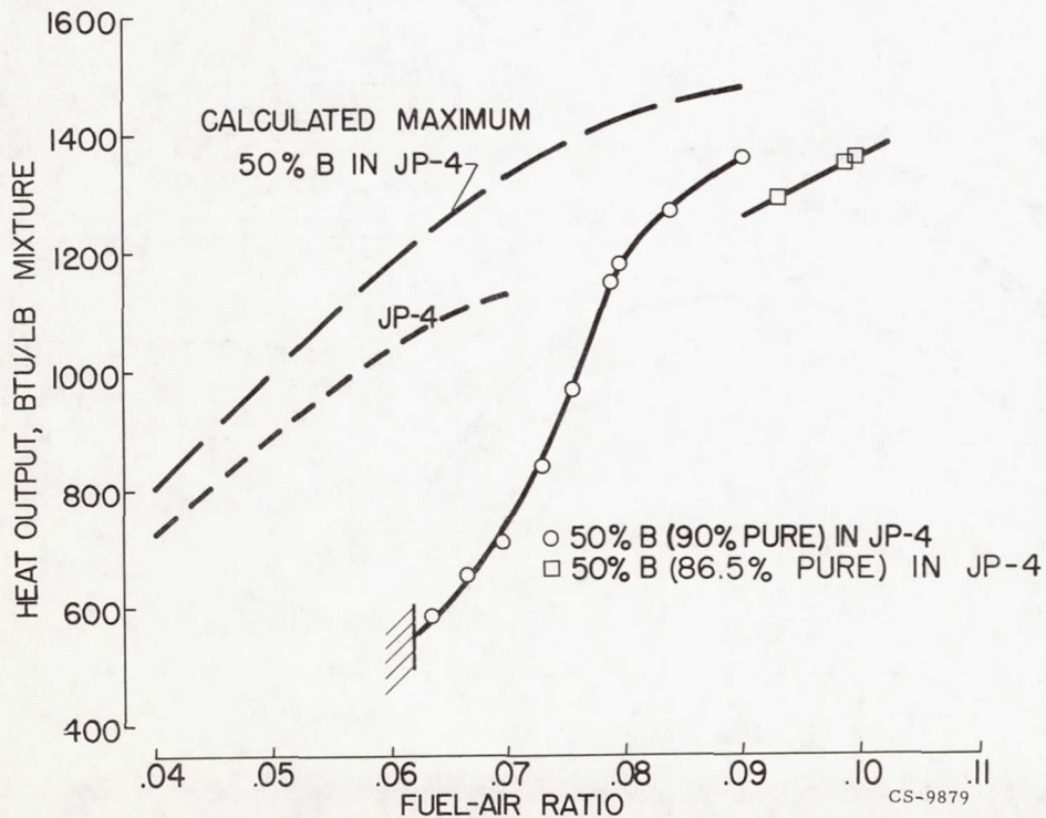
Figure 18. - Combustion of boron slurries in 5-inch diameter burner. Burner length, 40 inches; temperature, approximately 680° R; pressure, 11.8 to 14.8 square inches absolute; velocity, 131 to 181 feet per second.
