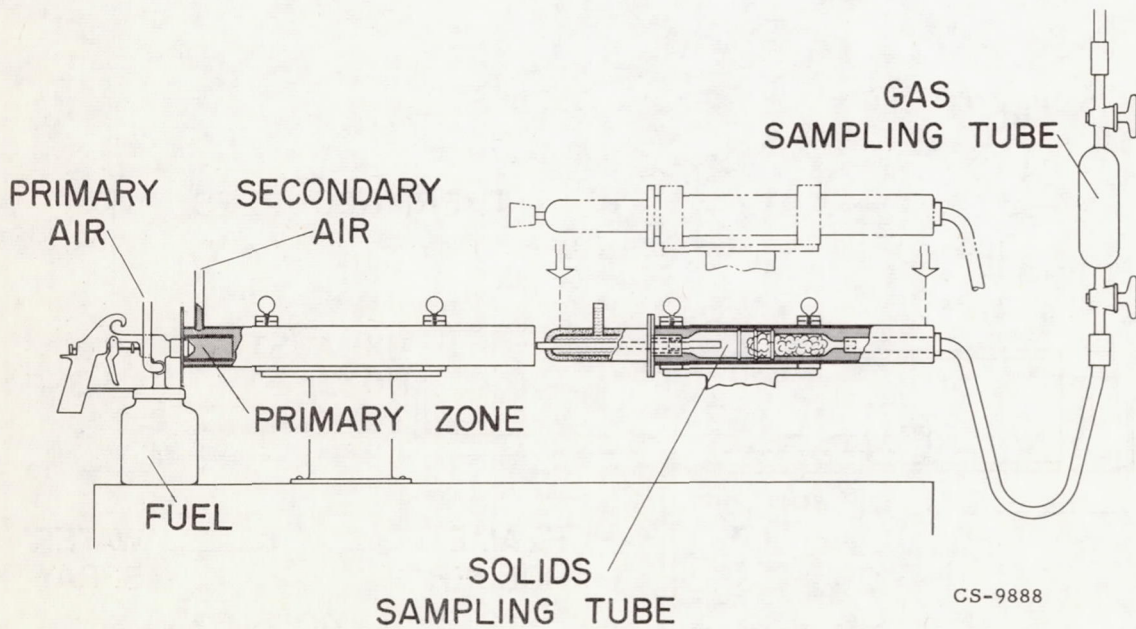
Figure 14. - Slurry burner and exhaust sampling device.
