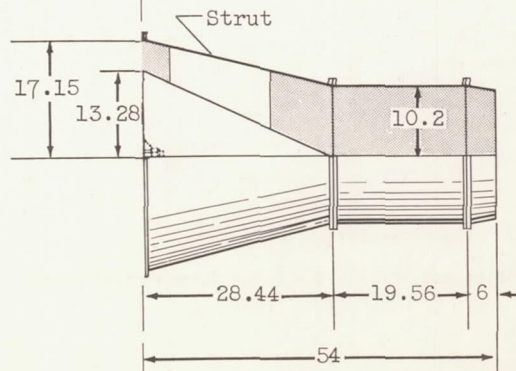
(c) Standard tail pipe.
