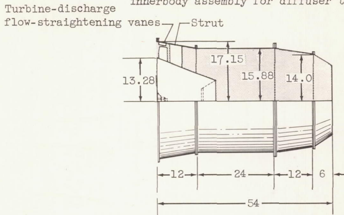
(b) 18-Inch conical innerbody diffuser (ref.1).
