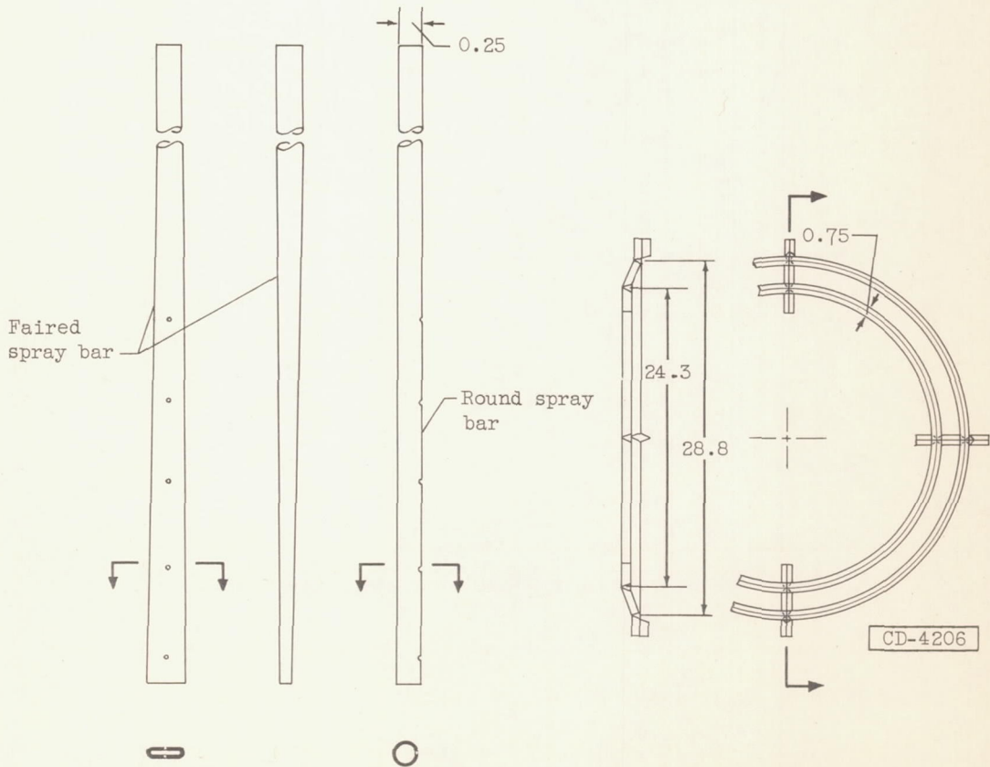
(b) Faired and round spray bars.
