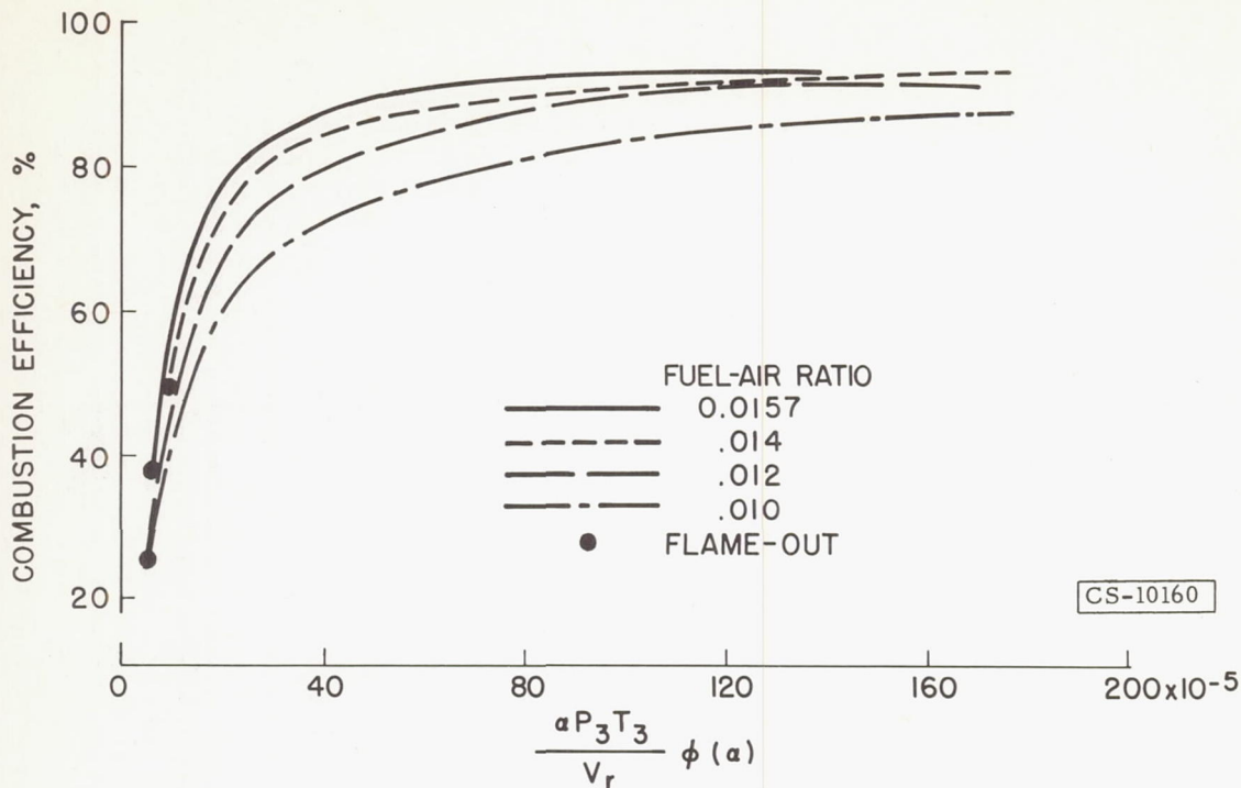
Figure 13. - Combustor operating lines for several fuel-air ratios.
