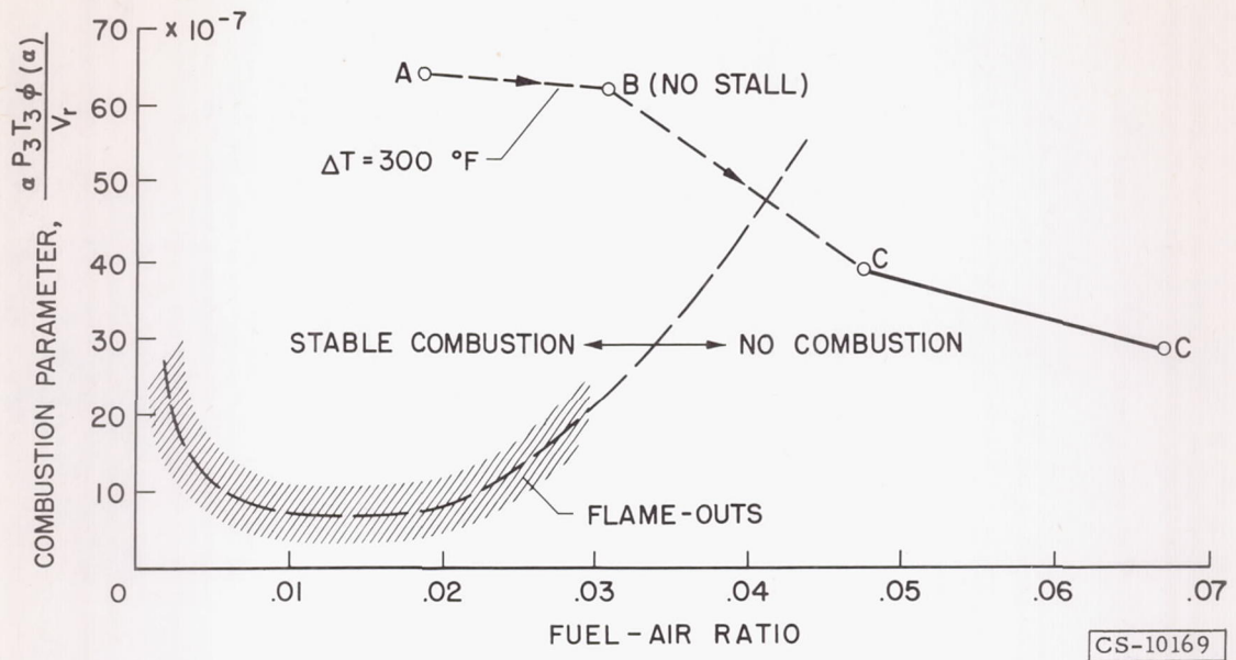
Figure 15. - Combustor conditions during rocket firing.
