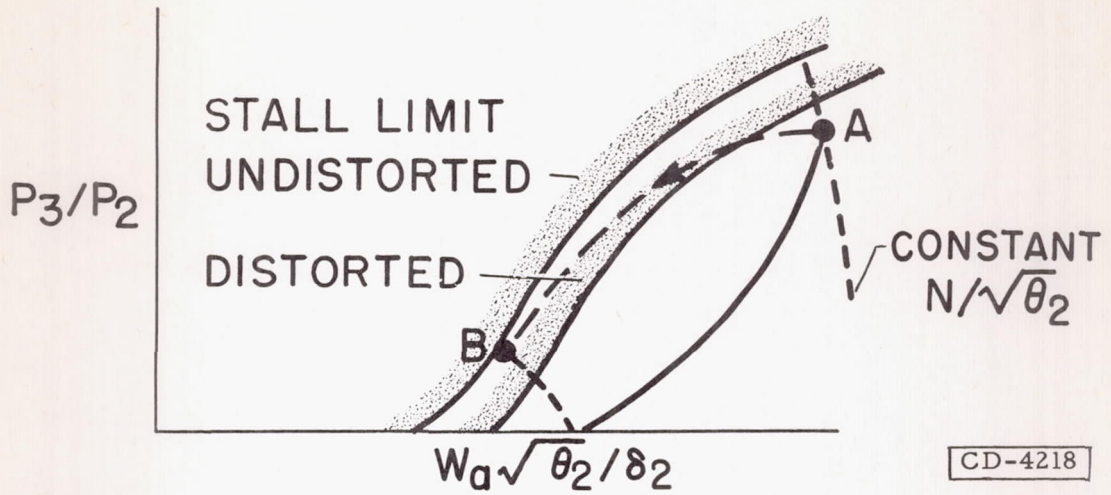
Figure 11. - Effect of inlet distortions.
