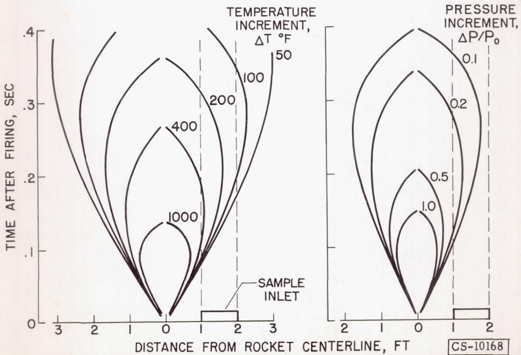
Figure 4. - Pressure and temperature increments for 2.75-inch rocket. Free-stream Mach number, 0.9; altitude, 45,000 feet.
