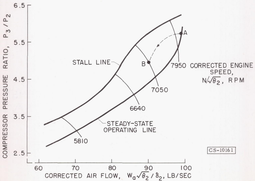
Figure 8. - Theoretical compressor operation for instantaneous inlet-temperature increase.
