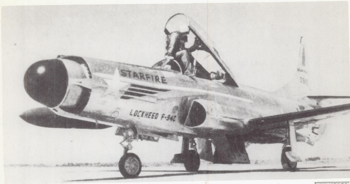
Figure 5. - Rocket installation for F-94C.
