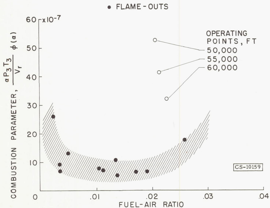
Figure 14. - Combustor flame-outs.
