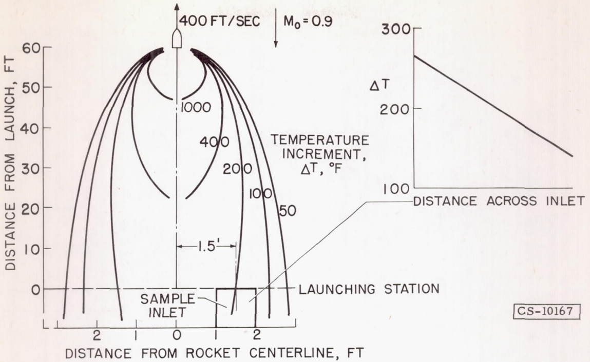
Figure 3. - Temperature contours for 2.75-inch rocket. Altitude 45,000 feet; time after firing, 0.3 second.
