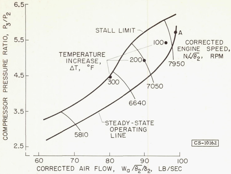
Figure 9. - Calculated effect of various inlet-temperature increases.
