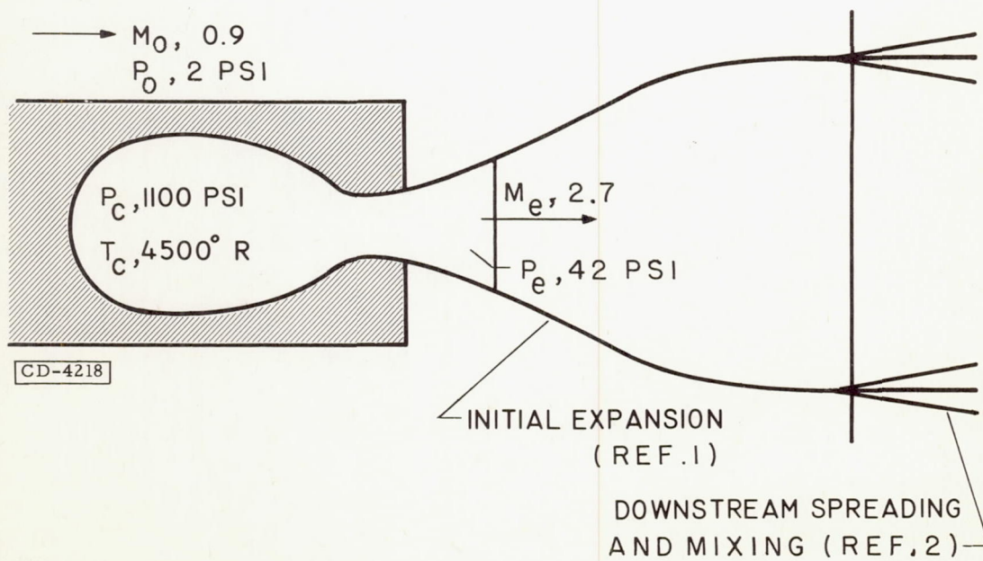
Figure 2. - Jet spreading from 2.75-inch rocket. Altitude, 45,000 feet.
