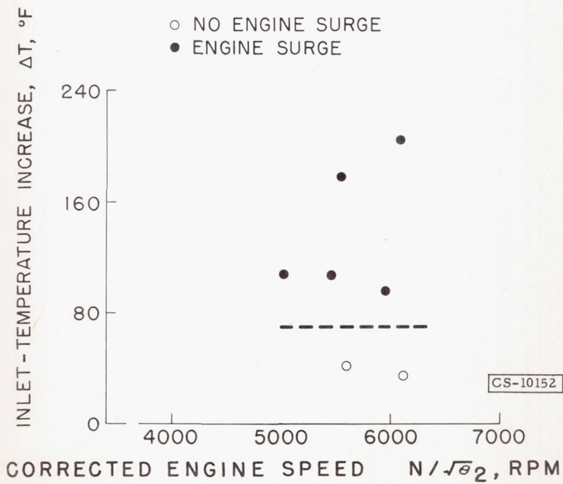
Figure 12. - Experimental effect of various inlet-temperature increases.
