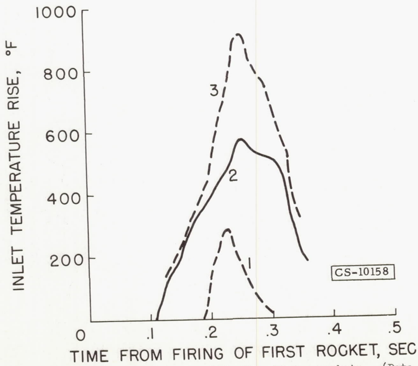
Figure 6. - Inlet temperatures for F-94C after firing rockets. (Data from ref. 3).
