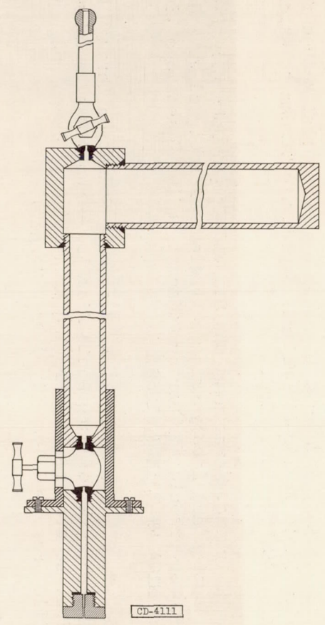
Figure 1. - Fuel injector, showing auxiliary remote-control opening equipment and helium line.
