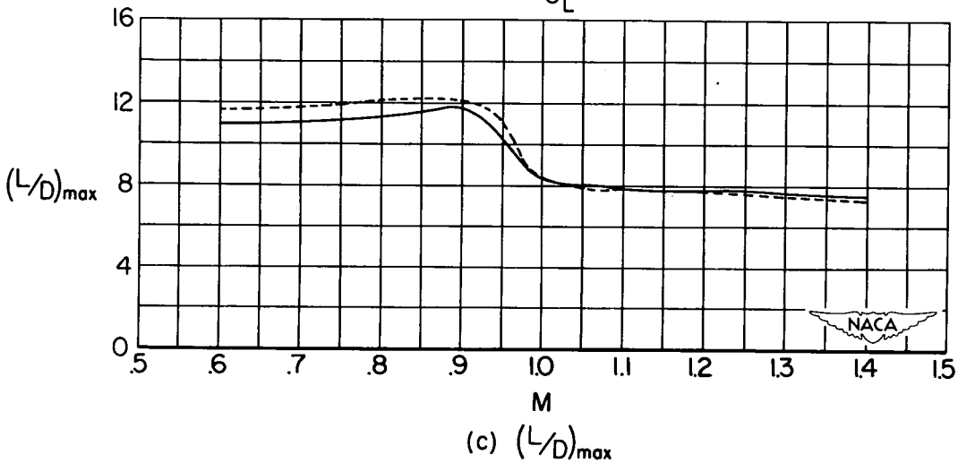
Figure 17.- The effect of taper ratio on the variation of minimum drag coefficient, drag-rise factor and maximum lift-drag ratio with Mach number for an unswept wing-body-tail combination.
