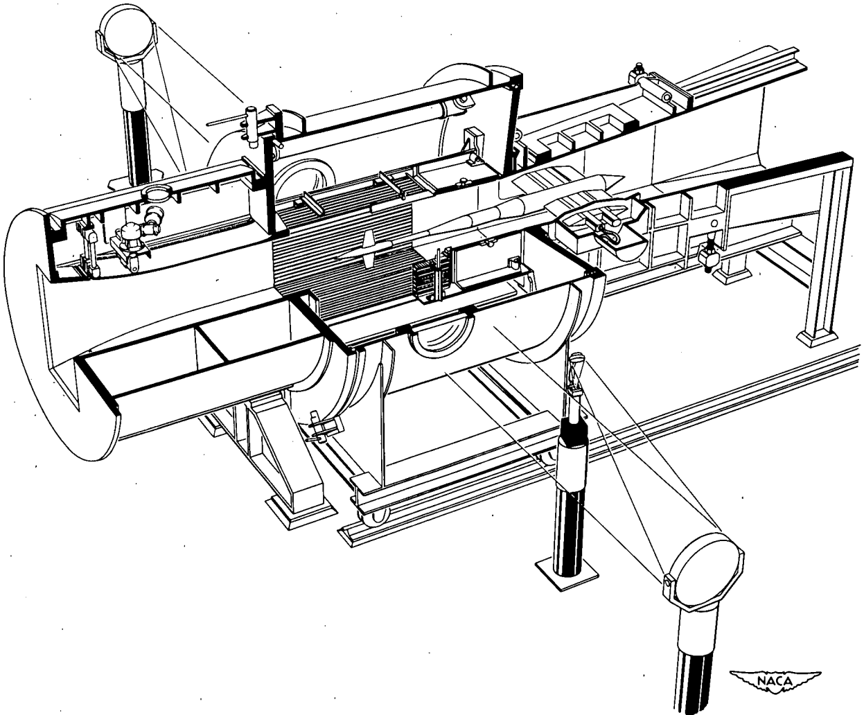
Figure 1.- Test section of the Ames 2-by 2-foot transonic wind tunnel.
