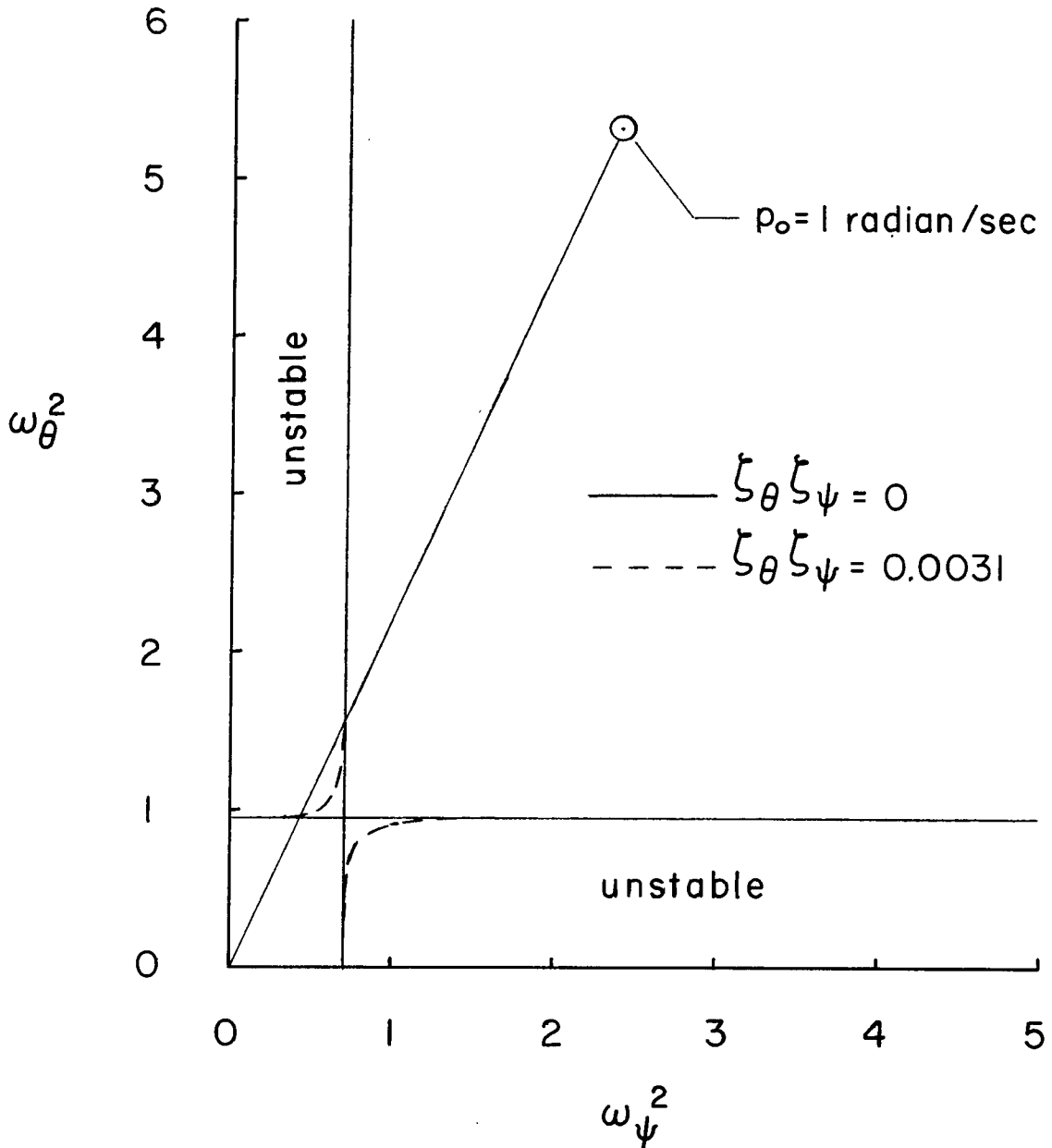
Figure 1.- Boundaries in the \omega_\psi^2, \omega_\theta^2 plane which define regions of aperiodic divergence for example aircraft. I_{X_e} \omega_e = 0 .
