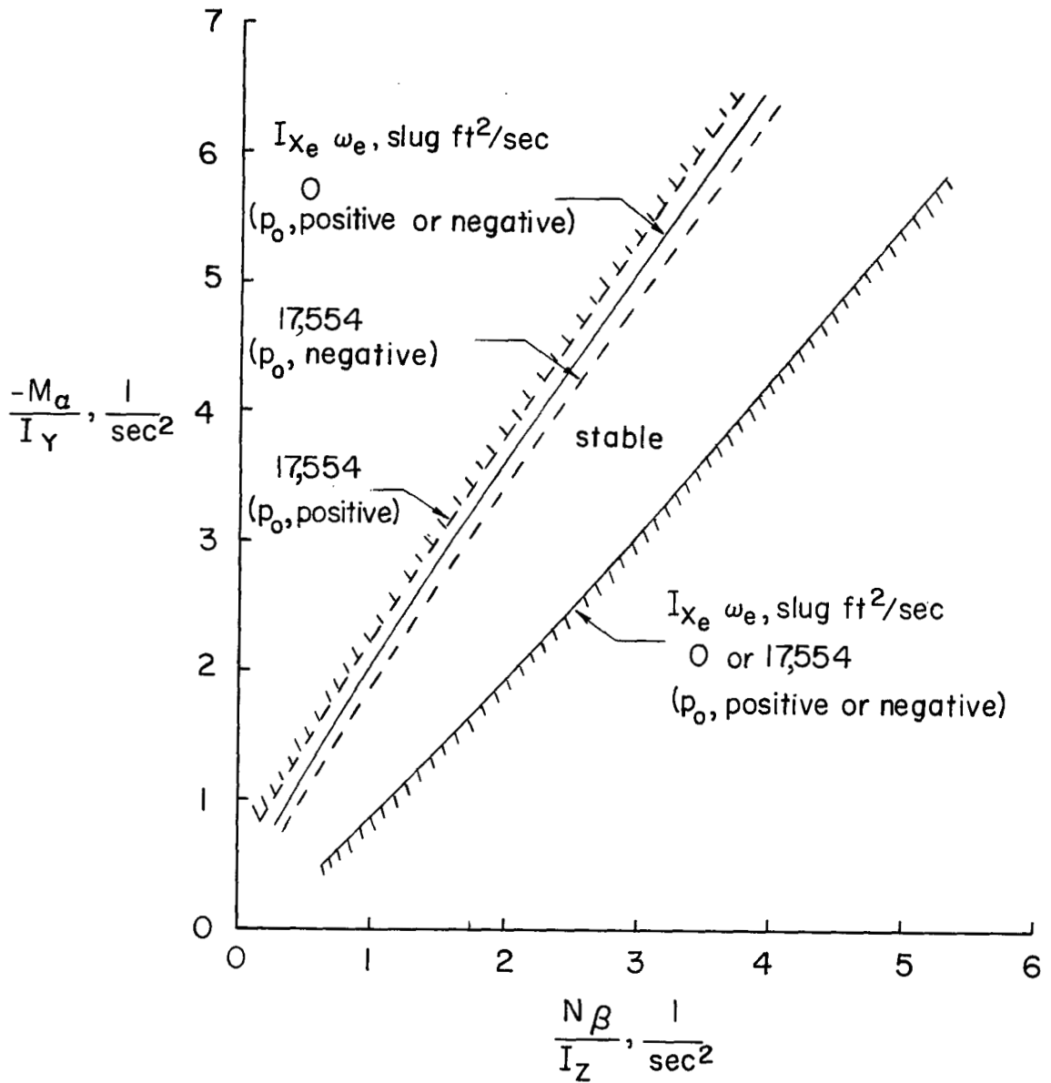
Figure 5.- Envelopes of divergence boundaries presented in figures 2 and 3.
