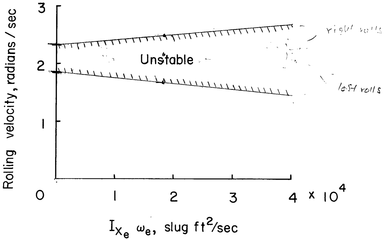
Figure 4.- Effect of engine momentum I_{X_e} \omega_e on rolling-velocity range for which example aircraft is unstable.
