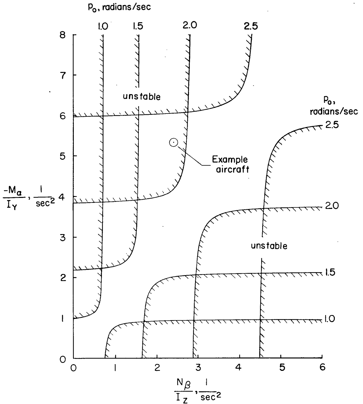
Figure 2.- Boundaries in the N_\beta/I_Z, M_\alpha/I_Y plane for example aircraft which define regions of aperiodic divergence as a function of rolling velocity. I_{X_e}\omega_e = 0 .
