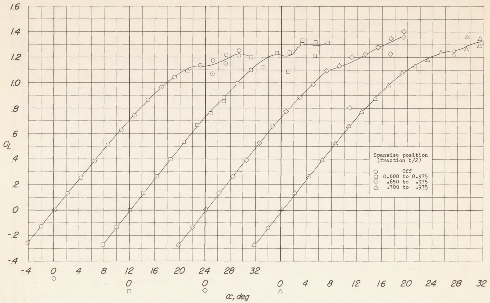
(c) C_L against \alpha .
