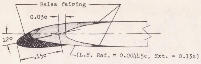
Drooped (L.E. Rad. = 0.00890c, Ext. = 0.18c)
