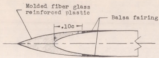
Undrooped (L.E. Rad. = 0, Ext. = 0.13c)
