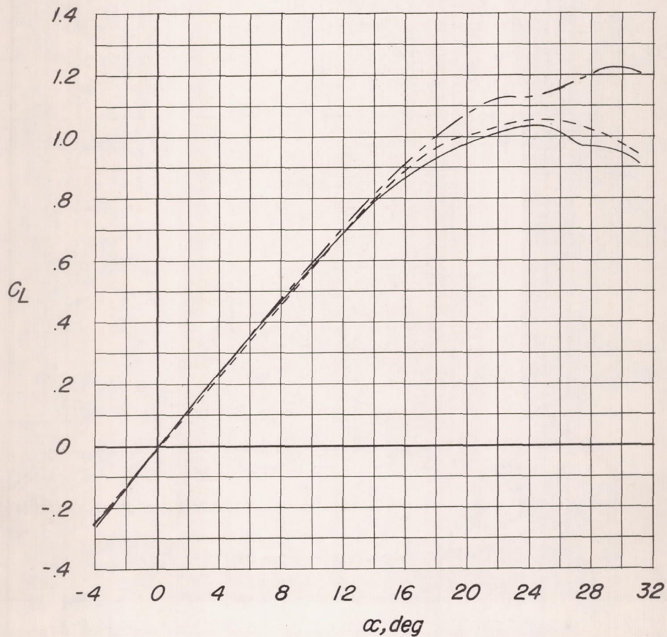
Figure 4.- Lift and pitching-moment characteristics of the basic wing.
