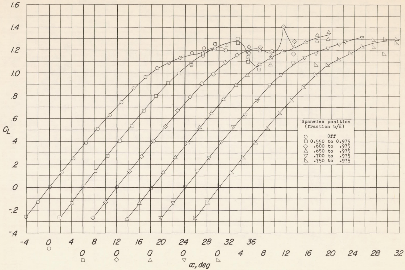
(c) C_L against \alpha .
