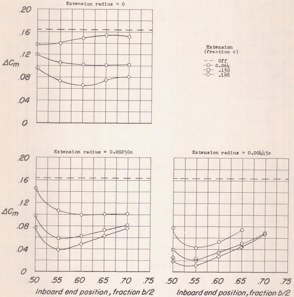
(b) 0.0050c-leading-edge-radius wing.
