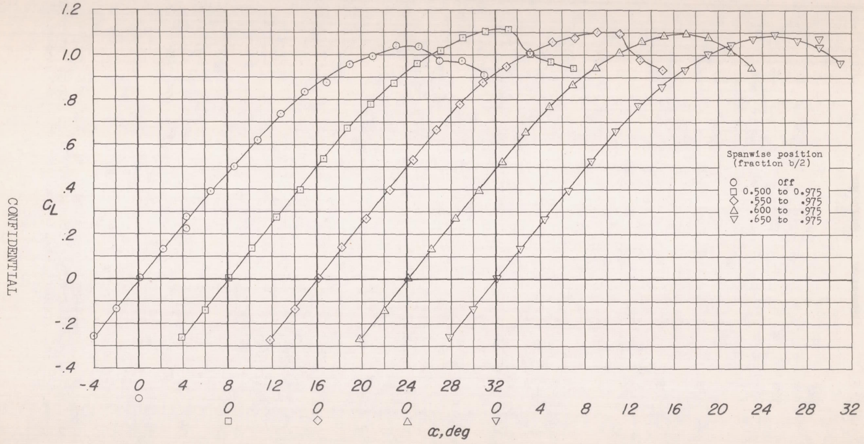
(c) C_L against \alpha .
