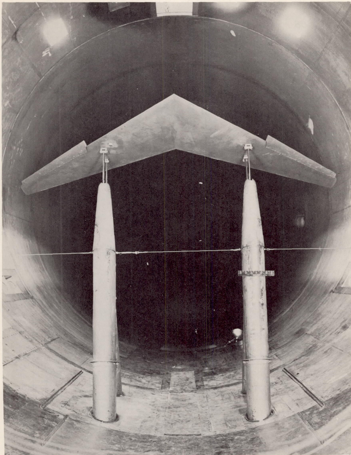
Figure 3.- A 45^\circ sweptback, aspect ratio 5 wing equipped with leading-edge chord-extensions mounted in the Langley 19-foot pressure tunnel.
