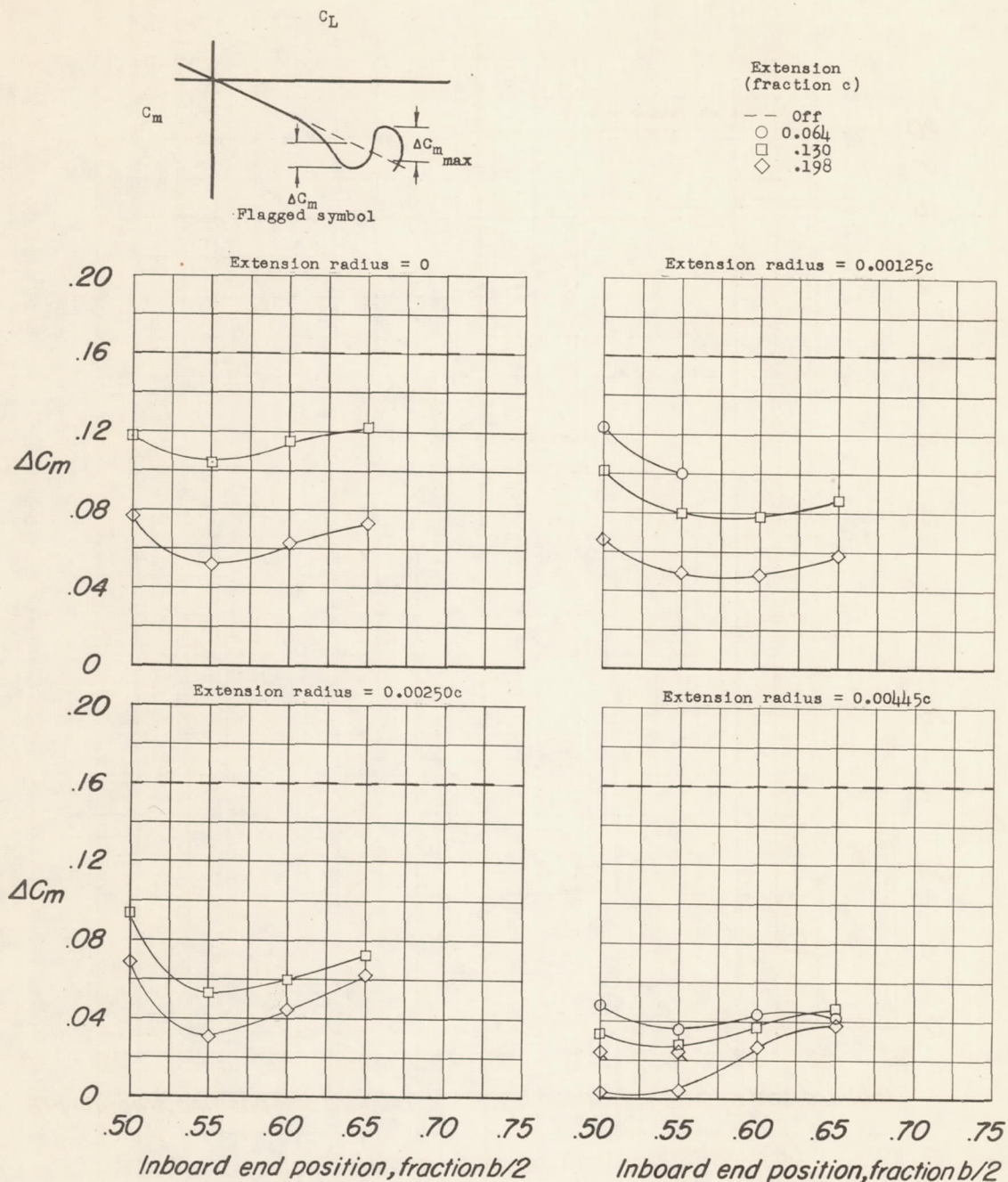
(a) 0.0025c-leading-edge-radius wing.
