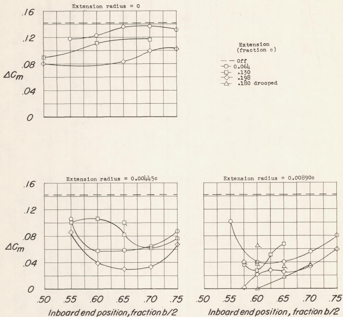
(c) 0.0089c-leading-edge-radius wing.
