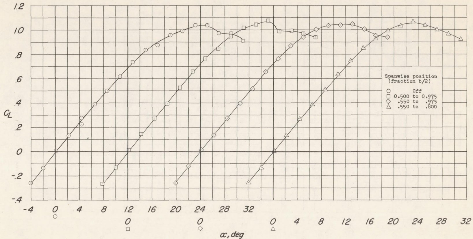
(c) C L against α.
