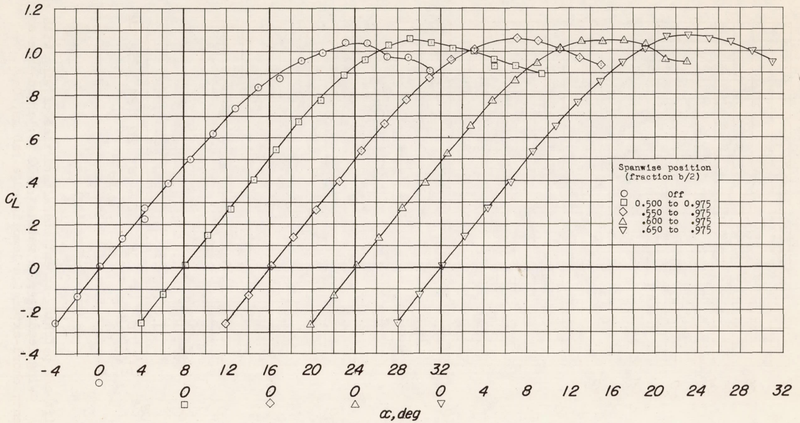
(c) C L against α.
