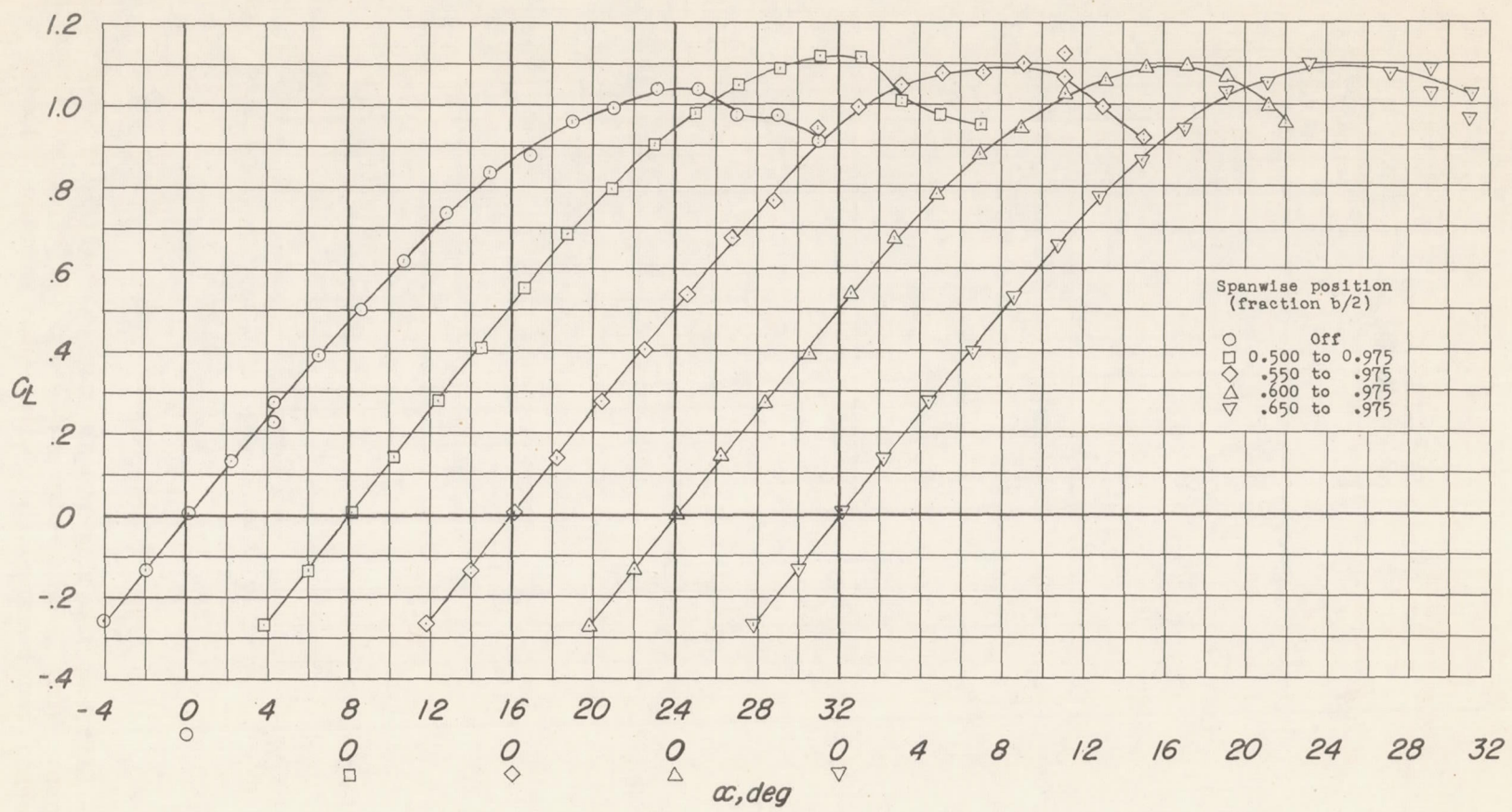
(c) C L against α.
