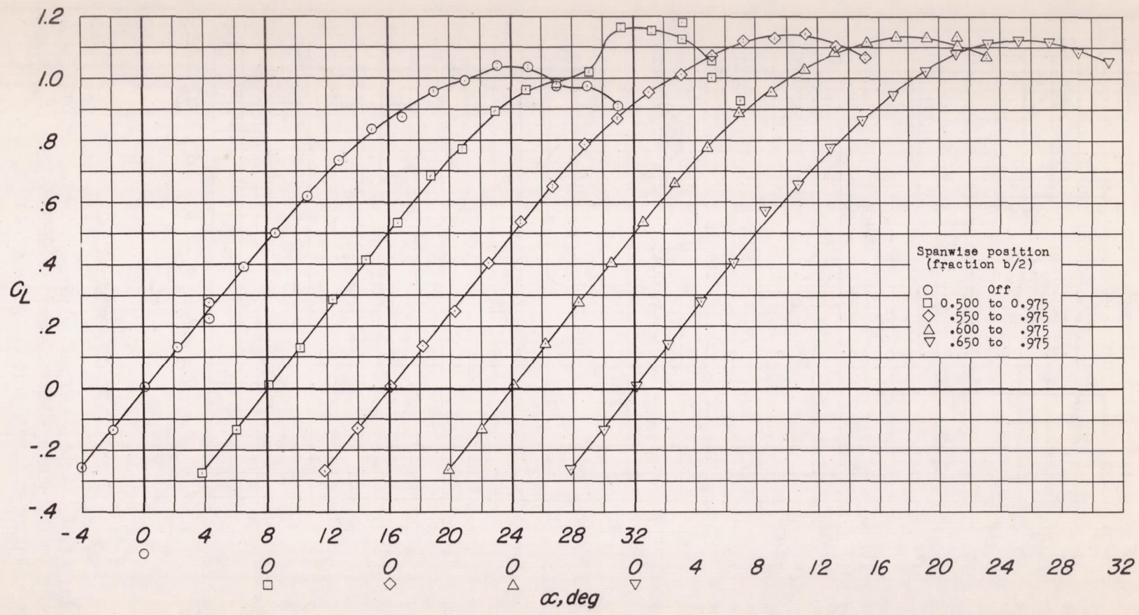
(c) C L against α.
