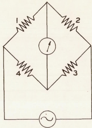
(b) Bridge formed by connecting gages to strain indicator.
