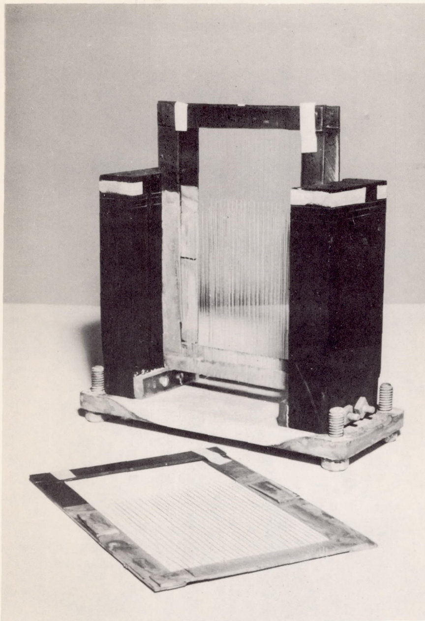
Figure 11.- Winding frames and holder for copper plating gage lead wires. L-92486
