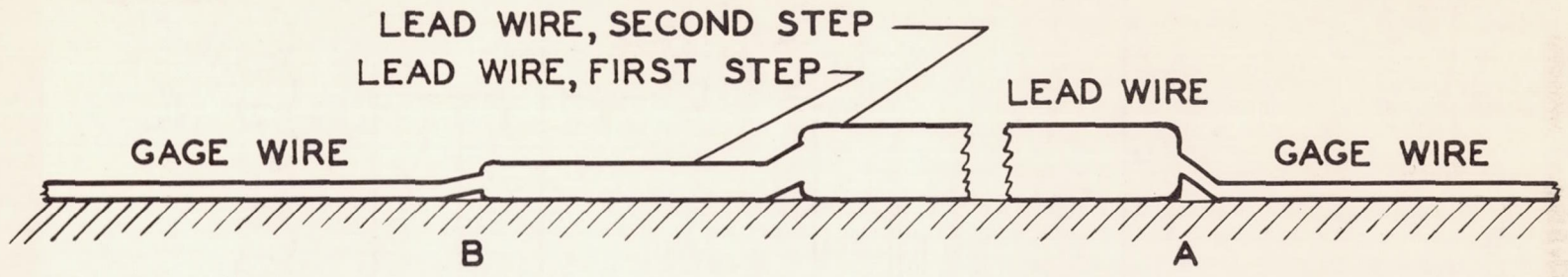
Figure 13.- Schematic representation of lead wire junction with gage wire. A, single-step arrangement, not recommended; B, two-step arrangement, recommended.
