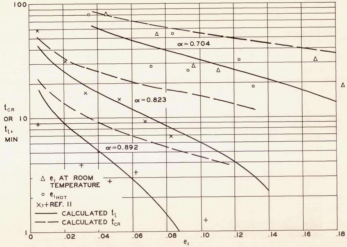
Figure 5.- Variation of critical time with initial deviation from straightness.
