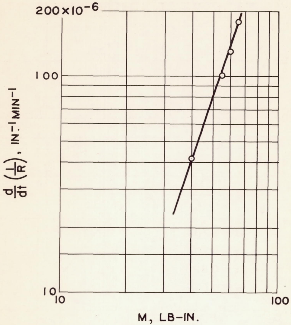
Figure 9.- Variation of steady creep rate of curvature with bending moment.
