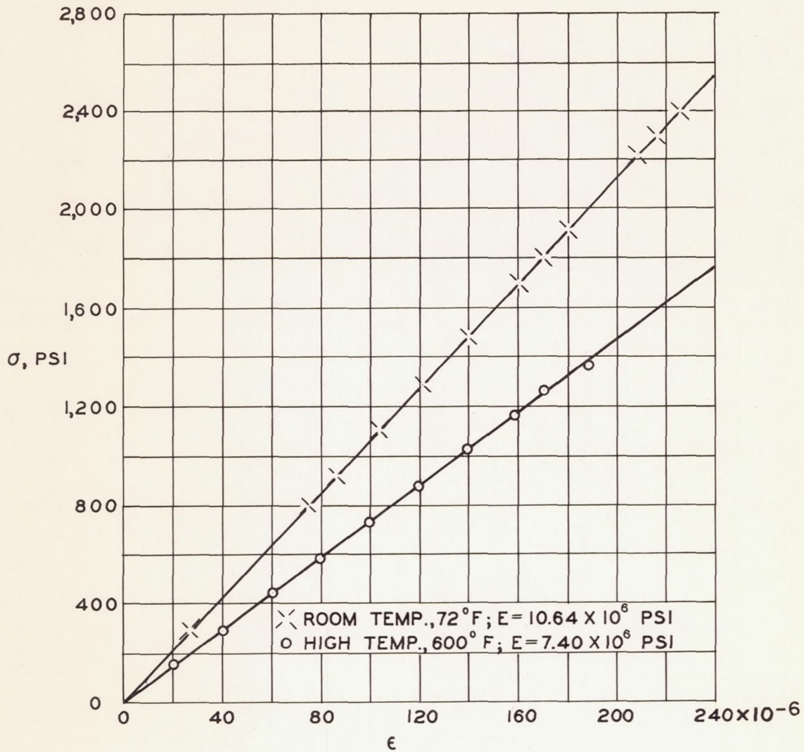
Figure 15.- Experimental stress-strain curve for 2024-T4 aluminum-alloy column (1/2 inch by 1/4 inch by 12 inches).
