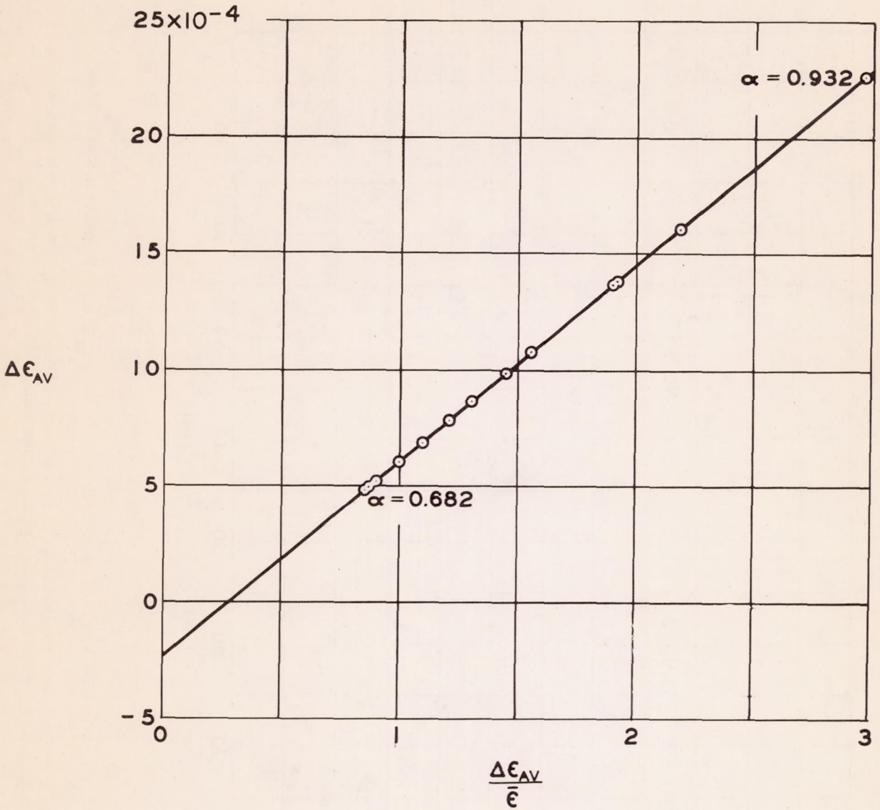
Figure 3.- Plot used in determination of \epsilon_E and e_1 . Column 3; \epsilon_E = 845 \times 10^{-6} ; e_1 = 0.096 .
