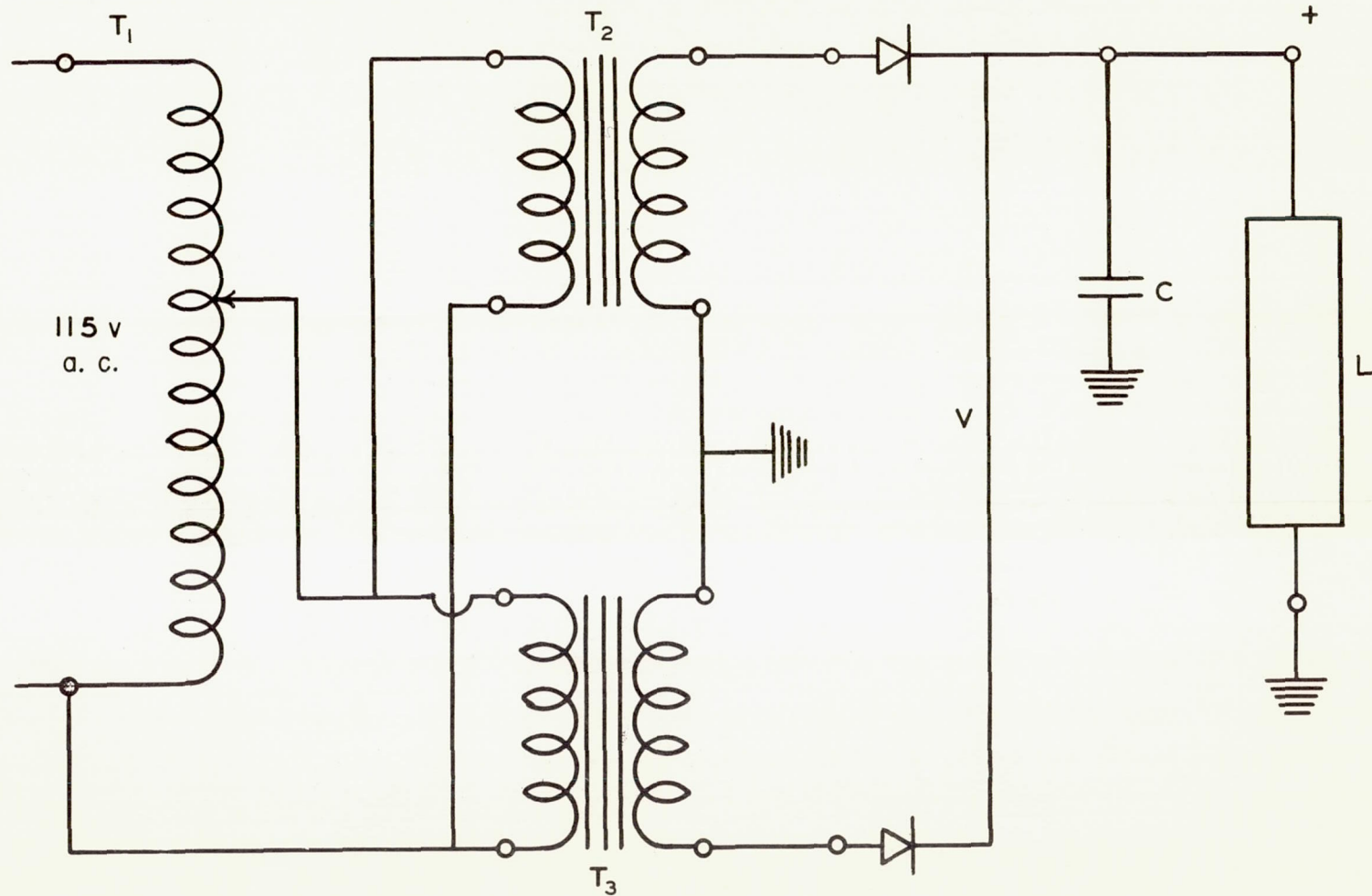
Figure 14.- Diagram of plating circuit. T 1 , variac; T 2 and T 3 , transformers; V, rectifier; C, condenser; L, load.
