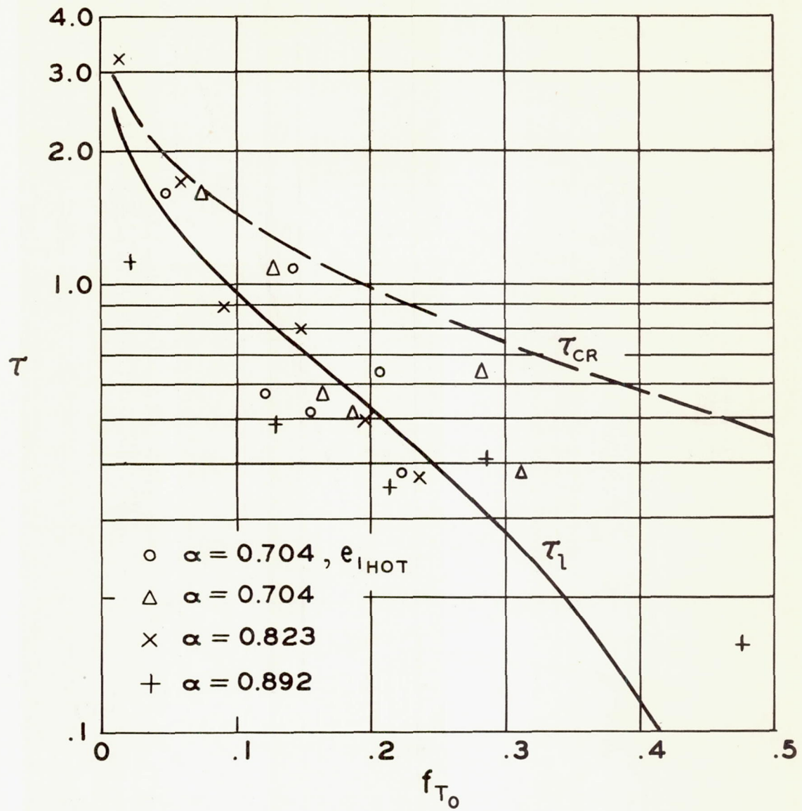
Figure 10.- Variation of experimental and calculated critical-time parameters with f_{T_0} .
