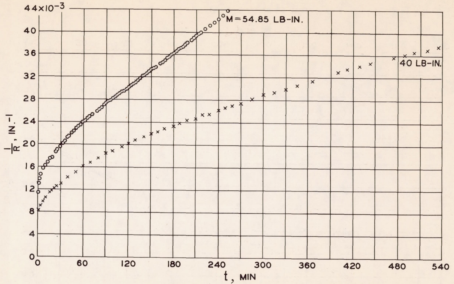
(a) M = 40 and 54.85 lb-in.
