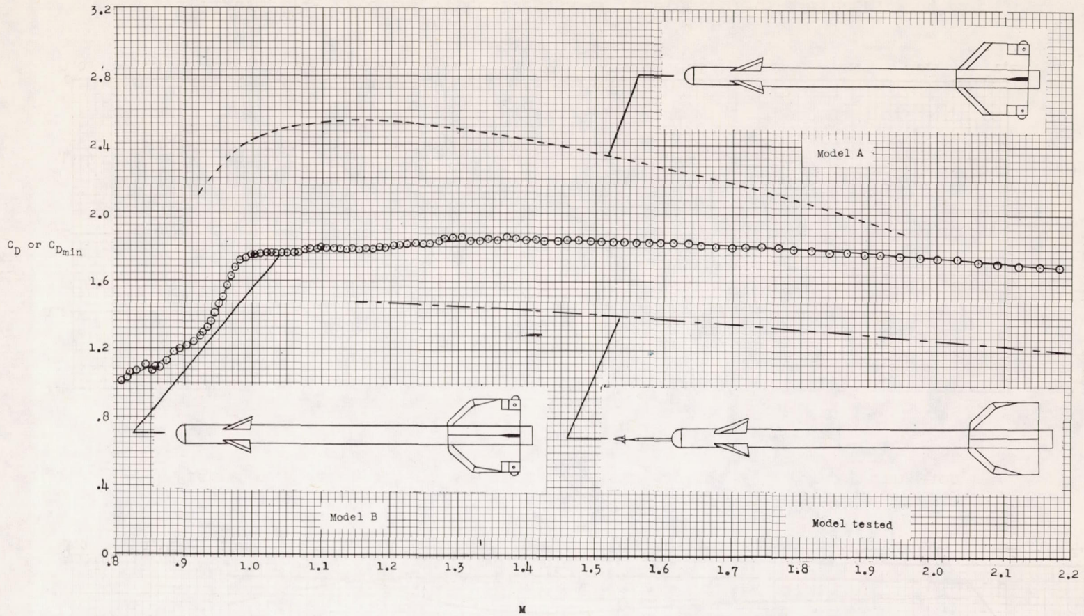
Figure 18.- Variation of the drag coefficient with Mach number of two similar models (from unpublished data) and the model tested.
