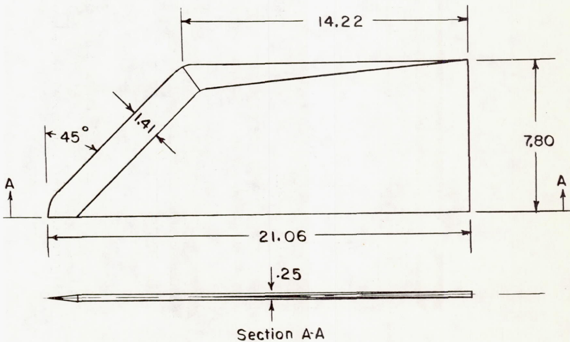
Figure 2.- Sketch of control surface and wing surface for model tested. All dimensions are in inches.
