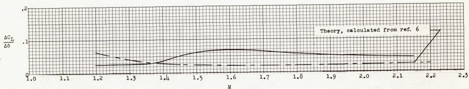
Figure 16.- Variation of the lift per unit control deflection with Mach number.
