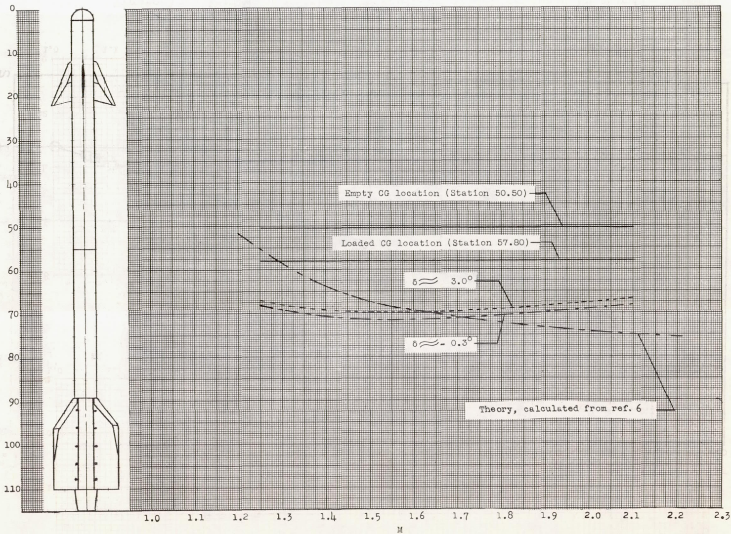
Figure 13.- Variation of the aerodynamic-center location with Mach number.
