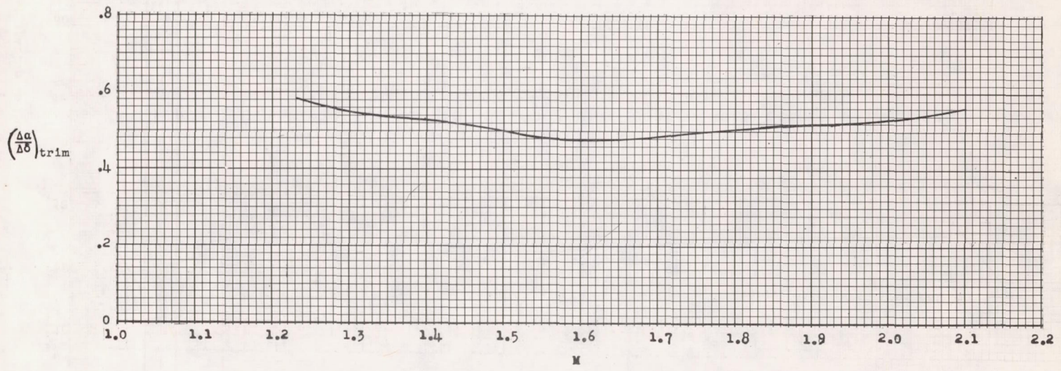
Figure 15.- Variation of the trim angle of attack produced by a unit control deflection with Mach number.
