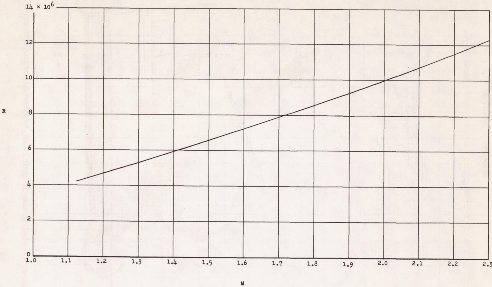
Figure 5.- Variation of Reynolds number, per foot, with Mach number.
