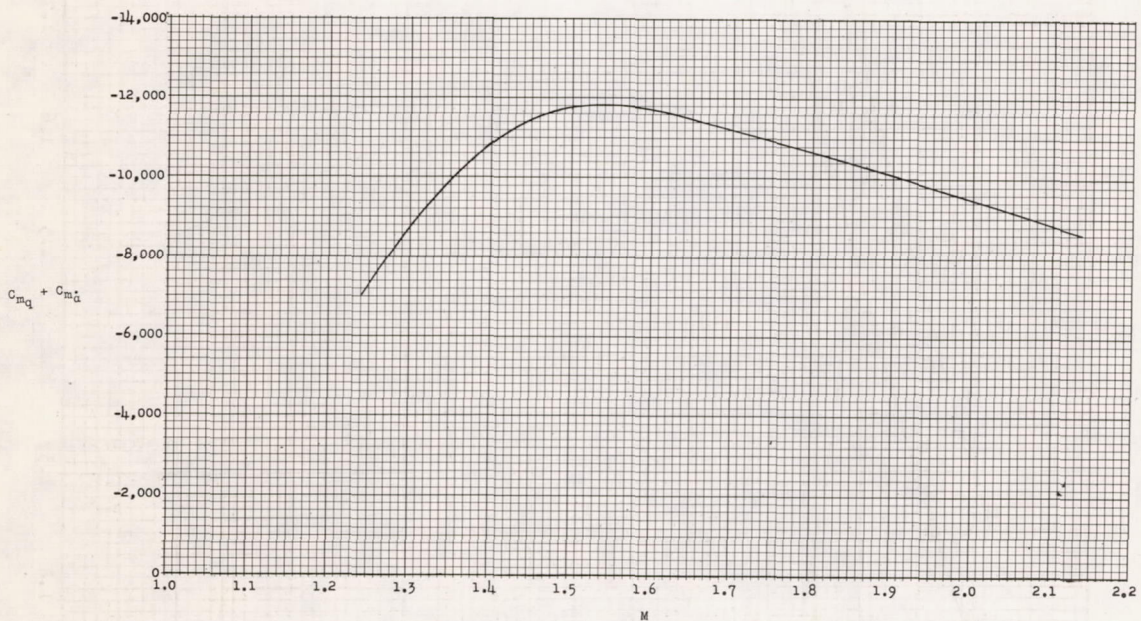
Figure 9.- Variation of the aerodynamic damping-in-pitch derivative C_{m_q} + C_{m_{\dot{\alpha}}} with Mach number.
