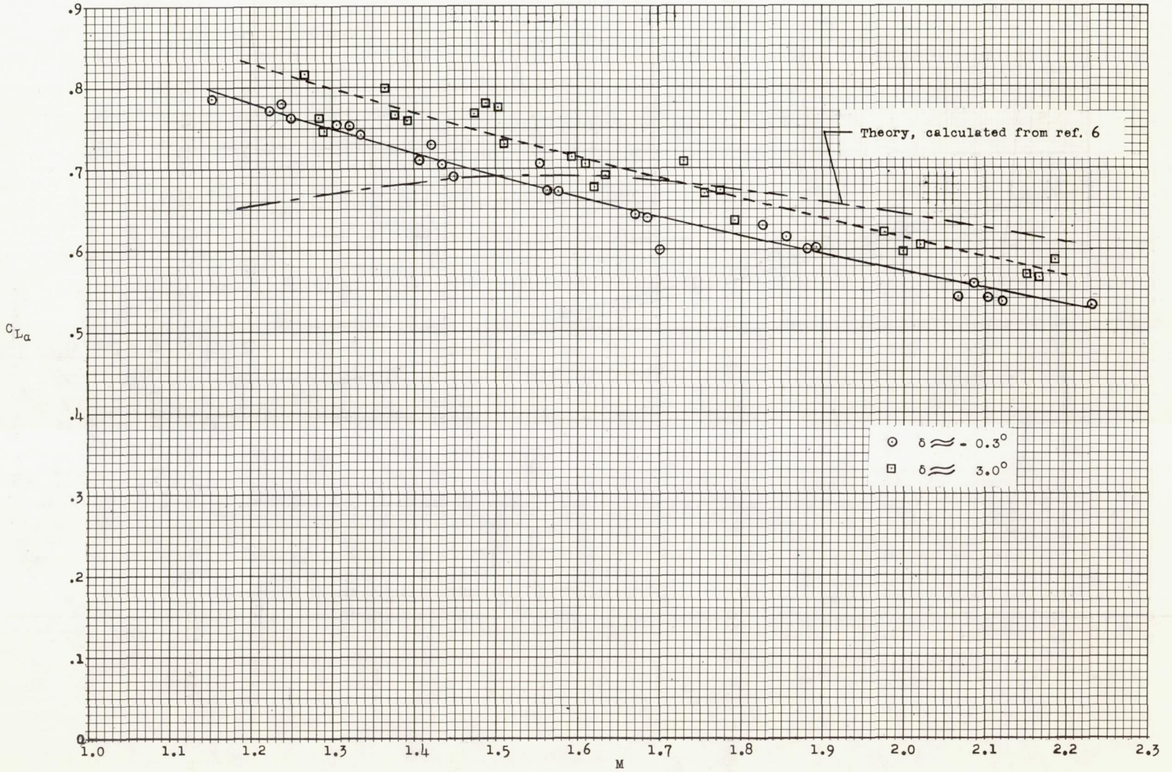
Figure 7.- Variation of average lift-curve slope with Mach number.
