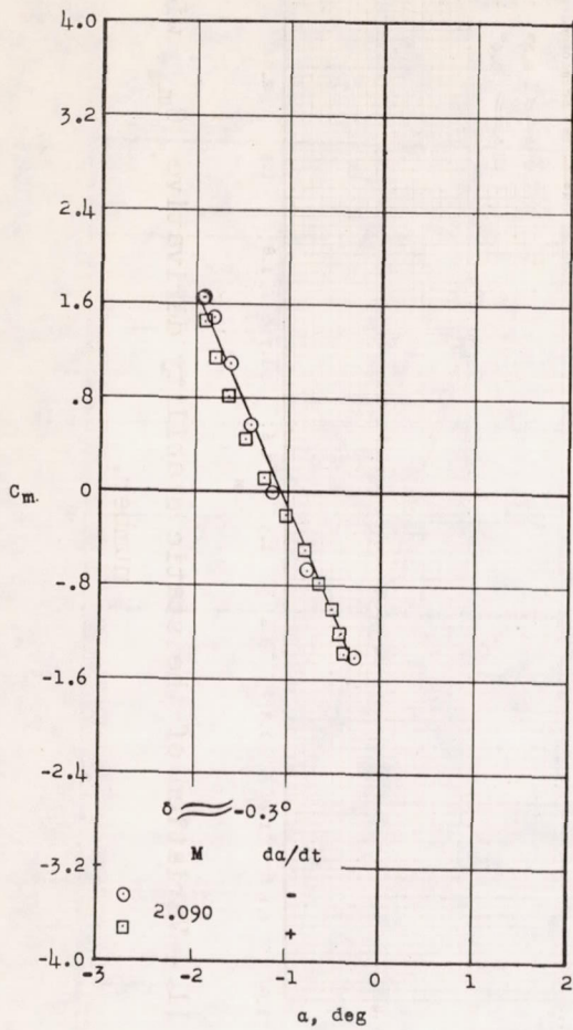
Figure 12.- Variation of pitching-moment coefficient with angle of attack.
