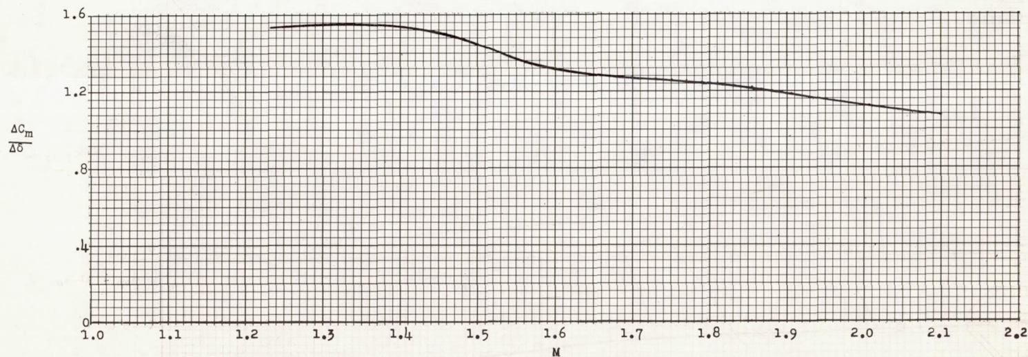
Figure 17.- Pitching effectiveness of canard control surfaces.
