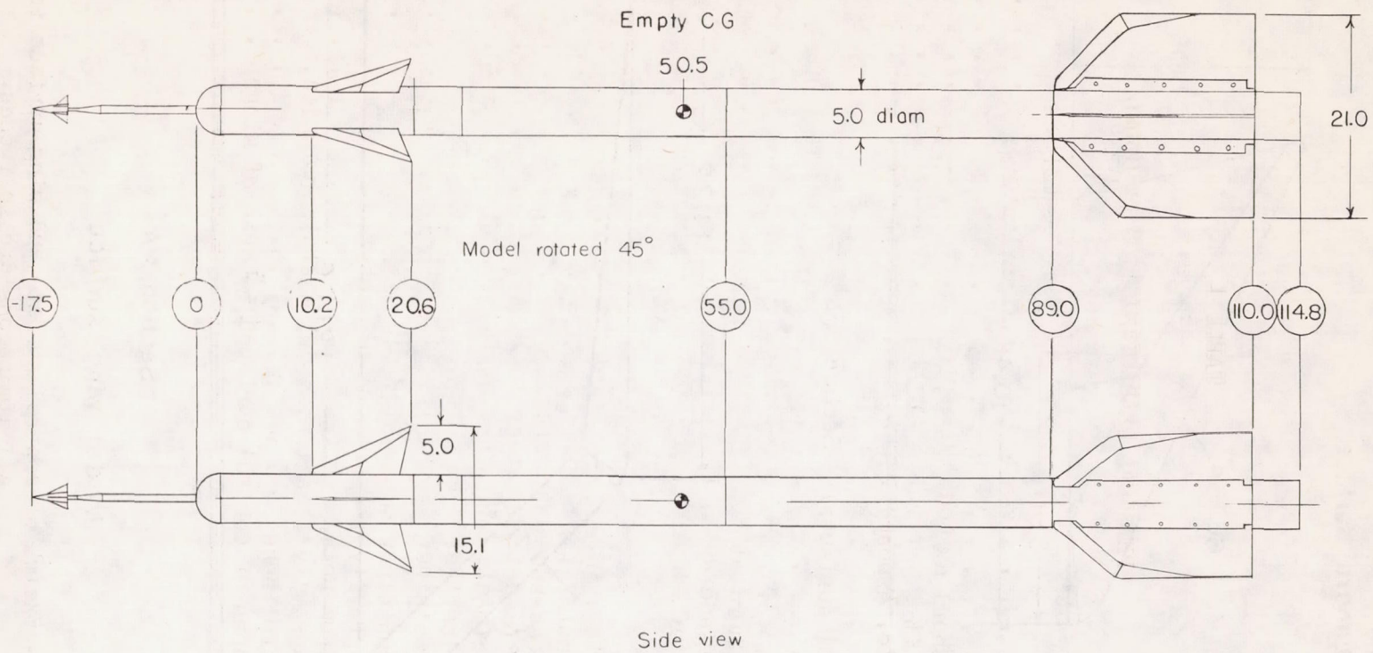
Figure 1.- Sketch of model tested. All dimensions are in inches.
