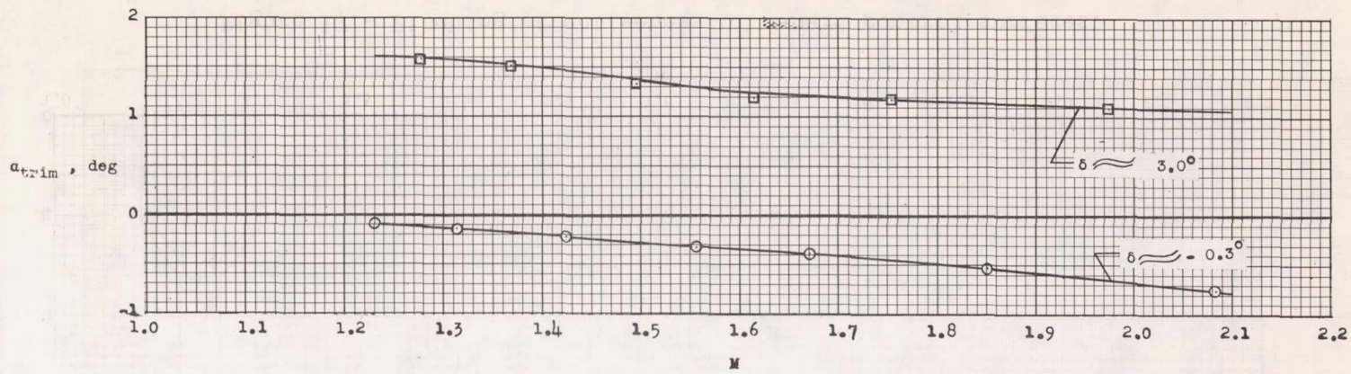
Figure 14.- Variation of trim angle of attack with Mach number.
