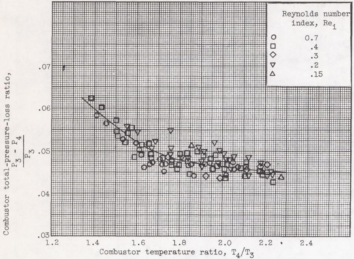
Figure 10. - Variation of combustor total-pressure-loss ratio with combustor temperature ratio.
