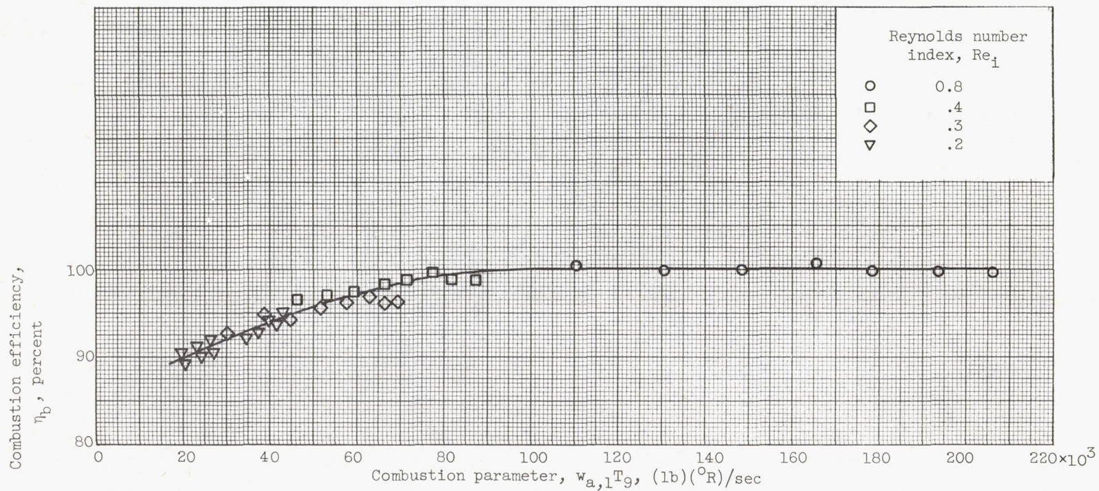
Figure 9. - Variation of combustion efficiency with combustion parameter. Fixed exhaust-nozzle area, 3.01 square feet.
