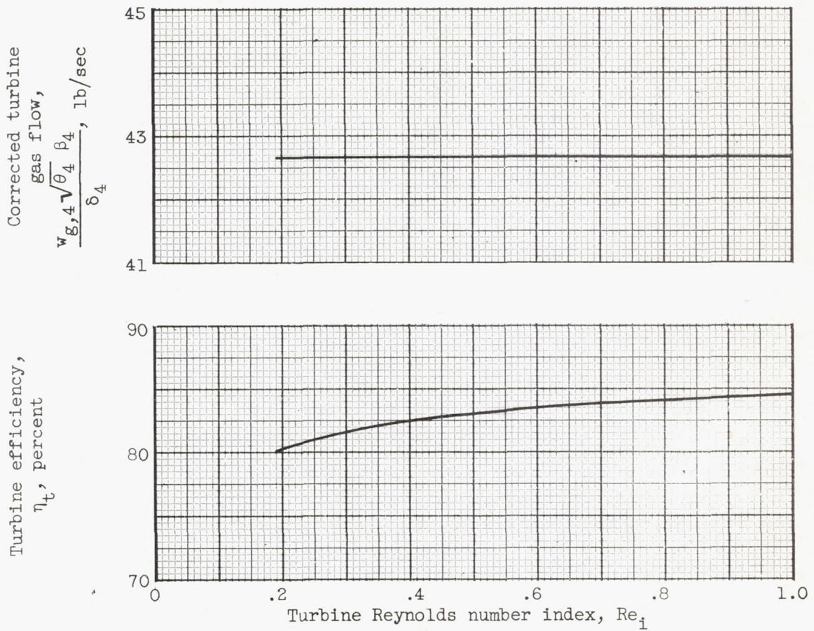
Figure 13. - Effect of turbine Reynolds number index on corrected turbine gas flow and turbine efficiency.
