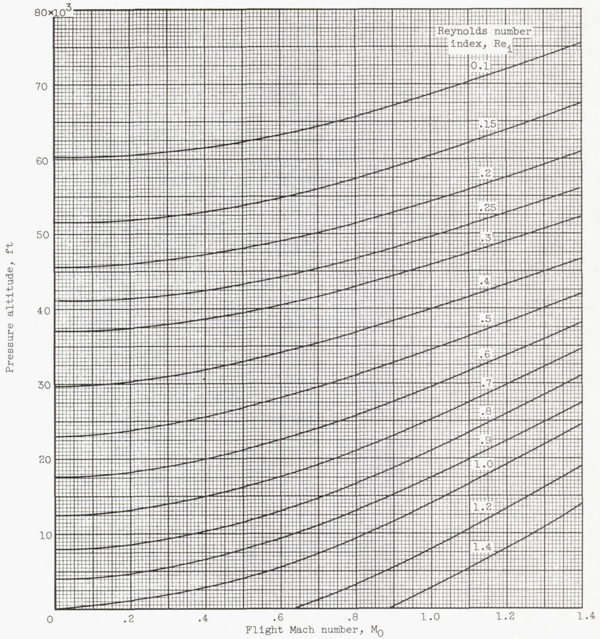
Figure 3. - Variation of Reynolds number index with altitude and flight Mach number. NACA standard atmosphere; 100-percent ram-pressure recovery assumed.
