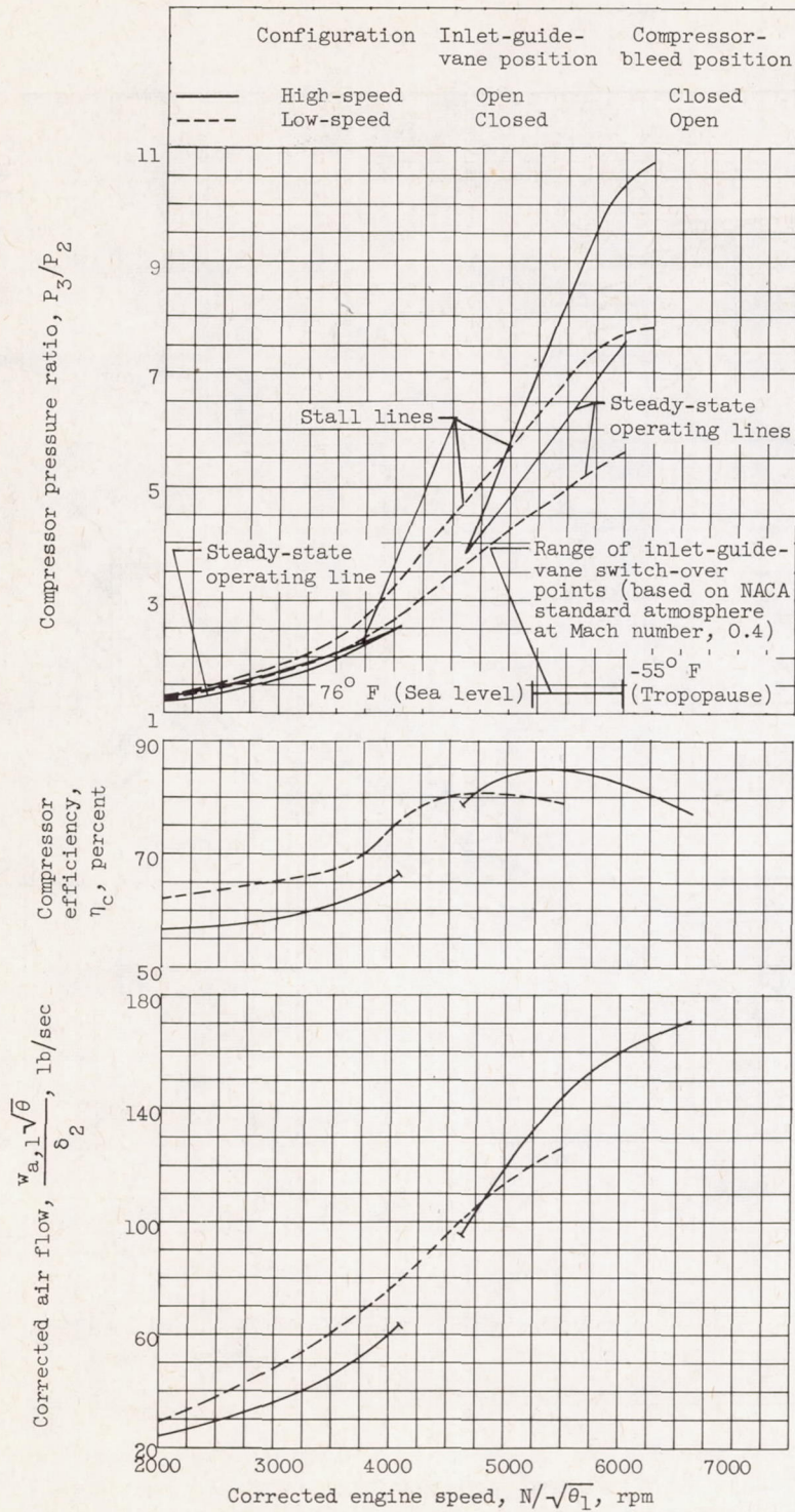
Figure 5. - Effect of interstage bleeds and inlet-guide-vane position on steady-state air flow and compressor efficiency. Exhaust nozzle open; altitude, 35,000 feet; Mach number, 0.4; inlet temperature, -30^\circ\text{F} .
