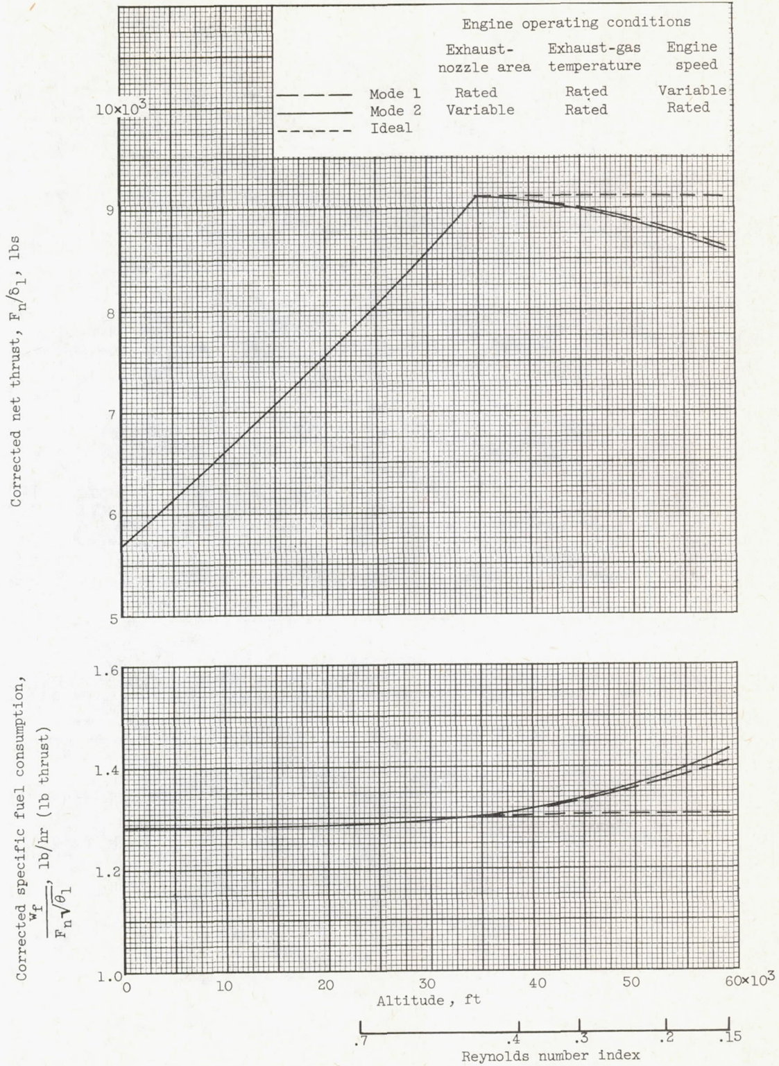
Figure 15. - Effect of altitude on corrected net thrust and corrected specific fuel consumption. Mach number, 0.9.
