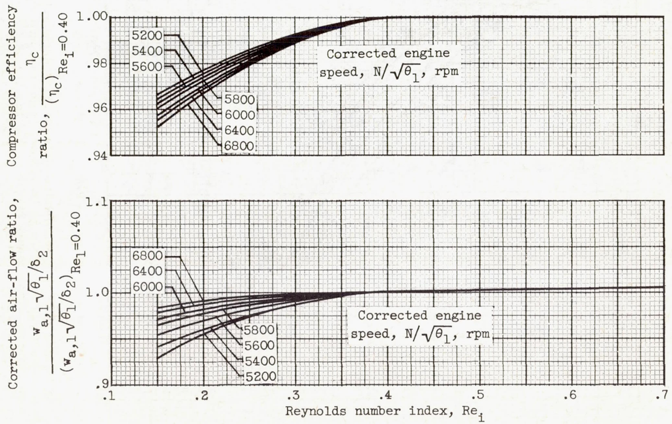
Figure 7. - Effect of Reynolds number index on compressor efficiency and corrected air flow. Inlet guide vanes open; compressor acceleration bleeds closed; exhaust-nozzle area, 3.01 square feet.
