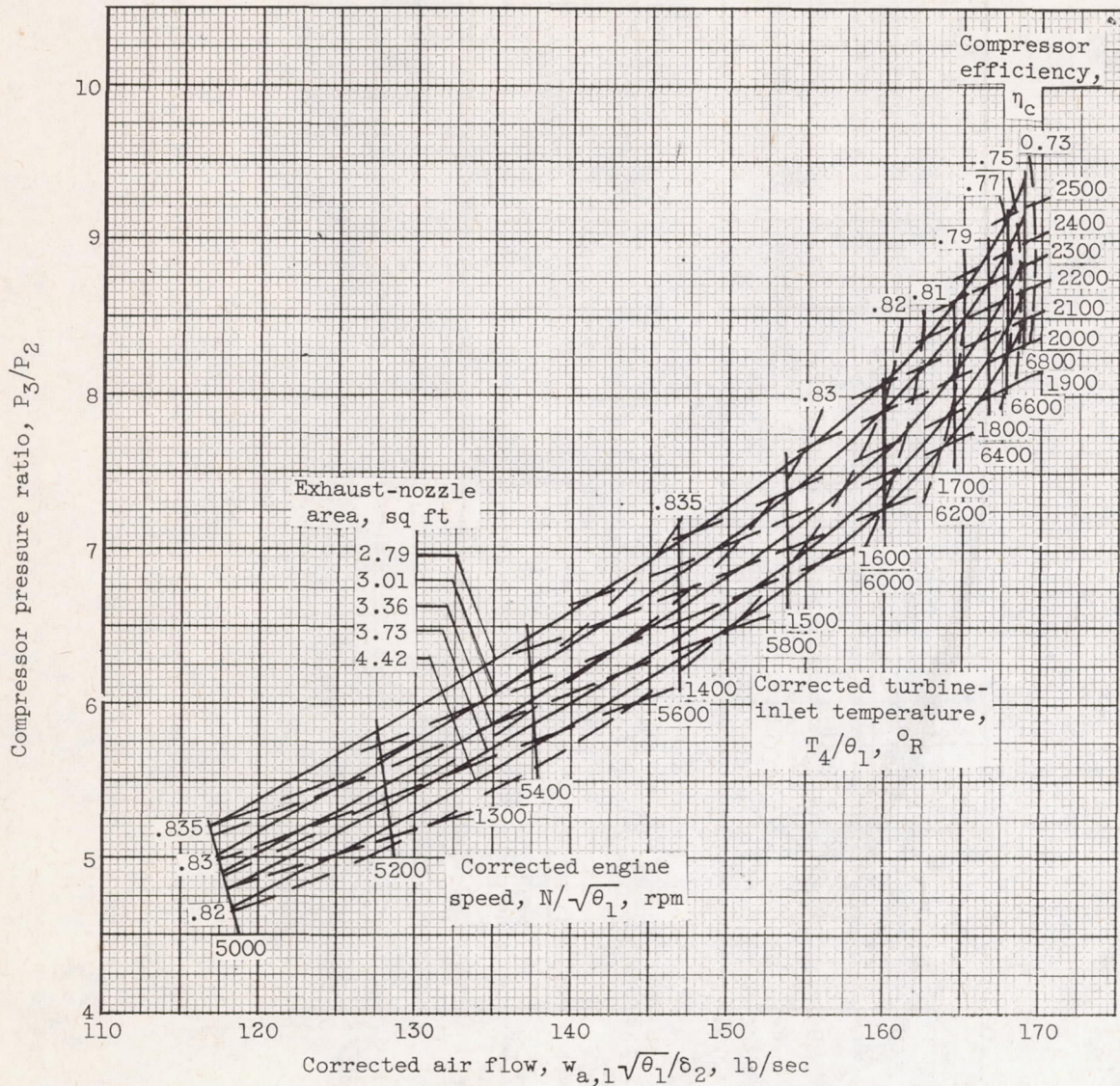
Figure 8. - Compressor performance map showing lines of constant corrected turbine-inlet temperature. Inlet guide vanes open; compressor acceleration bleeds closed; Reynolds number index, 0.4.
