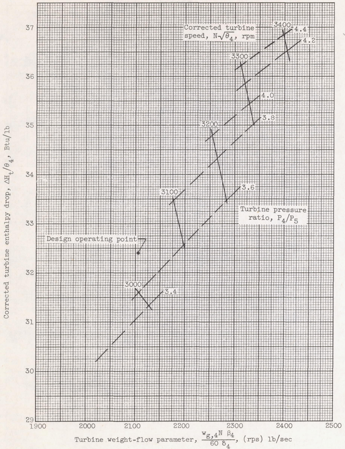
Figure 12. - Turbine performance map for Reynolds number index of 0.4.
