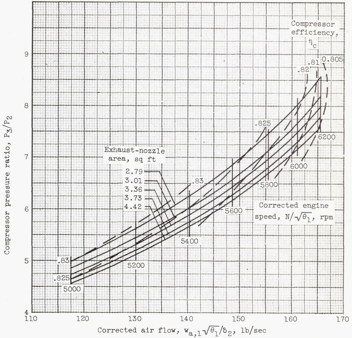
Figure 6. - Compressor performance map for high-speed configuration (inlet guide vanes open; compressor acceleration bleeds closed).
