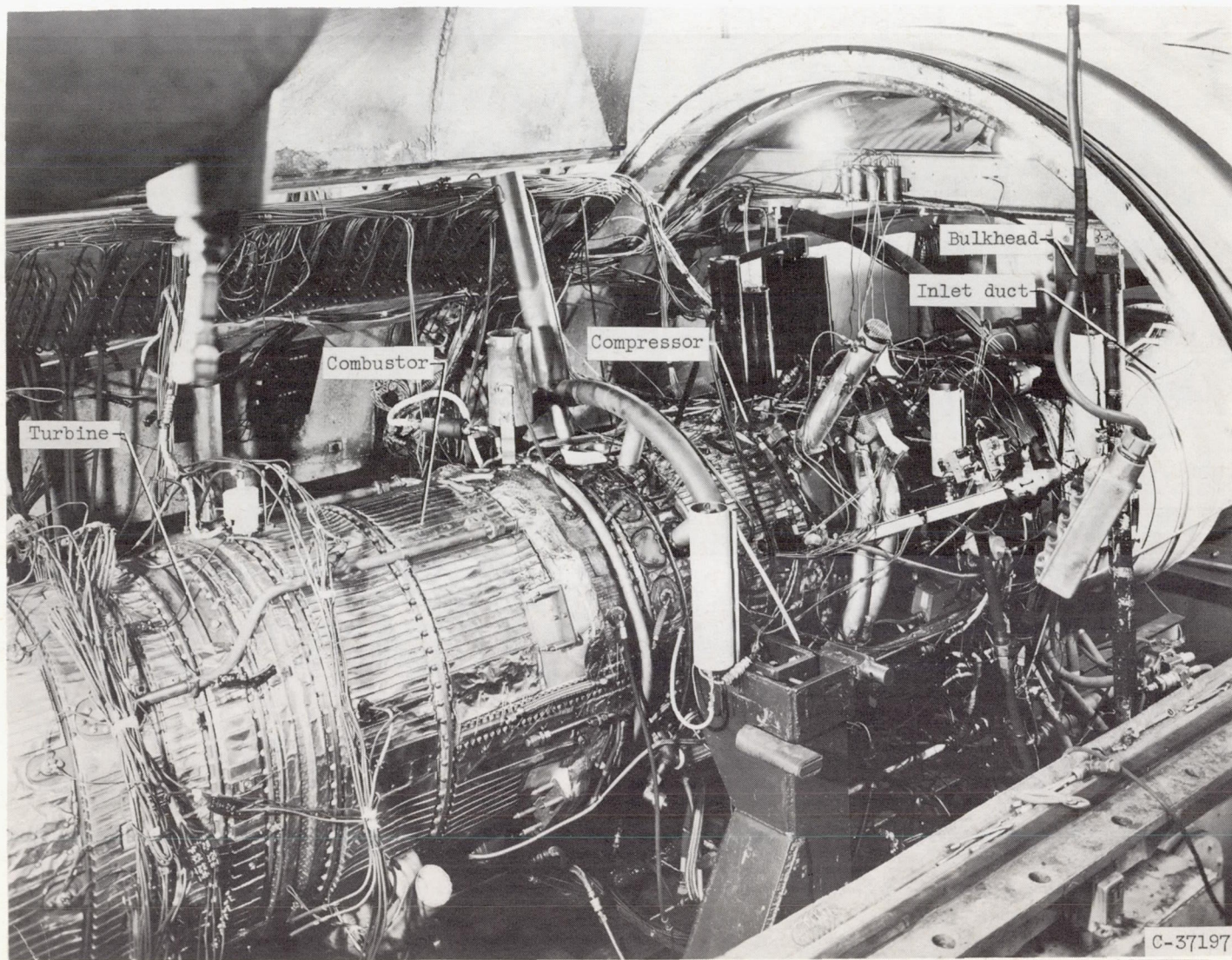
Figure 1. - Installation of J71-A-2(600-D1) turbojet engine in altitude test chamber.
