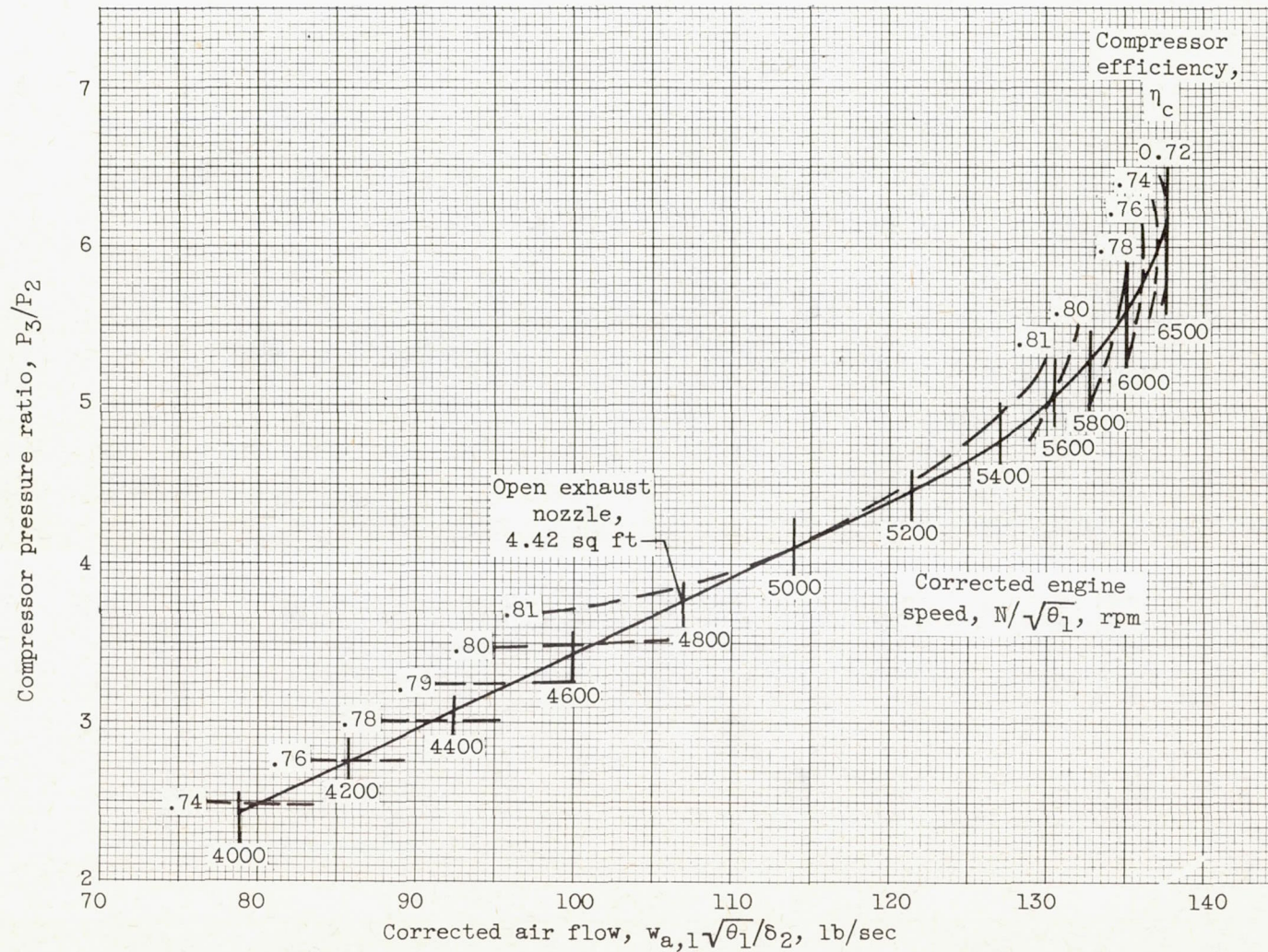
Figure 4. - Concluded. Compressor performance map. Reynolds number index, 0.4.
