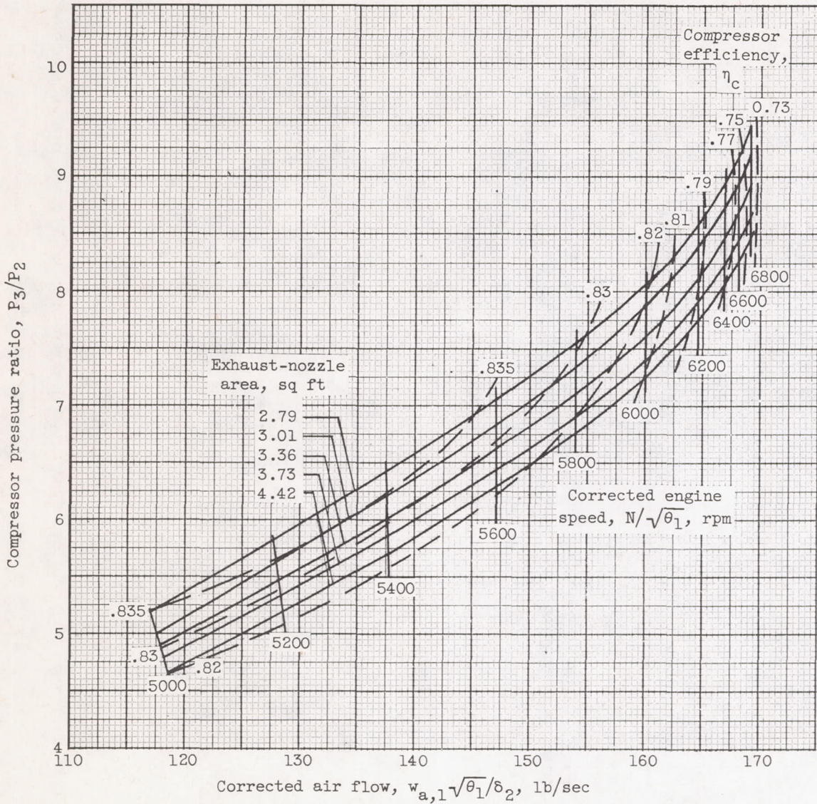
(a) High-speed configuration. Inlet guide vanes open; compressor acceleration bleeds closed.
