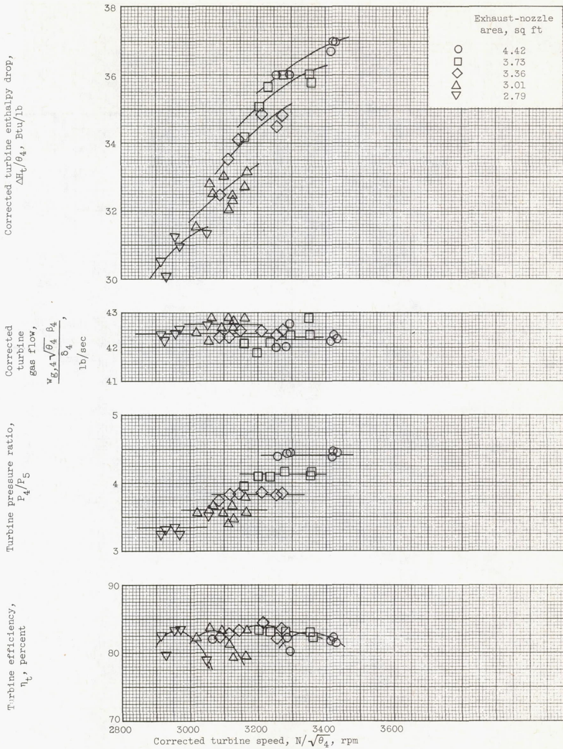
Figure 11. - Variation of turbine performance parameters with exhaust-nozzle area and corrected turbine speed.
