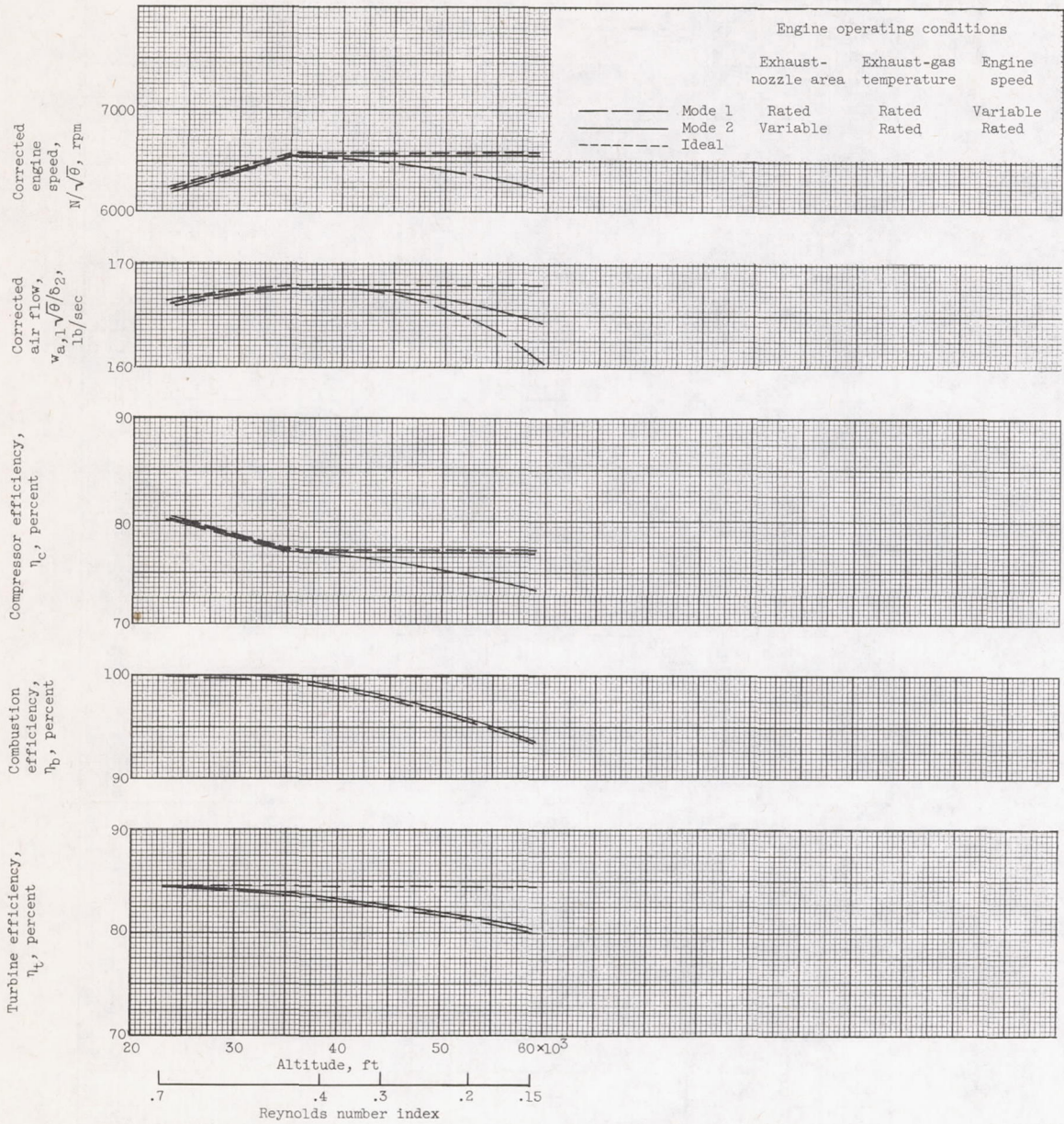
Figure 14. - Effect of altitude on corrected engine speed, corrected air flow, and compressor, combustion, and turbine efficiency. Mach number, 0.9.
