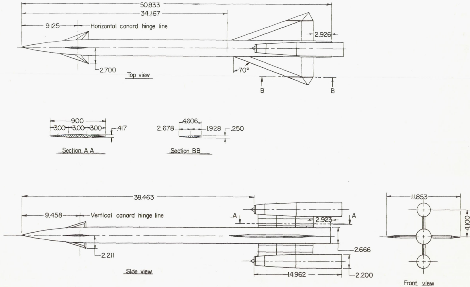
(a) General arrangement of model.
