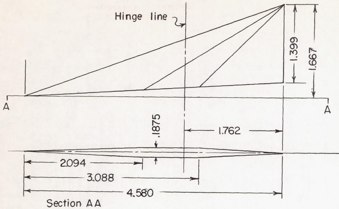
Horizontal canard
