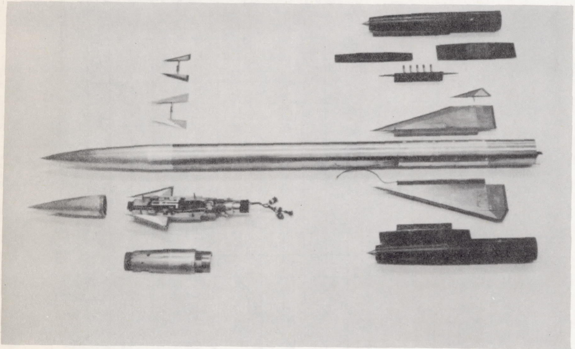
Figure 3.- Photograph of the model. L-74957
