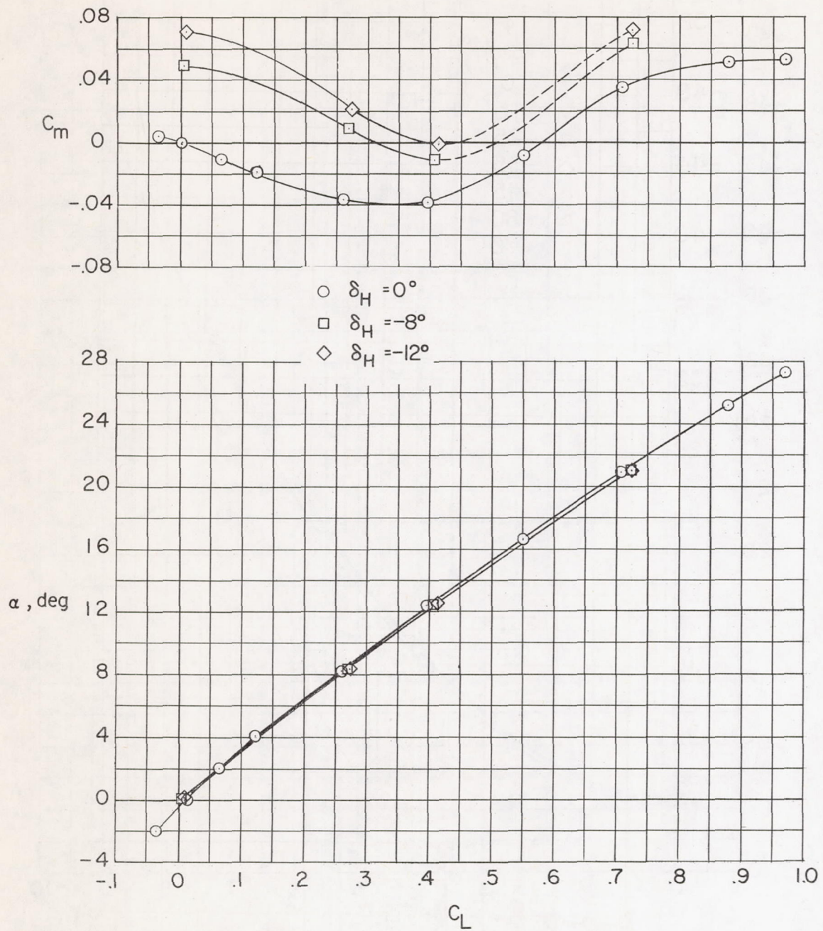
Figure 14.- Aerodynamic characteristics in pitch for several constant control deflections; \beta = 0^\circ .
