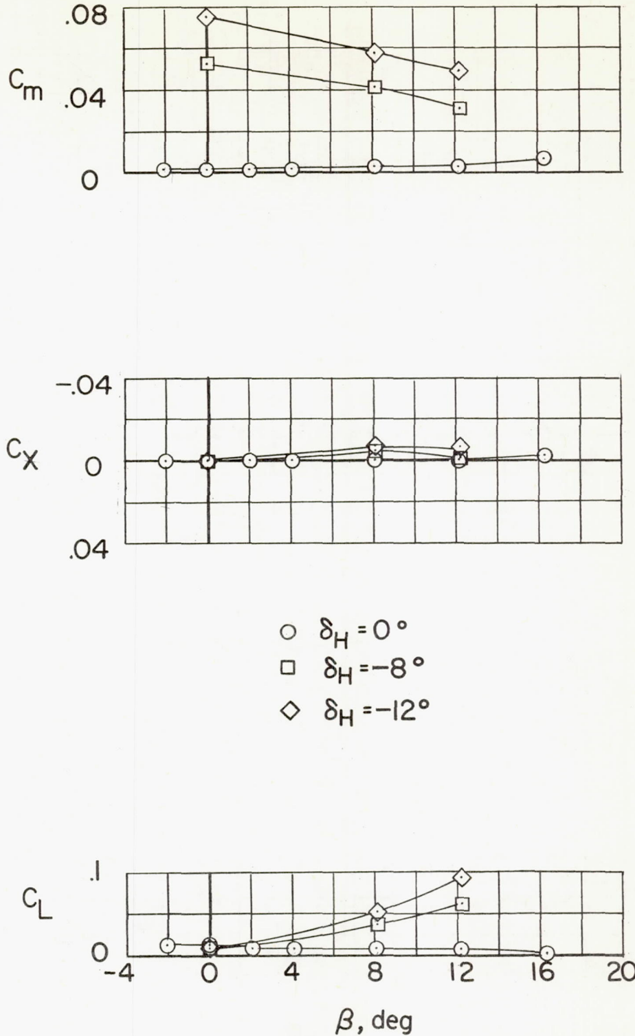
Figure 23.- Effect of horizontal canard deflection on the aerodynamic characteristics in sideslip; \alpha = 0^\circ .
