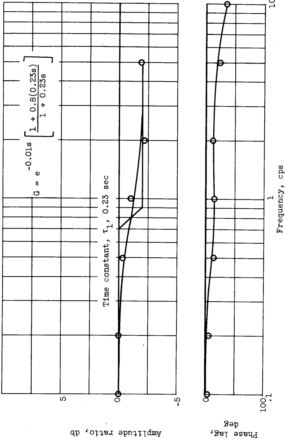
(d) Station 48; Mach number, 2.35; base diffuser-exit total-pressure ratio, 9.10; fuel-air ratio amplitude, 0.015.
