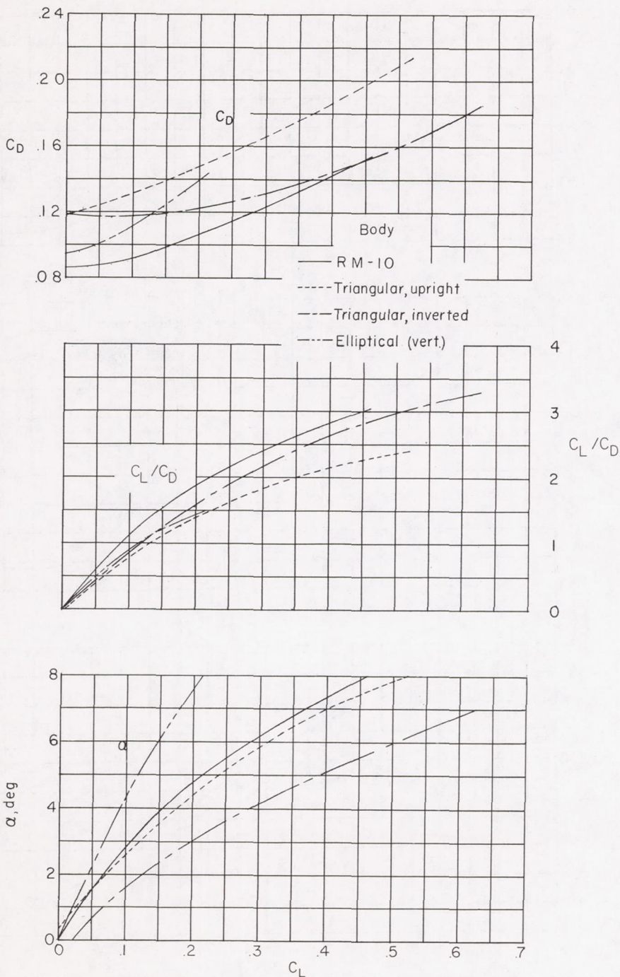
Figure 7.- Variation of \alpha , C_L/C_D , and C_D with C_L for four body configurations. M = 3.12 .
