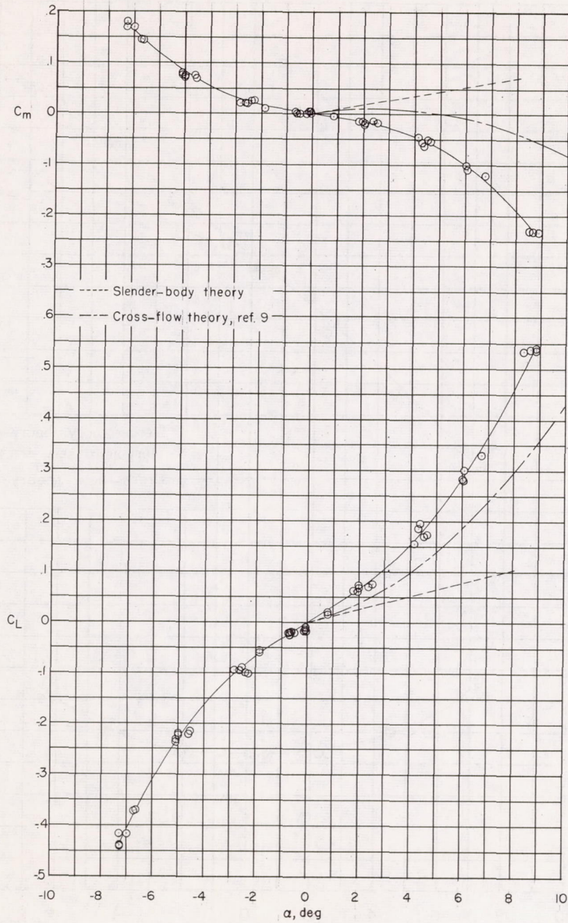
(a) Variation of C_L and C_m with \alpha .
