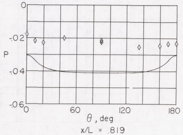
(a) Elliptical body (major axis vertical).
