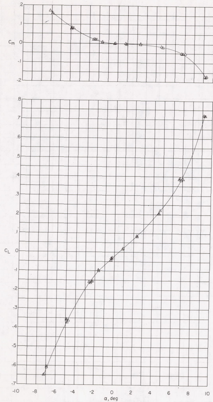
(a) Variation of C_L and C_m with \alpha .
