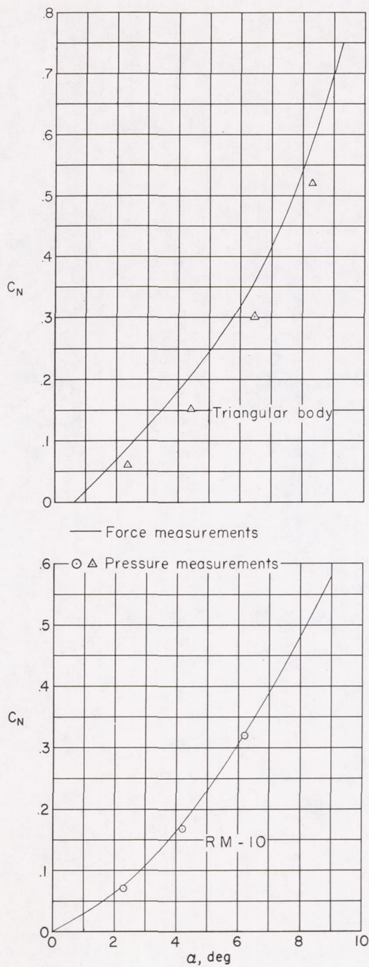
Figure 16.- Comparison of normal-force coefficients obtained from force measurements and from pressure measurements. M = 3.12 .
