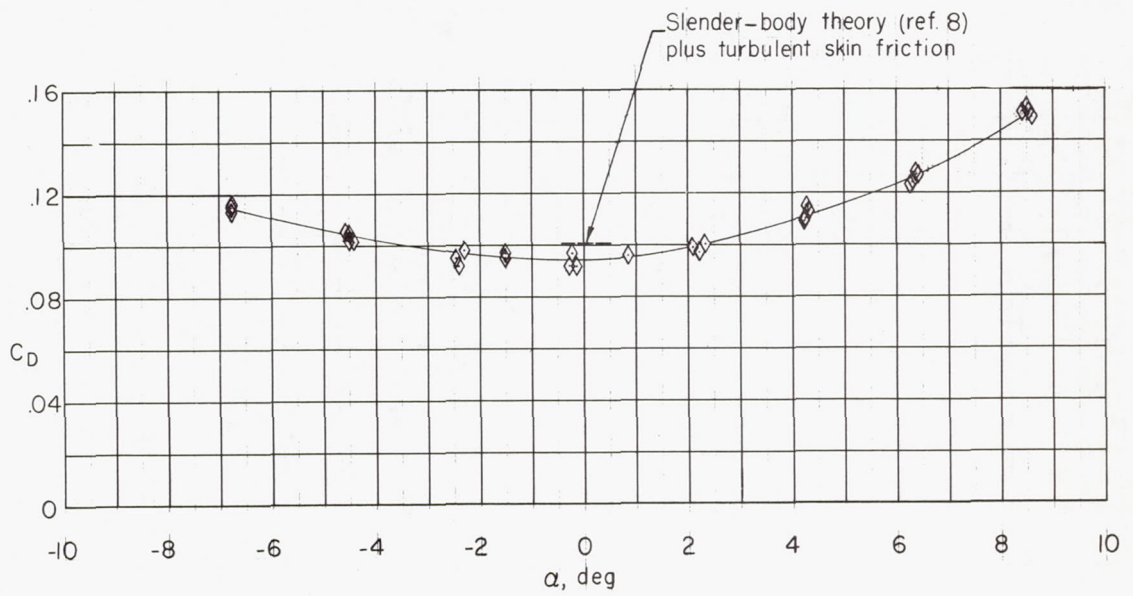
(b) Variation of C_D and C_L/C_D with \alpha .
