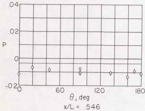
(a) Elliptical body (major axis vertical).
