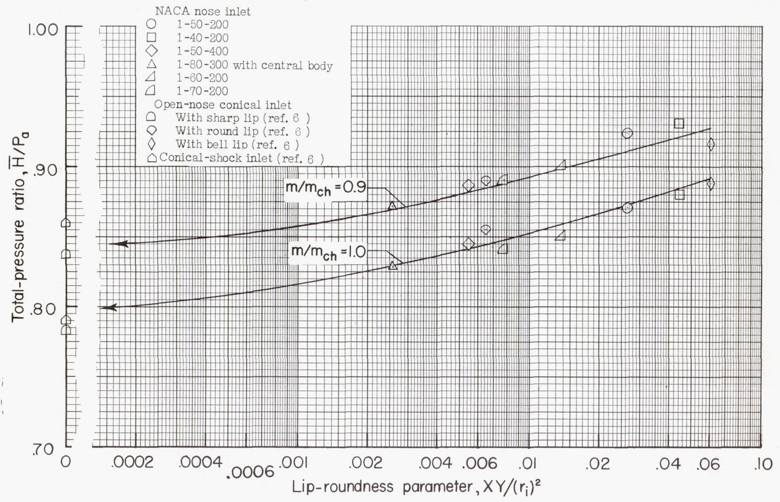
Figure 19.- Variation of average total-pressure ratio with the lip-roundness parameter \frac{XY}{r_i^2} .
