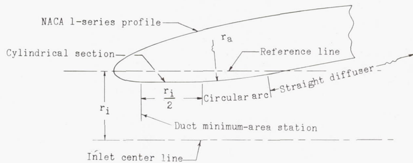
NACA Nose-Inlet Design Details
