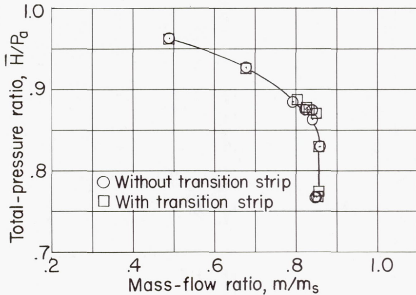
Figure 15.- Effect of transition strip on variation of total-pressure ratio with mass-flow ratio. NACA 1-70-200 nose inlet.
