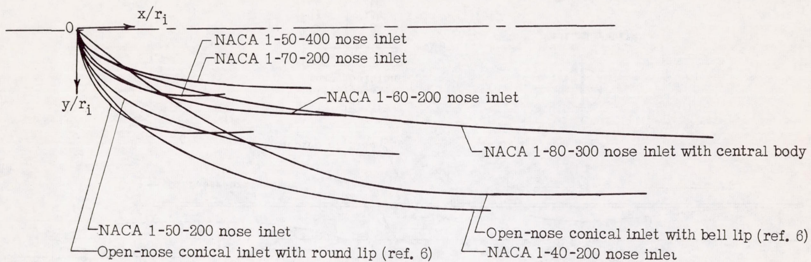
Figure 4.- Inner-lip-shape comparison based on common inlet radius r_i .
