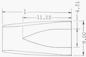
NACA 1-70-200 nose inlet
