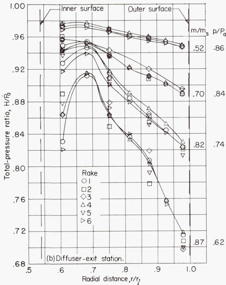
Figure 9.- Total-pressure-ratio variation with radial distance; NACA 1-70-200 nose inlet. Duct radius at 5-inch station is 2.86 inches.
