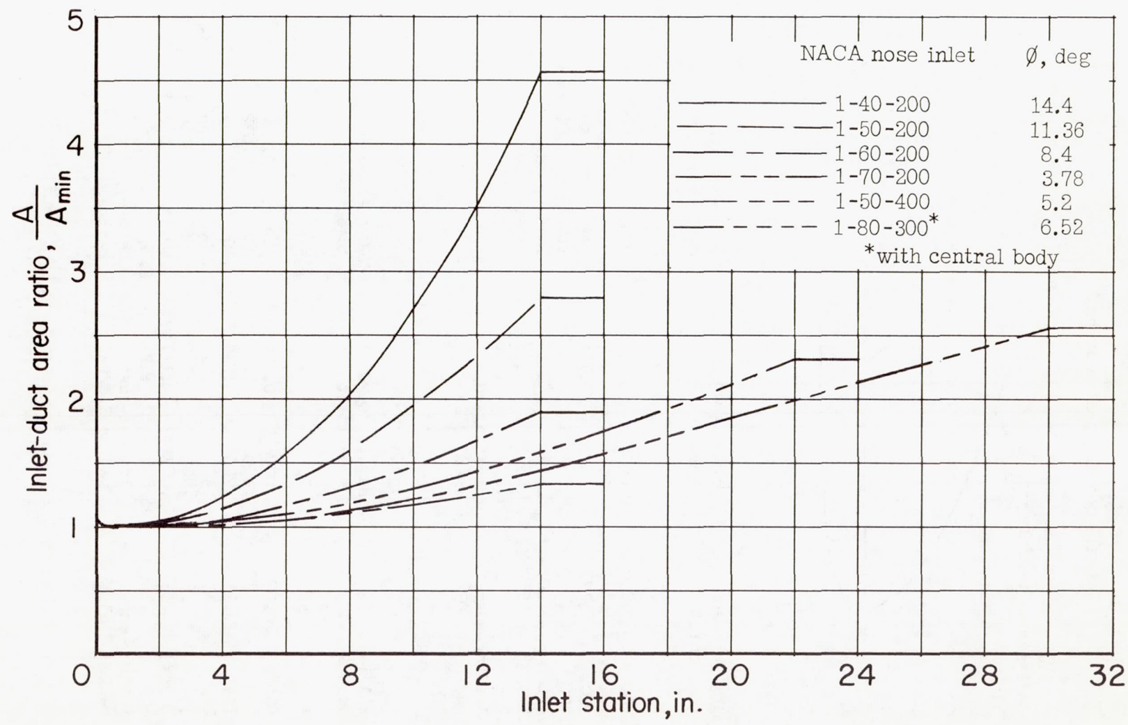
Figure 3.- Variation of inlet-duct area.
