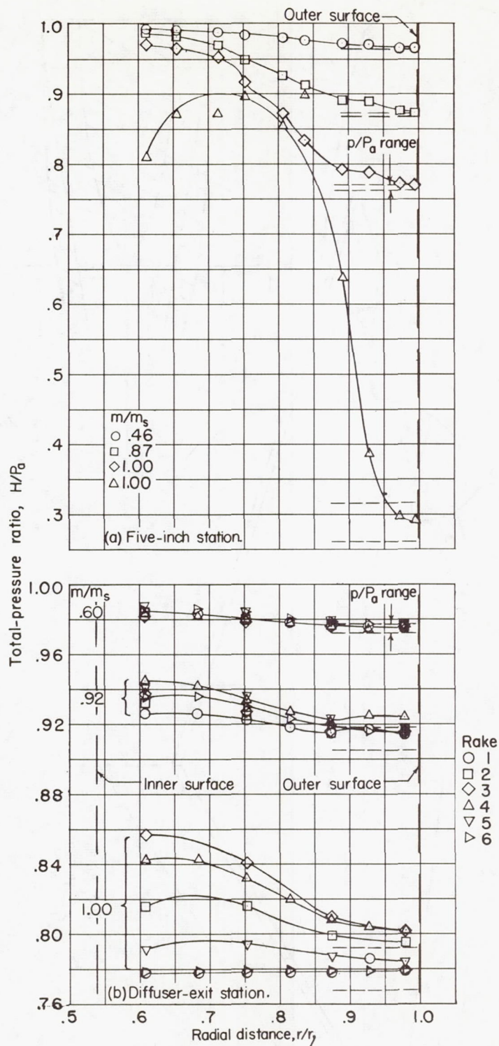
Figure 7.- Total-pressure-ratio variation with radial distance; NACA 1-40-200 nose inlet. Duct radius at 5-inch station is 1.85 inches.
