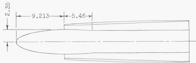
NACA 1-80-300 nose inlet with elliptical central body
