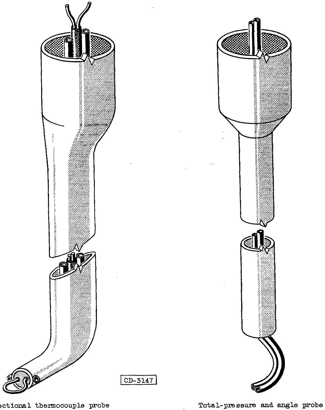
Figure 2. - Instrumentation used to survey downstream of turbine rotor.
