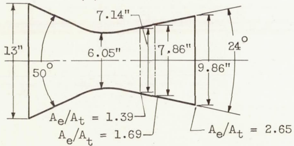
(c) 24° Nozzle.
