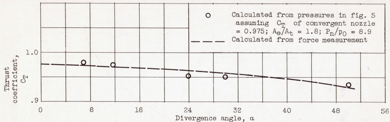
Figure 6. - Variation in thrust coefficient calculated from pressure distributions in divergent sections of nozzles at design pressure ratio with nozzle divergence angle.
