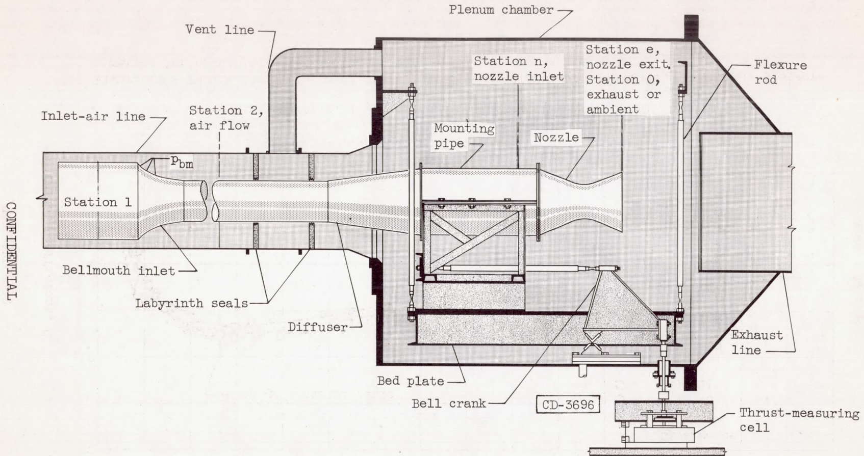
Figure 2. - Installation of nozzle in test chamber.
