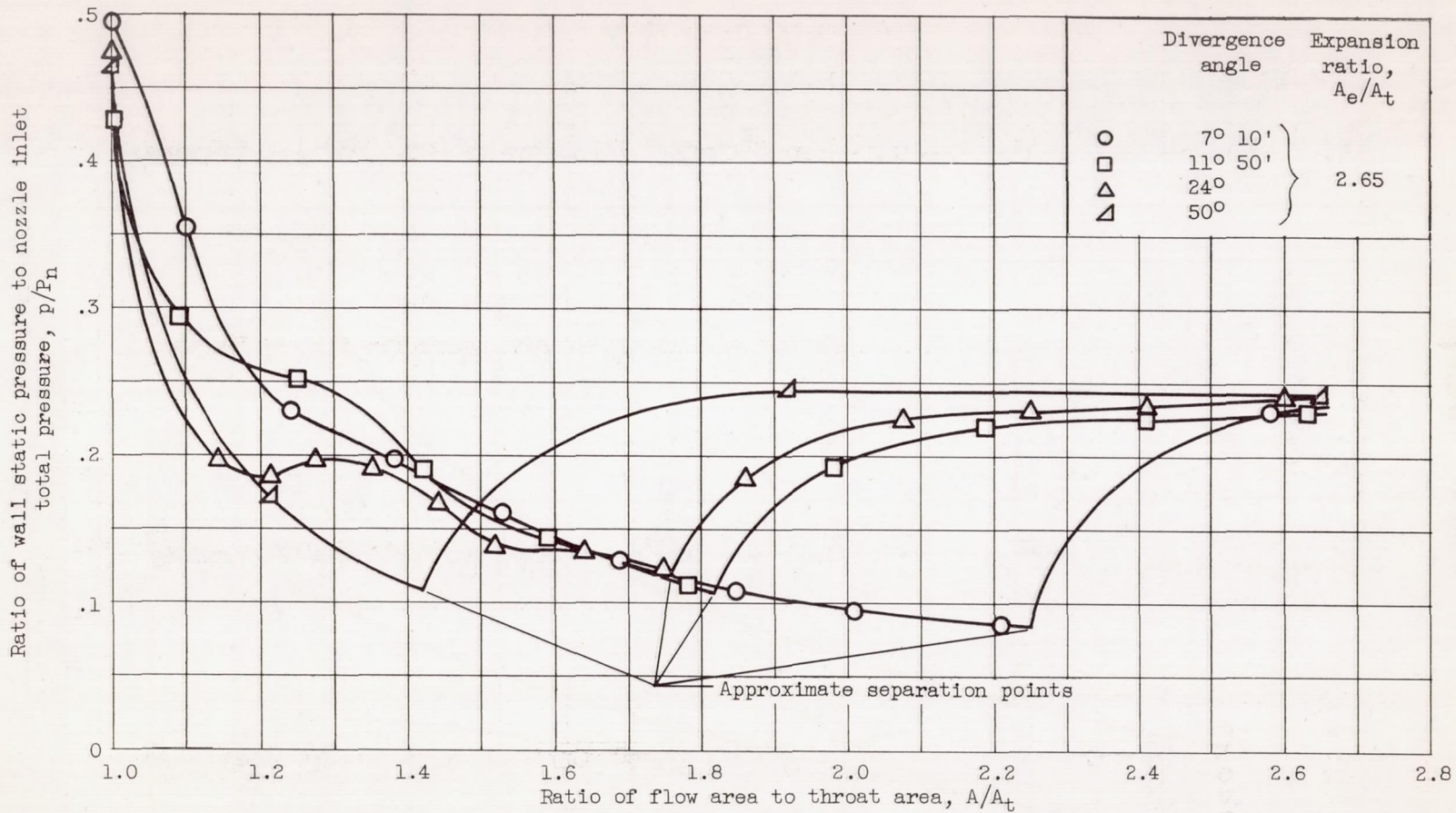
Figure 8. - Generalized pressure distributions along divergent walls of several convergent-divergent nozzles having various divergence angles at a nozzle pressure ratio of approximately 4.
