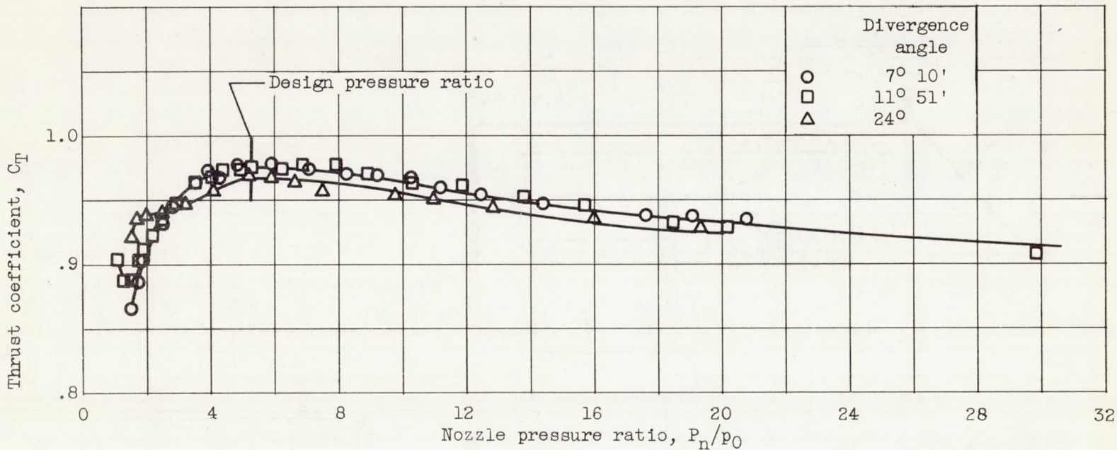
(a) Expansion ratio, 1.39; divergence angles, 7° 11', 11° 50', and 24°.
