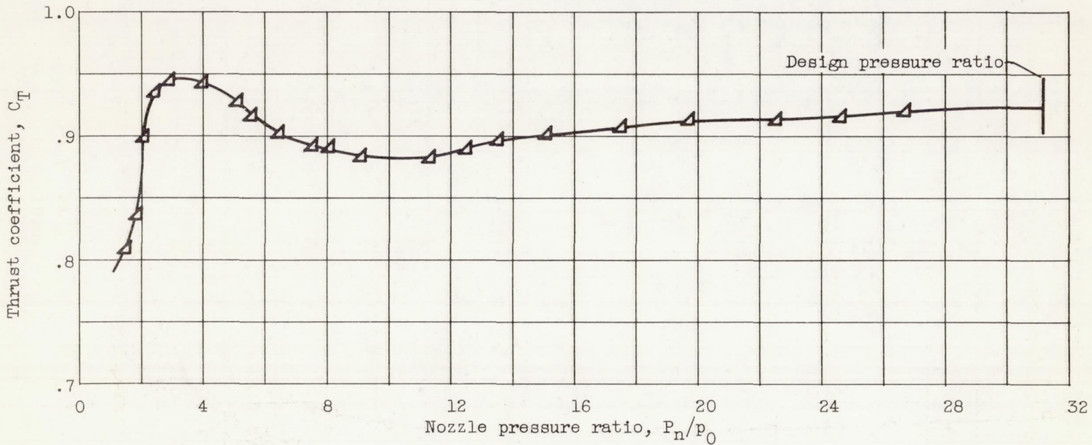
Figure 3. - Concluded. Thrust coefficients of convergent-divergent nozzles over a range of nozzle pressure ratios for specified expansion ratio and various divergence angles.
