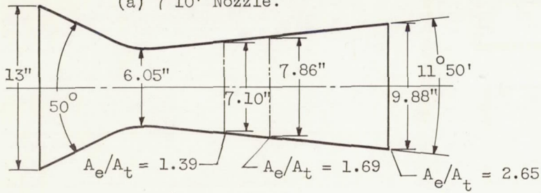
(b) 11° 50' Nozzle.
