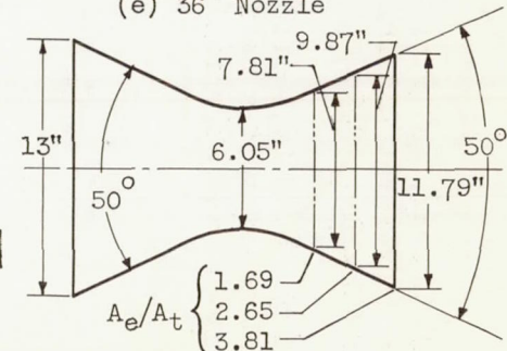
(f) 50° Nozzle.
