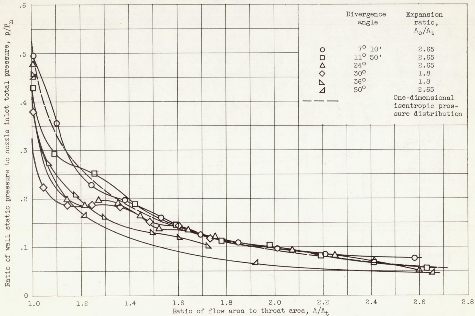
Figure 5. - Generalized pressure distributions along divergent walls of several convergent-divergent nozzles having various divergence angles at nozzle pressure ratios at or above design.
