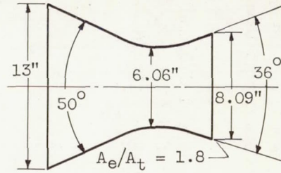
(e) 36° Nozzle
