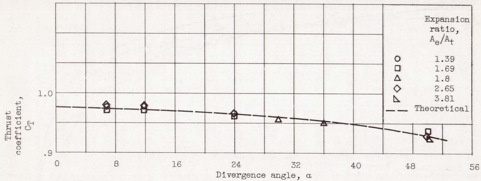
Figure 4. - Variation in thrust coefficient at design nozzle pressure ratio with nozzle divergence angle.
