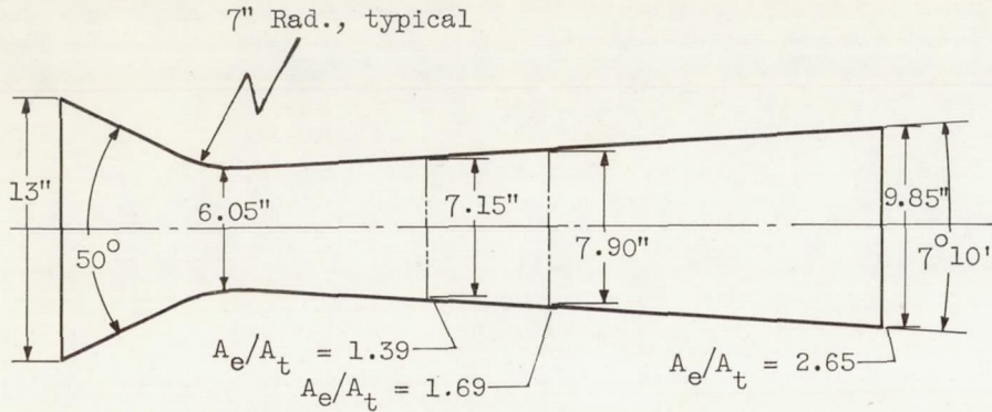
(a) 7° 10' Nozzle.
