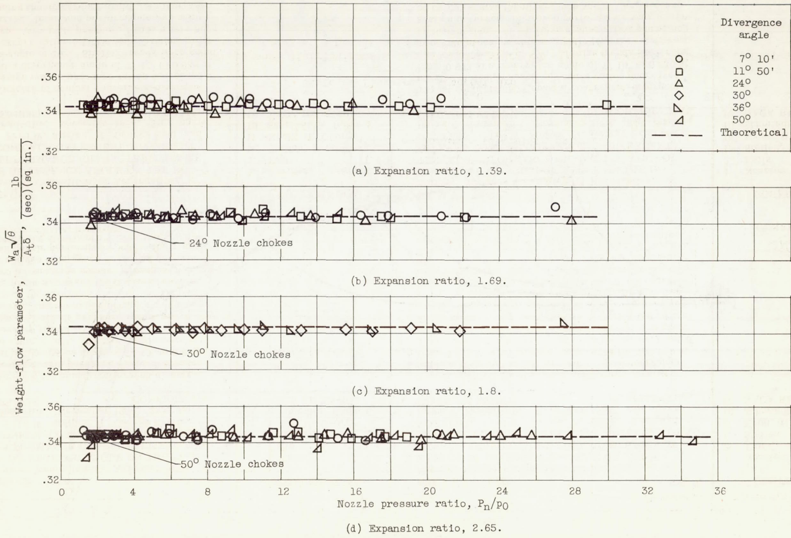
Figure 9. - Variation in weight-flow parameter with nozzle pressure ratio for nozzles having various expansion ratios and divergence angles.
