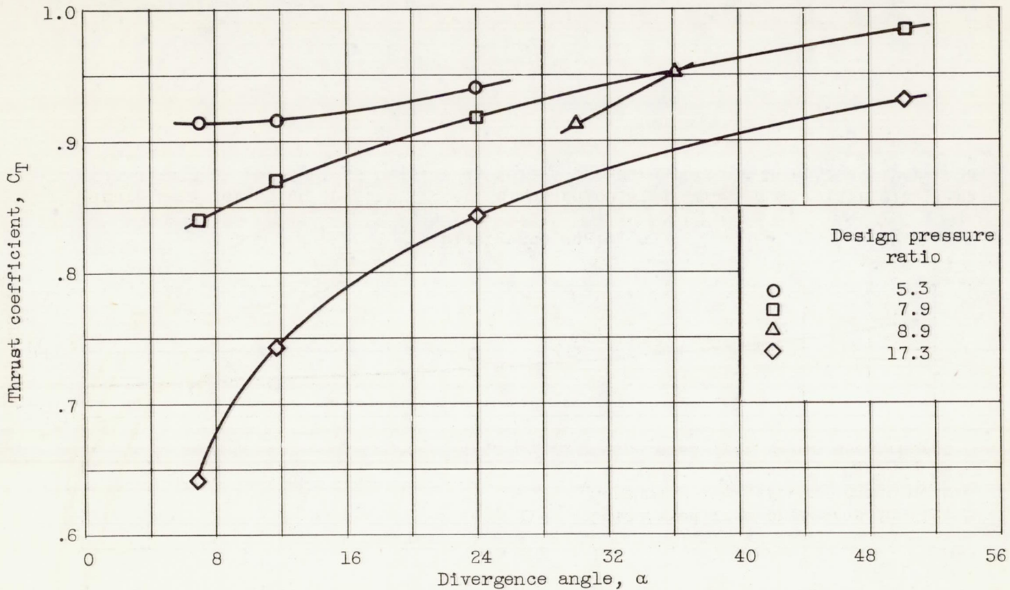
Figure 7. - Variation in thrust coefficient at a nozzle pressure ratio of 2.0 with divergence angle for nozzles of various design pressure ratios.
