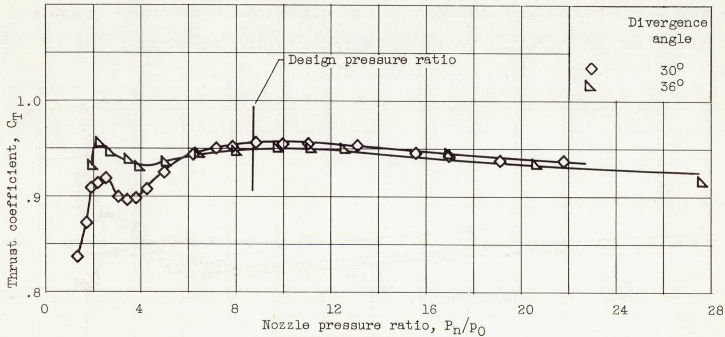
(c) Expansion ratio, 1.8; divergence angles, 30° and 36°.
