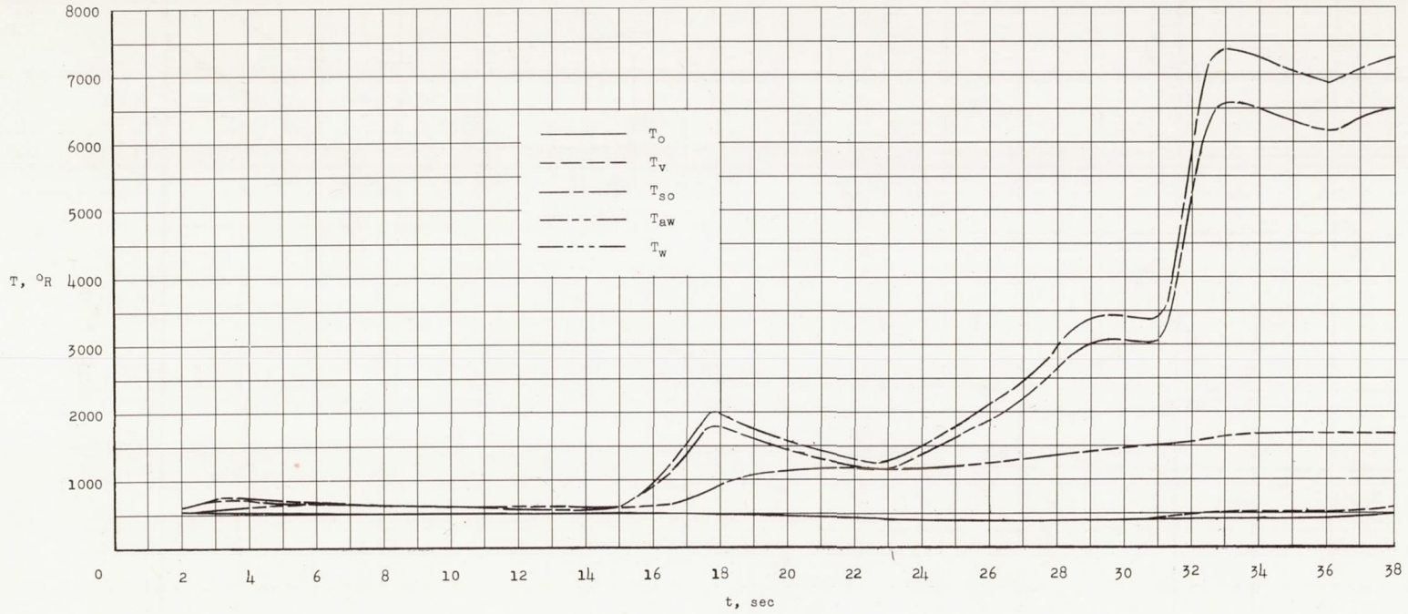
Figure 9.- Time histories of various temperatures.
