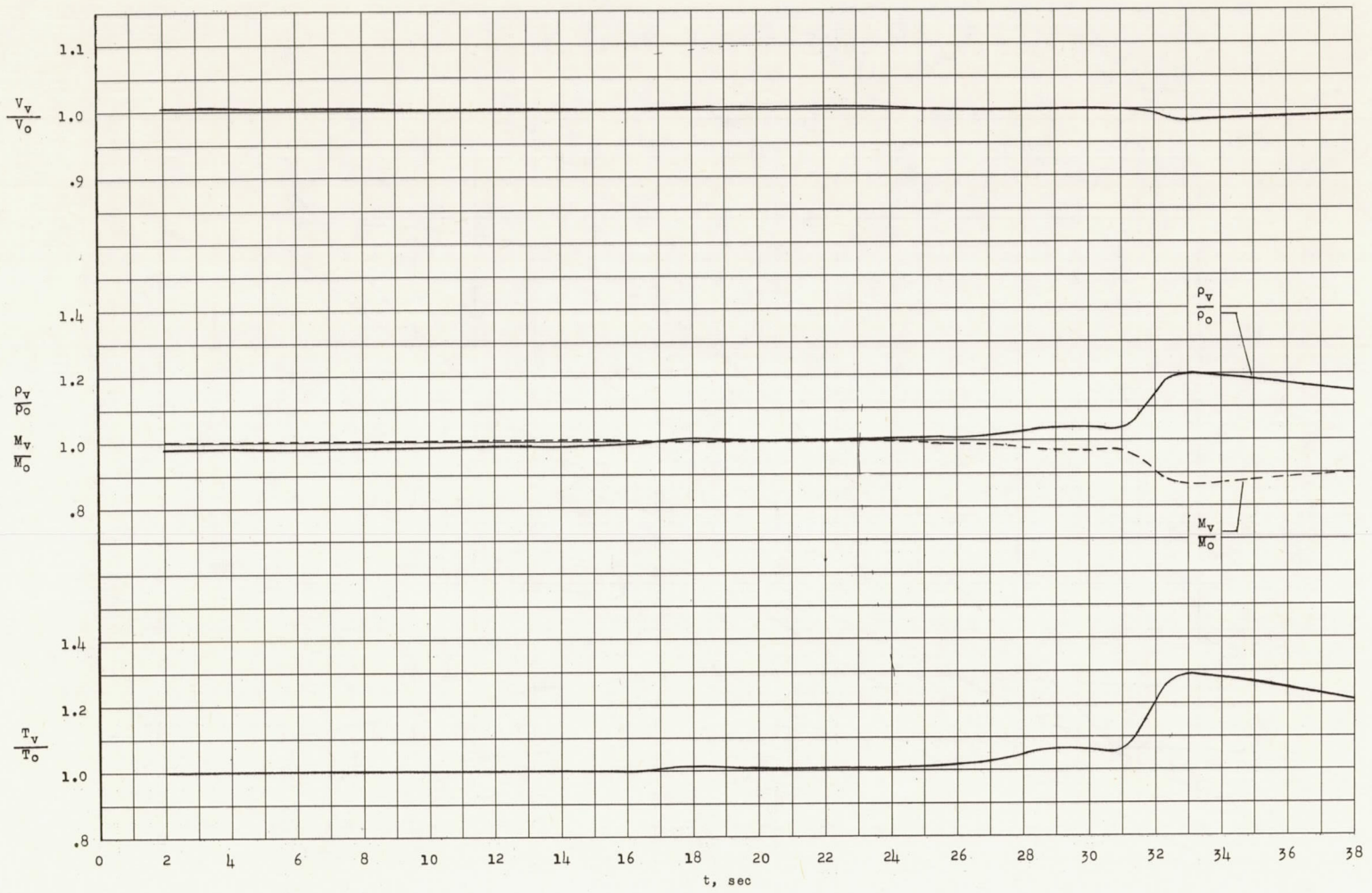
Figure 13.- Calculated flow parameters at the temperature measuring station.
