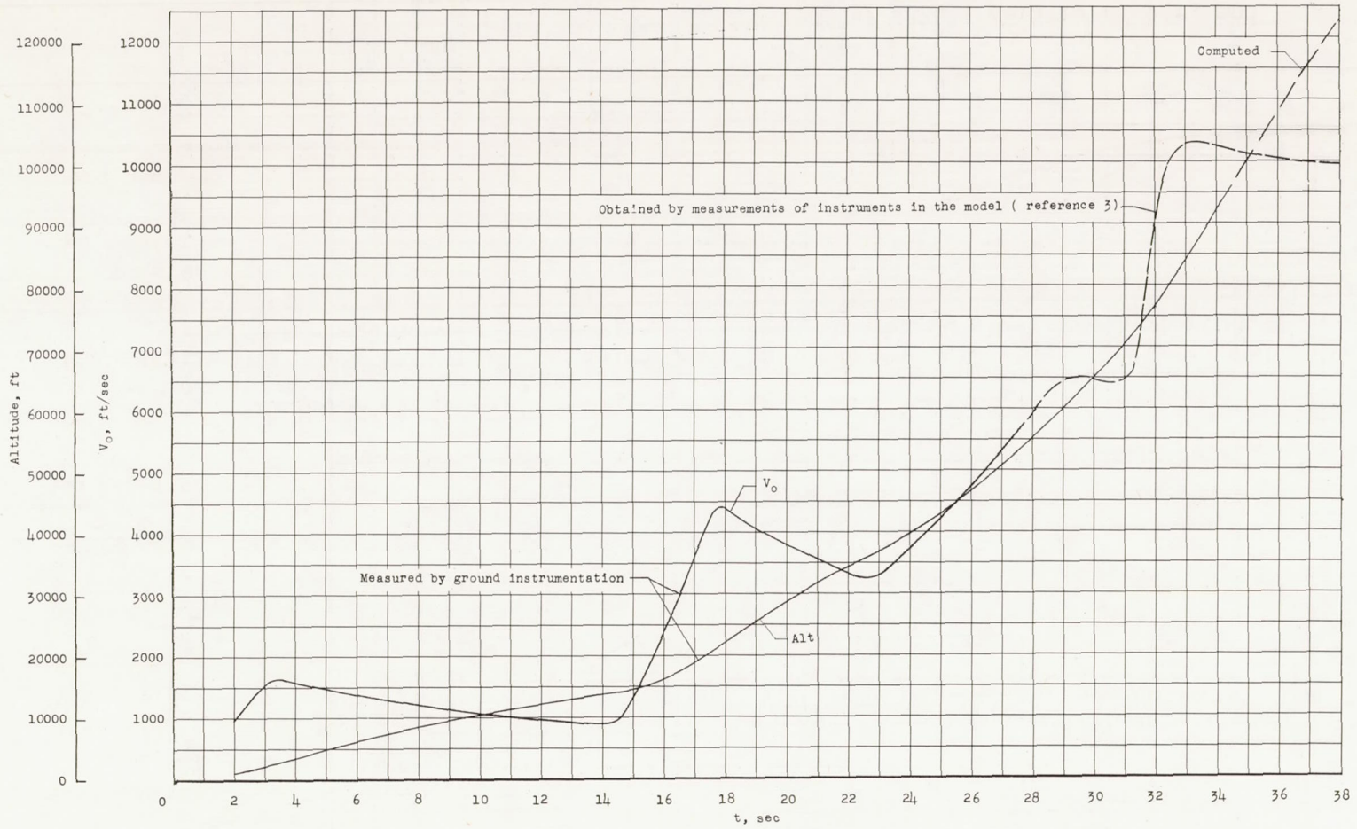
Figure 5.- Time histories of the flight-path velocity and altitude.
