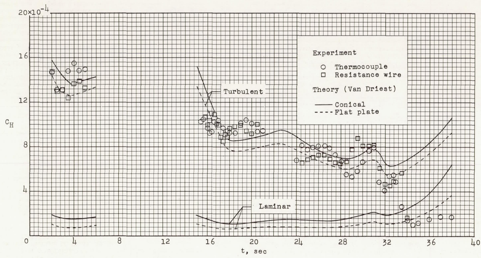
Figure 15.- Time histories of experimental and theoretical Stanton numbers.
