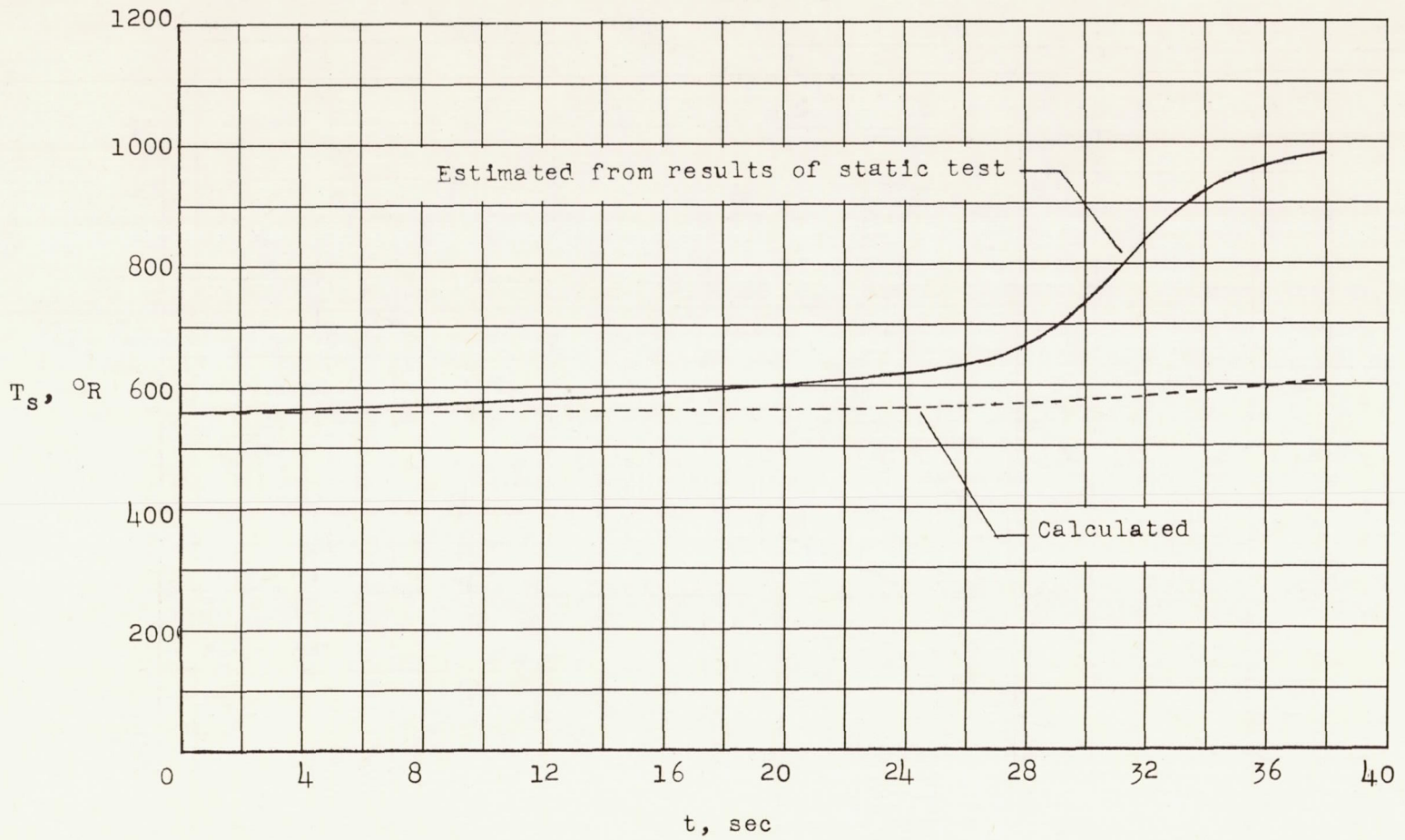
Figure 11.- Variation of shield temperature with time.
