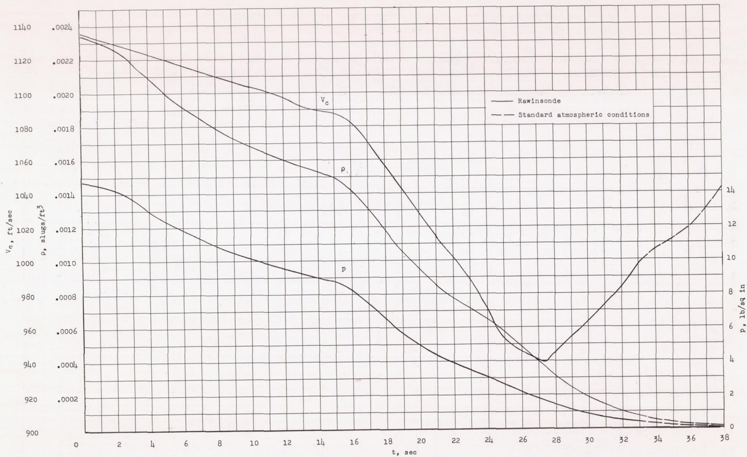
Figure 6.- Time histories of the velocity of sound, density of air, and the static air pressure.
