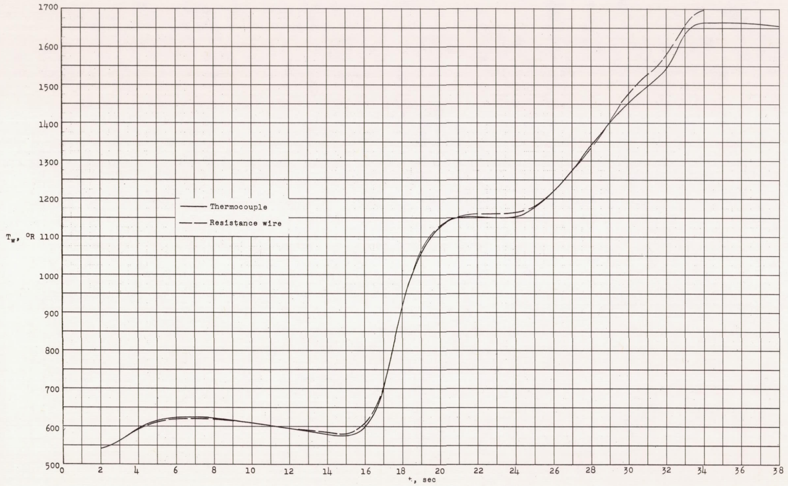
Figure 8.- Comparison of the skin temperatures measured by the thermocouple and by the resistance wire.
