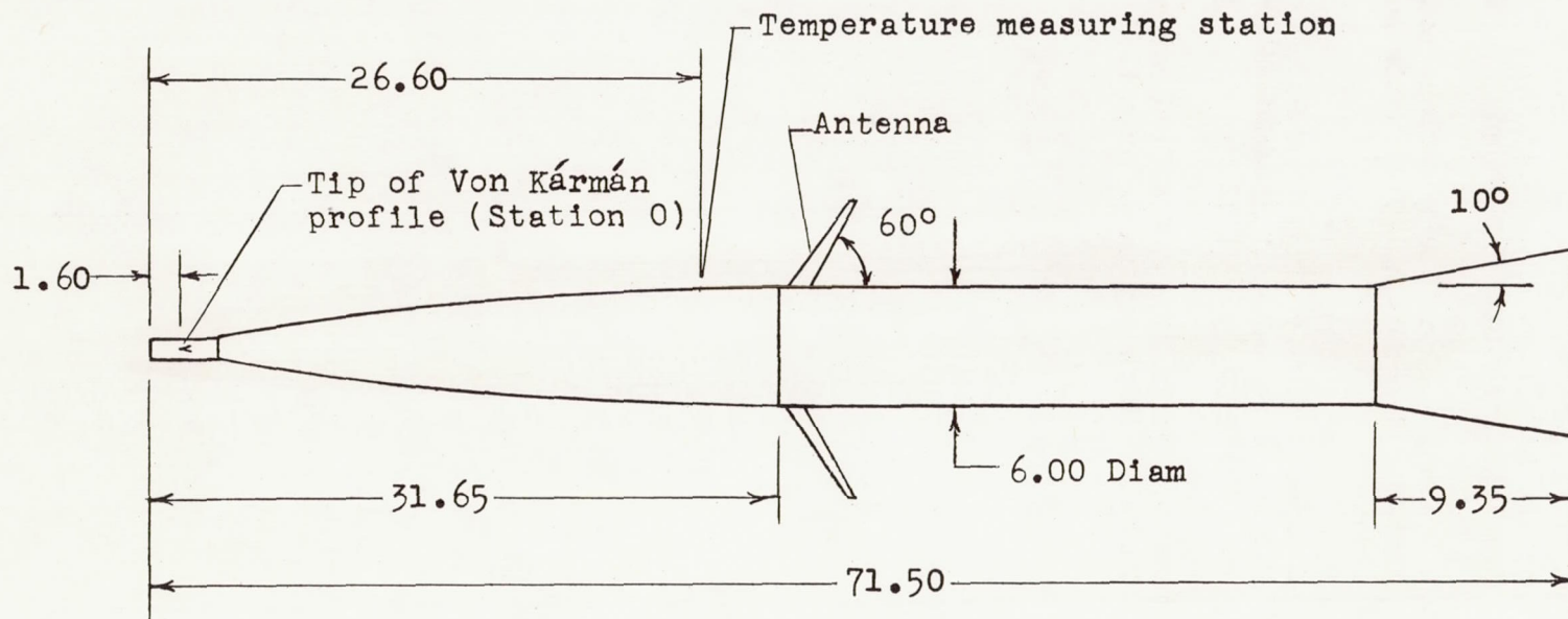
Figure 1.- Sketch of model and detail of nose construction. All linear dimensions in inches.
