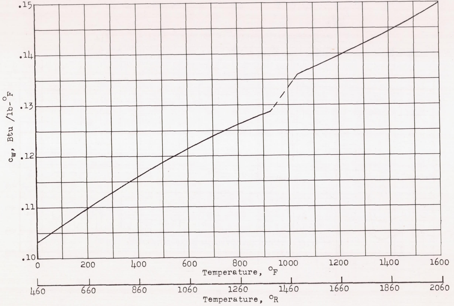
Figure 10.- Instantaneous specific heat of Inconel. (See ref. 6.)
