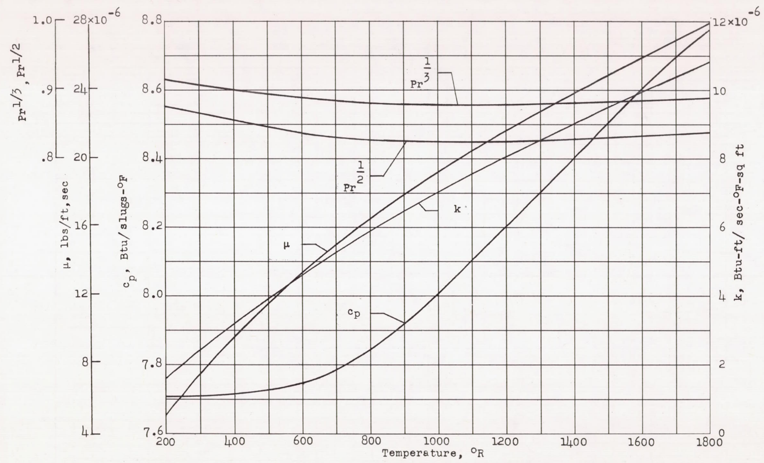
Figure 12.- Thermal properties of air. (See ref. 8.)
