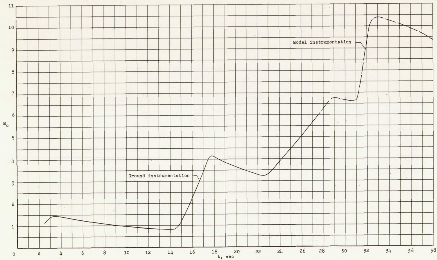
Figure 7.- Time history of the Mach number.
