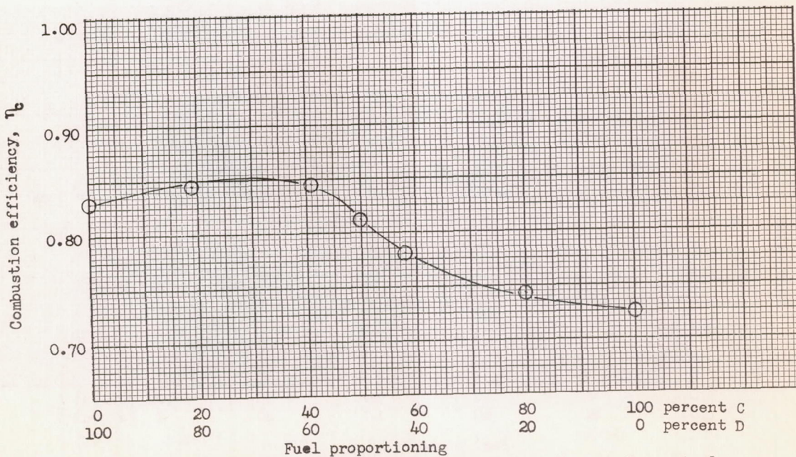
(d) Effect of proportioning fuel between profiles C and D ; actual fuel-air ratio, 0.035.
