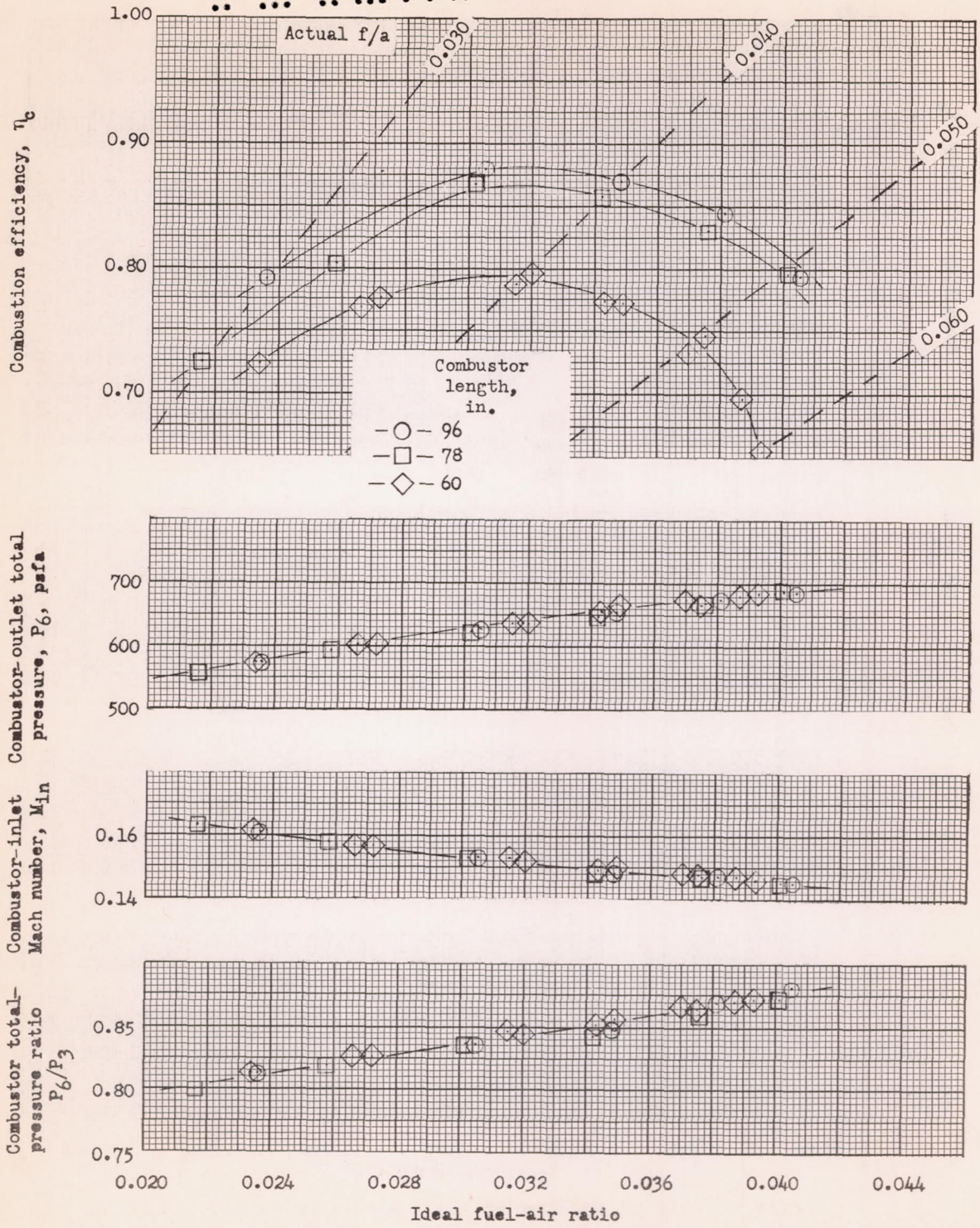
(a) Air flow, 40 pounds per second.
