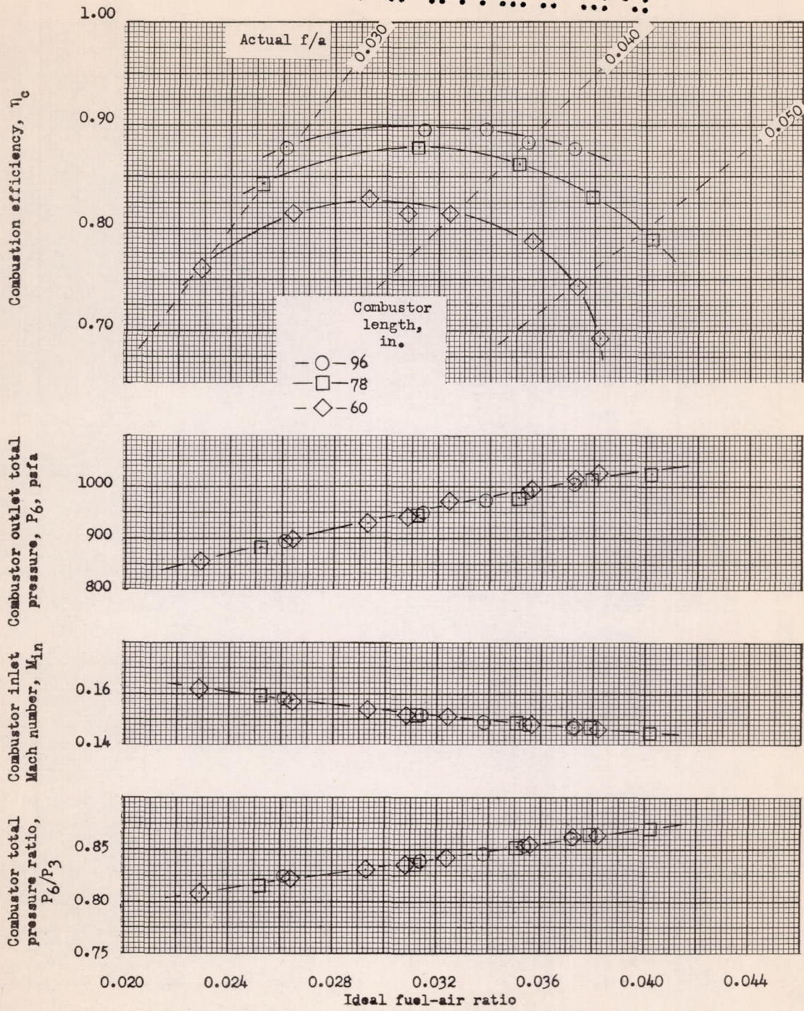
(b) Air flow, 60 pounds per second.
