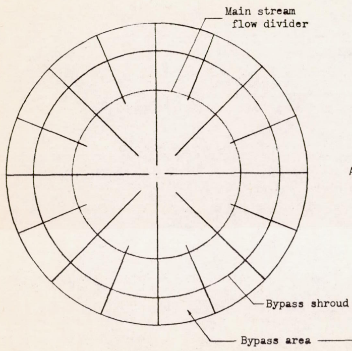
(a) Fuel bar arrangement.
