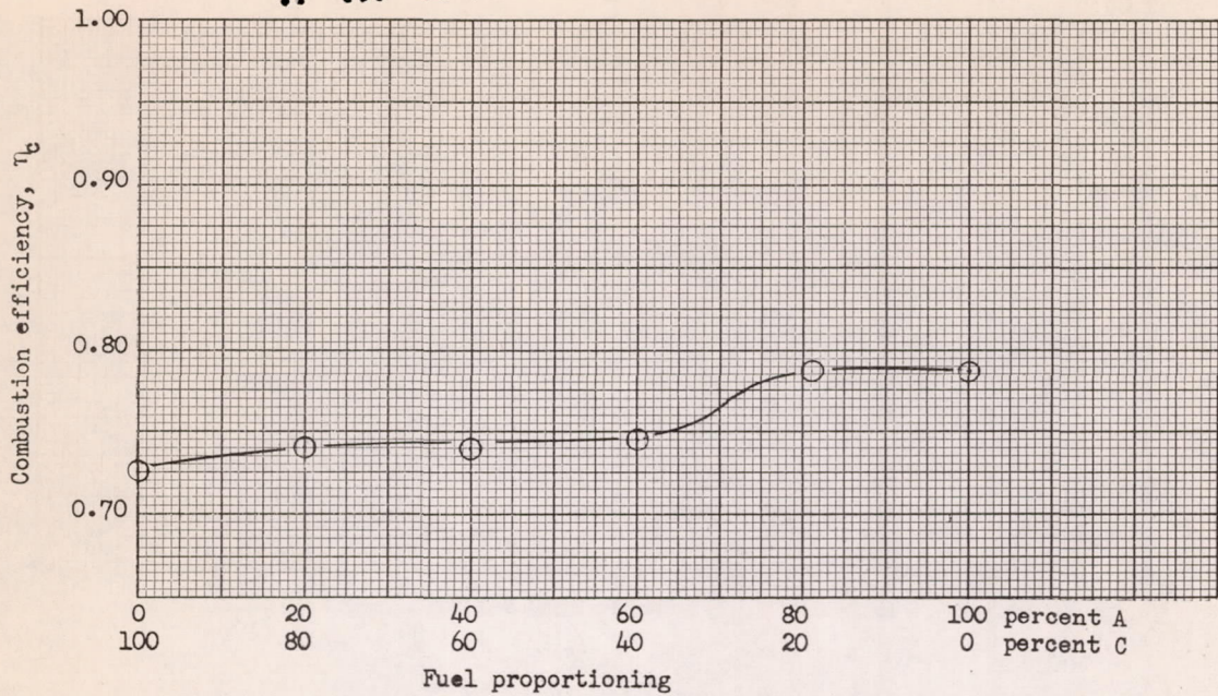
(a) Effect of proportioning fuel between profiles A and C; actual fuel-air ratio, 0.035.
