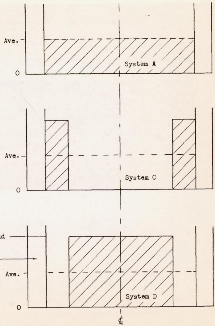
(b) Fuel profiles used.
