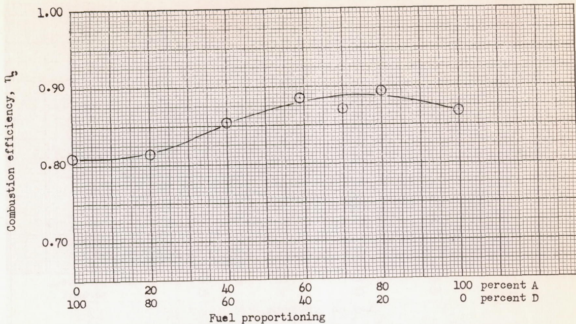
(c) Effect of proportioning fuel between profiles A and D ; actual fuel-air ratio, 0.040.
