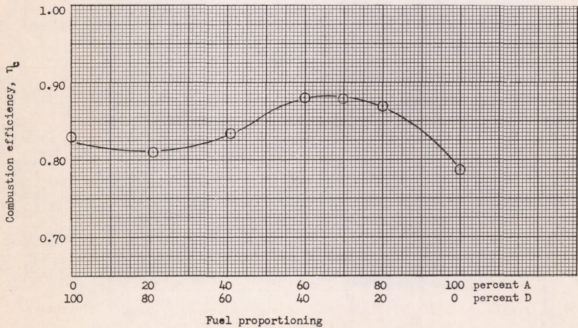
(b) Effect of proportioning fuel between profiles A and D; actual fuel-air ratio, 0.035.
