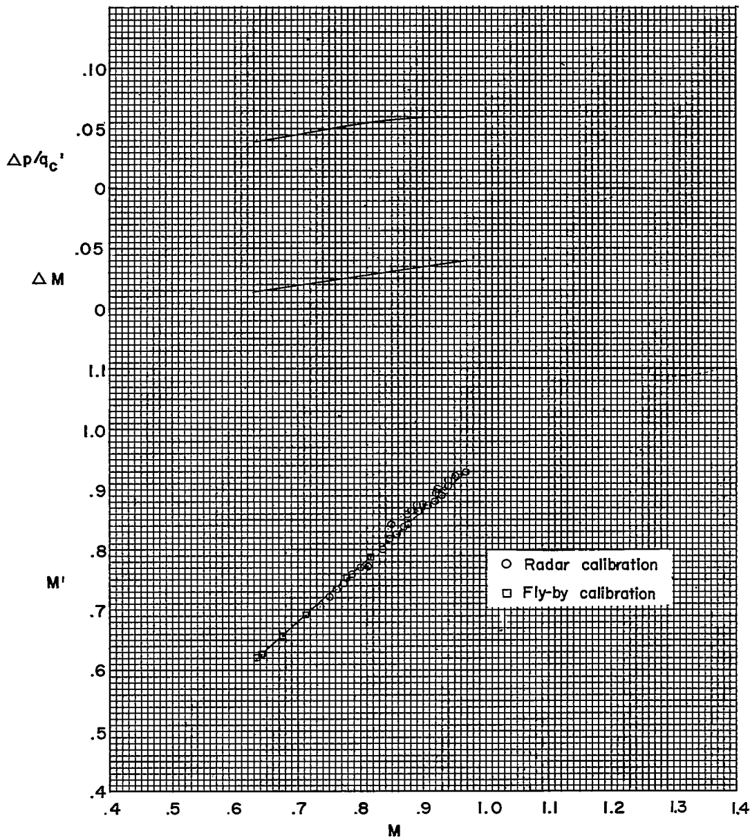
Figure 5.- Static-pressure errors for airplane C.
