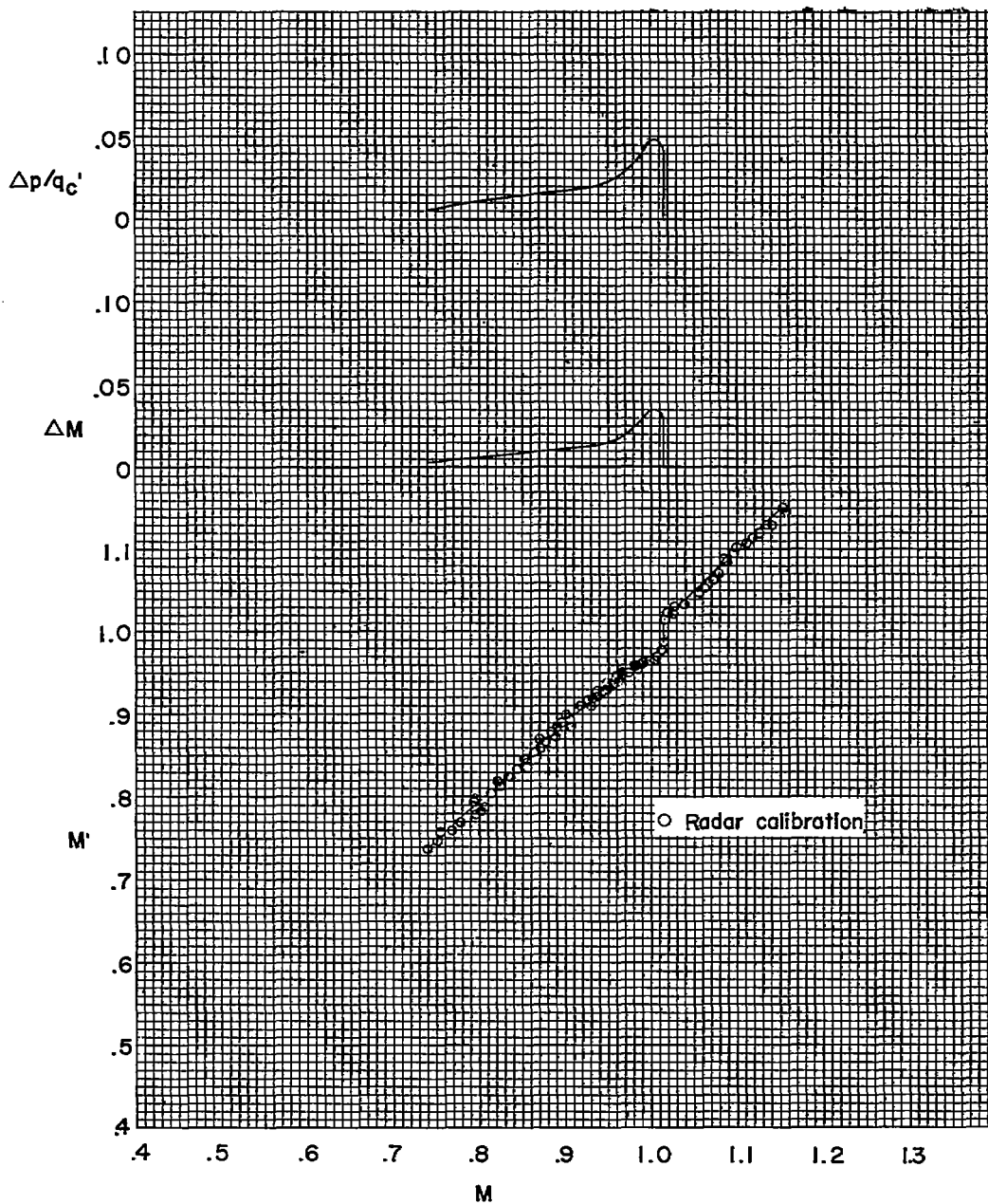
Figure 15.- Static-pressure errors for airplane P.
