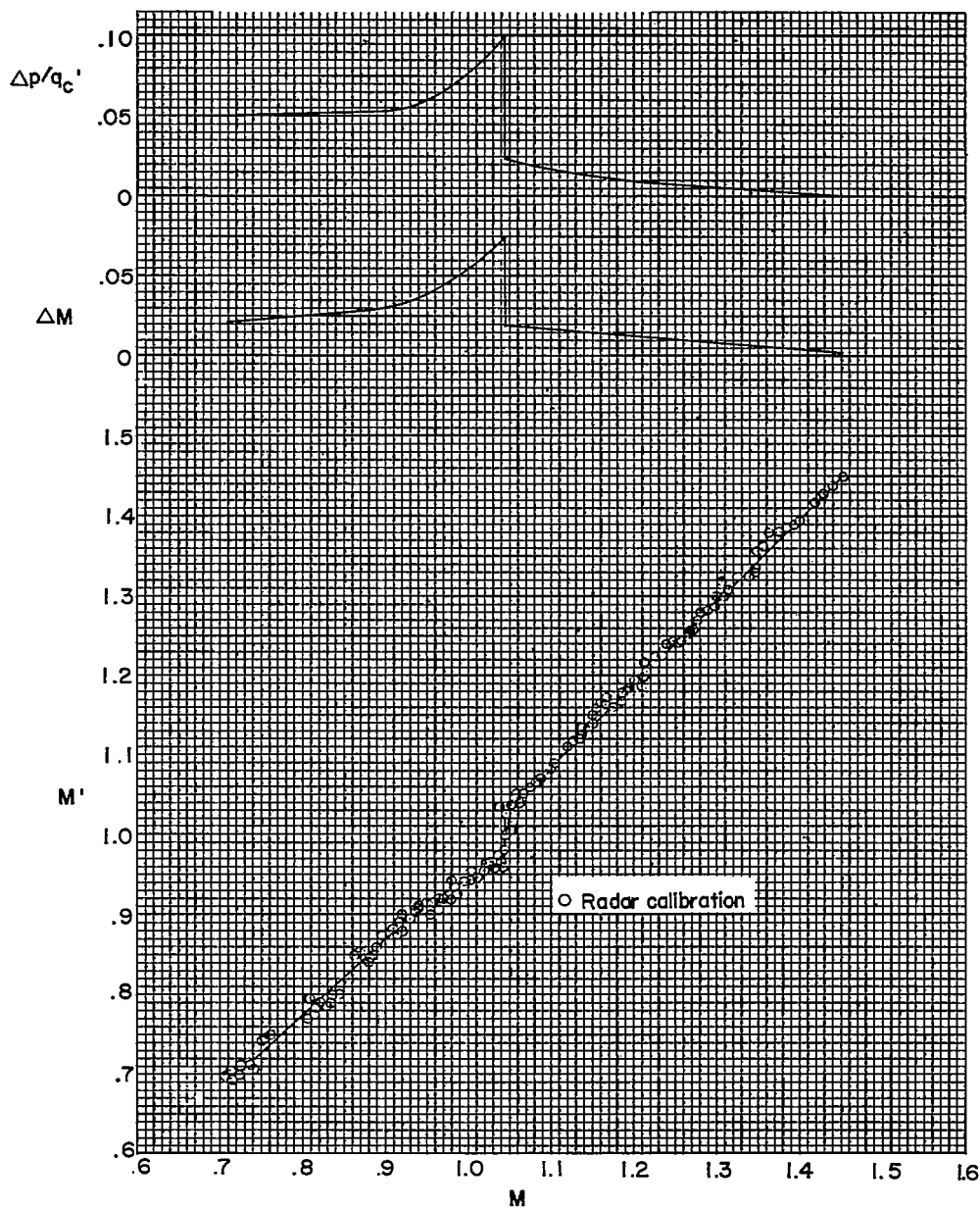
Figure 7.- Static-pressure errors for airplane E.
