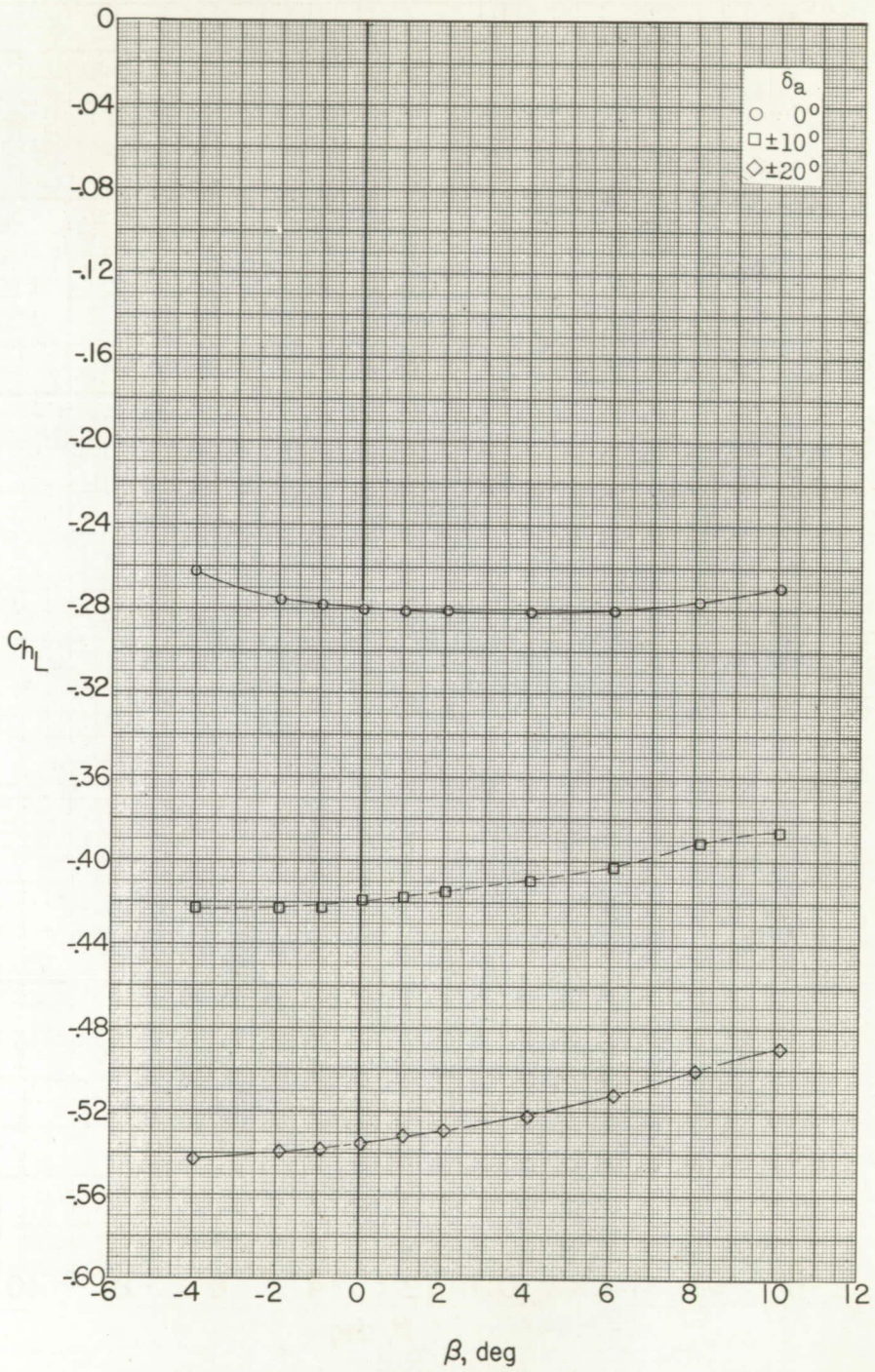
(c) M = 1.56 ; \alpha \approx 12.1^\circ .
