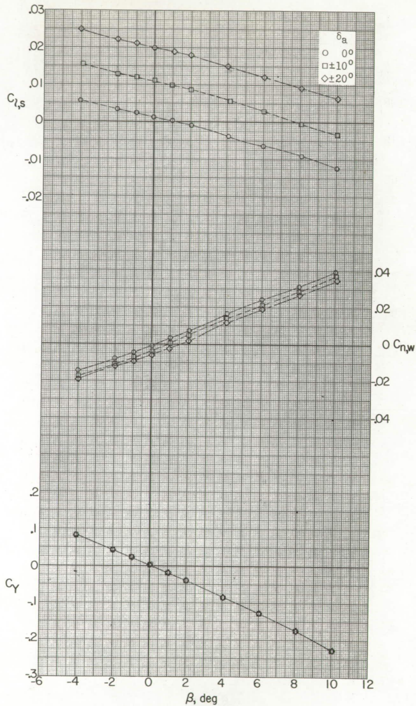
(c) M = 1.56; \alpha \approx 12.1^\circ .
