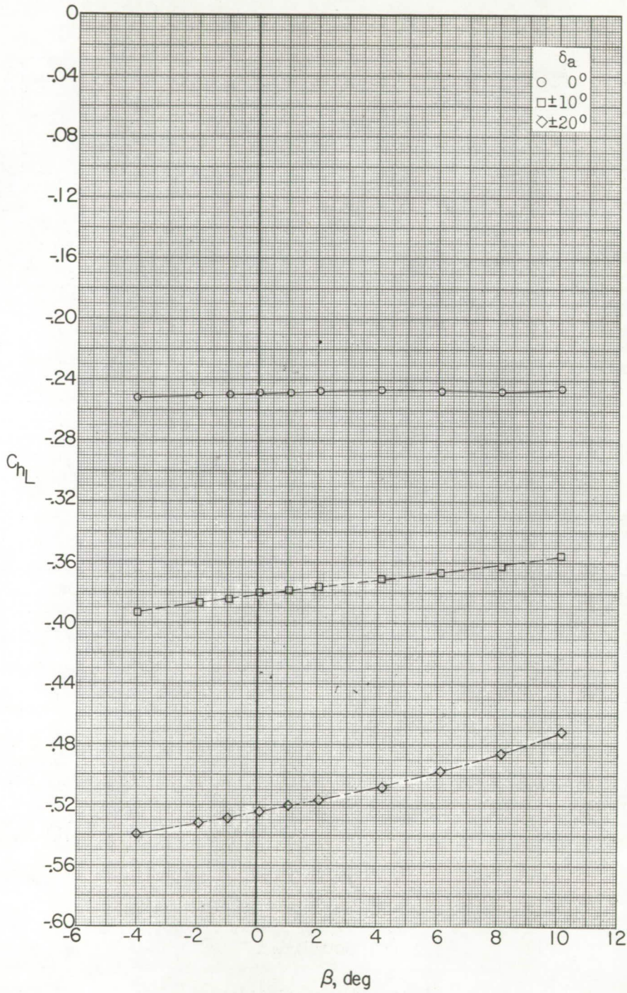
(h) M = 2.06 ; \alpha = 16.1^\circ .
