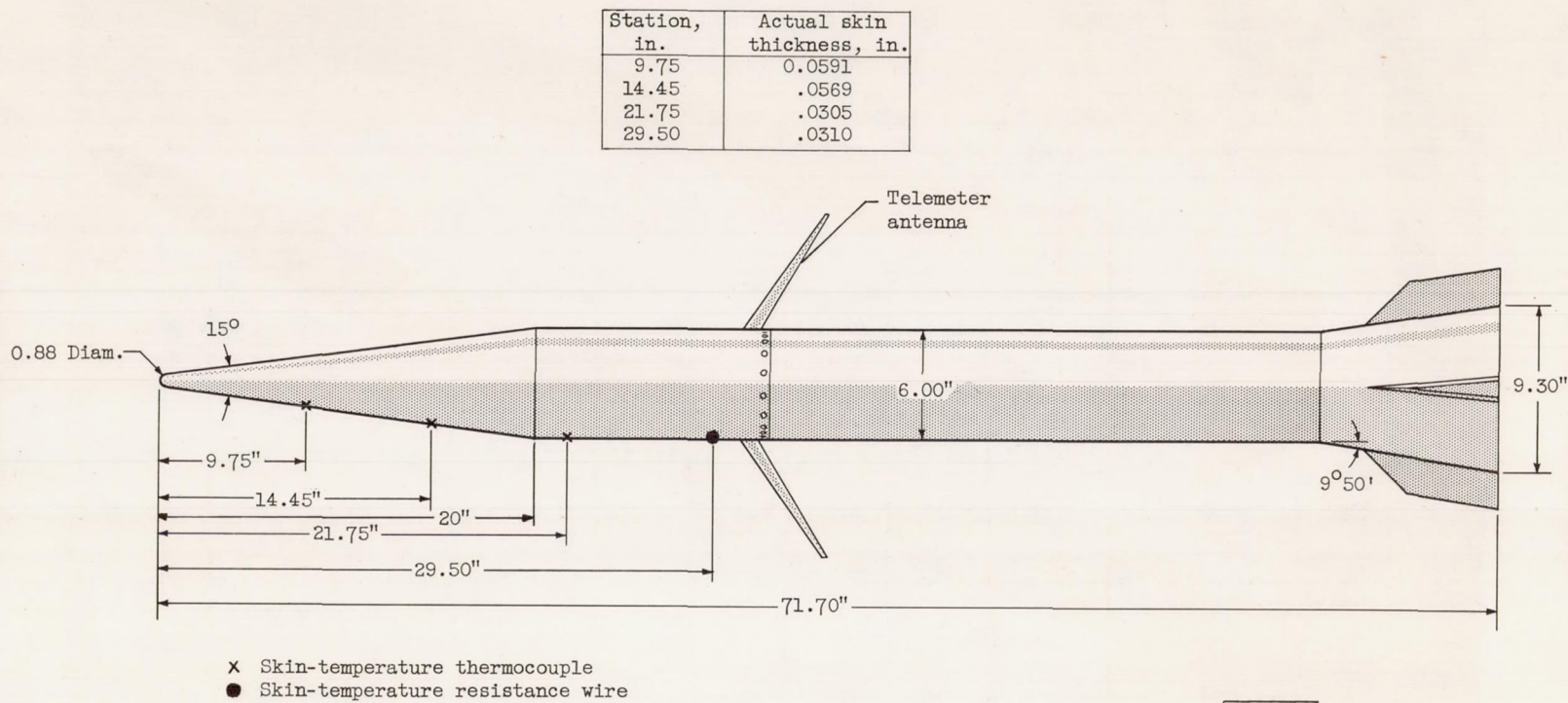
Figure 1. - Dimensions of model.
