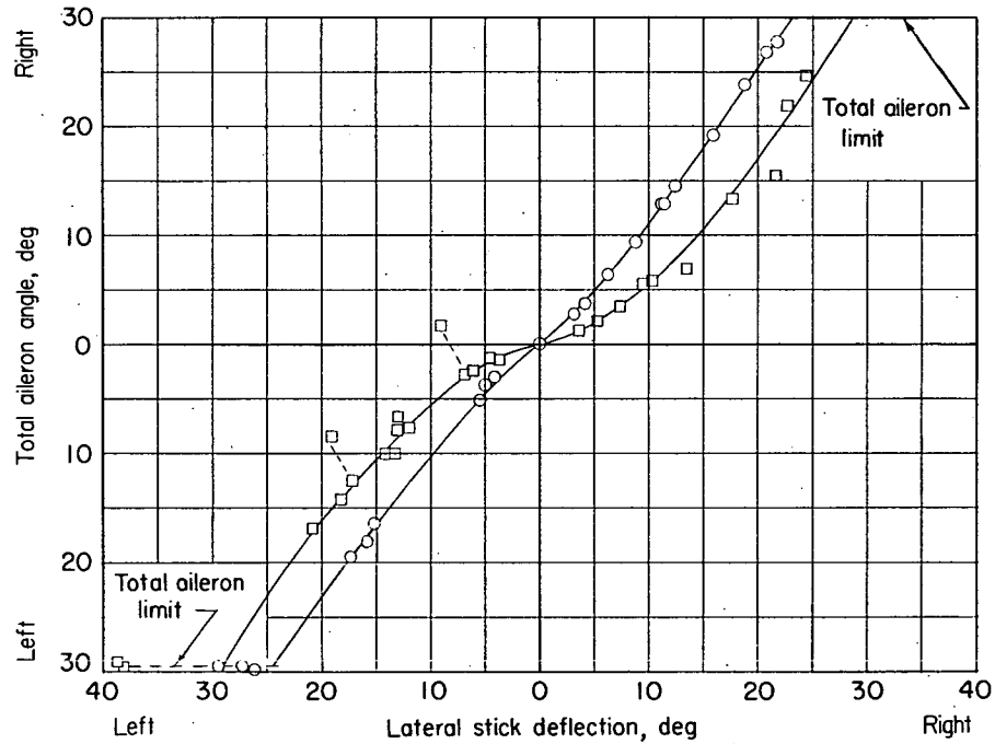
Figure 12.- Variation of total aileron deflection and rolling velocity with lateral stick deflection. Irreversible power control system; M = 0.6 ; h_p = 10,000 feet.
