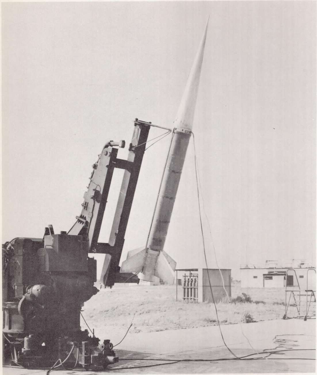
Figure 2.- Model on the launcher.
