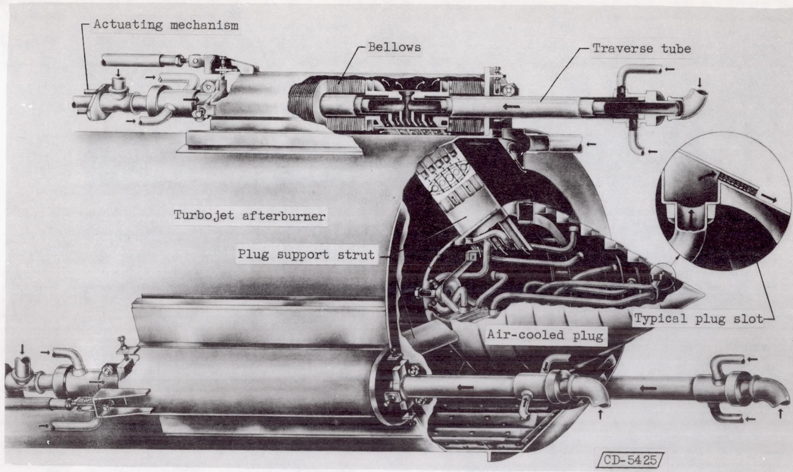
(a) Exhaust nozzle installed in afterburner.
