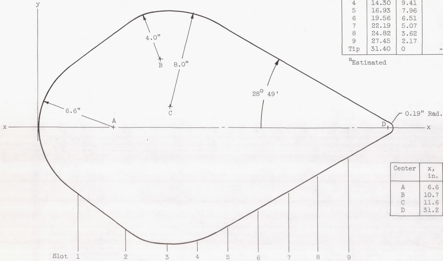
Figure 2. - Plug profile envelope dimensions.
