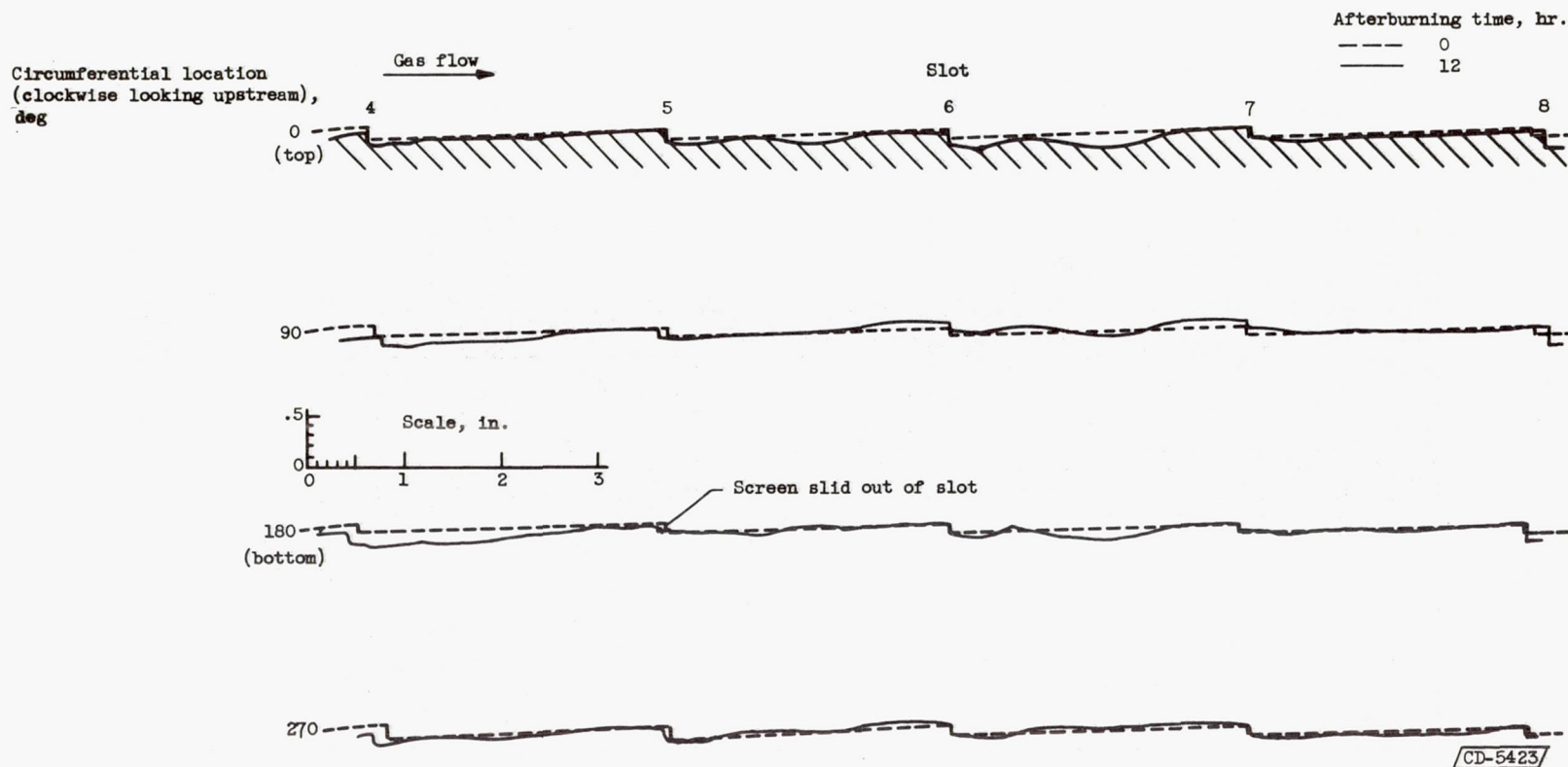
Figure 20. - Plug surface profiles of conical tailcone at beginning and end of afterburning phase.
