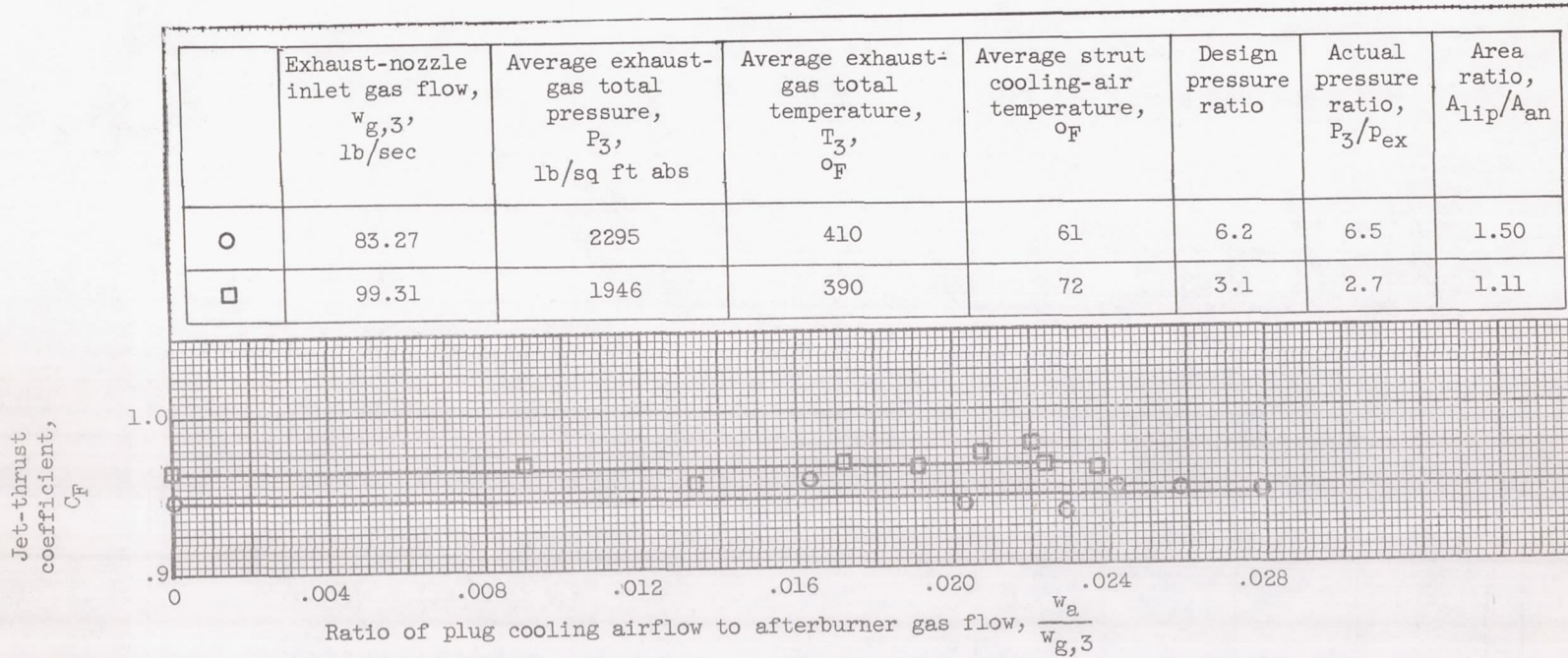
Figure 21. - Effect of plug cooling airflow on jet-thrust coefficient with outer shell cooled with corrugated louvered liner, a rough plug tailcone, and cooling air to plug slots only.
