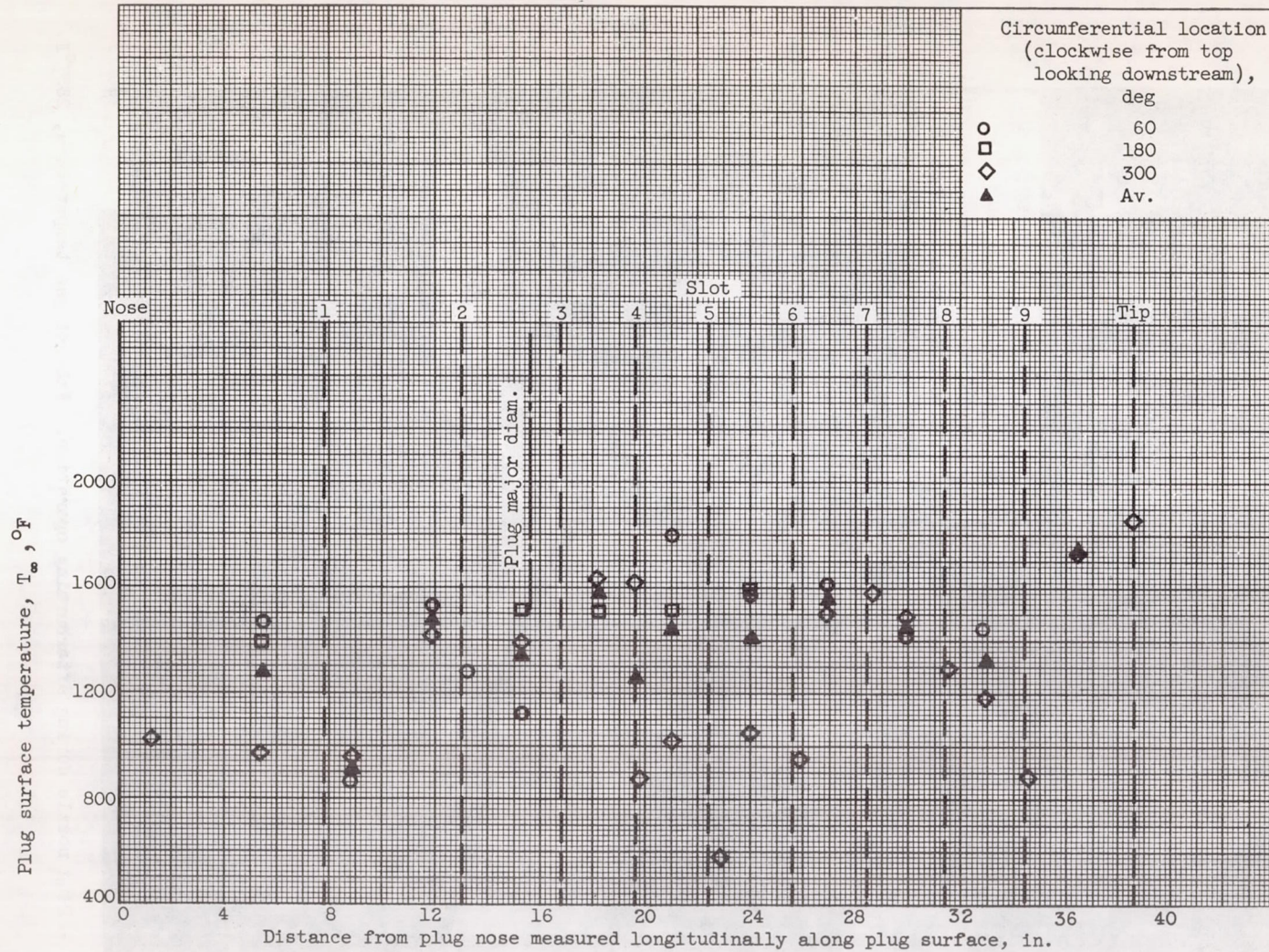
Figure 13. - Typical plug surface temperature distribution. Exhaust-gas temperature, 2585° F; weighted average plug surface temperature, 1437° F; cooling-air temperature, 86° F; total nozzle cooling air-flow, 3.97 percent of afterburner gas flow; afterburner total pressure, 3644 pounds per square foot absolute; pressure ratio, 1.76; afterburner gas flow, 83.19 pounds per second.
