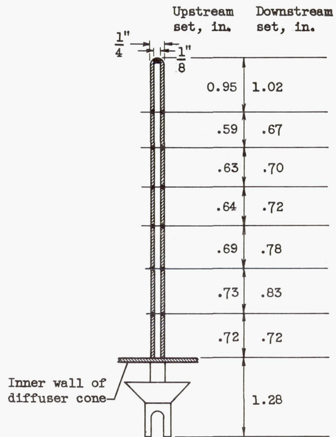
(b) Hole spacing of fuel spray bars.
