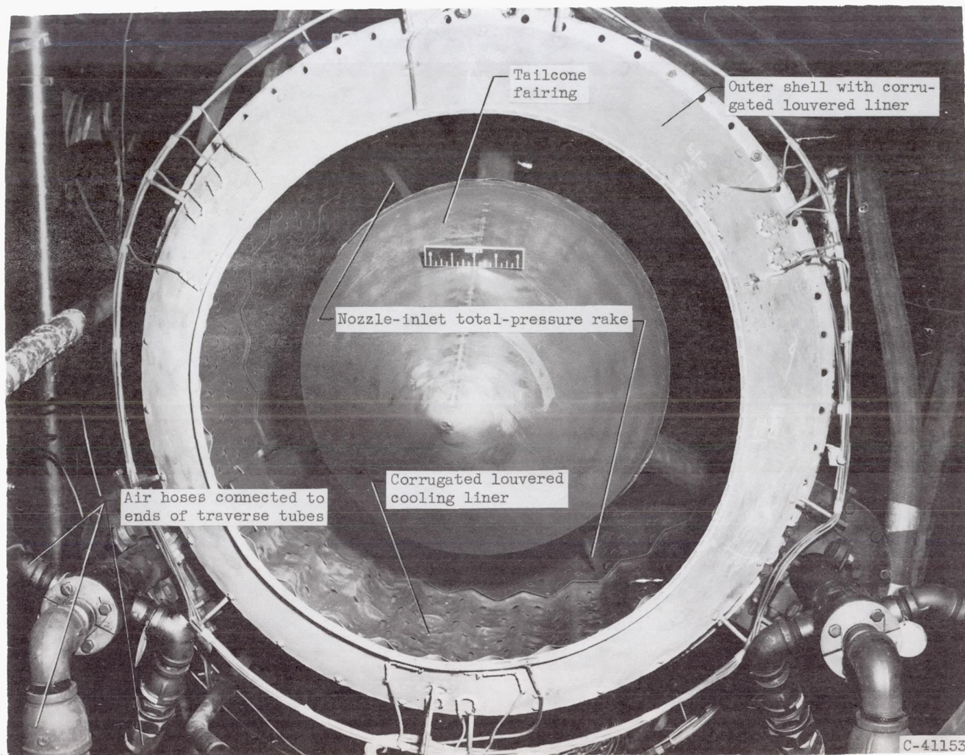
Figure 3. - Plug nozzle with smooth fairing covering tailcone
