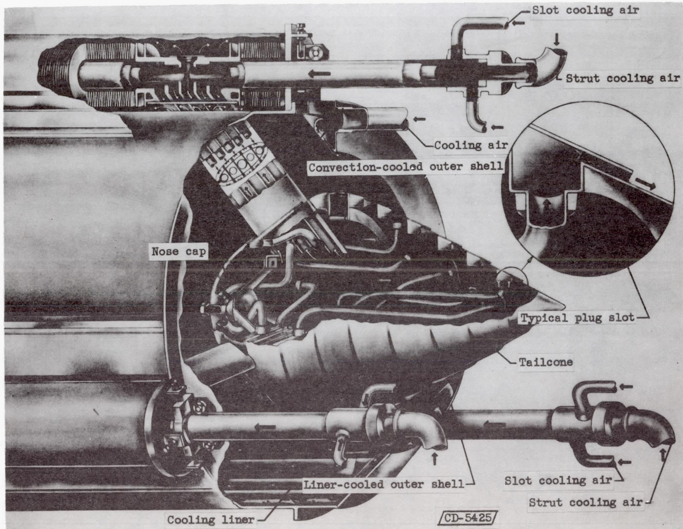
(b) Plug-nozzle cooling systems.
