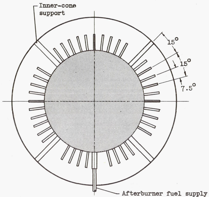
(a) Circumferential location of spray bars.
