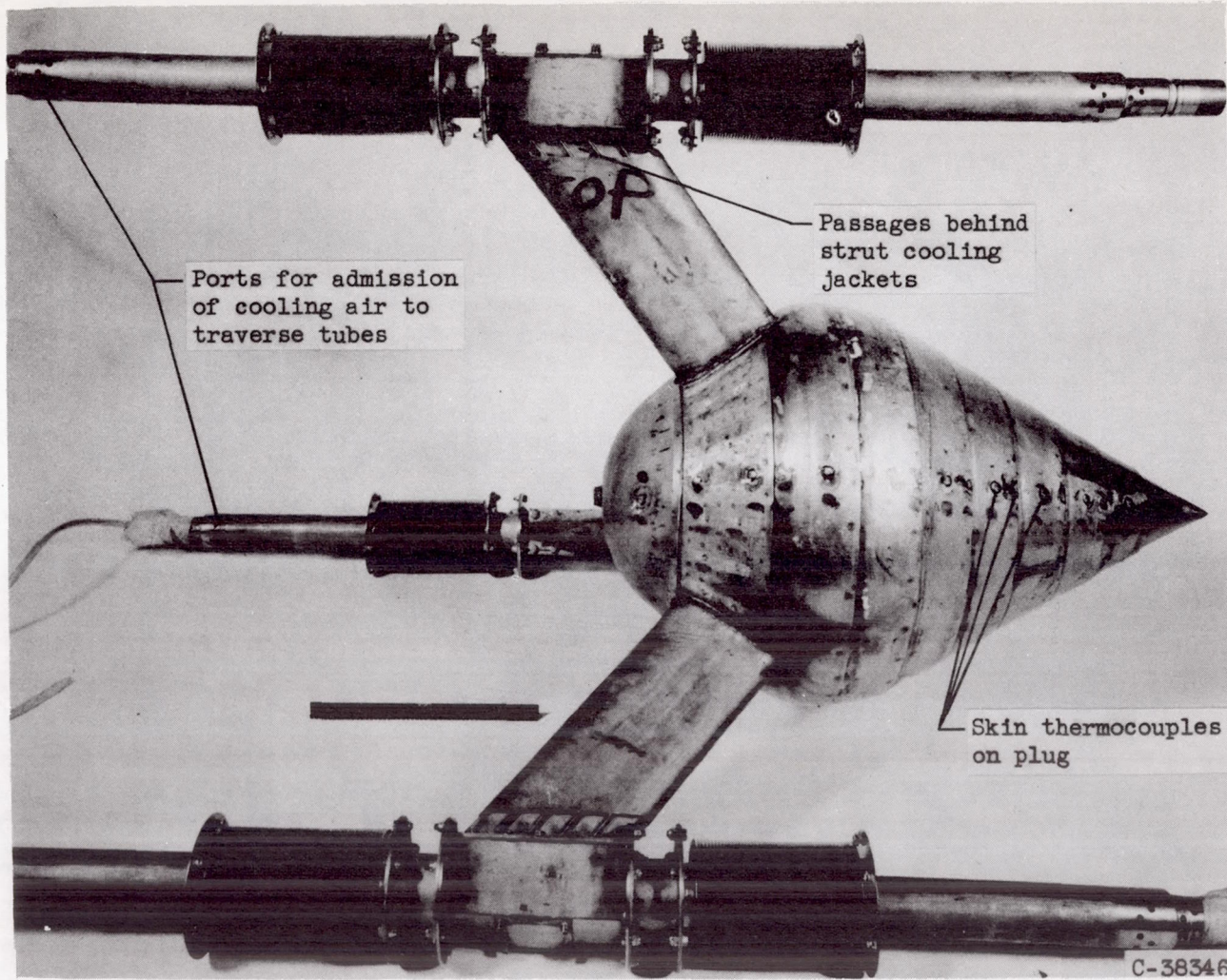
Figure 4. - Plug and traverse tube assembly.
