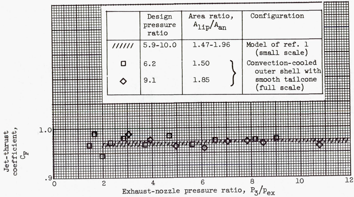
Figure 18. - Effect of nozzle pressure ratio on jet-thrust coefficient with smooth tailcone, no cooling airflow, and no afterburning.
