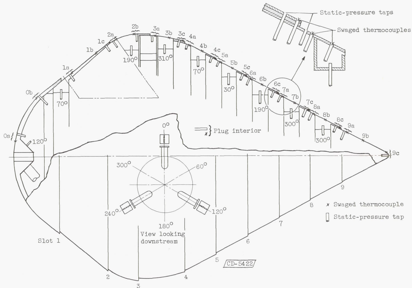
Figure 10. - Plug instrumentation and internal construction.
