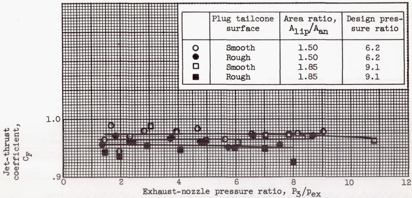
Figure 19. - Effect of plug tailcone roughness on jet-thrust coefficient with a convection-cooled outer shell, no cooling airflow, and no afterburning.
