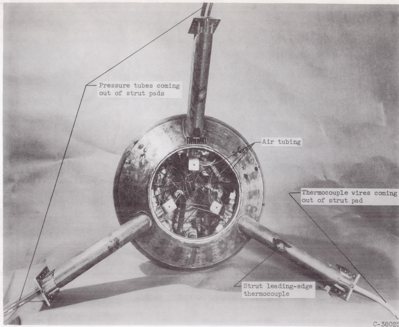
Figure 11. - Tail plug with nose cap removed to show instrumentation and cooling-air tubing.
