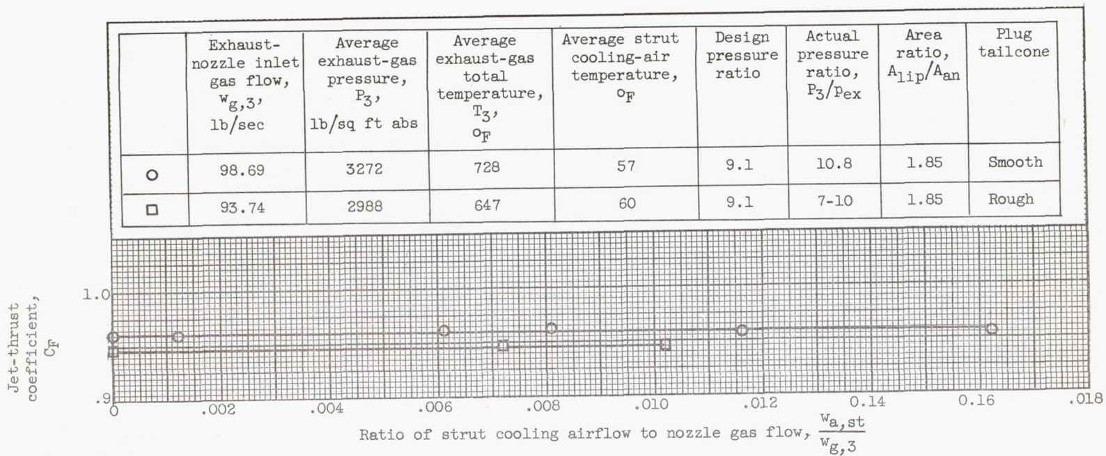
Figure 22. - Effect of strut cooling airflow on jet-thrust coefficient with forced-convection film-cooled outer shell and cooling air to struts only.
