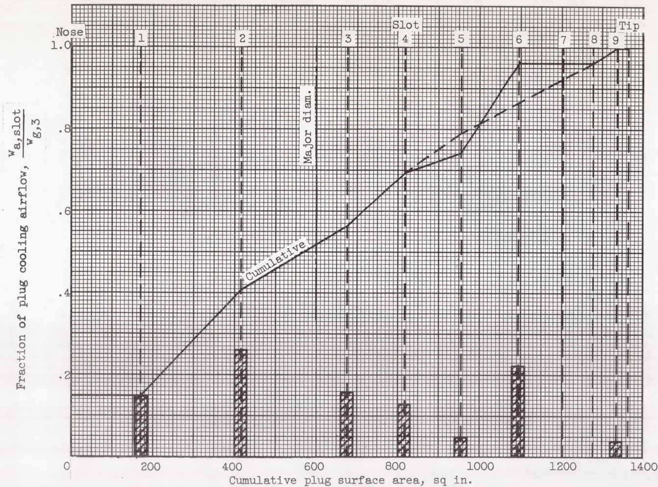
Figure 15. - Typical plug airflow distribution. Average plug surface temperature, 1437° F; exhaust-gas temperature, 2585° F; cooling-air temperature, 86° F; afterburner total pressure, 3644 pounds per square foot absolute; afterburner total-pressure ratio, 1.761; afterburner gas flow, 83.19 pounds per second; total nozzle cooling airflow, 3.87 percent of afterburner gas flow.
