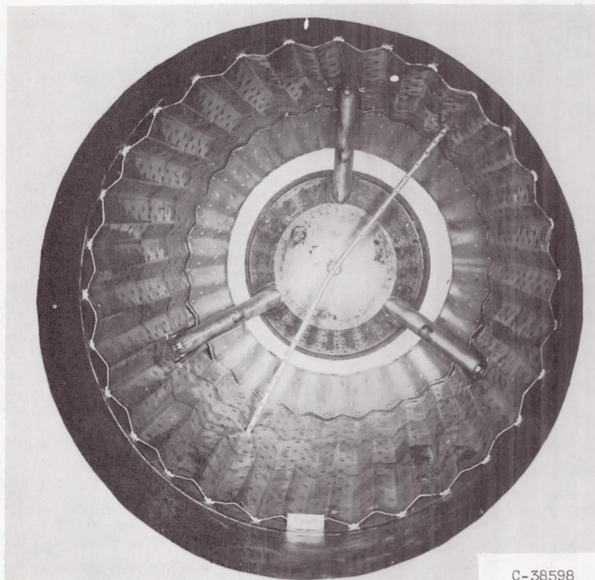
Figure 9. - Interior view of plug-nozzle afterburner showing antiscreech cooling liner.
