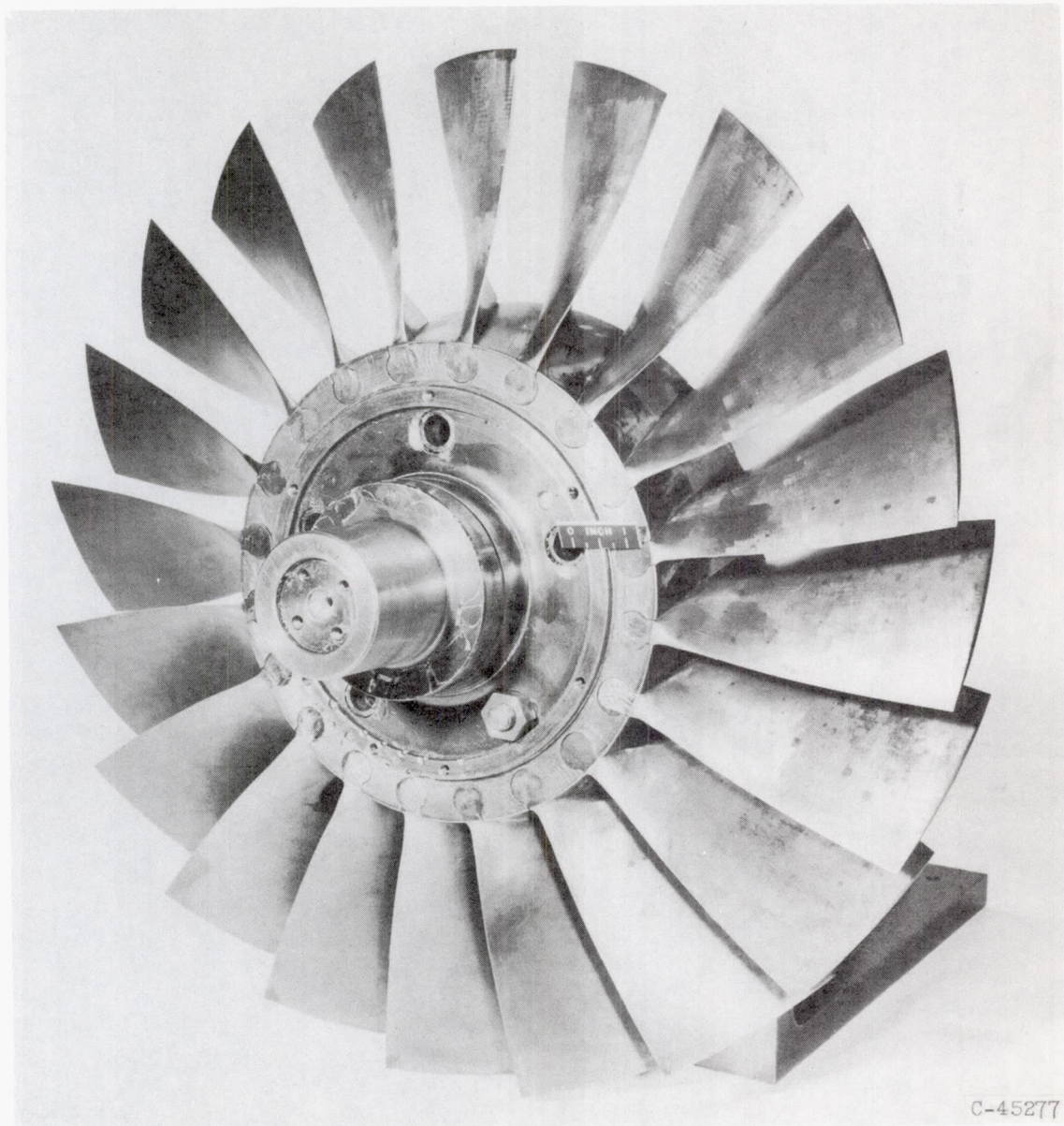
(b) First-stage rotor of medium-chord compressor of reference 6.
