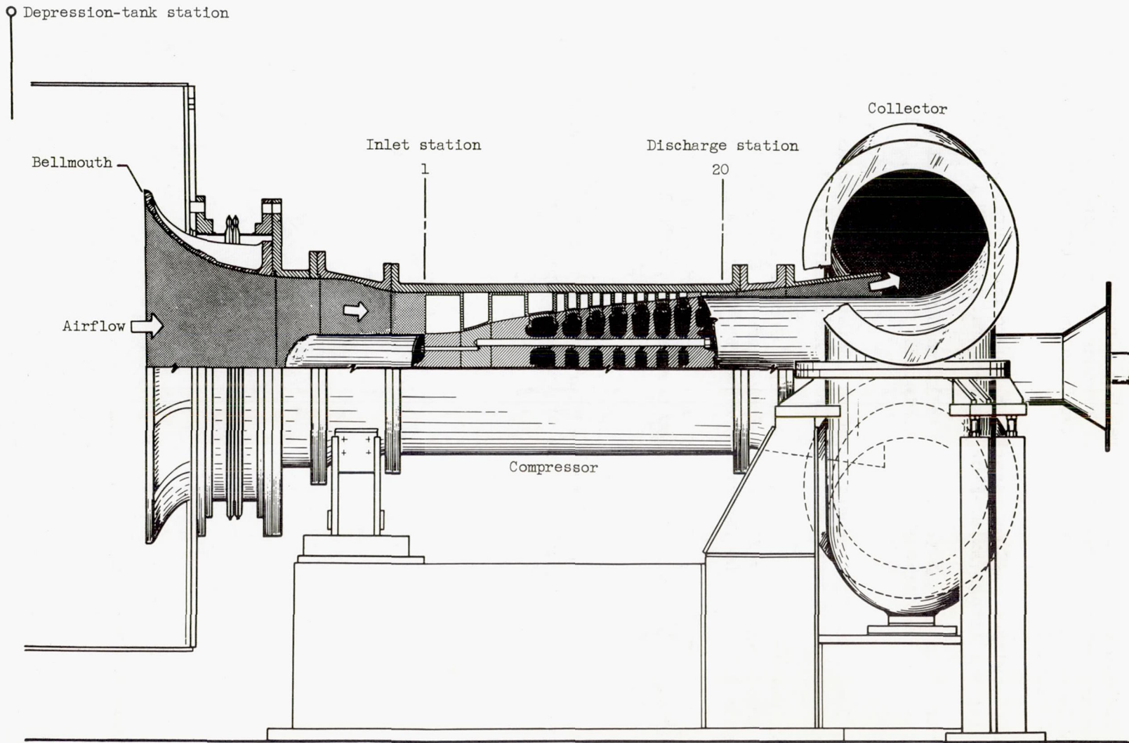
Figure 1. - Cross section of long-chord eight-stage axial-flow compressor, inlet bellmouth, and discharge collector.
