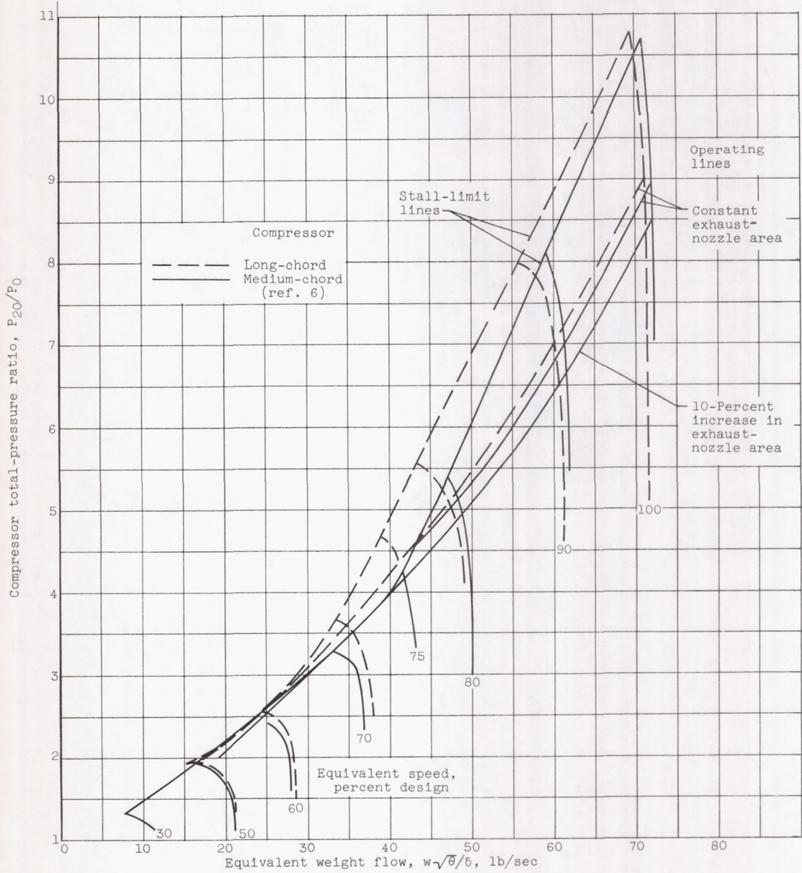
Figure 7. - Over-all performance map of long- and medium-chord compressors showing typical equilibrium operating lines.
