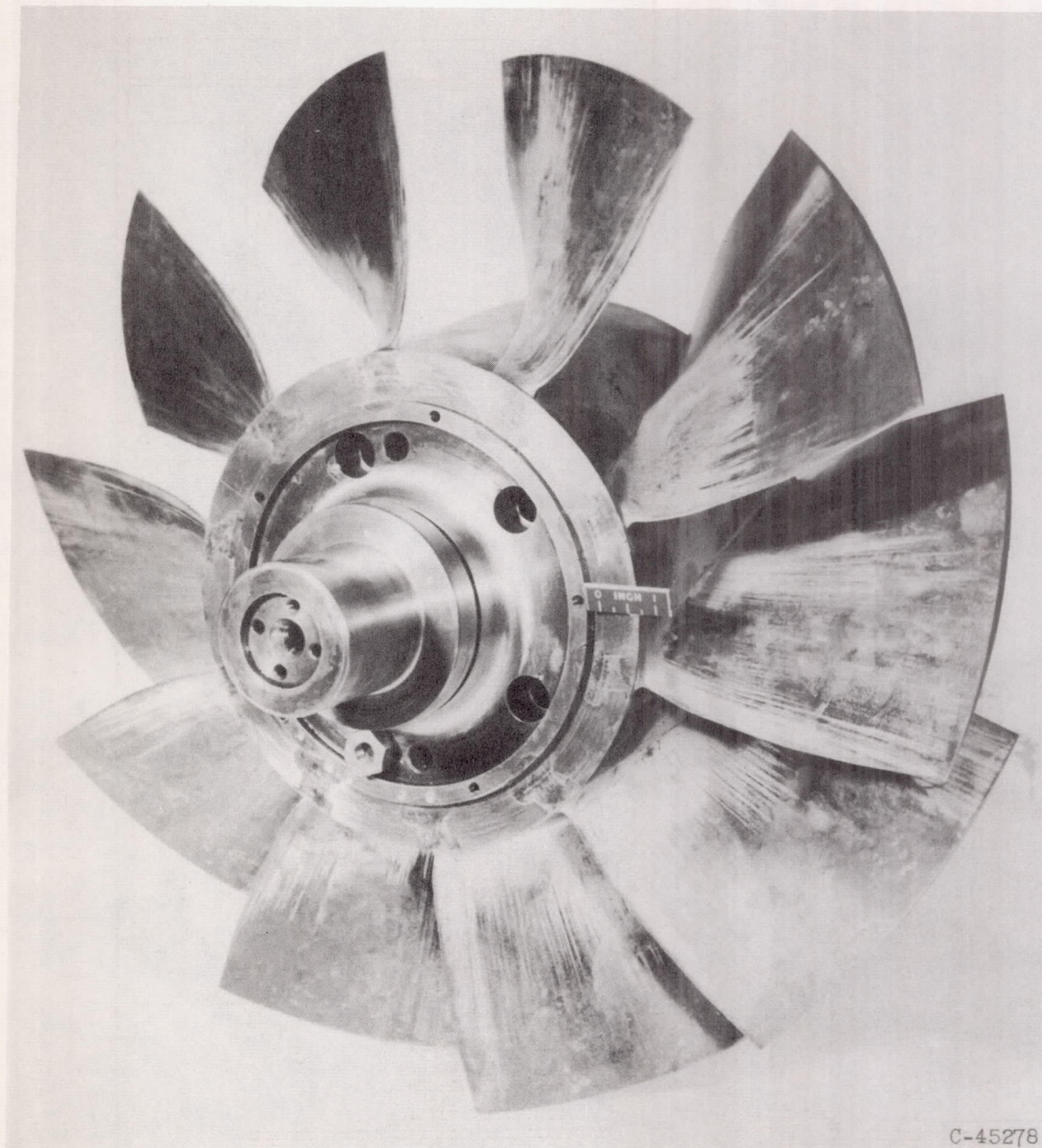
(a) First-stage rotor of long-chord compressor.
