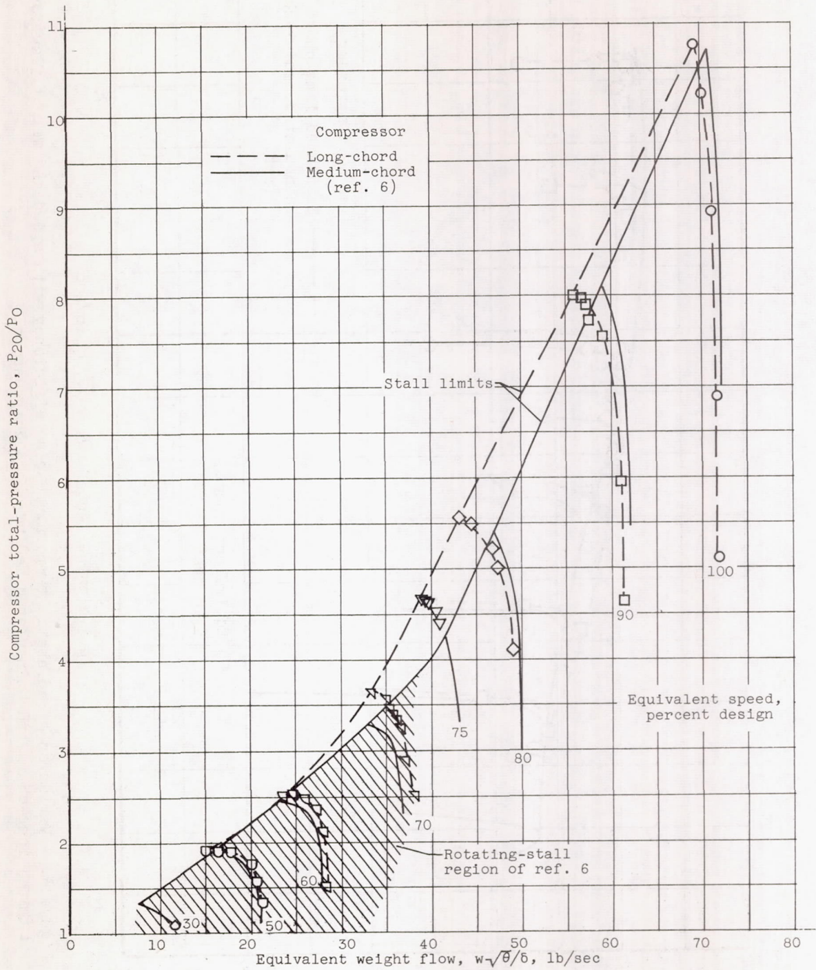
Figure 5. - Comparison of over-all performance characteristics of long- and medium-chord compressors.
