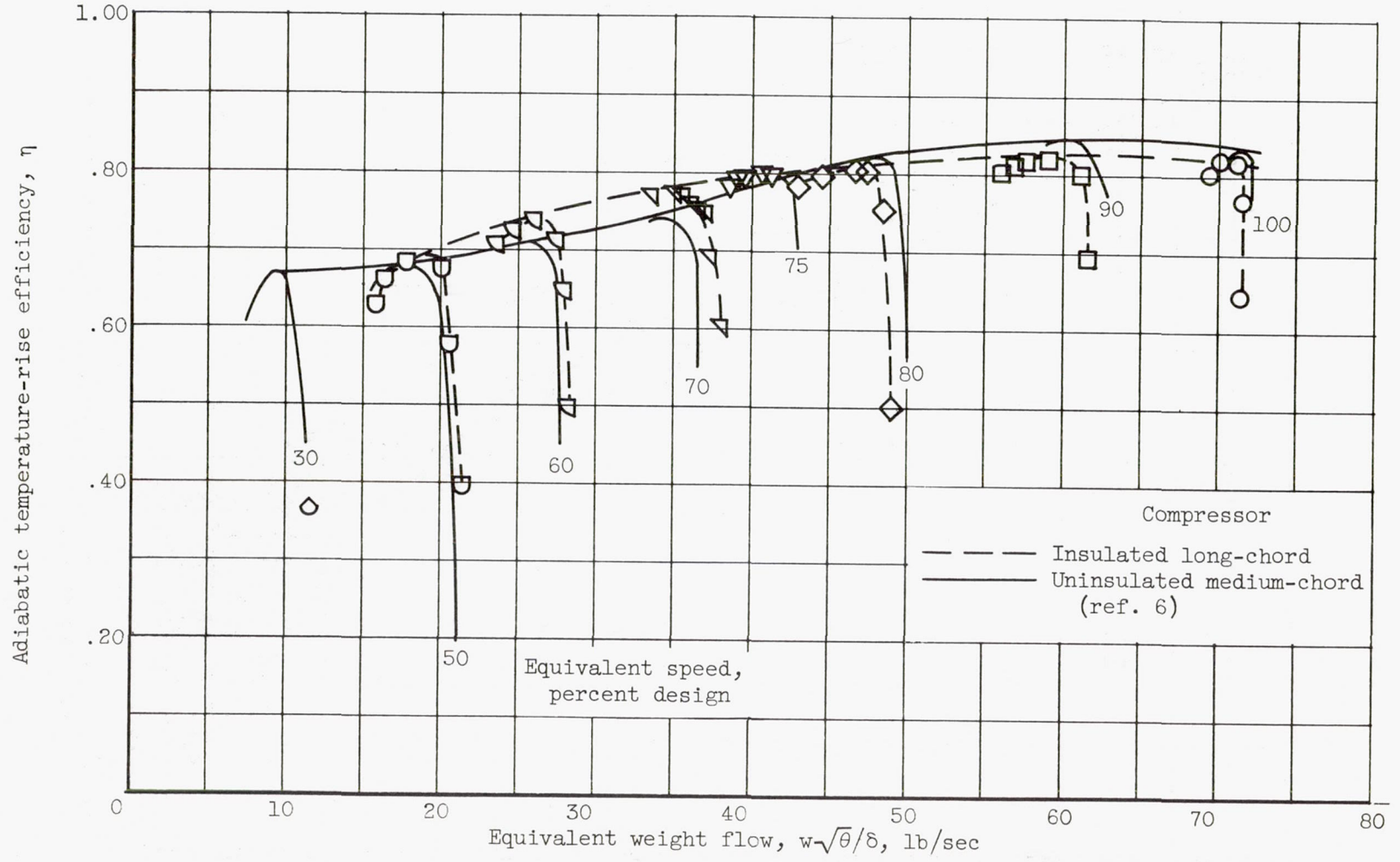
Figure 6. - Variation of adiabatic temperature-rise efficiency with speed and weight flow for insulated long-chord and uninsulated medium-chord compressors.
