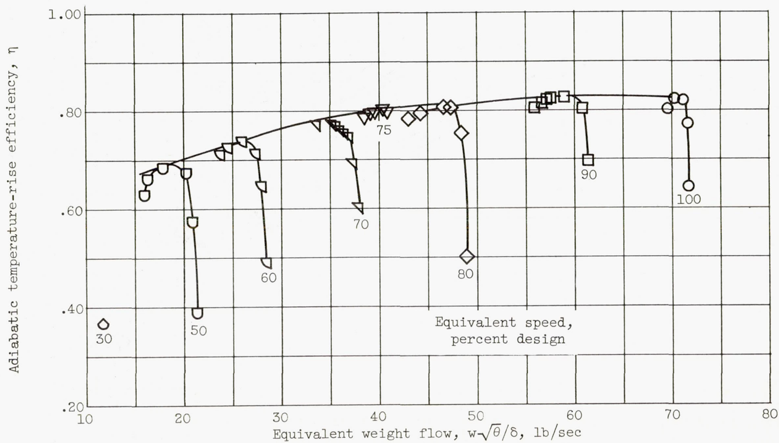
Figure 4. - Variation of adiabatic temperature-rise efficiency with speed and weight flow for long-chord compressor.
