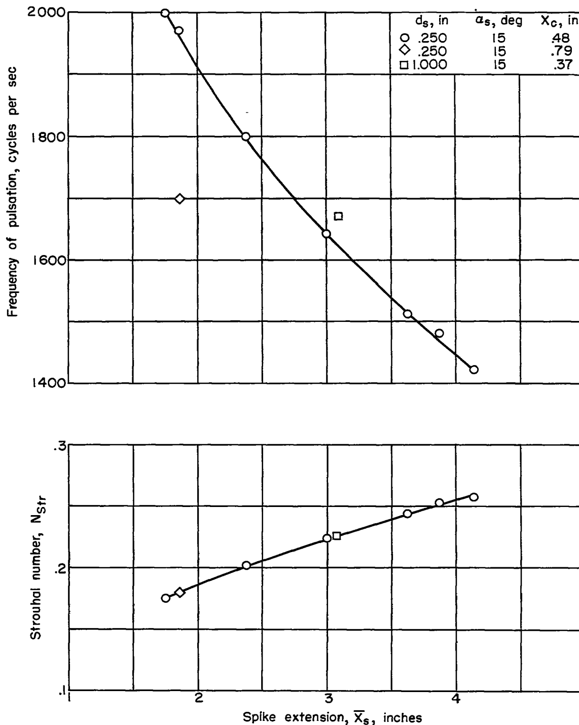
Figure 11.- Variation of frequency and Strouhal number with spike extension.
