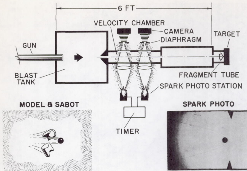
Figure 1.- Test apparatus.
