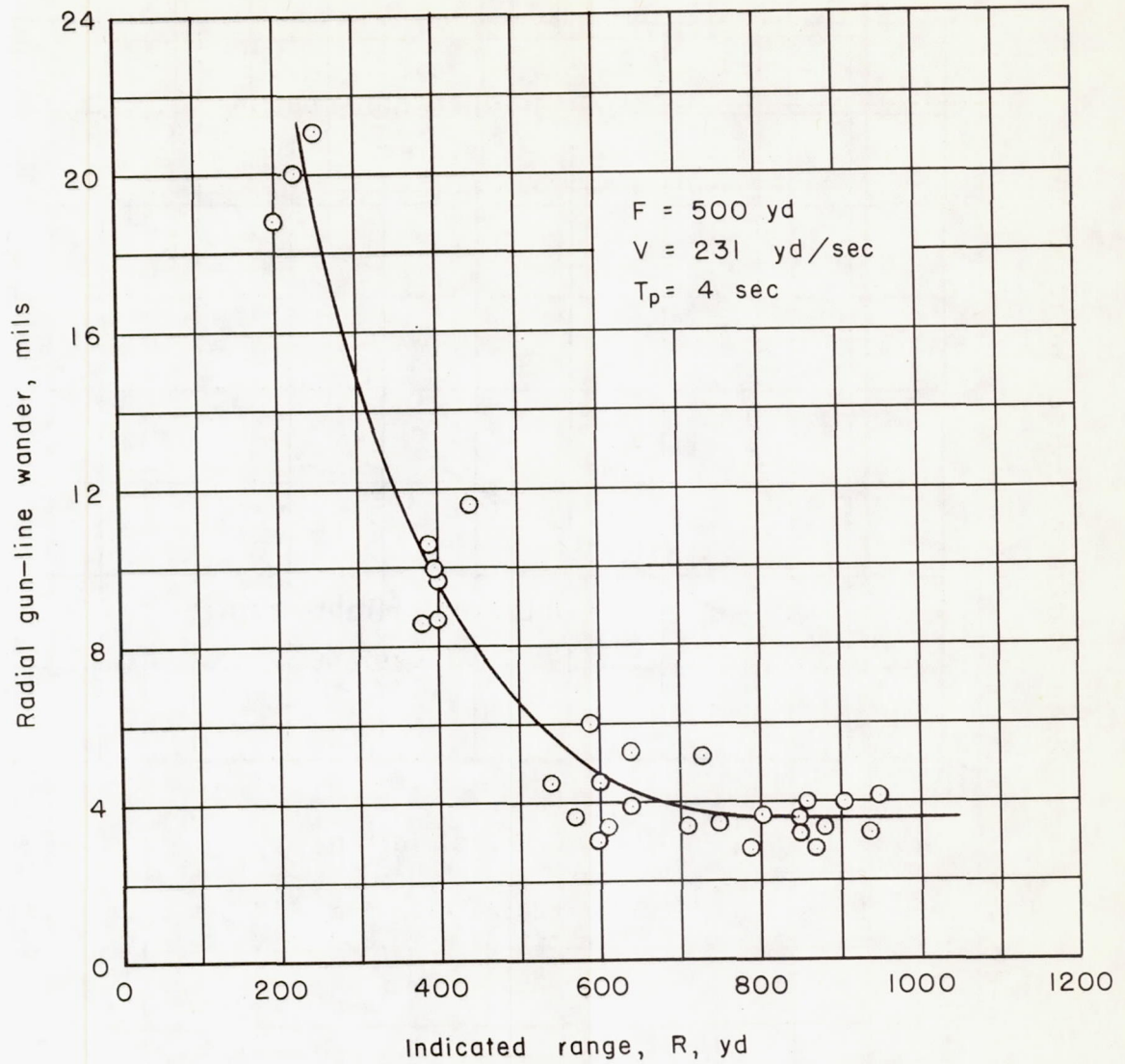
Figure 6.- Effect of range on the gun-line wander in a tail chase maneuver; K S = 24 yd/sec/in.
