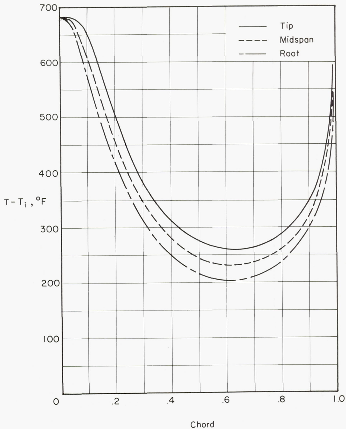
Figure 3.- Calculated chordwise temperature distribution at \tau = 2 seconds, and M = 2.0 .
