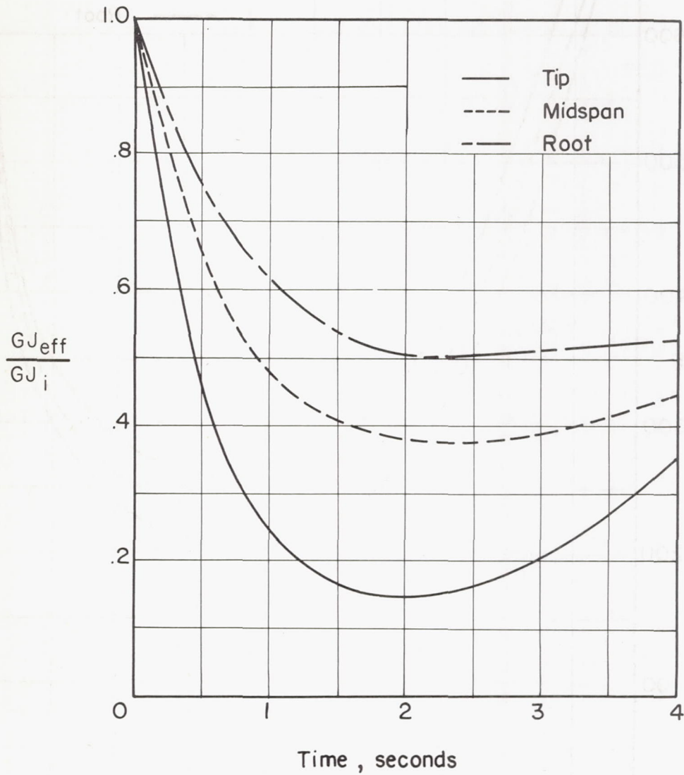
Figure 4.- Calculated loss in torsional stiffness against time at M = 2.0 . (Tip uncorrected for zero stress.)
