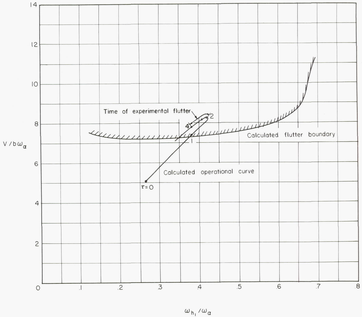
Figure 5.- Effect of aerodynamic heating on flutter.
