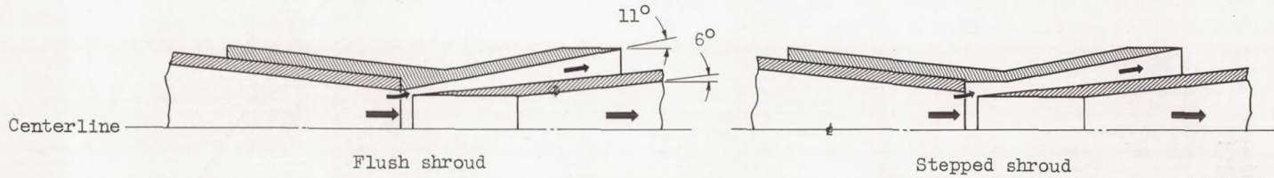
(b) Types of boundary-layer-bleed passages.
