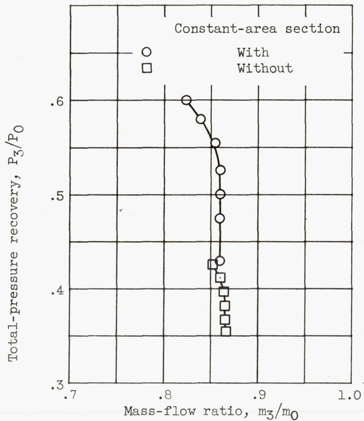
Figure 9. - Effect of constant-area section at throat of subsonic diffuser. Spacing ratio, S/d_1 , 0.144; diameter ratio, d_t/d_1 , 0.885.
