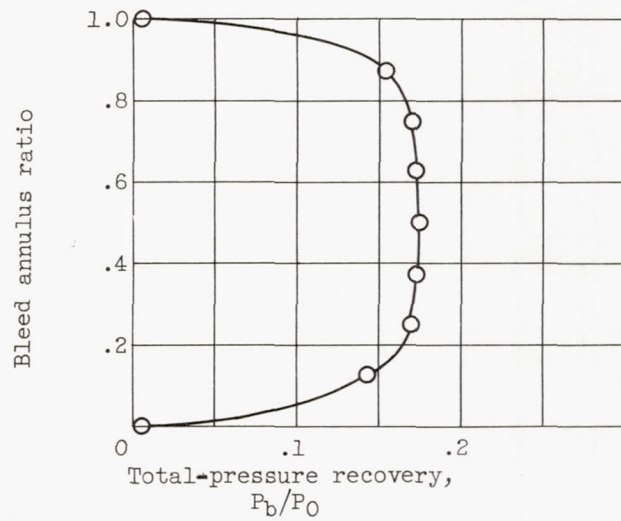
Figure 11. - Total-pressure-recovery profile for annular bleed duct. Spacing ratio, S/d_1 , 0.144; diameter ratio, d_t/d_1 , 0.885.
