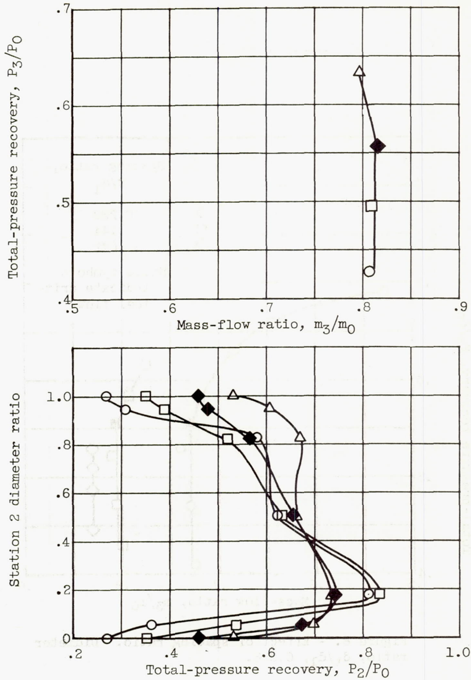
Figure 7. - Total-pressure-recovery profiles at station 2. Spacing ratio, S/d_1 , 0.144; diameter ratio, d_t/d_1 , 0.828.
