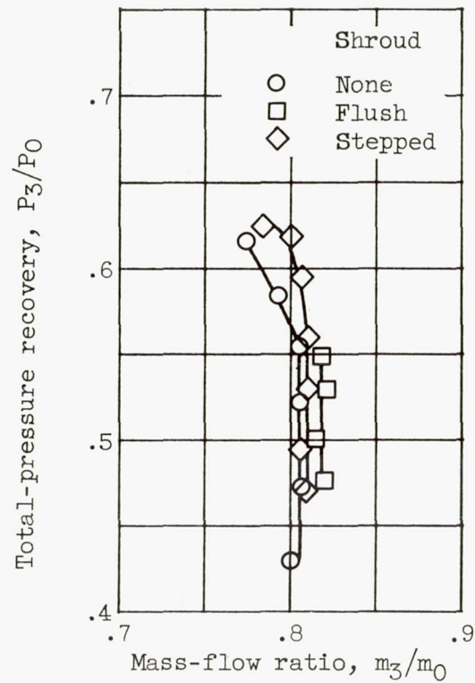
Figure 10. - Effect of shrouding inlet throat. Spacing ratio, S/d_1 , 0.144; diameter ratio, d_t/d_1 , 0.828.
