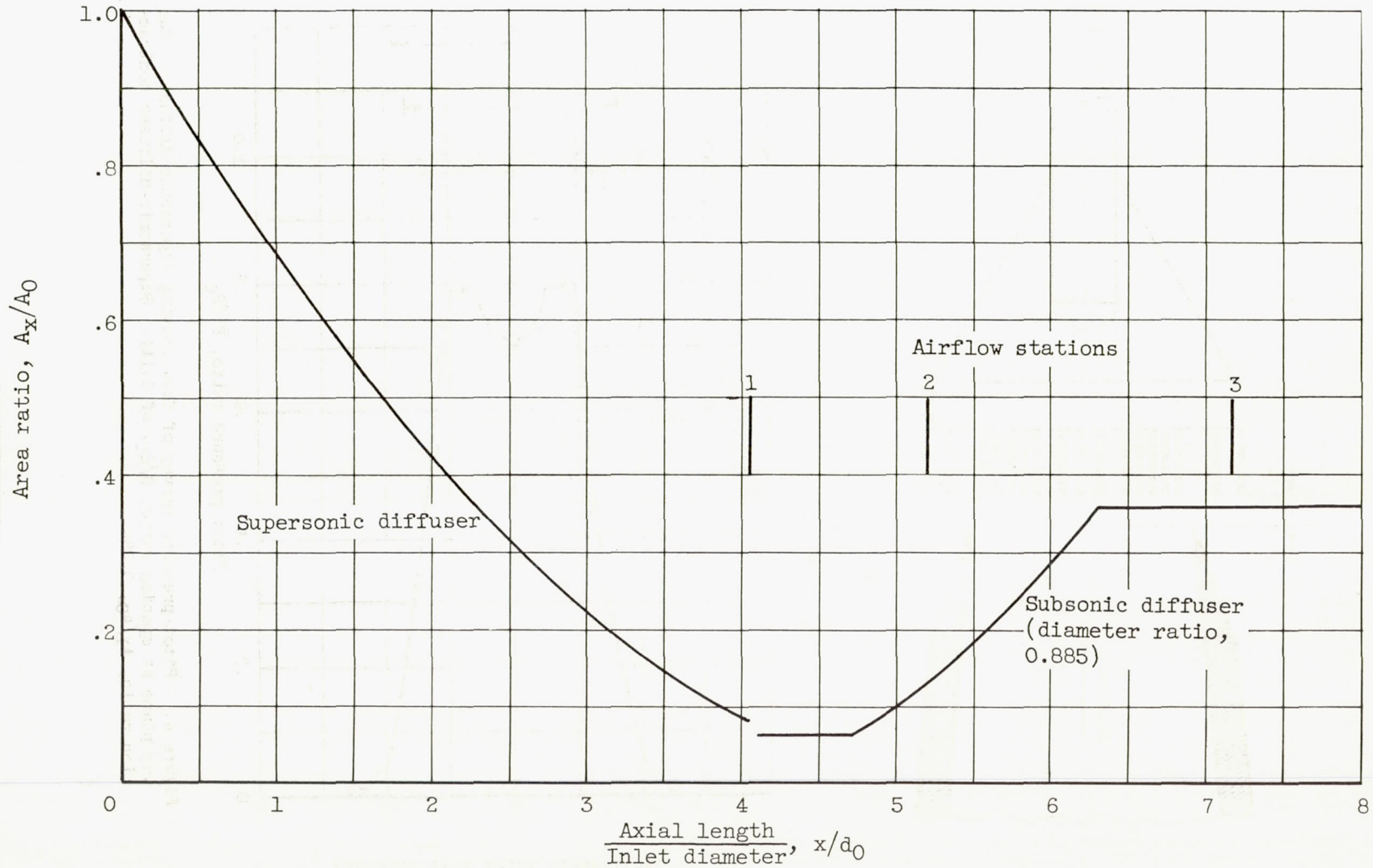
Figure 3. - Internal area variation. Inlet capture area, A_0 , 28.3 square inches; inlet diameter, d_0 , 6 inches.
