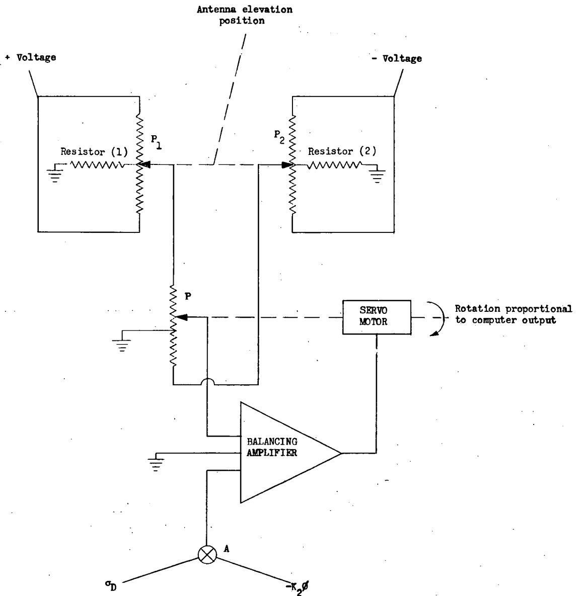
Figure 4.- Schematic diagram of bank-angle-error computer.
