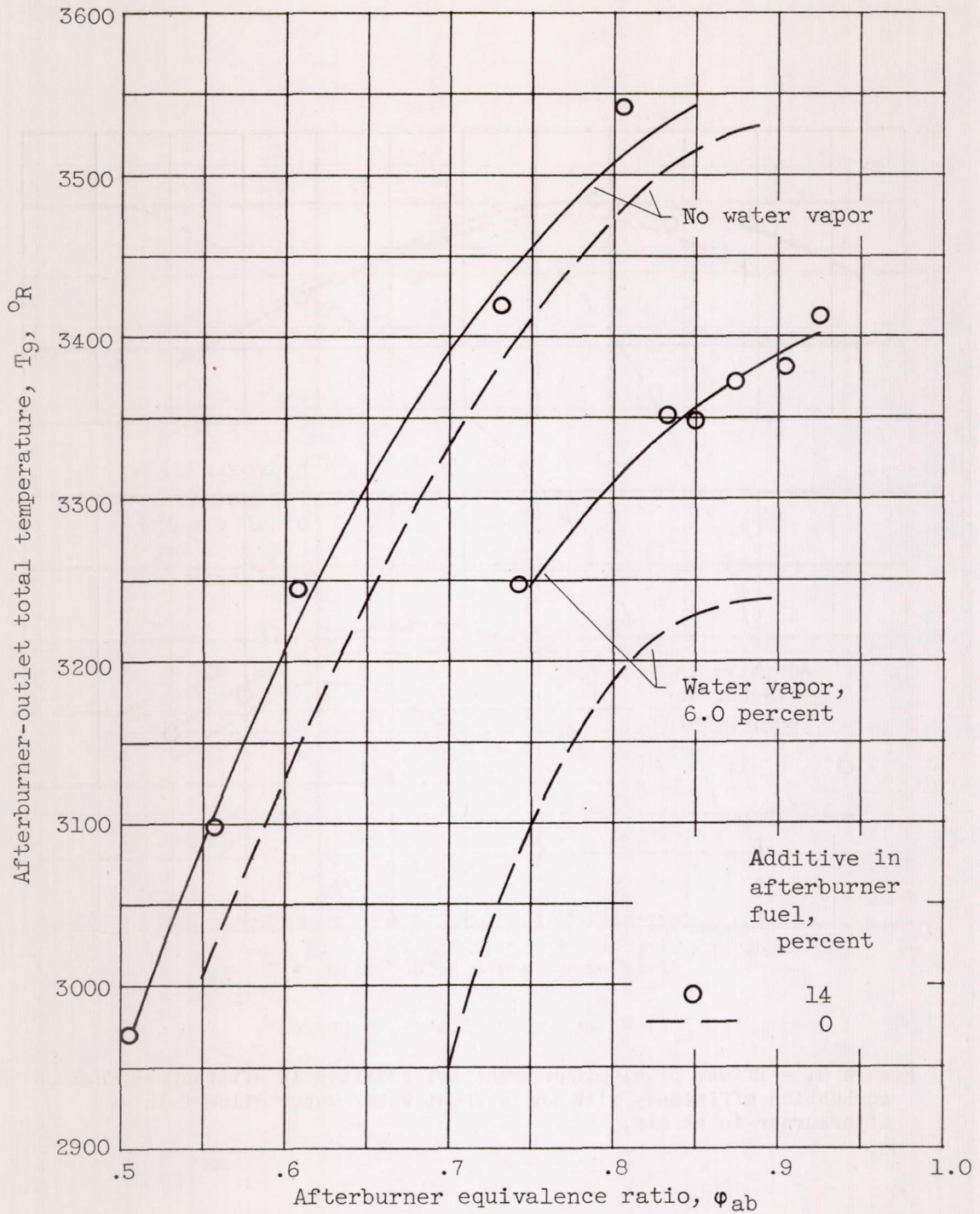
Figure 9. - Effect of aluminum trimethyl additive in afterburner fuel on afterburner-outlet total temperature with and without water vapor diluent in afterburner-inlet air.
