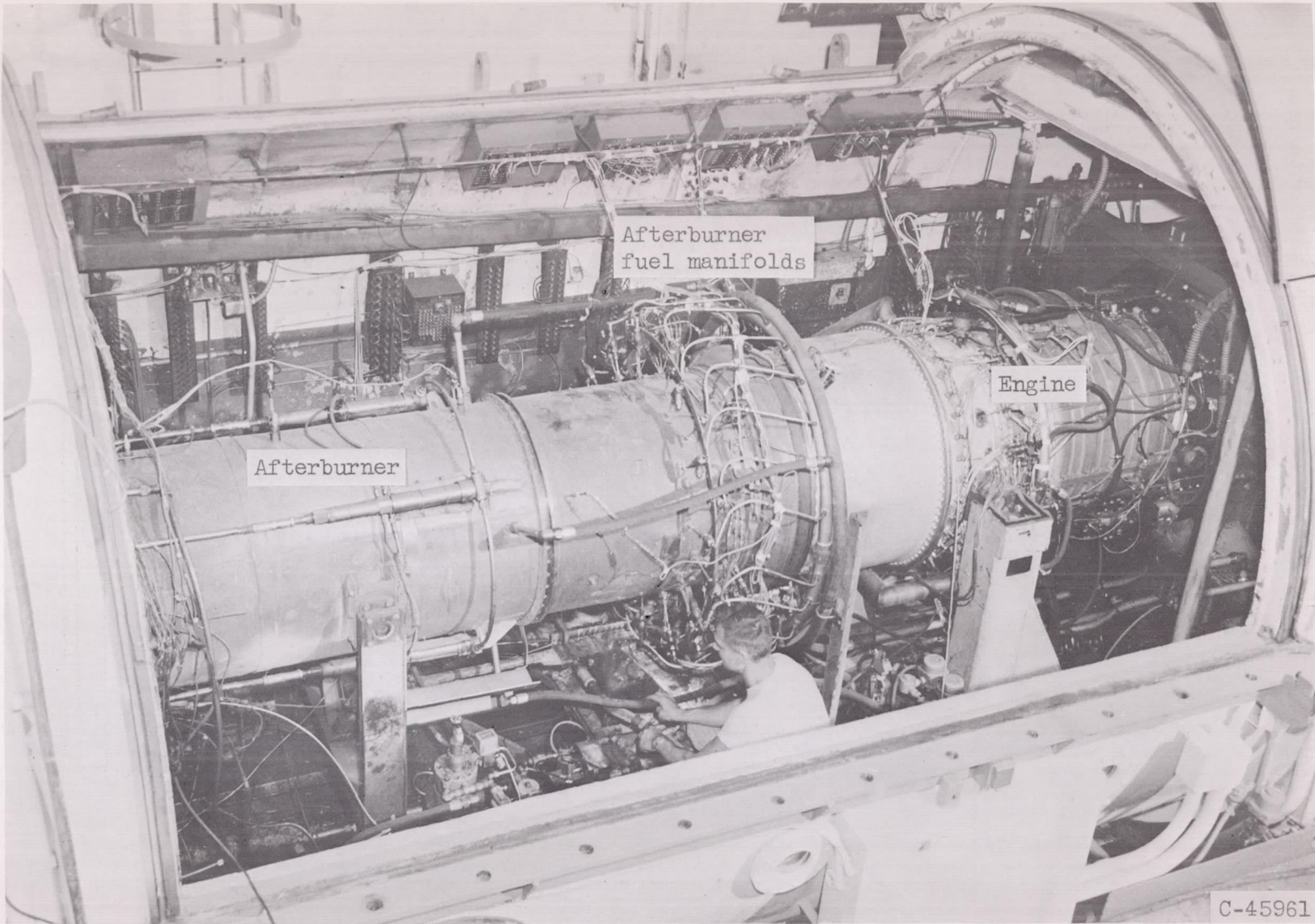
Figure 1. - Installation of engine with afterburner in altitude test chamber.
