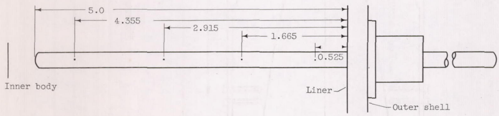
(b) Spray bar.
