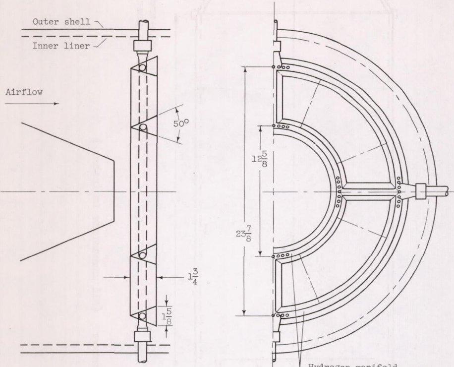
(a) Flameholder.
