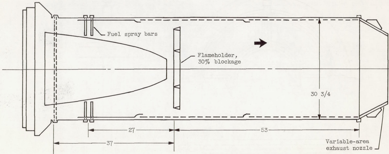
Figure 2. - Afterburner. (All dimensions in inches.)
