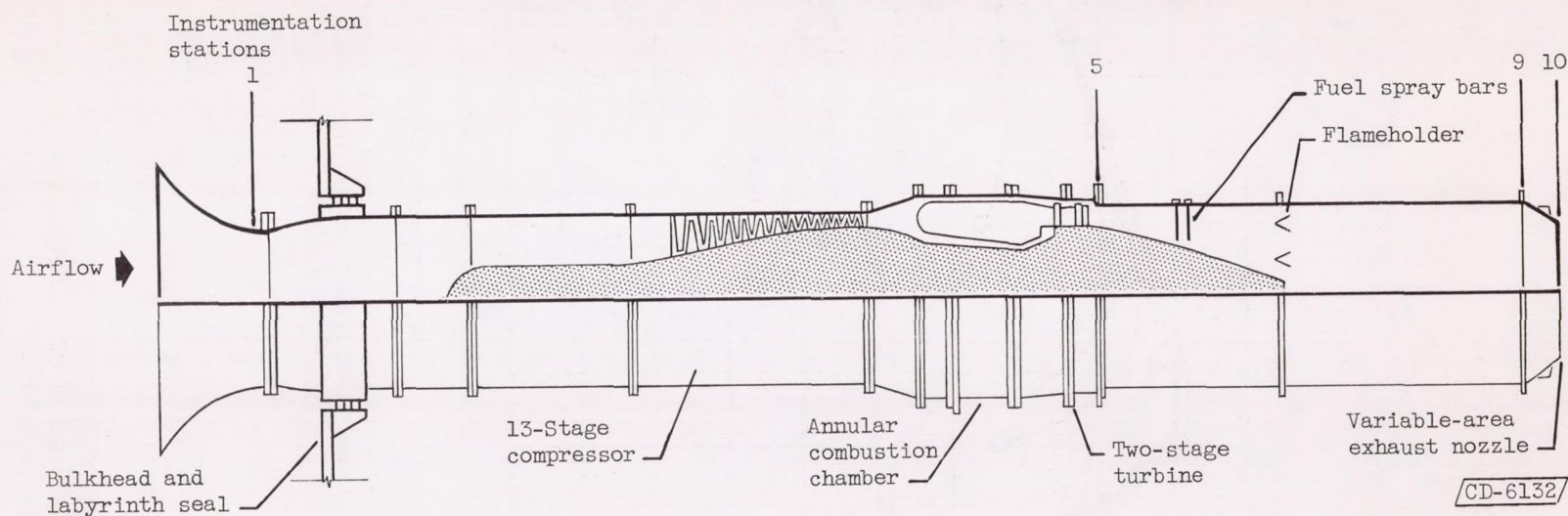
Figure 5. - Engine and afterburner showing location of instrumentation stations.
