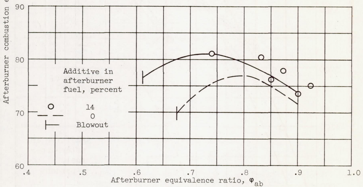
(b) Water vapor diluent, 6 percent.
