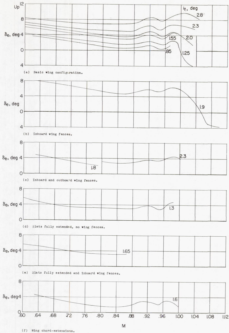
Figure 19.- Effect of several wing modifications on the variation with Mach number of the elevator deflection required to trim the Douglas D-558-II research airplane. h_p = 35,000 feet; W = 13,000 pounds; a_n = 1 .
