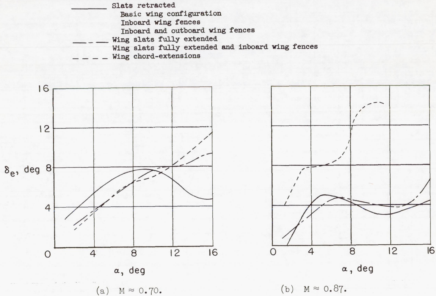
Figure 15.- Effect of several wing modifications on the apparent stick-fixed stability characteristics of the D-558-II airplane at two representative Mach numbers. ( \delta_e values corrected to zero pitching acceleration.)
