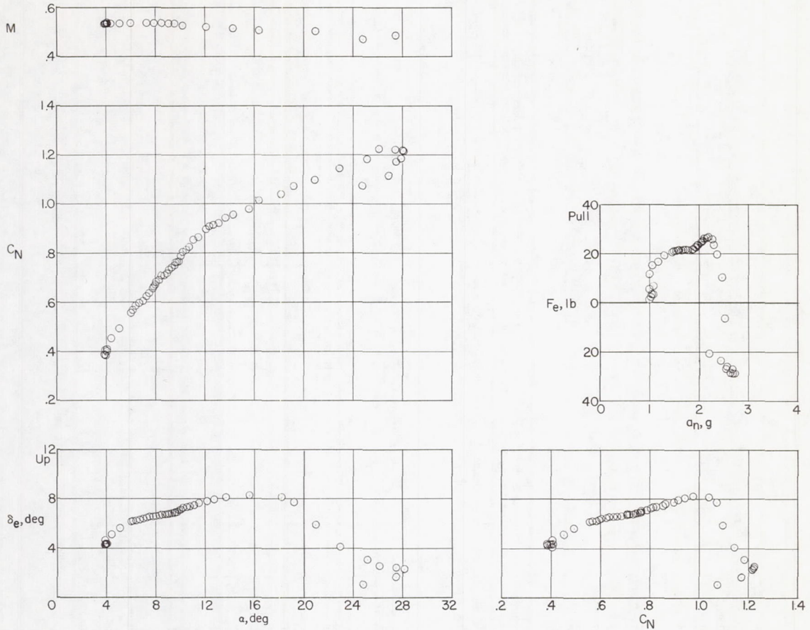
(a) h_p \approx 23,300 feet; i_t = 2.2^\circ ; center of gravity at 0.259\bar{c} ; slats retracted.
