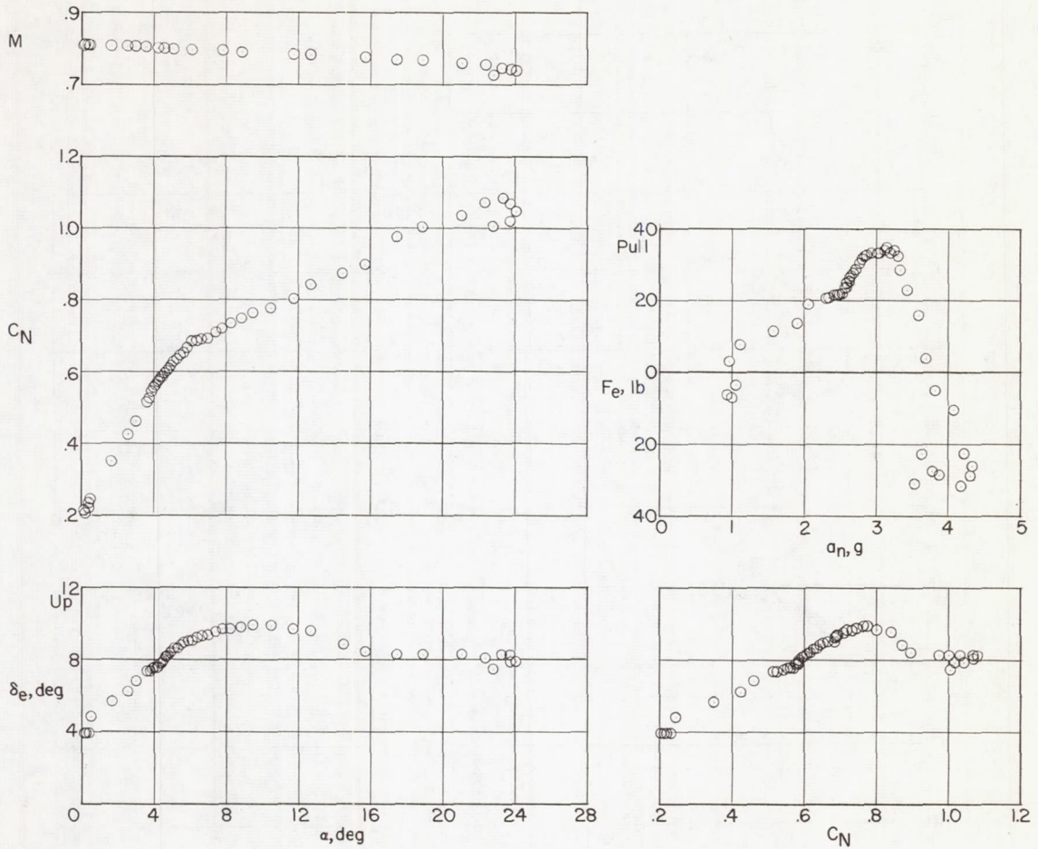
(c) h_p \approx 28,700 feet; i_t = 2.0^\circ ; center of gravity at 0.253\bar{c} ; slats retracted.
