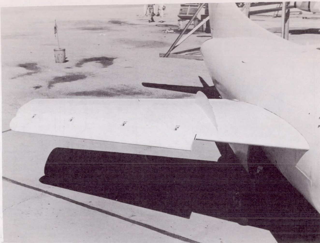
Figure 6.- Photograph of right wing of D-558-II airplane showing slat in fully extended position and inboard fence on wing.
