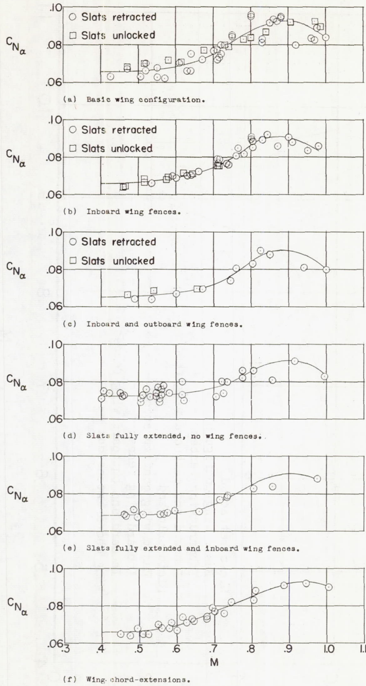
Figure 17.- Effect of several wing modifications on the variation of C_{N_\alpha} with Mach number for the Douglas D-558-II research airplane.
