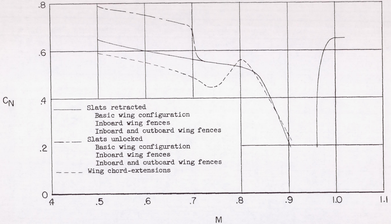
Figure 16.- Effect of wing modifications on buffet boundary of the D-558-II airplane.
