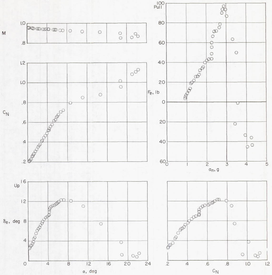
(c) h_p \approx 35,600 feet; i_t = 2.1^\circ ; center of gravity at 0.248\bar{c} ; slats retracted.
