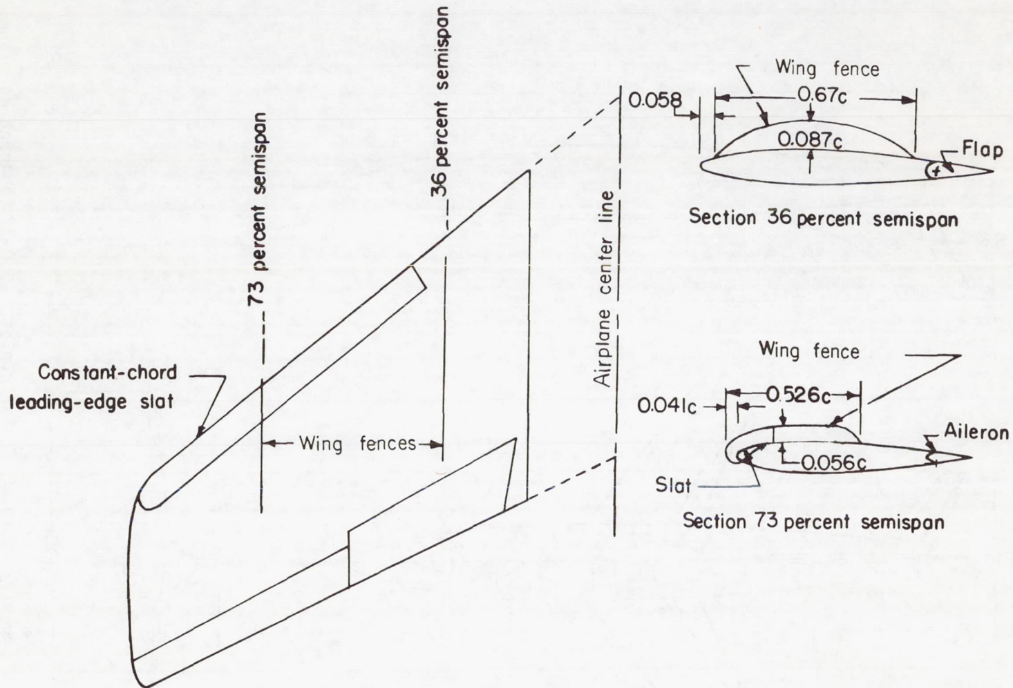
Figure 3.- Plan form and sections of the wing of the D-558-II airplane showing the location and shape of wing fences (stall-control vanes) used in the investigation.
