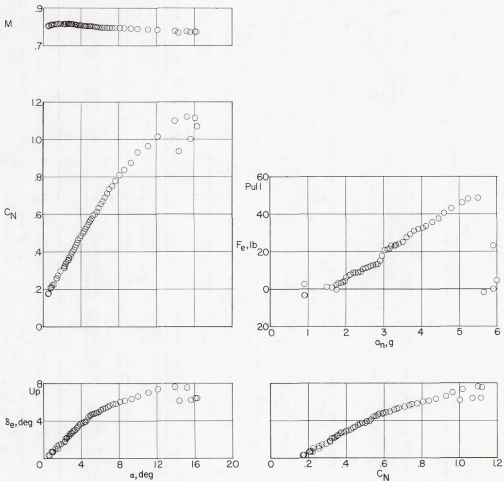
(c) h_p \approx 23,000 feet; i_t = 1.3^\circ ; center of gravity at 0.262\bar{c} .
