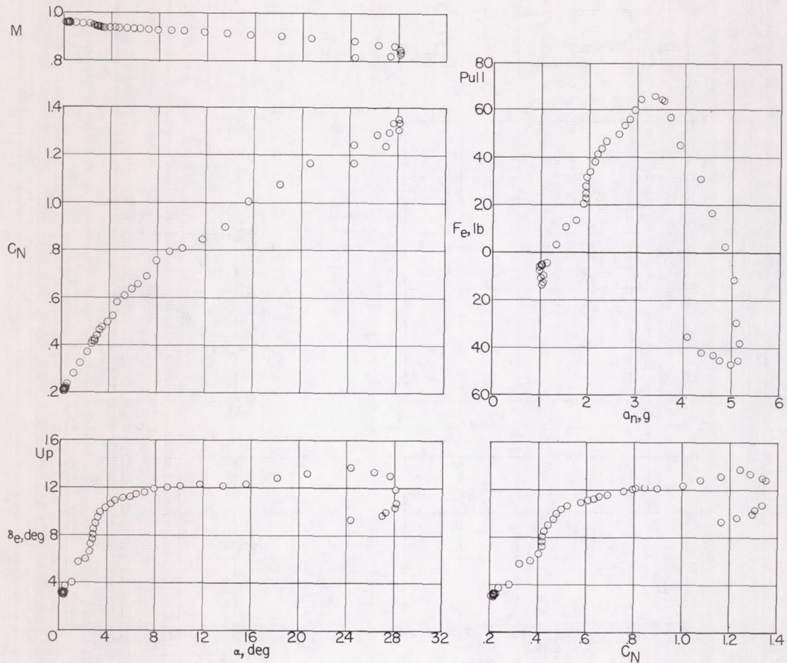
(d) h_p \approx 34,800 feet; i_t = 1.6^\circ ; center of gravity at 0.261\bar{c} ; slats retracted.
