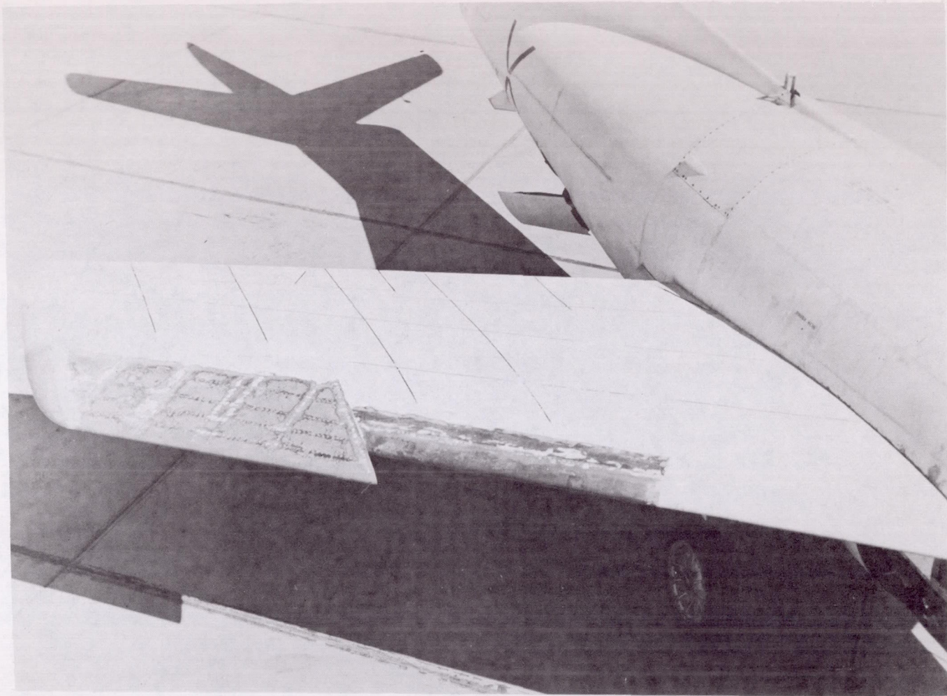
Figure 8.- Photograph of the wing of the D-558-II airplane showing the wing leading-edge chord-extension configuration.
