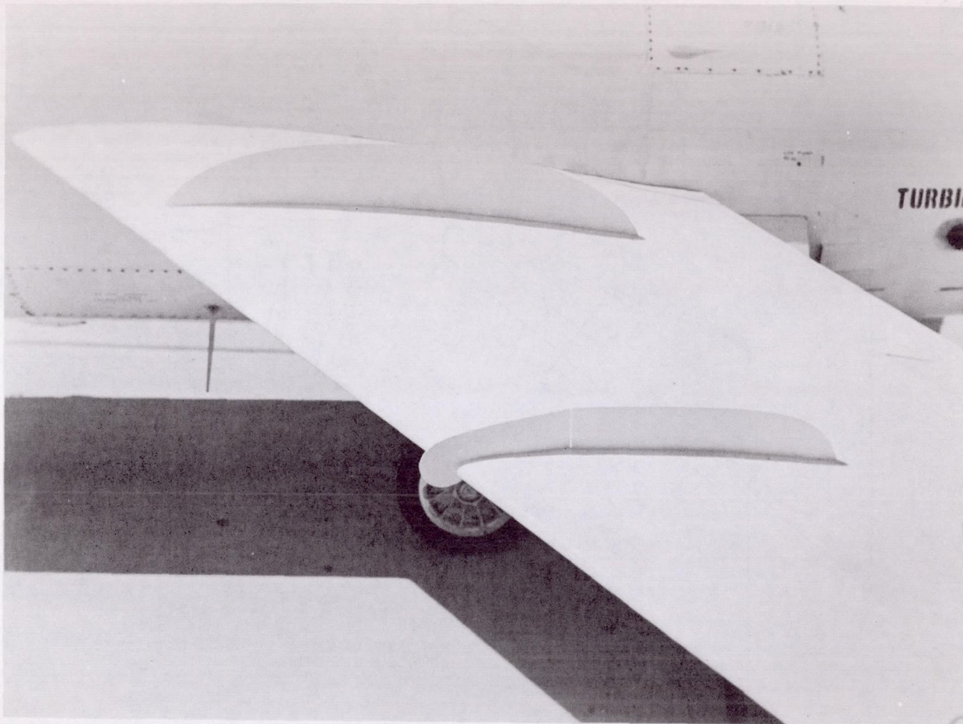
Figure 4.- Photograph of the D-558-II wing, showing the inboard and outboard fences (stall-control vanes) on the wing.
