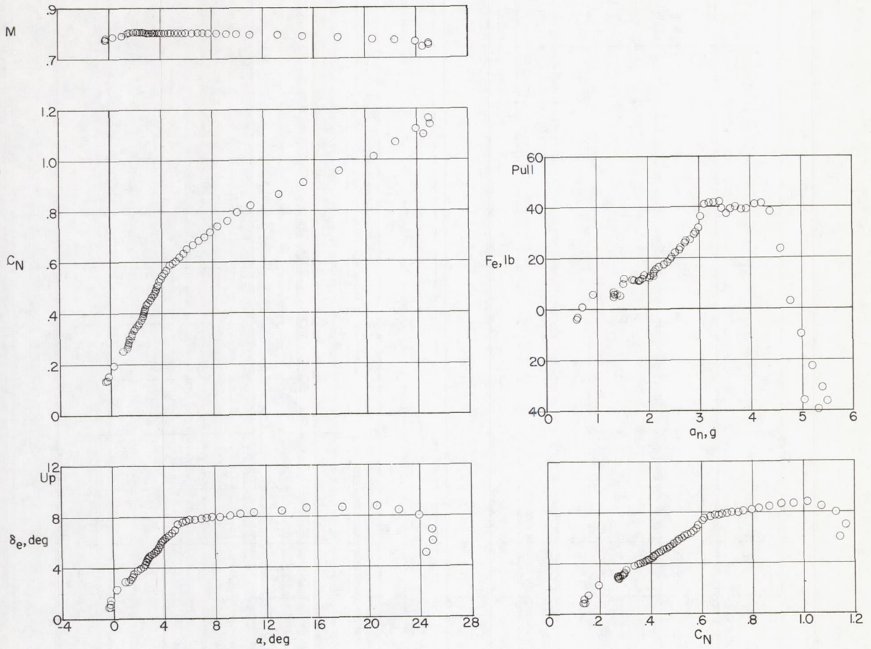
(c) h_p \approx 25,900 feet; i_t = 2.1^\circ ; center of gravity at 0.249\bar{c} ; slats retracted.
