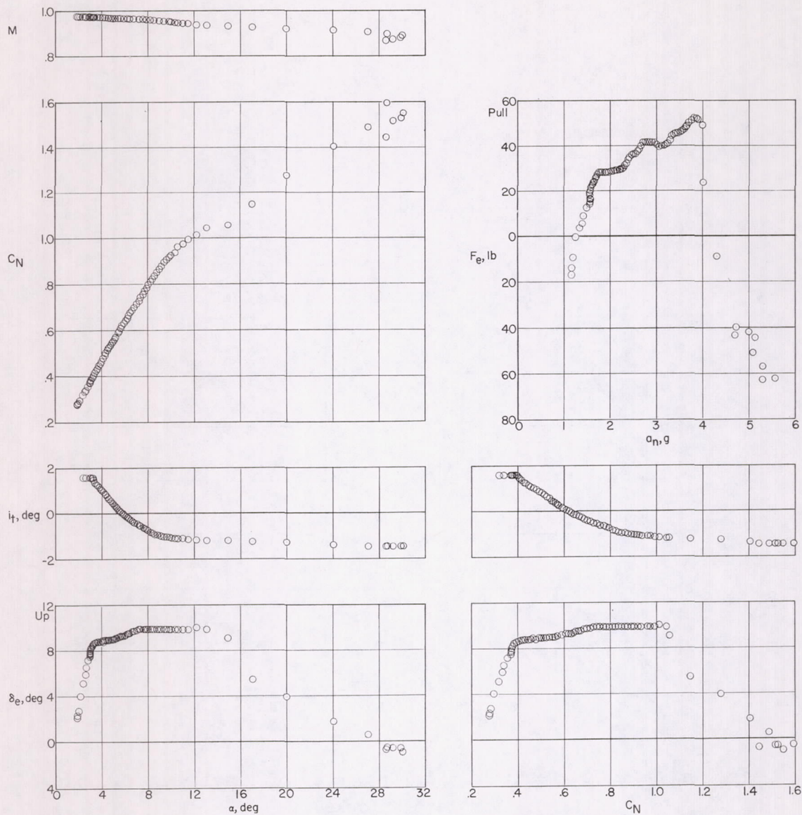
(d) h_p \approx 37,200 feet; center of gravity at 0.272\bar{c} ; slats retracted.
