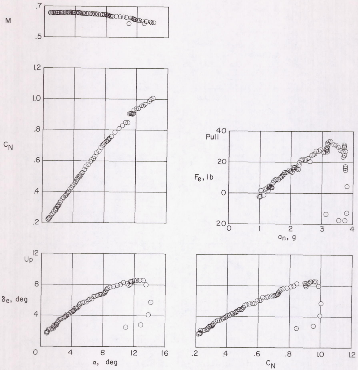
(d) h_p \approx 20,200 feet; i_t = 2.3^\circ ; center of gravity at 0.266\bar{c} ; slats unlocked.
