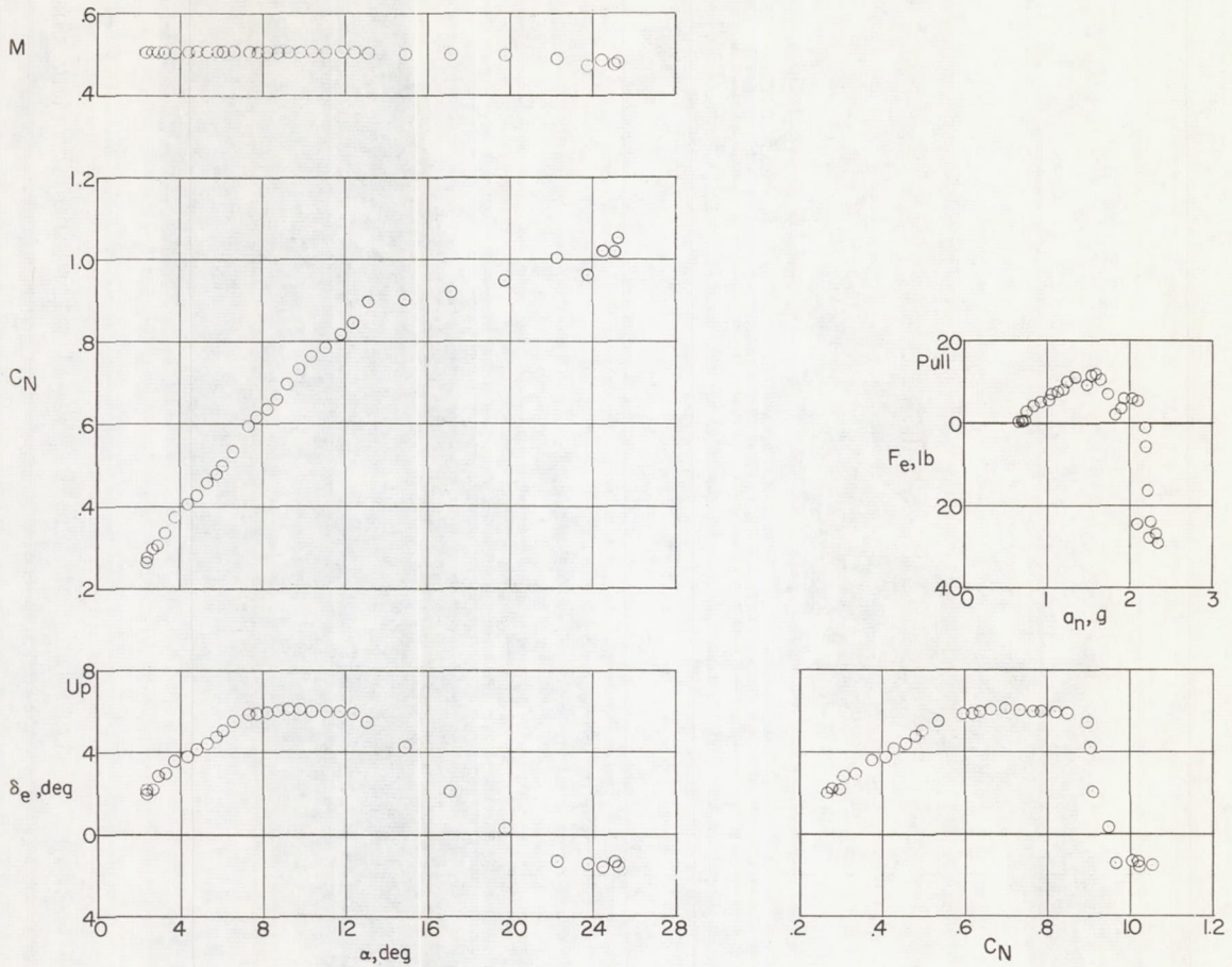
(a) h_p \approx 22,000 feet; i_t = 1.6^\circ ; center of gravity at 0.268\bar{c} ; slats retracted.
