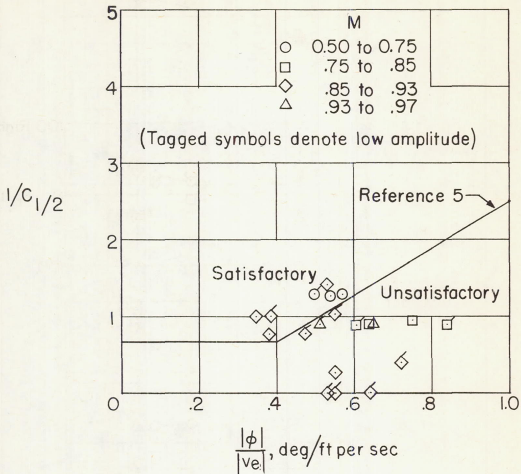
Figure 5.- Comparison of damping characteristics with the Military Specification.
