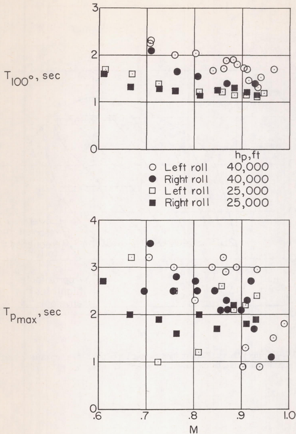
Figure 12.- Variation of time to bank to 100° and time to bank to maximum rolling velocity with Mach number for full-deflection rolls.
