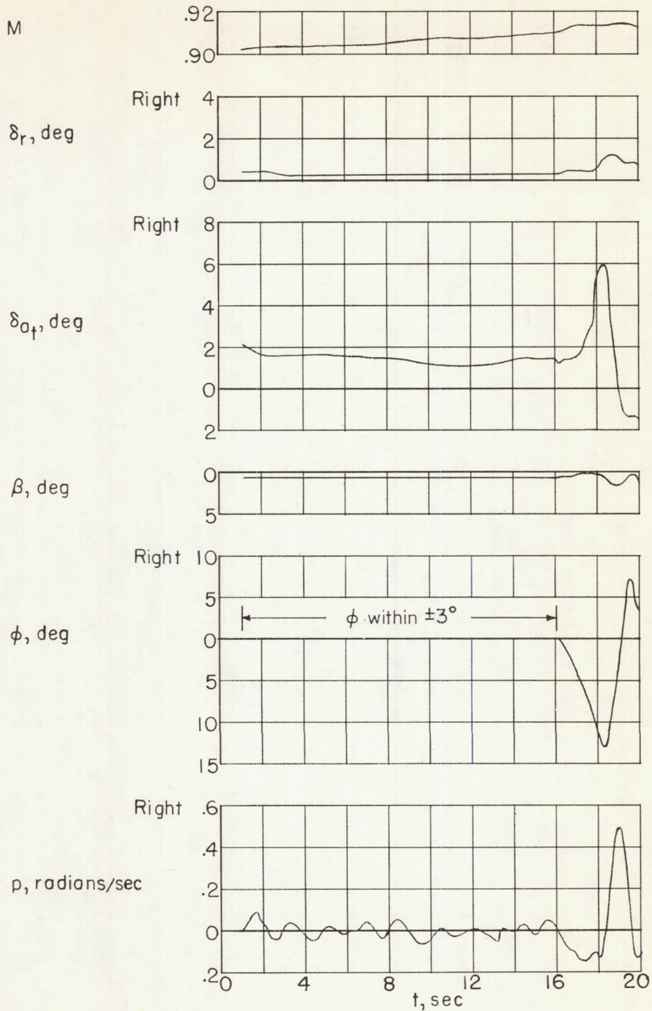
Figure 19.- Example of wing drooping at an altitude of 40,000 feet.
