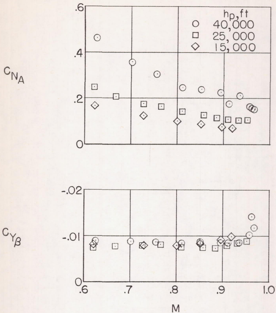
Figure 9.- Variation of C_{Y\beta} and C_{NA} determined in sideslip maneuvers at several altitudes.
