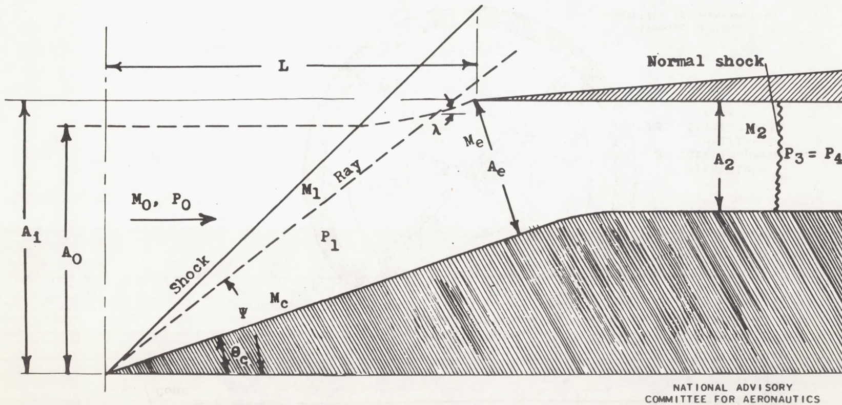
Figure 1.- Notation used at shock-diffuser inlet.
