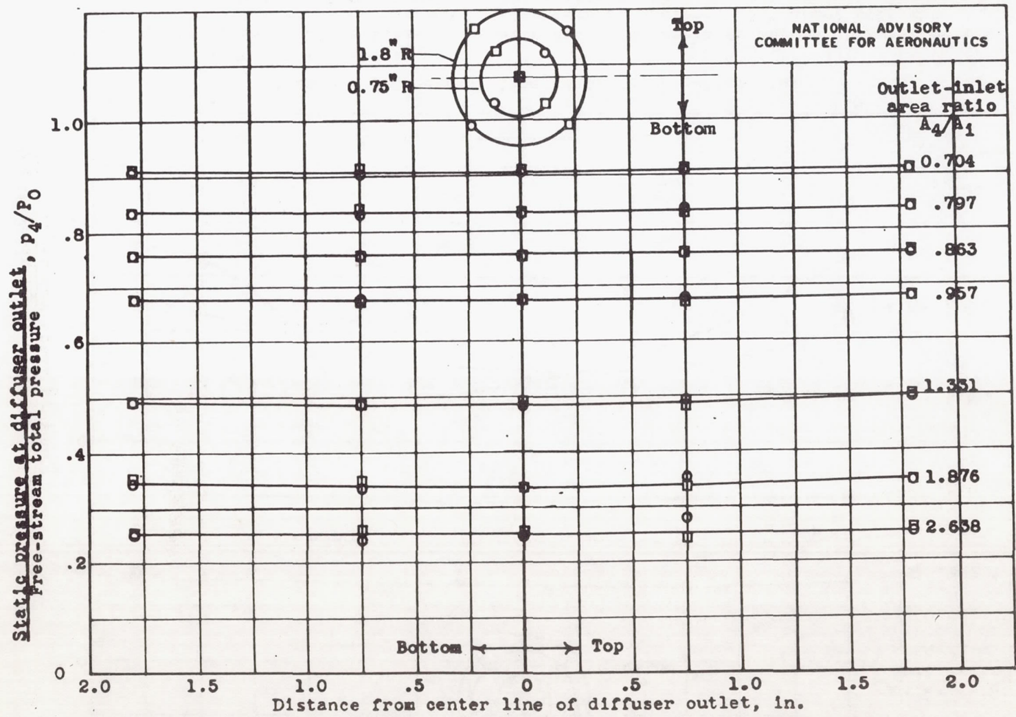
(a) Static-pressure distribution. Figure 7.- Distribution of static and total pressure across diffuser outlet with configuration yielding maximum total-pressure recovery. 50° cone; straight inlet; tip projection, 1.25 inches; angle of attack, 0°.
