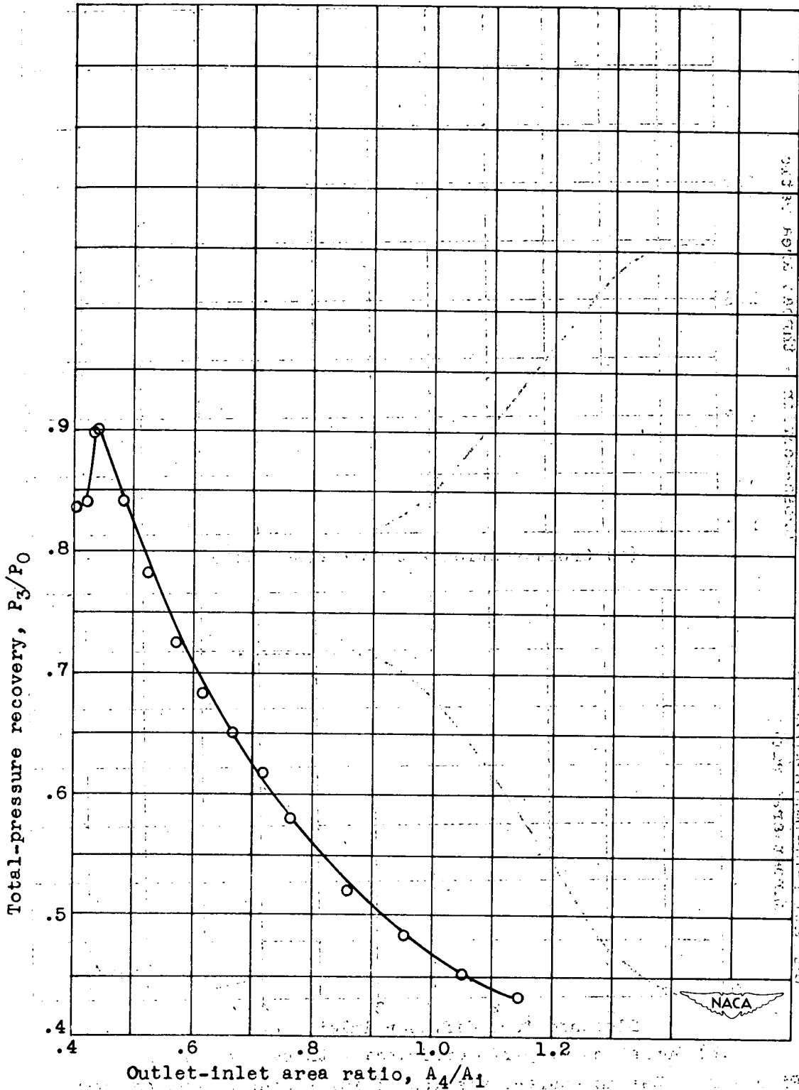
Figure 3. - Variation of total-pressure recovery with outlet-inlet area ratio without combustion.
