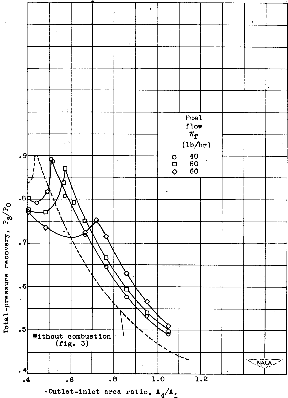
Figure 5. - Variation of total-pressure recovery with outlet-inlet area ratio for constant fuel flows.
