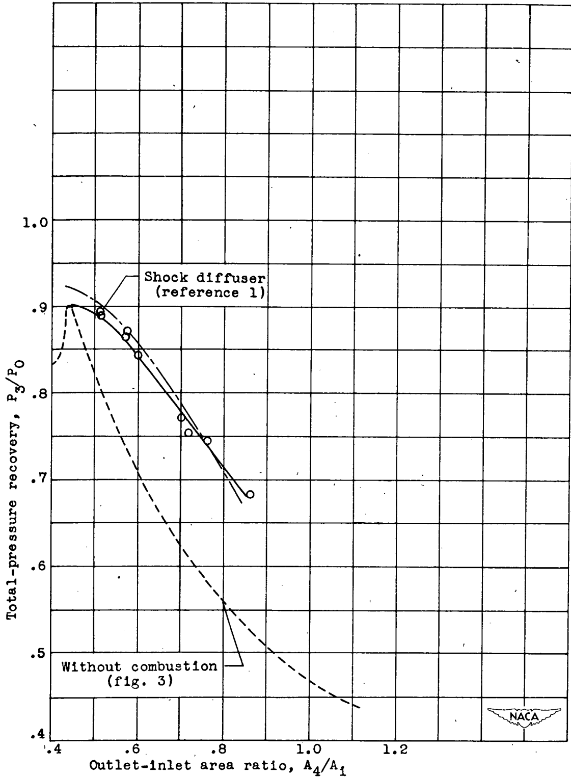
Figure 6. - Variation of peak total-pressure recovery with outlet-inlet-area ratio.
