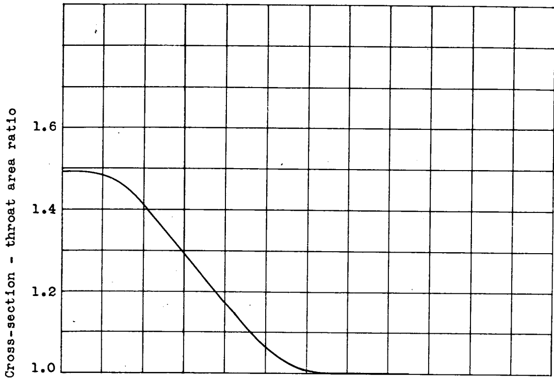
(a) Cross-section - throat area ratio.
