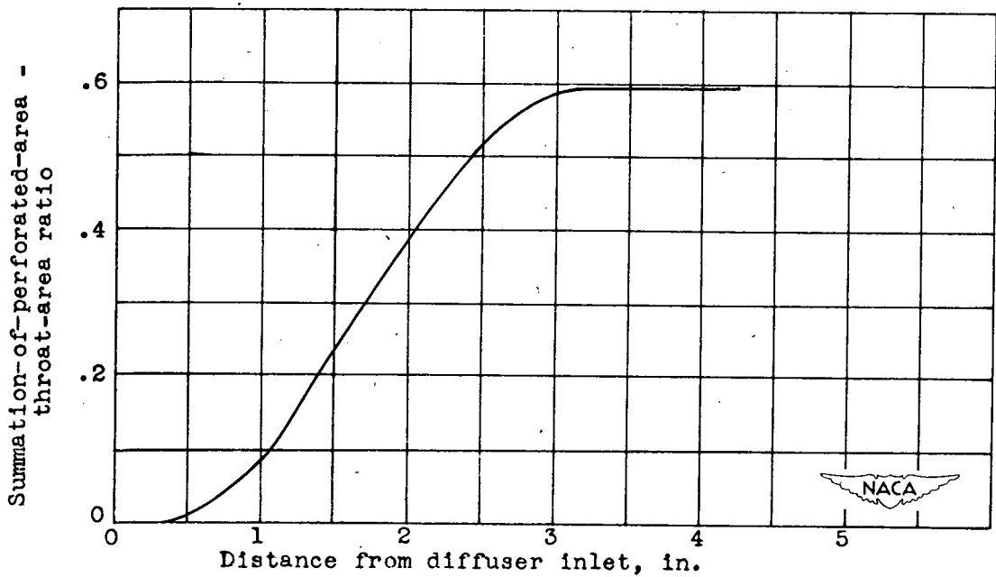
(b) Summation-of-perforated-area - throat-area ratio.
