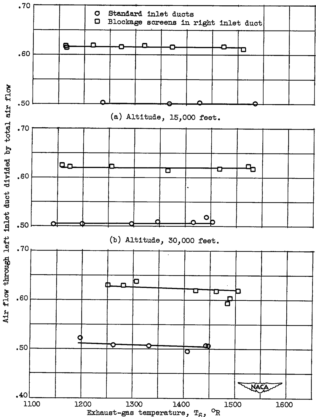
Figure 4. - Division of air flow between inlet ducts with and without blockage screens in right inlet duct.
