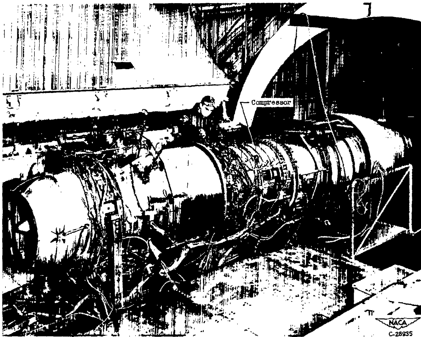
Figure 1. - Turbojet engine used for uneven air-flow-distribution study.
