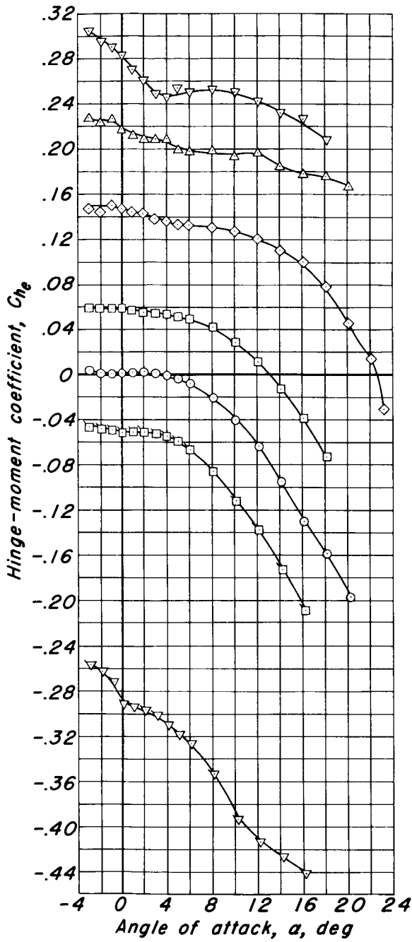
(b) C_{he} vs a , C_{ht} vs a
