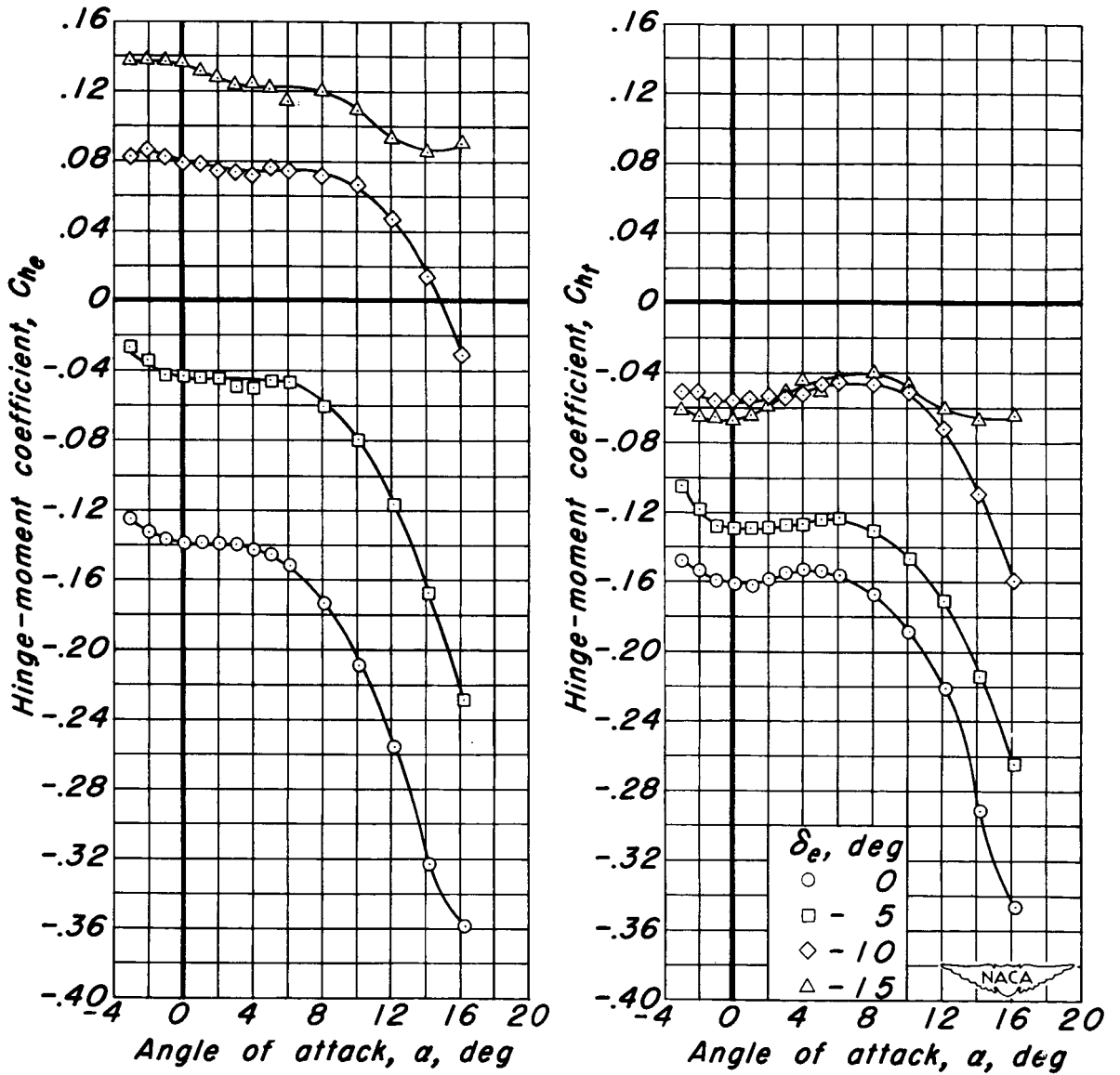
(b) C_{H_e} vs \alpha , C_{H_f} vs \alpha
