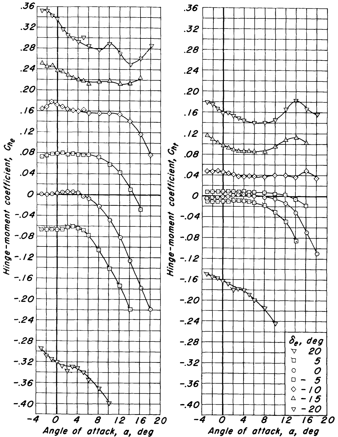
(b) C_{he} vs a , C_{hf} vs a
