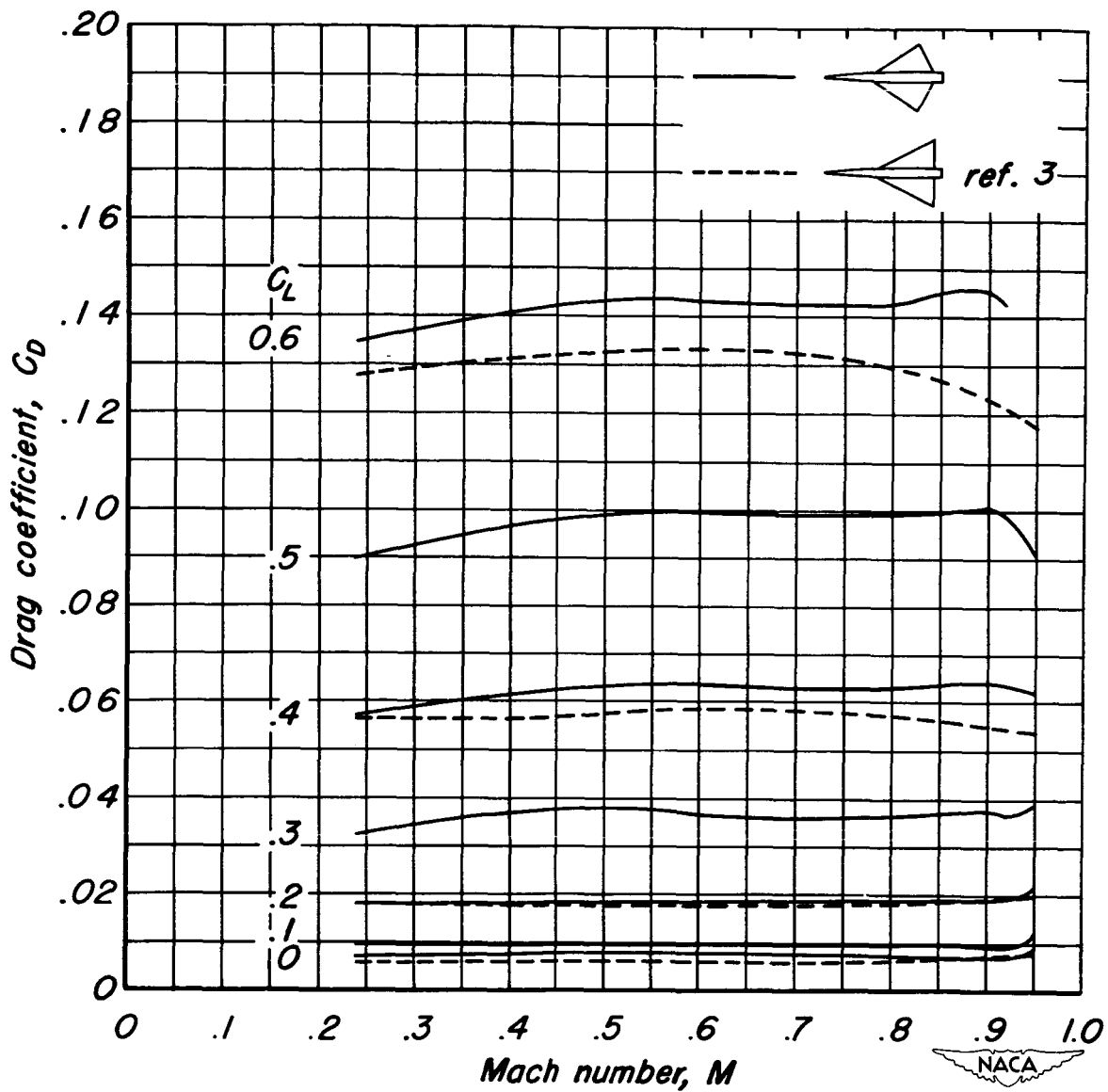
(e) C_D vs M
