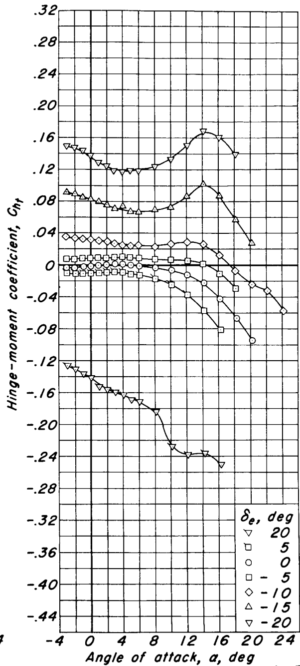
(b) C_{he} vs a , C_{ht} vs a
