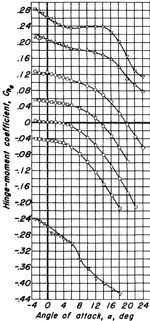
(b) C_{H_e} vs a , C_{H_f} vs a
