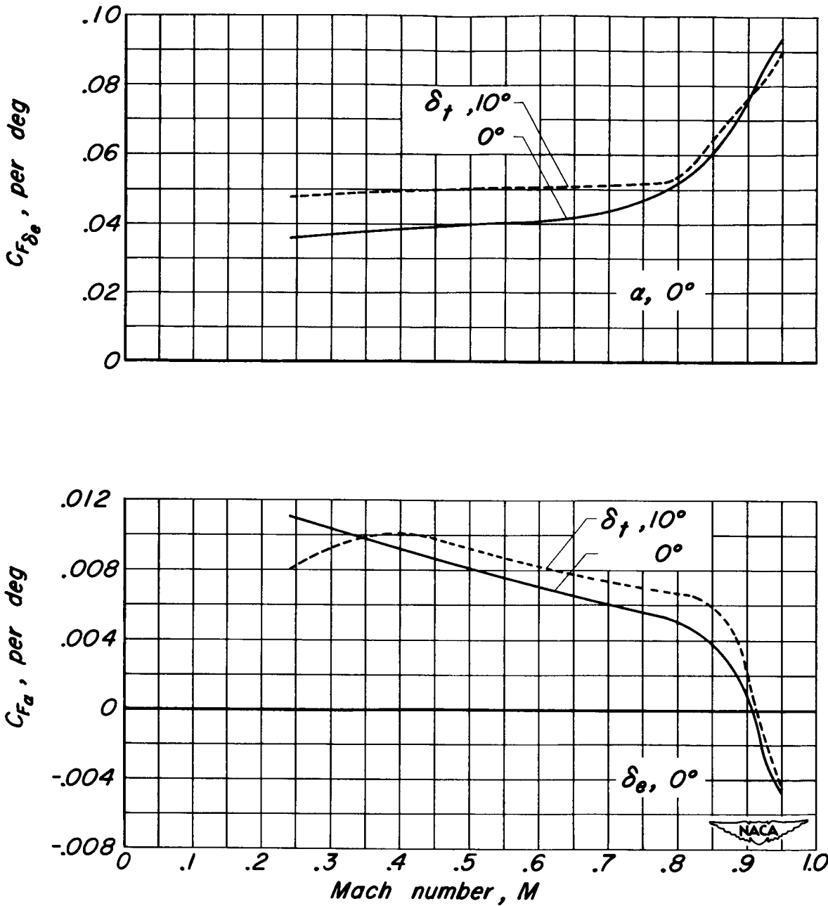
Figure 45.- The effect of Mach number on the elevator load parameters, C_{F_{\delta_e}} and C_{F_a} . R, 3.0 million.
