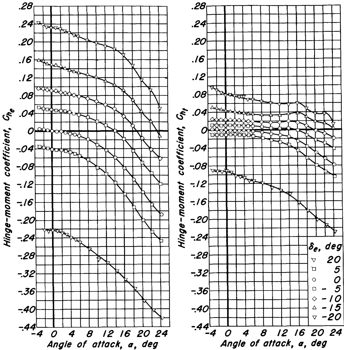
(b) C_{h_e} vs a , C_{h_f} vs a
