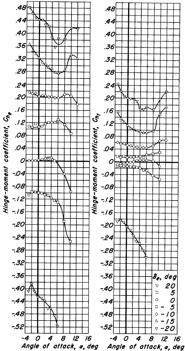
(b) C_{he} vs \alpha , C_{hh} vs \alpha
