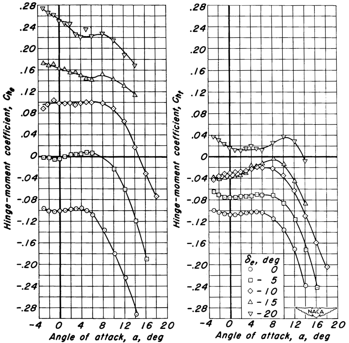
(b) C_{h_e} vs \alpha , C_{h_f} vs \alpha
