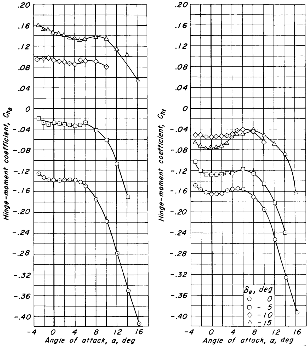
(b) C_{h_e} vs a , C_{h_t} vs a
