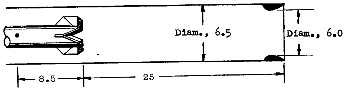
Combustor F
