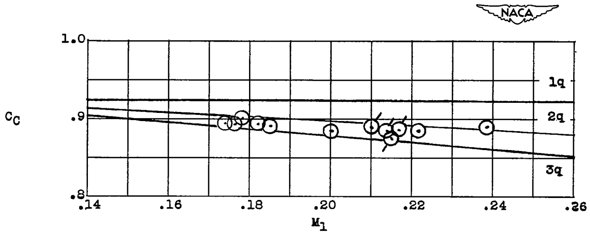
(b) A_4/A_3 = 1.28 , expanding exit.
