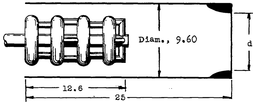
Combustor A
