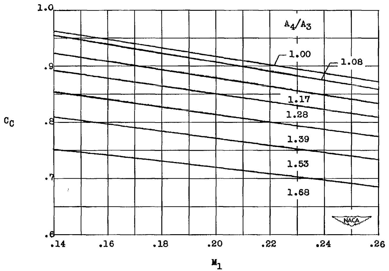
Figure 5.- The effect of expanding exit nozzle sizes on combustor-force coefficient C_C in a 4q combustor.
