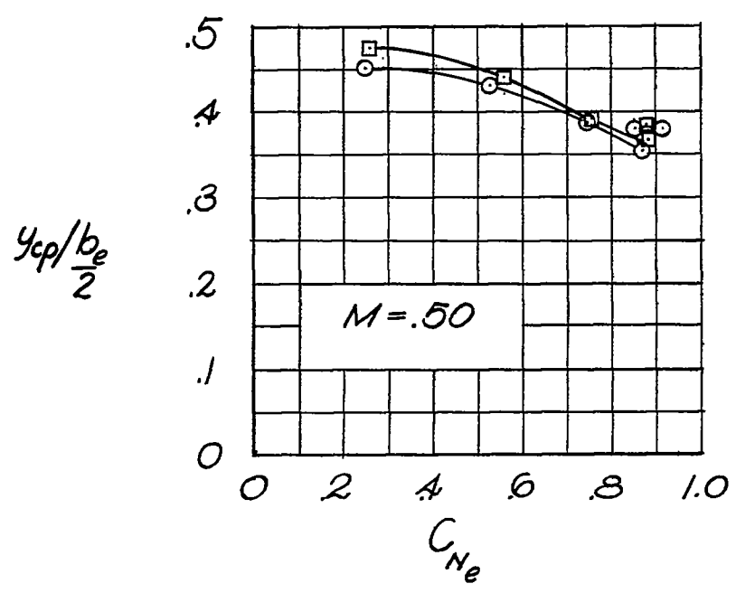
Figure 5.- Location of the lateral centers of pressure of the model without external stores and with the tip external stores.
