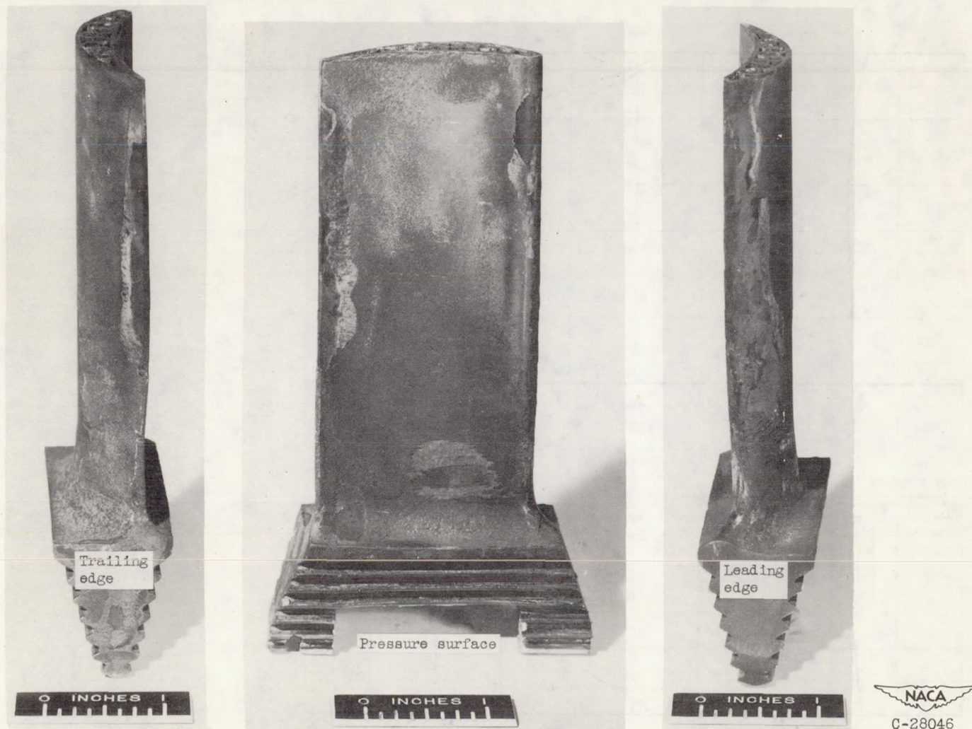
(a) Blade 1 after 7.3 hours (20 cycles plus 2.3 hours at rated test conditions) with coolant-flow ratio of 0.048. Complete breakdown of coating along leading and trailing edges evident.
