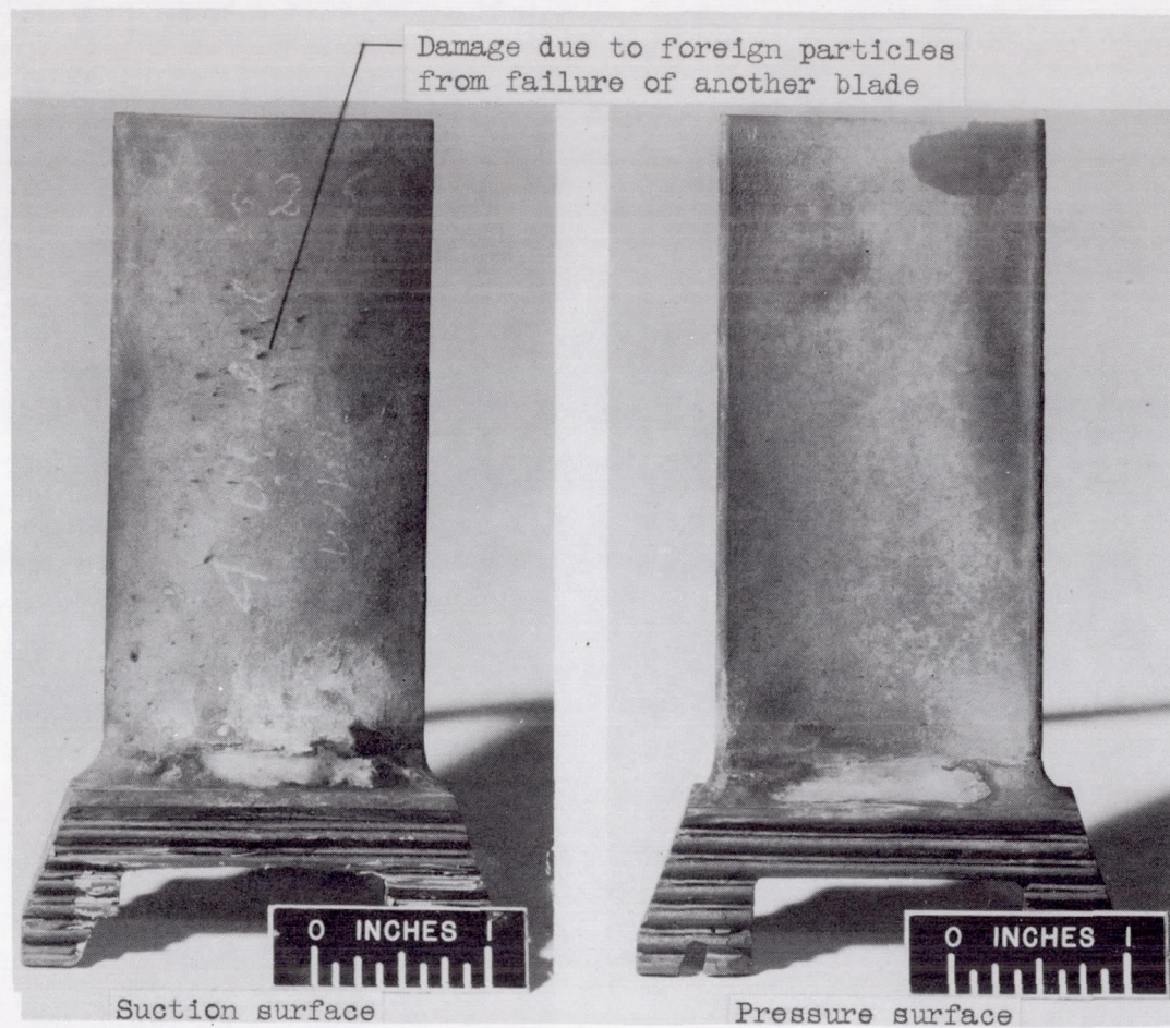
(a) Blade after 50 hours at rated test conditions with coolant-flow ratio of 0.048. Blade surfaces in excellent condition except where hit by foreign particles.
