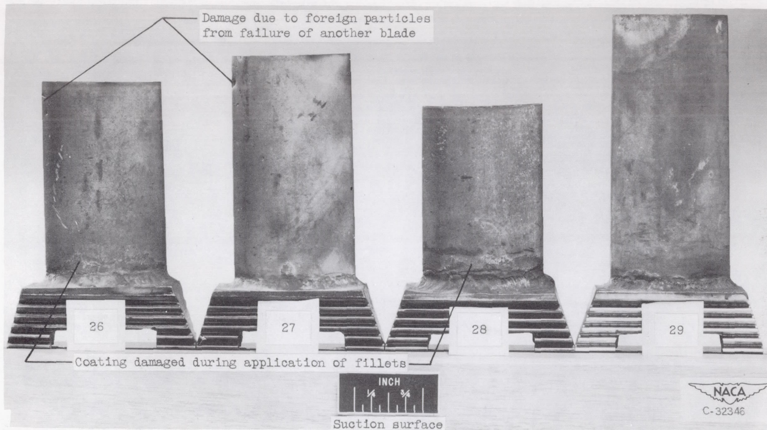
(a) Blades during early stages of endurance running with coolant-flow ratio of 0.03. Time on blades 26 and 27, 23.8 hours; on blade 28, 18.1 hours; on blade 29, no time. Surfaces in excellent condition.
