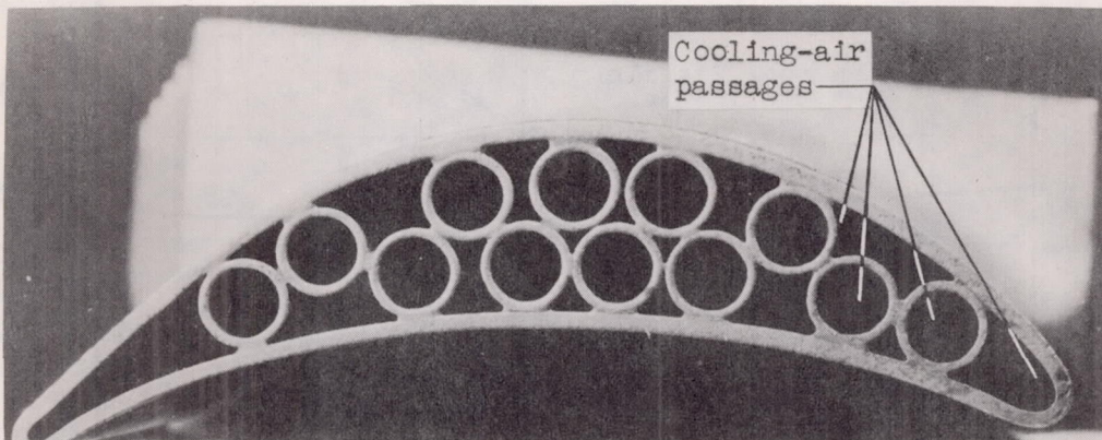
(a) Formed-shell blade with profile A.
