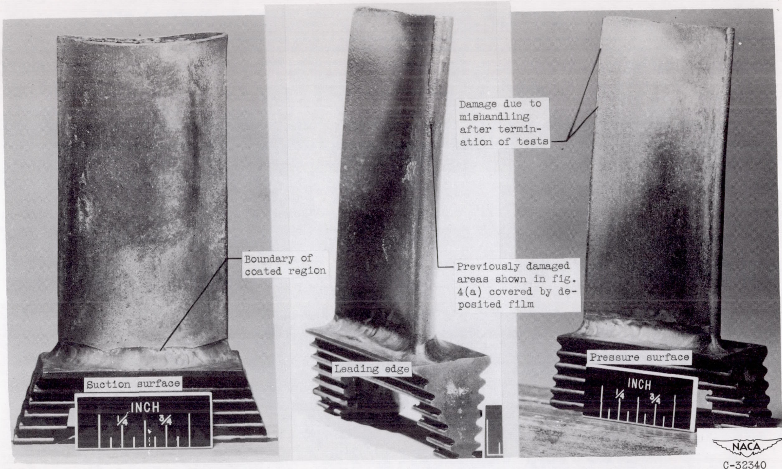
(b) Blade 5 after 100 hours at rated test conditions with coolant-flow ratio of 0.048. Coating in excellent condition except where hit by foreign objects.
