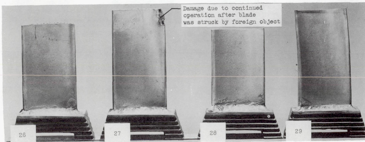
Pressure surface
