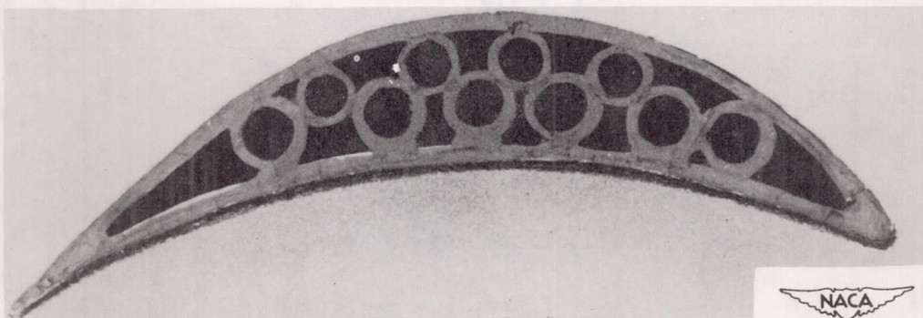
(c) Cast-shell blade with profile C.
