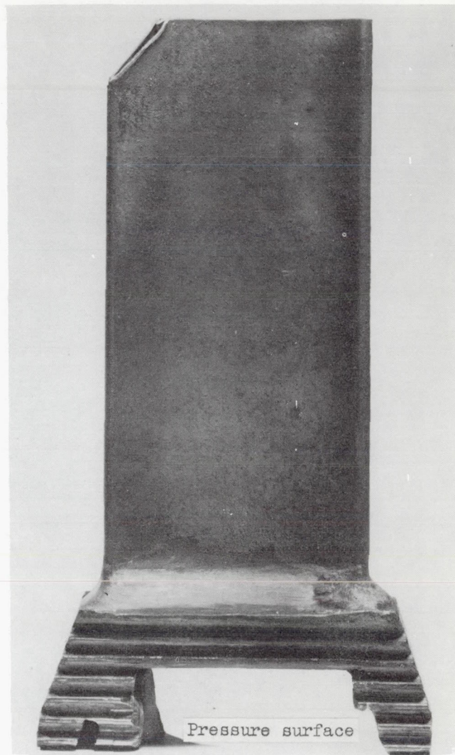
(b) Blade after 100 hours at rated test conditions with coolant-flow ratio of 0.048. Surfaces in excellent condition. Previously damaged areas shown on figure 7(a) indistinguishable from adjoining surfaces.
