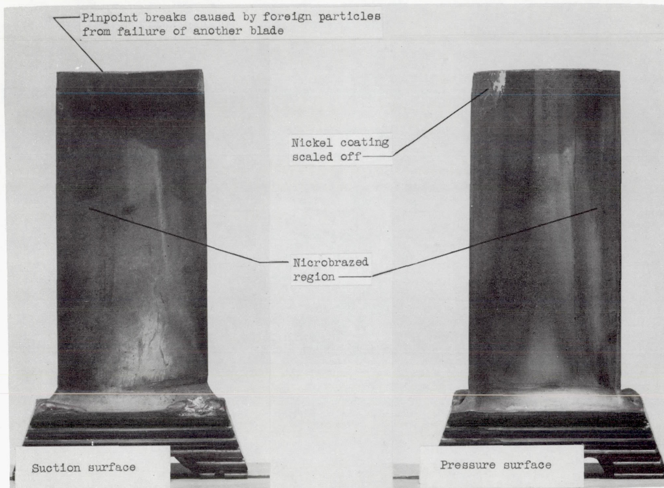
Figure 6. - Nickel-coated blade 20 with Microbraz along leading edge. Blade after 100 hours at rated test conditions with coolant-flow ratio of 0.048. Leading edge and midchord region in excellent condition.
