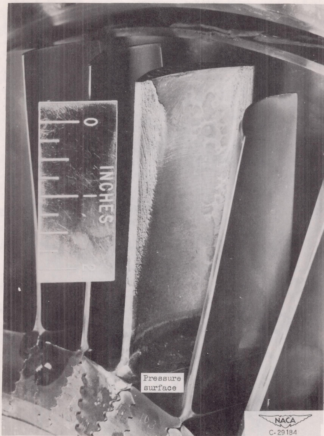
(b) Blade 2 after 4.8 hours at rated test conditions with coolant-flow ratio of 0.048. Coating softened and flowed toward tip.
